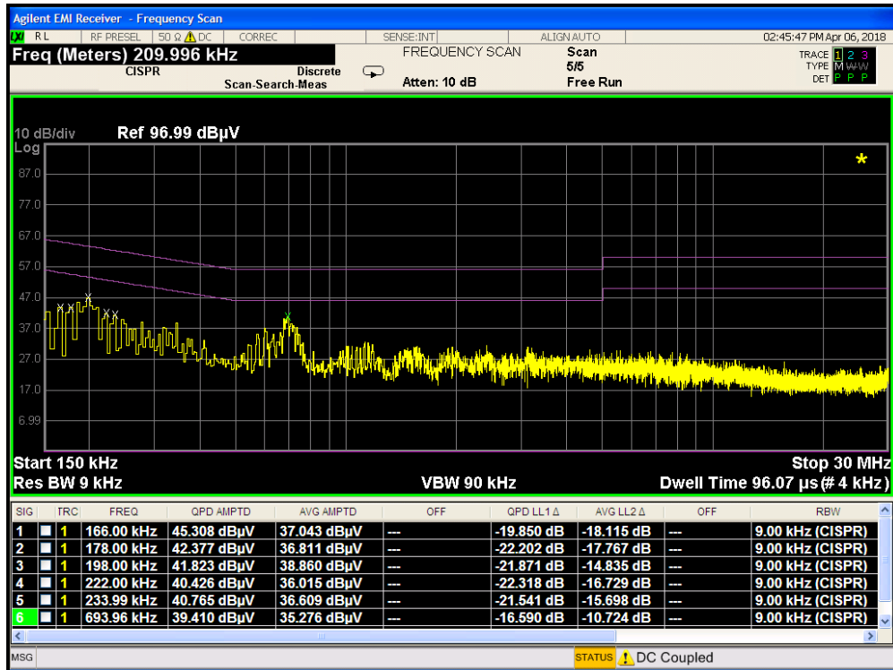
Plot 7-37. Line Conducted Plot Bluetooth with Travel Adapter LE (L1)
