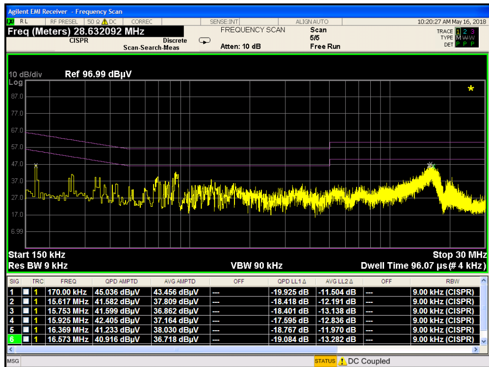
Plot 7-40. Line Conducted Plot Bluetooth LE with Wireless Charging Pad (N)
