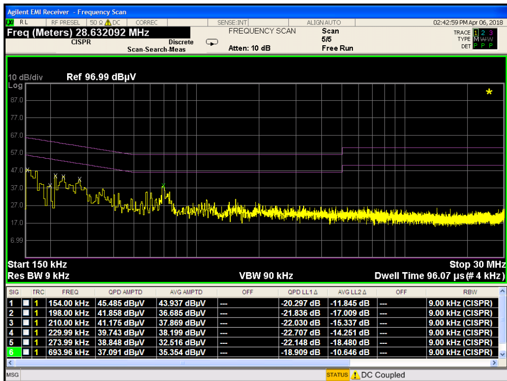
Plot 7-38. Line Conducted Plot Bluetooth LE with Travel Adapter (N)
