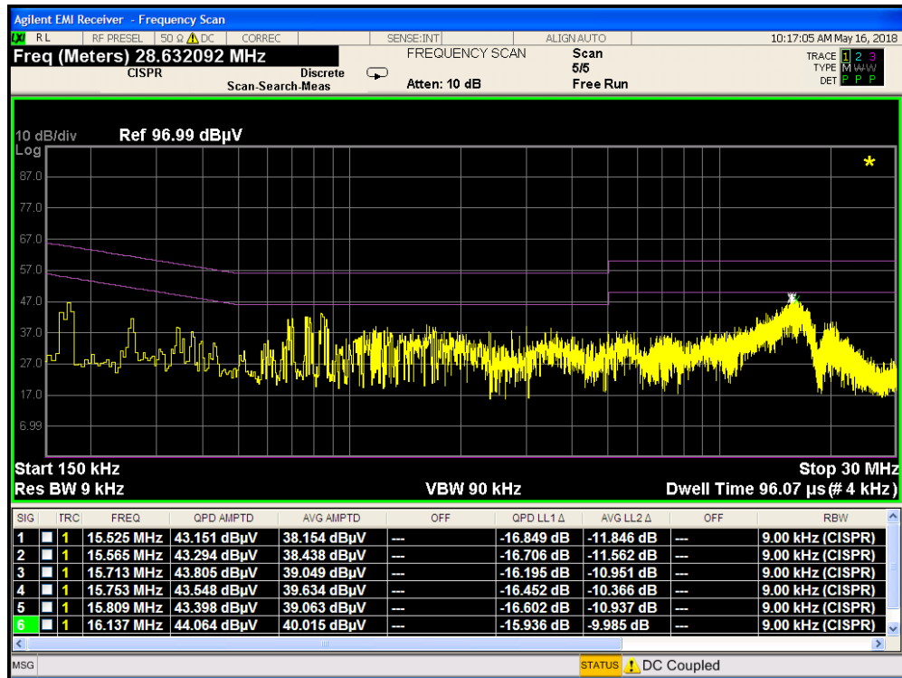
Plot 7-39. Line Conducted Plot Bluetooth LE with Wireless Charging Pad (L1)
