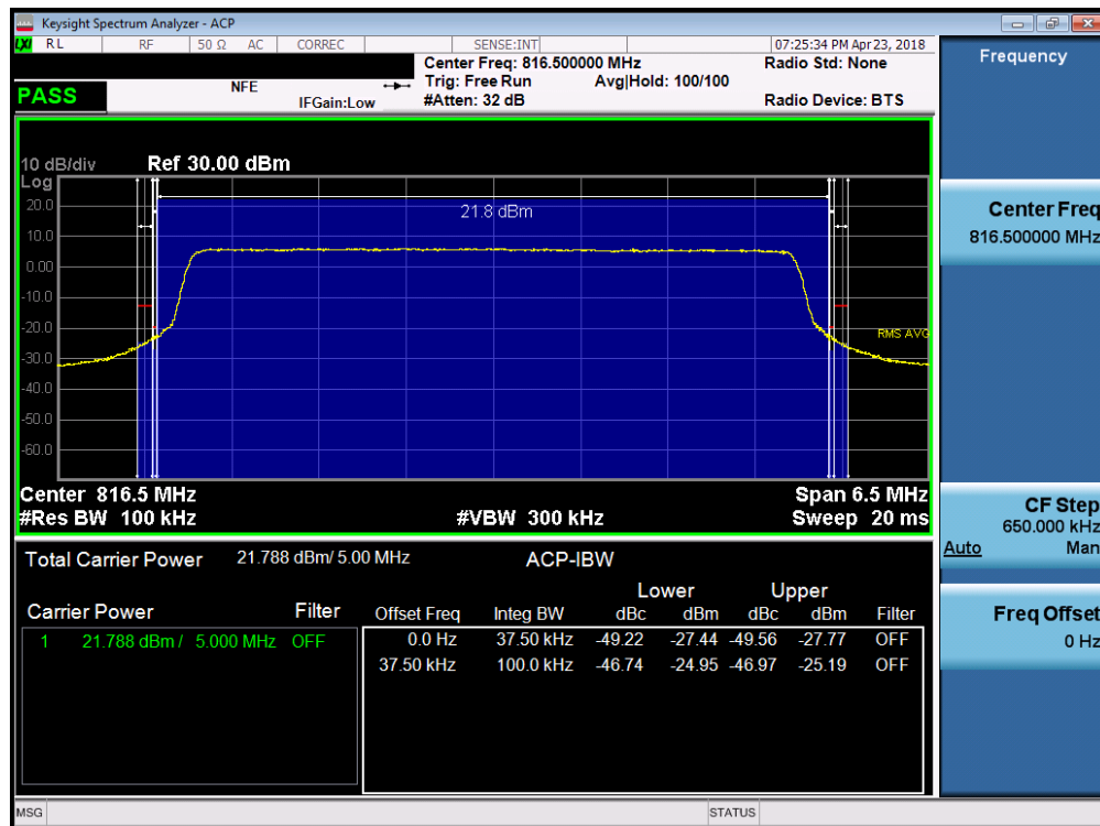
Plot 7-26. Channel Edge Plot (5MHz QPSK – RB Size 25– Low Channel)
