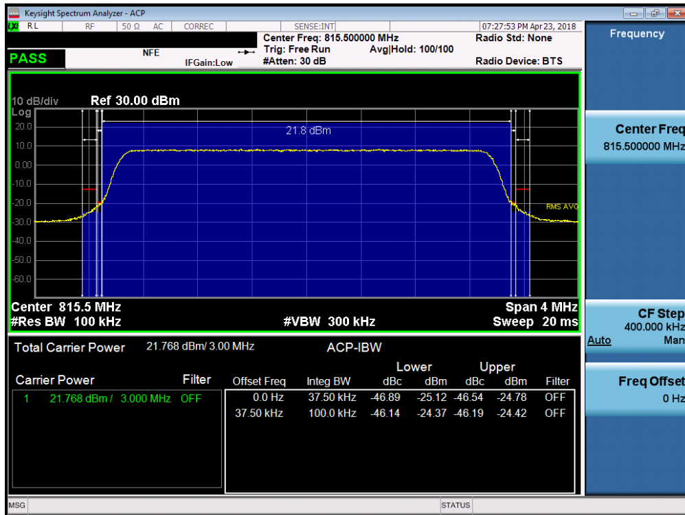
Plot 7-24. Channel Edge Plot (3MHz QPSK – RB Size 15– Low Channel)
