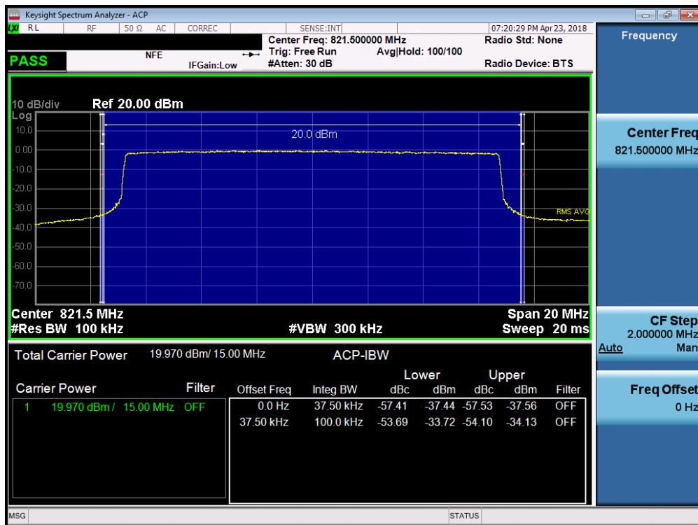
Plot 7-29. Channel Edge Plot (15MHz QPSK – RB Size 75)
