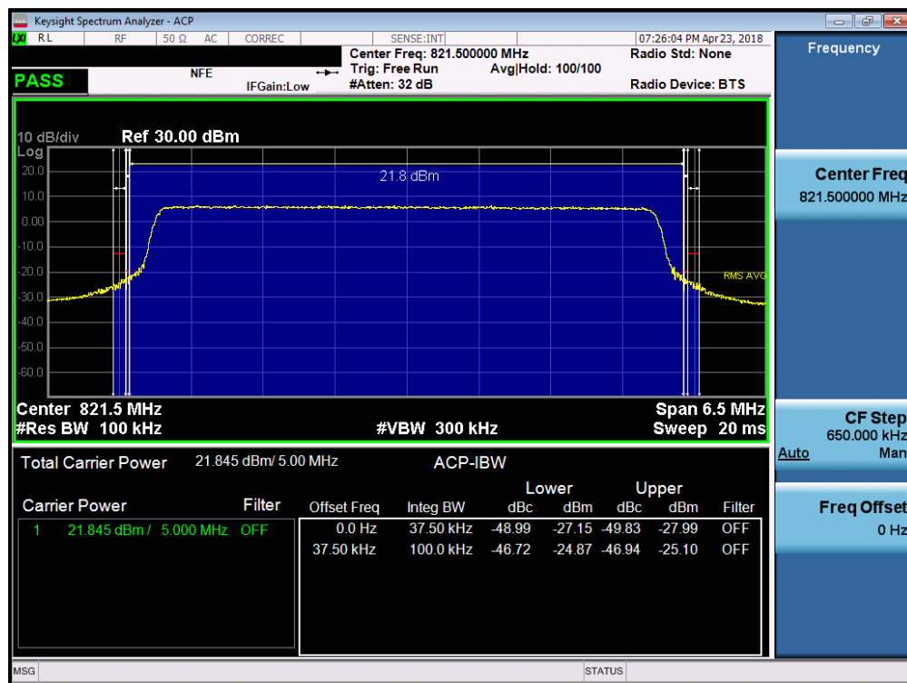
Plot 7-27. Channel Edge Plot (5MHz QPSK – RB Size 25 – High Channel)
