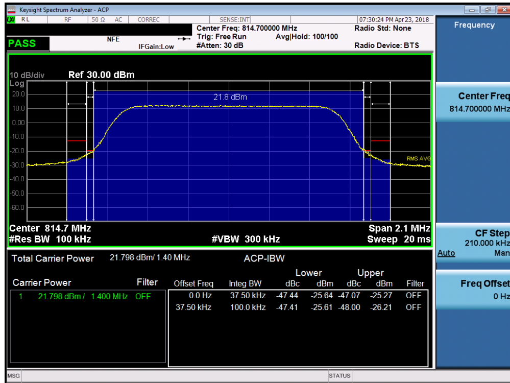
Plot 7-22. Channel Edge Plot (1.4MHz QPSK – RB Size 6– Low Channel)
