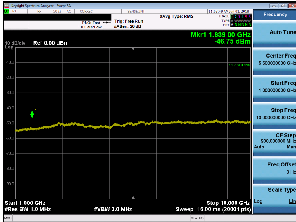
Plot 7-21. Conducted Spurious Plot ( 5MHz QPSK – RB Size 1, RB Offset 0 – High Channel)
