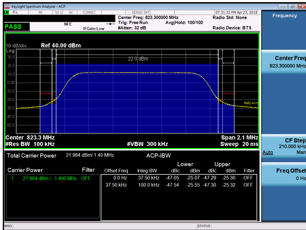
Plot 7-23. Channel Edge Plot (1.4MHz QPSK – RB Size 6 – High Channel)
