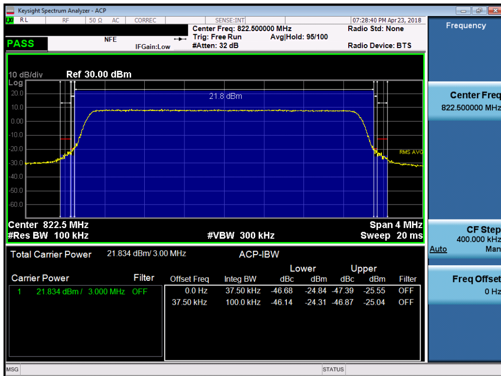
Plot 7-25. Channel Edge Plot (3MHz QPSK – RB Size 15 – High Channel)
