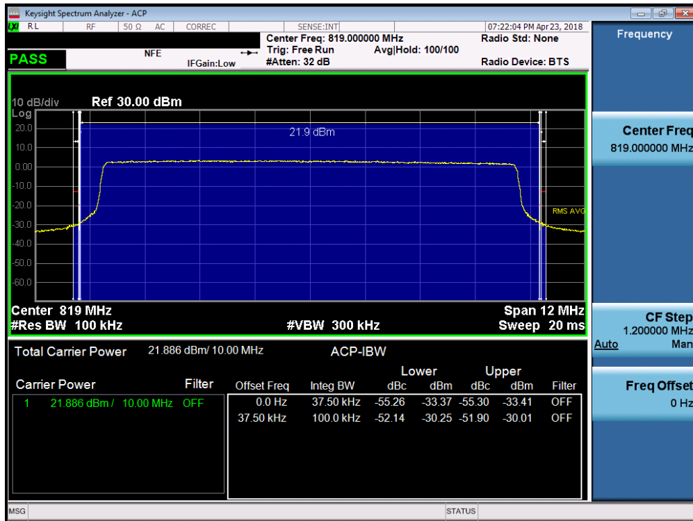
Plot 7-28. Channel Edge Plot (10MHz QPSK – RB Size 50)
