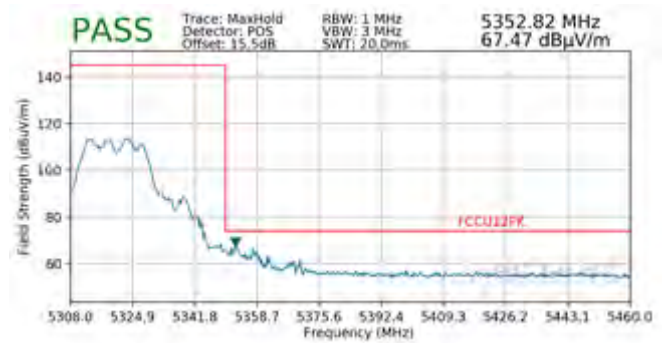
Plot 7-267. Radiated Band Edge Plot (Peak – WCP)
