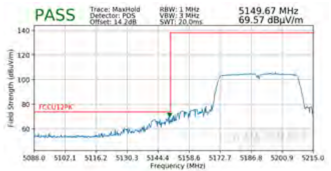
Plot 7-195. Radiated Band Edge Plot (Peak – WCP)
