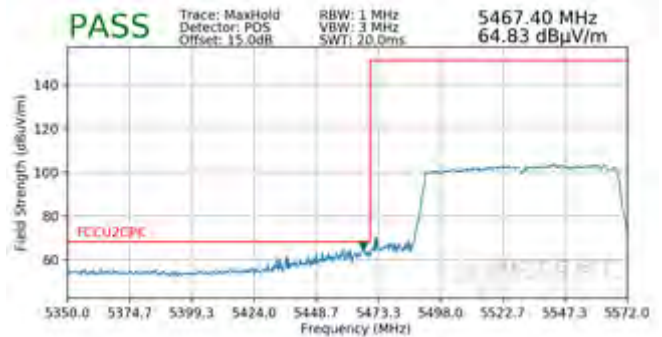
Plot 7-255. Radiated Lower Band Edge Plot (Peak – UNII Band 2C)
