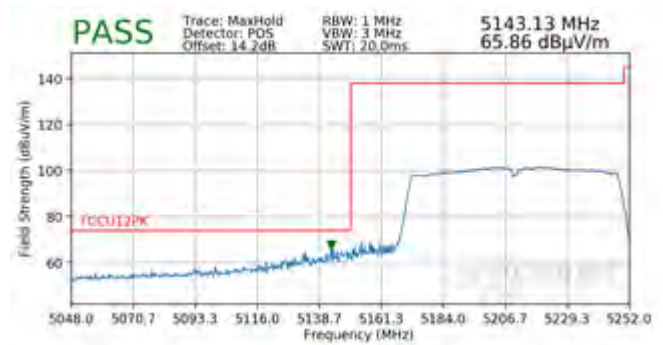
Plot 7-204. Radiated Band Edge Plot (Peak – WCP)
