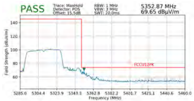
Plot 7-222. Radiated Band Edge Plot (Peak – WCP)
