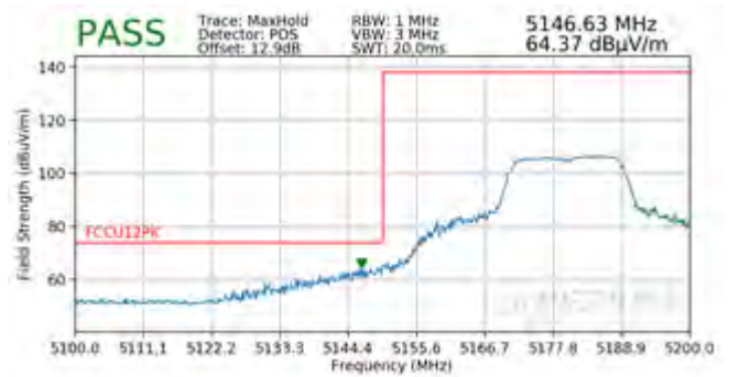
Plot 7-186. Radiated Band Edge Plot (Peak – WCP)
