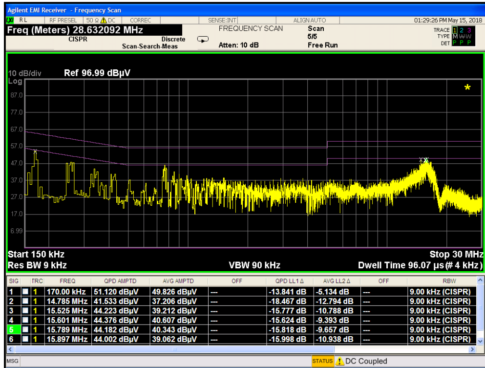
Plot 7-97. Line Conducted Plot 802.11b with Wireless Charging Pad (L1)
