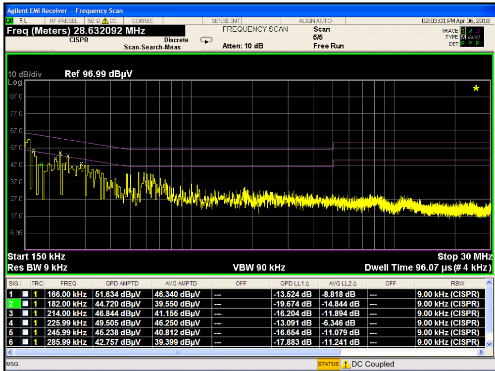
Plot 7-96. Line Conducted Plot 802.11b with Travel Adapter (N)
