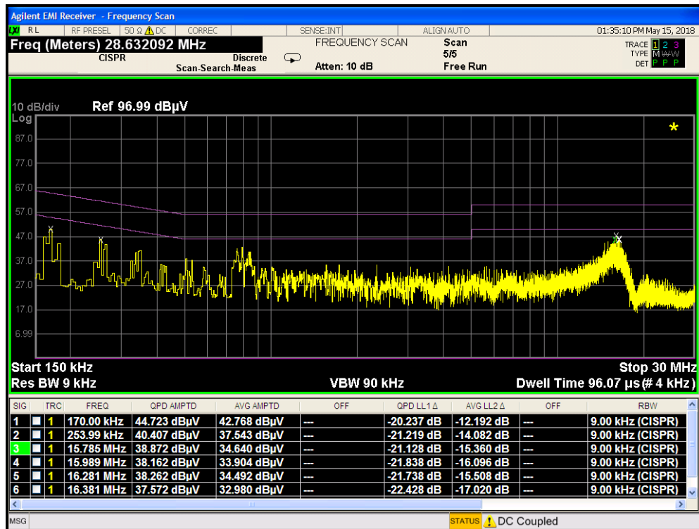
Plot 7-98. Line Conducted Plot 802.11b with Wireless Charging Pad (N)
