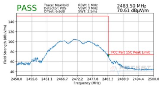
Plot 7-92. Radiated Restricted Band Edge Measurement CDD with WCP (Peak)
