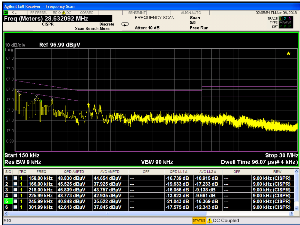
Plot 7-95. Line Conducted Plot 802.11b with Travel Adapter (L1)
