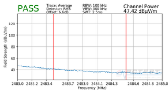
Plot 7-91. Radiated Restricted Band Edge Measurement CDD with WCP (Average)
