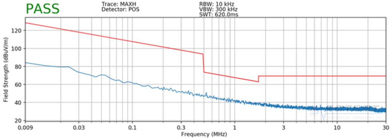
Plot 7-8. Inductive Coupling Mode #3 Spurious Plot 9kHz – 30MHz (Pol. Y)
