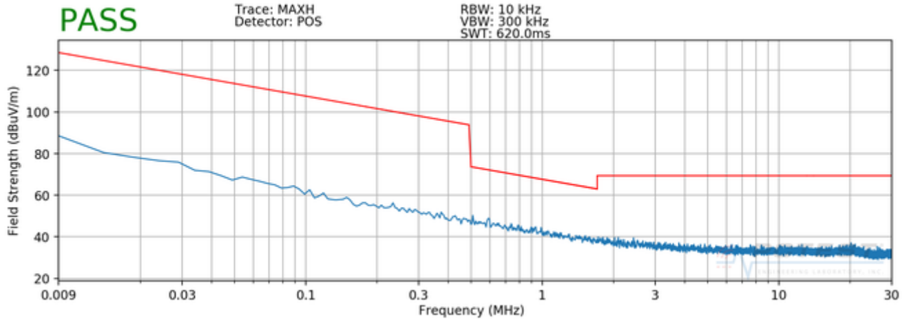
Plot 7-2. Inductive Coupling Mode #1 Radiated Spurious Plot 9kHz – 30MHz (Pol. Y)
