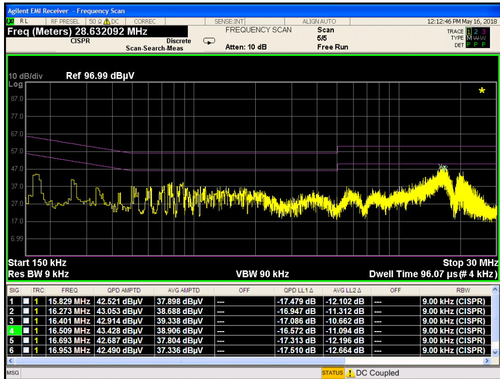
Plot 7-11. Line-Conducted Test Plot with Travel Adapter (N)
