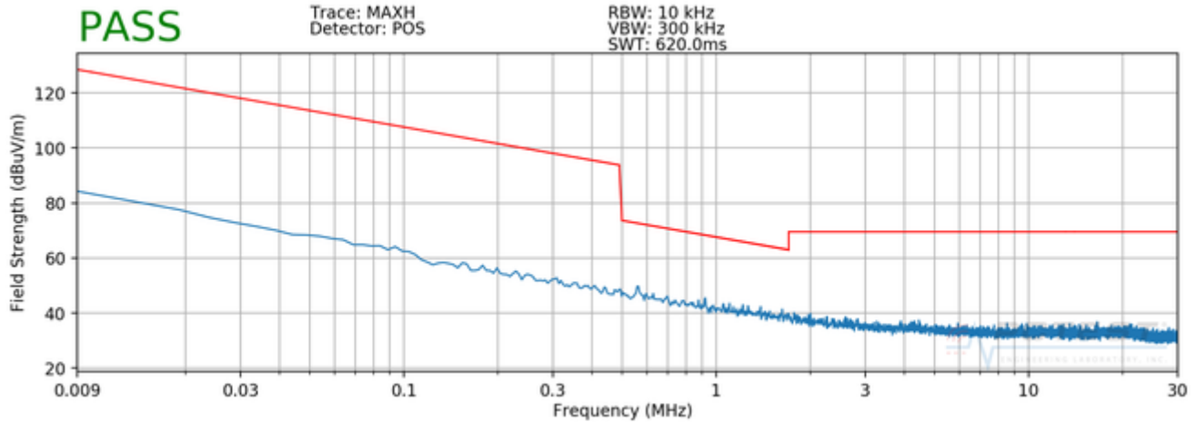
Plot 7-5. Inductive Coupling Mode #2 Radiated Spurious Plot 9kHz – 30MHz (Pol. Y)
