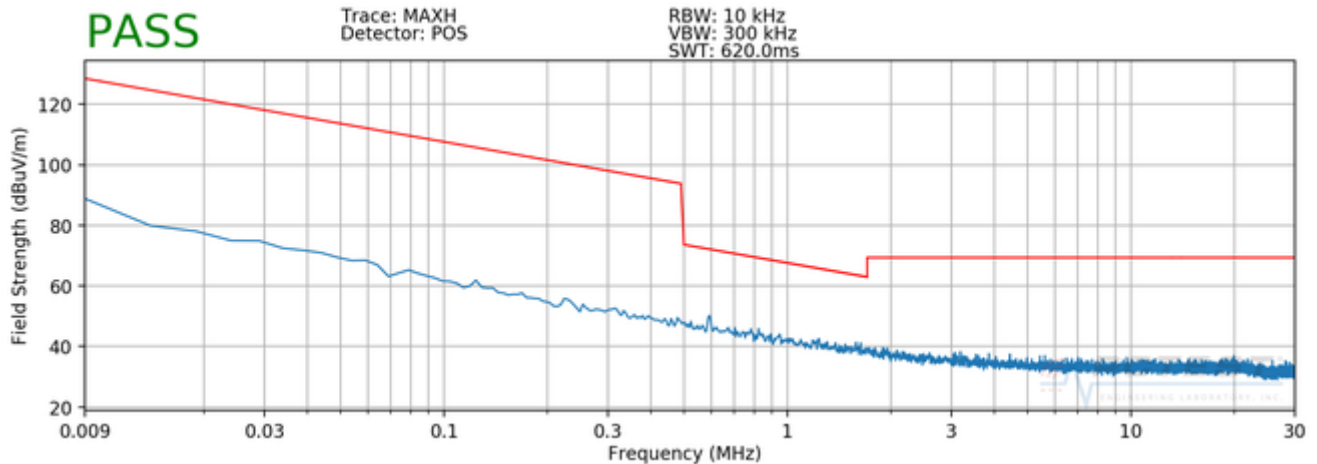
Plot 7-3. Inductive Coupling Mode #1 Radiated Spurious Plot 9kHz – 30MHz (Pol. Z)
