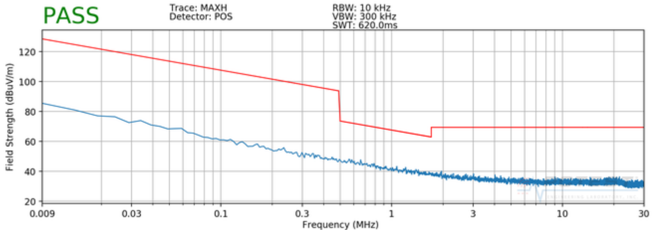
Plot 7-6. Inductive Coupling Mode #2 Radiated Spurious Plot 9kHz – 30MHz (Pol. Z)
