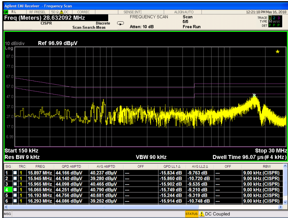
Plot 7-12. Line-Conducted Test Plot with Wireless Charging Pad (L1)
