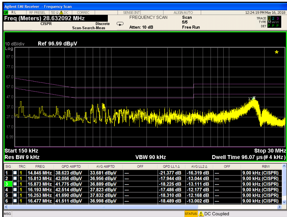
Plot 7-13. Line-Conducted Test Plot with Wireless Charging Pad (N)
