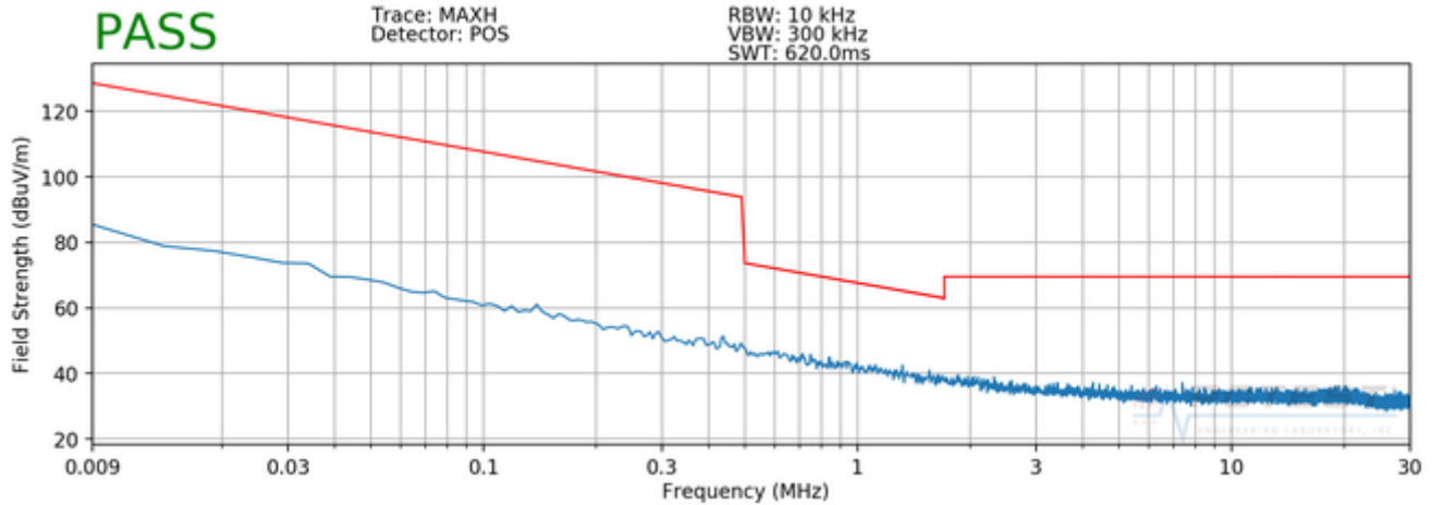
Plot 7-7. Inductive Coupling Mode #3 Radiated Spurious Plot 9kHz – 30MHz (Pol. X)
