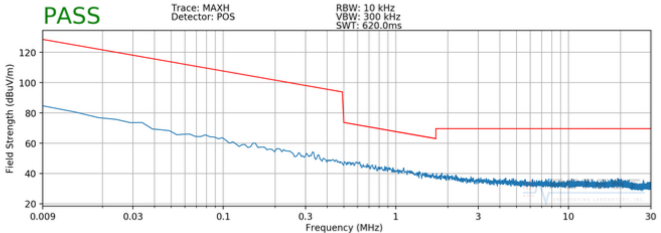
Plot 7-9. Inductive Coupling Mode #3 Radiated Spurious Plot 9kHz – 30MHz (Pol. Z)
