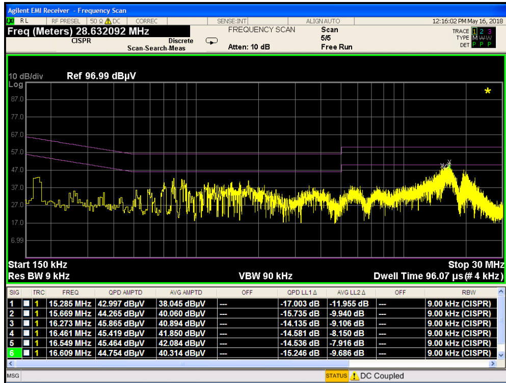
Plot 7-10. Line-Conducted Test Plot with Travel Adapter (L1)
