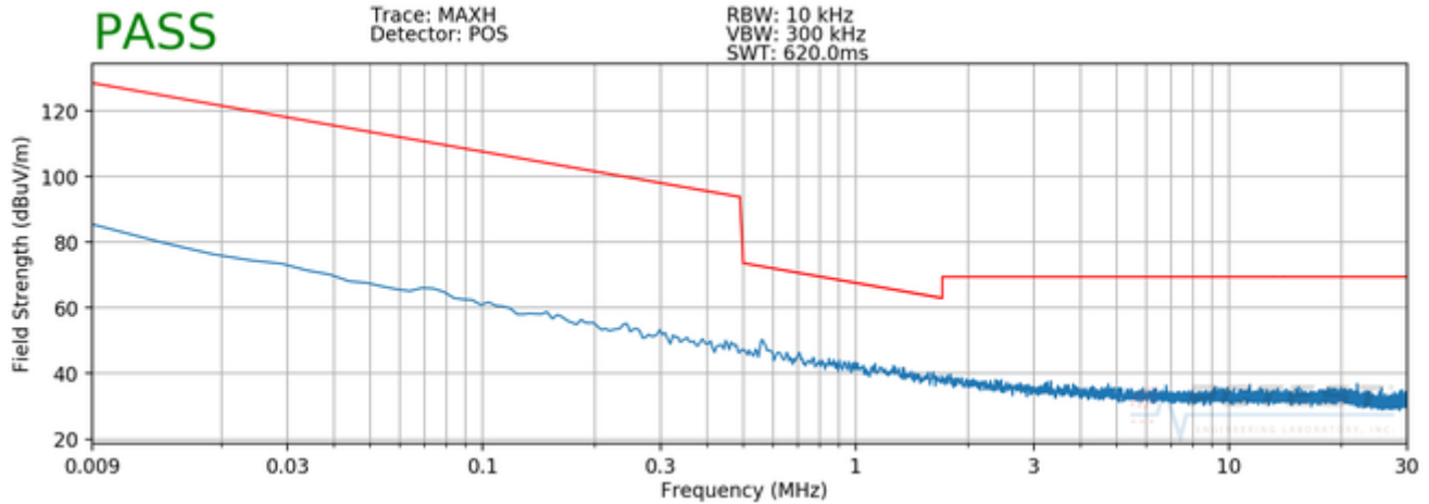
Plot 7-4. Inductive Coupling Mode #2 Radiated Spurious Plot 9kHz – 30MHz (Pol. X)
