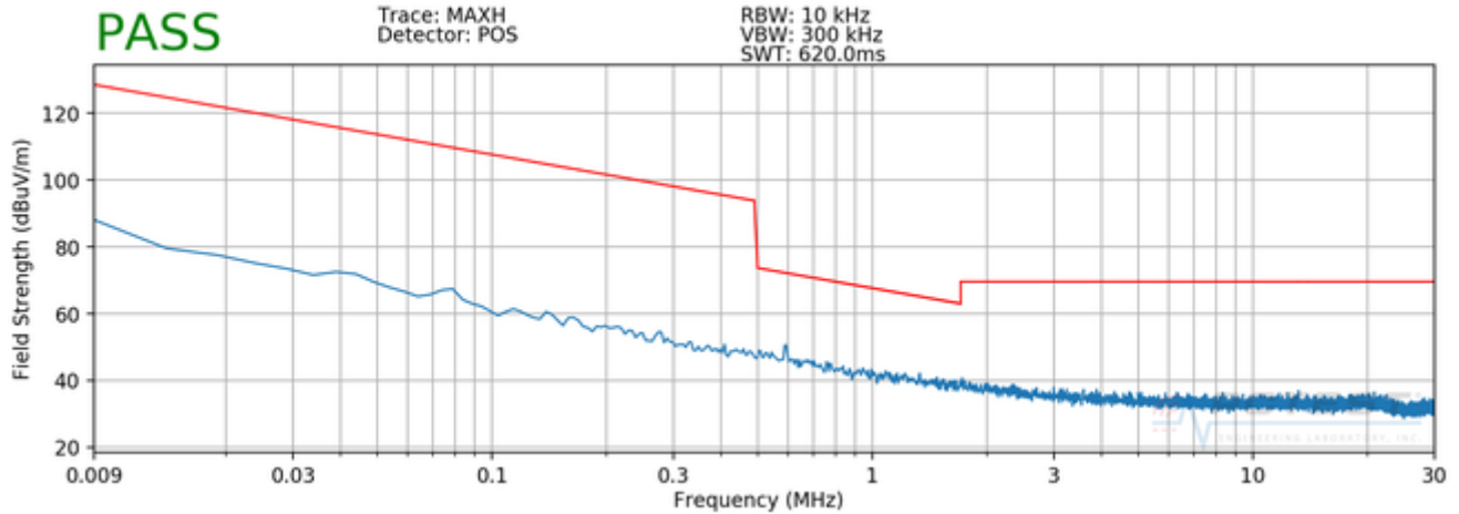
Plot 7-1. Inductive Coupling Mode #1 Radiated Spurious Plot 9kHz – 30MHz (Pol. X)
