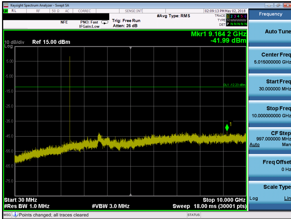
Plot 7-29. Conducted Spurious Plot (Bluetooth (LE), 2Mbps - Ch. 0)
