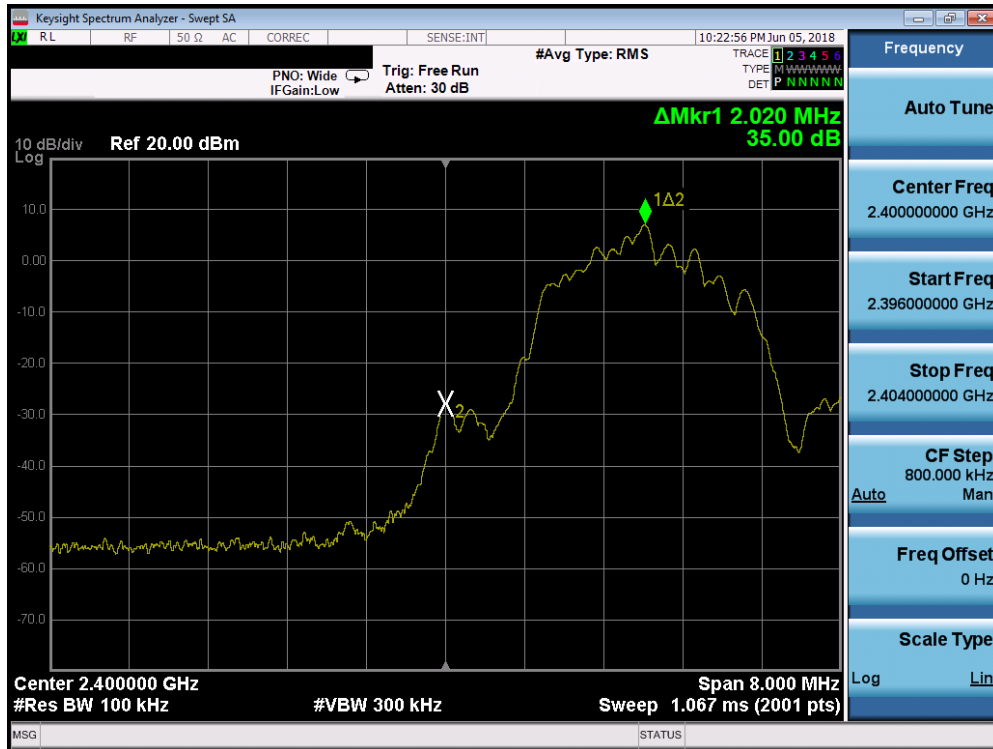
Plot 7-21. Band Edge Plot (Bluetooth (LE), 2Mbps – Ch. 0)
