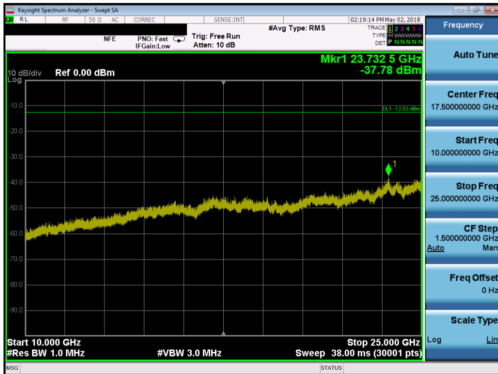
Plot 7-34. Conducted Spurious Plot (Bluetooth (LE), 2Mbps – Ch. 39)
