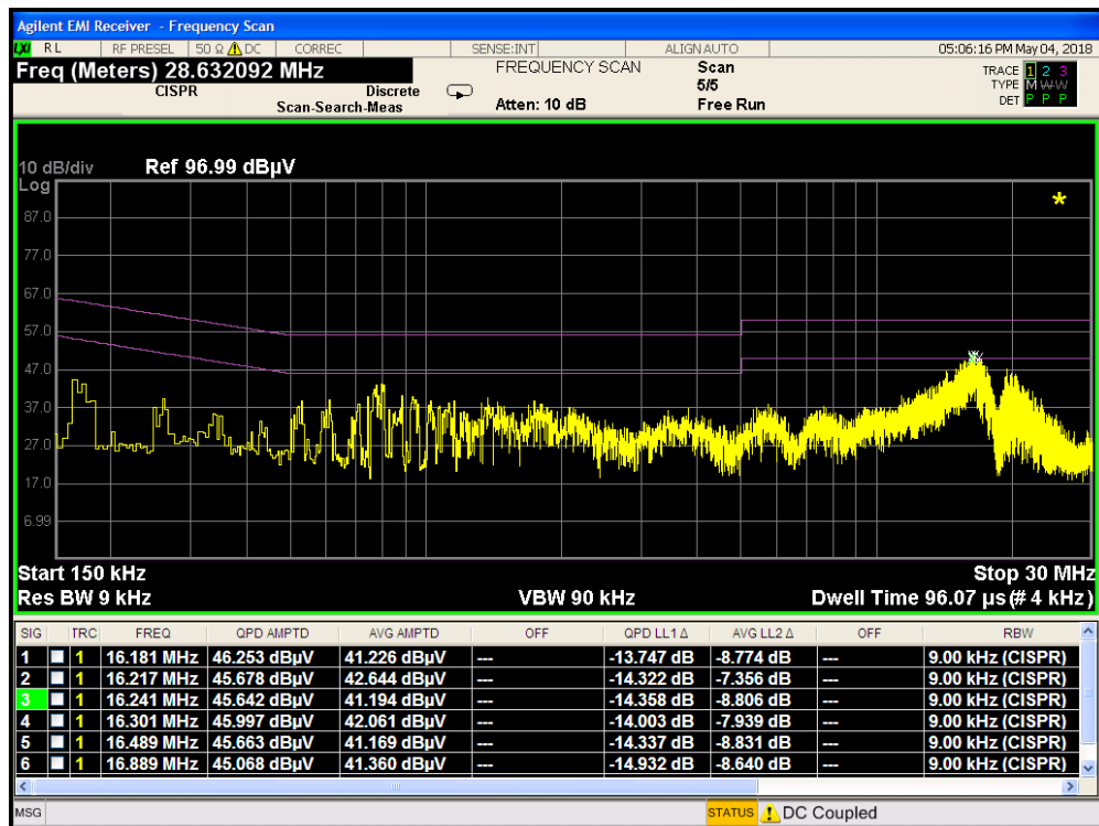
Plot 7-40. Line Conducted Plot with Bluetooth LE (N) with Travel Adapter
