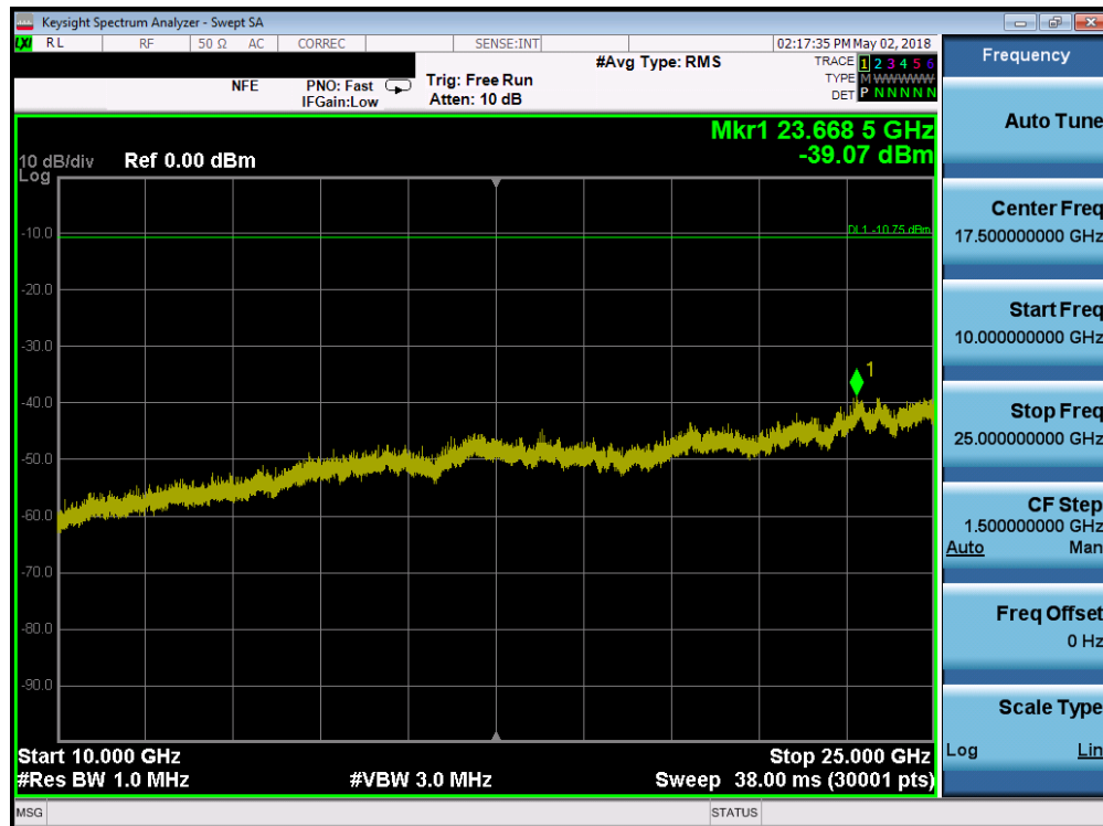
Plot 7-32. Conducted Spurious Plot (Bluetooth (LE), 2Mbps – Ch. 19)
