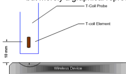
Figure 4-10 Measurement Distance
