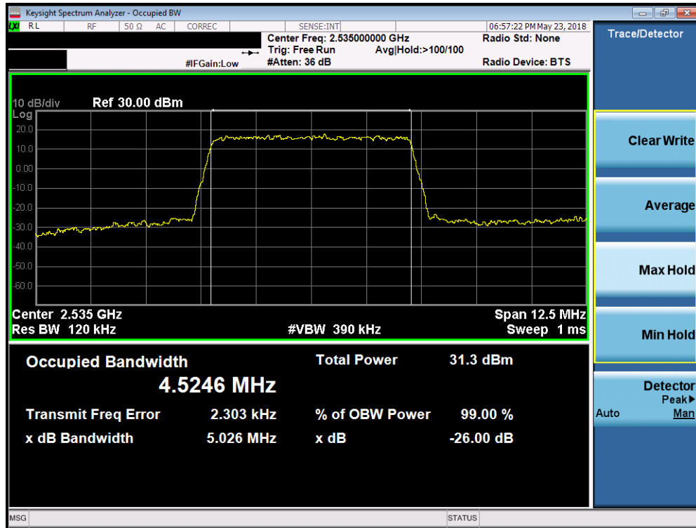
Plot 7-106. Occupied Bandwidth Plot (Band 7 - 5.0MHz QPSK - Full RB Configuration)
