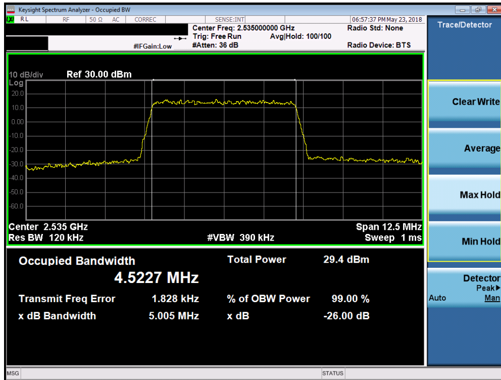
Plot 7-108. Occupied Bandwidth Plot (Band 7 - 5.0MHz 64-QAM - Full RB Configuration)
