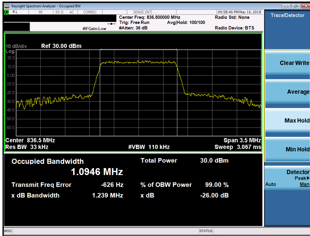
Plot 7-33. Occupied Bandwidth Plot (Band 26/5 - 1.4MHz 64-QAM - Full RB Configuration)
