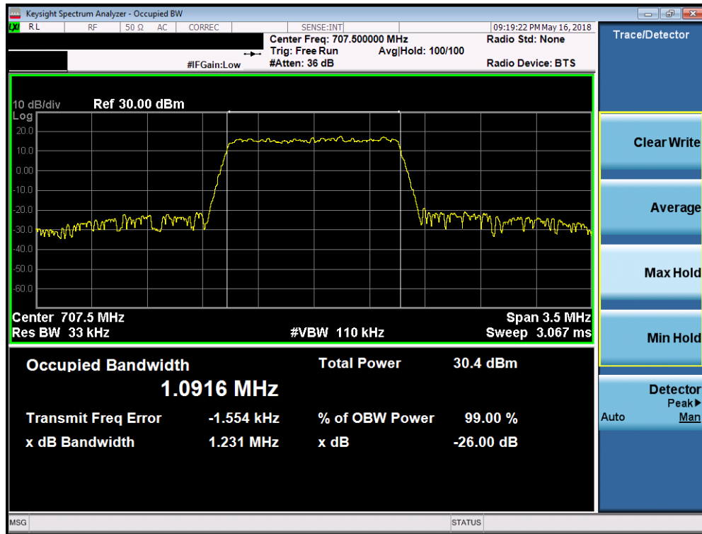
Plot 7-15. Occupied Bandwidth Plot (Band 12 - 1.4MHz 64-QAM - Full RB Configuration)
