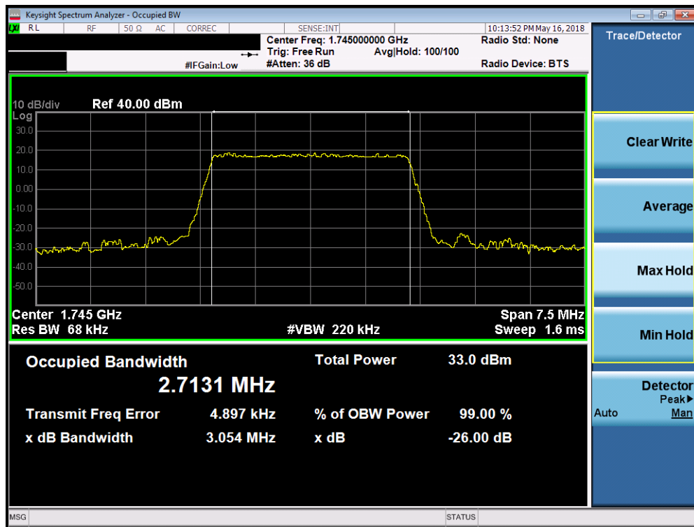
Plot 7-49. Occupied Bandwidth Plot (Band 66/4 - 3.0MHz QPSK - Full RB Configuration)
