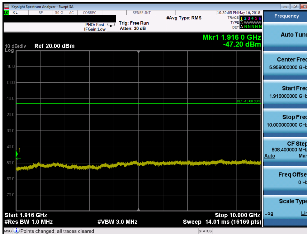
Plot 7-188. Conducted Spurious Plot (Band 25/2 - 20.0MHz QPSK - RB Size 1, RB Offset 0 - High Channel)
