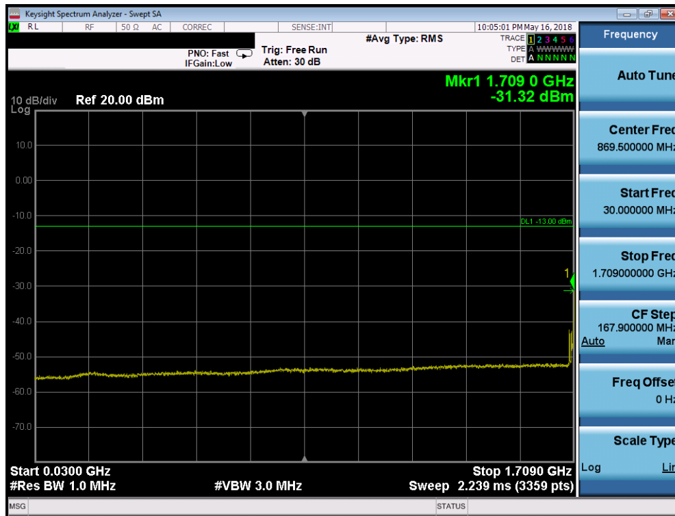
Plot 7-172. Conducted Spurious Plot (Band 66/4 - 20.0MHz QPSK - RB Size 1, RB Offset 0 - Low Channel)
