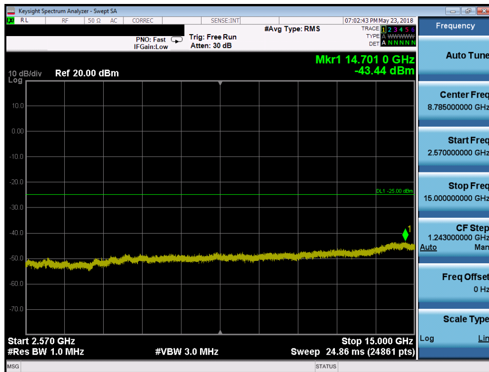
Plot 7-212. Conducted Spurious Plot (Band 7 - 15.0MHz QPSK - RB Size 1, RB Offset 0 - Low Channel)
