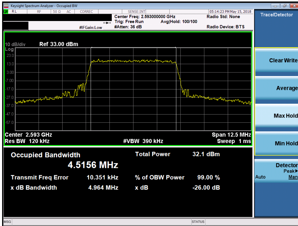
Plot 7-132. Occupied Bandwidth Plot (Band 41 - 5.0MHz 64-QAM - Full RB Configuration)
