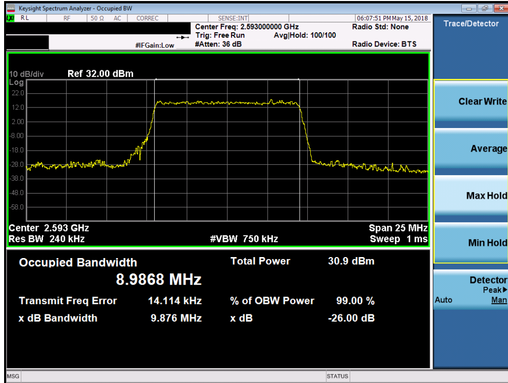
Plot 7-122. Occupied Bandwidth Plot (Band 41/38 - 10.0MHz 16-QAM - Full RB Configuration)
