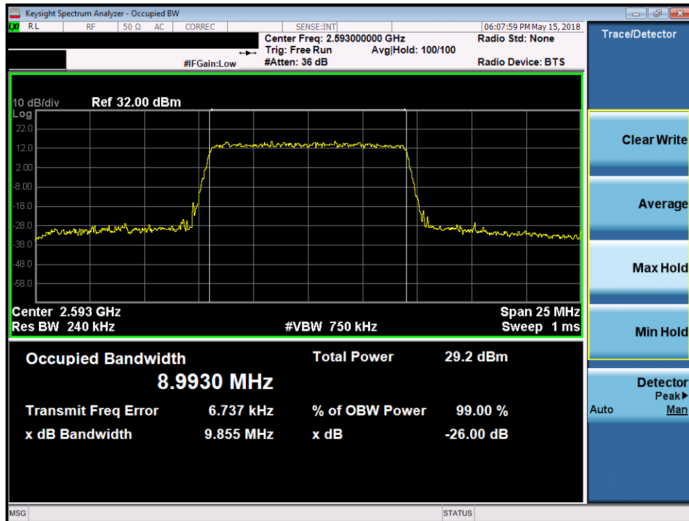
Plot 7-123. Occupied Bandwidth Plot (Band 41/38 - 10.0MHz 64-QAM - Full RB Configuration)
