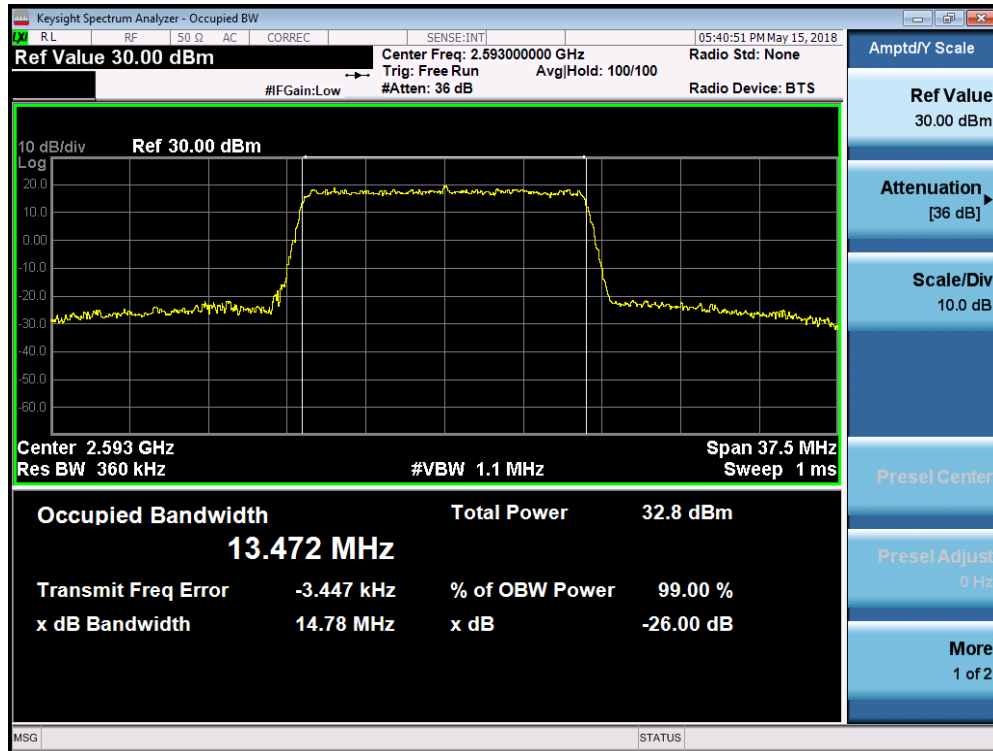
Plot 7-138. Occupied Bandwidth Plot (Band 41 - 15.0MHz 64-QAM - Full RB Configuration)
