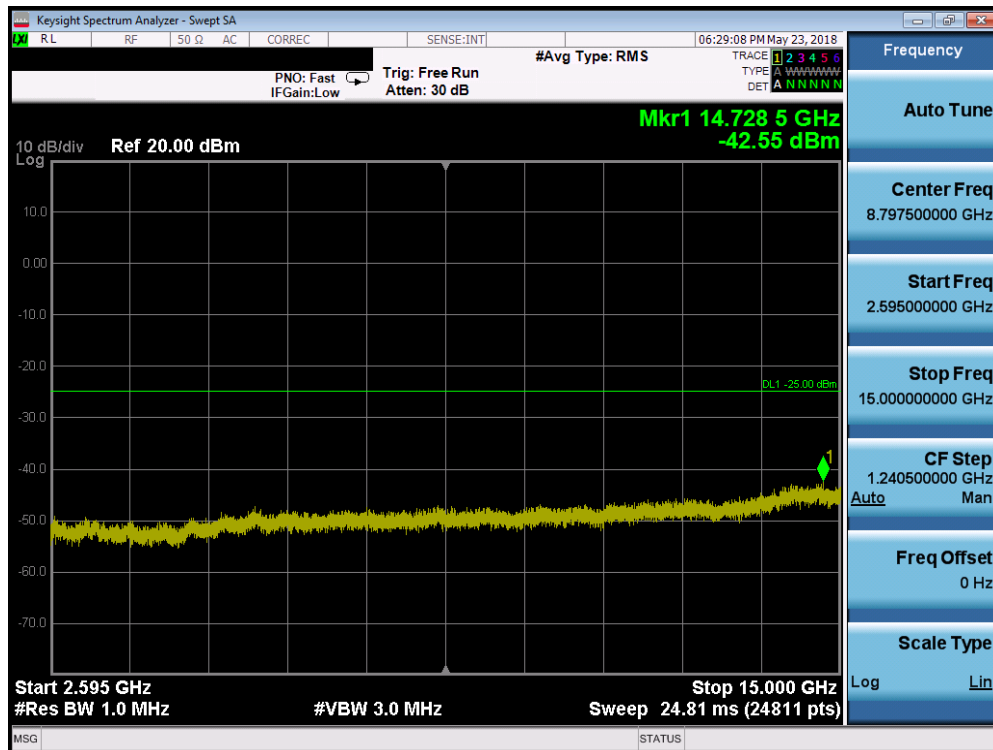
Plot 7-209. Conducted Spurious Plot (Band 7 - 15.0MHz QPSK - RB Size 1, RB Offset 0 - High Channel)
