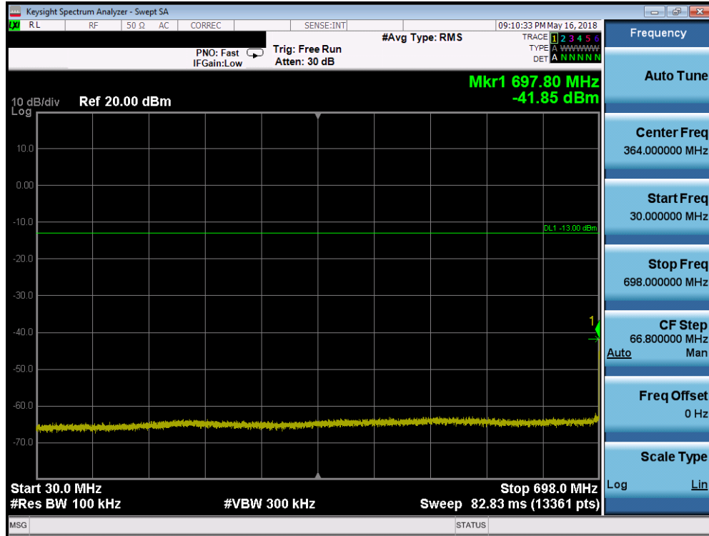
Plot 7-157. Conducted Spurious Plot (Band 12/17 - 10.0MHz QPSK - RB Size 1, RB Offset 0 - High Channel)
