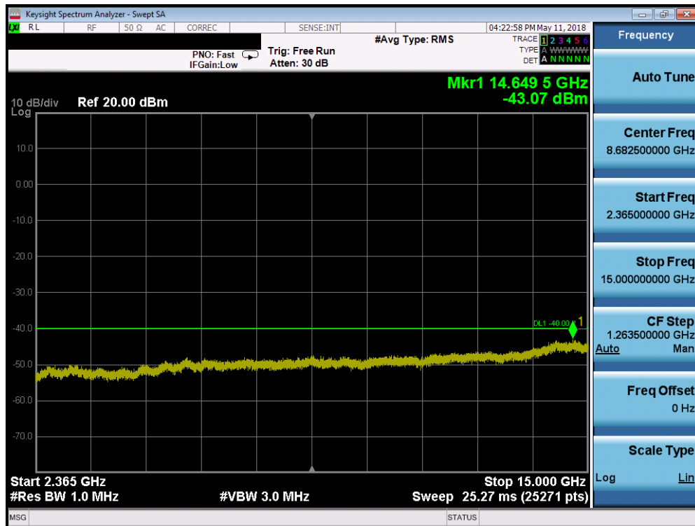
Plot 7-194. Conducted Spurious Plot (Band 30 - 5.0MHz QPSK - RB Size 1, RB Offset 0 - Low Channel)
