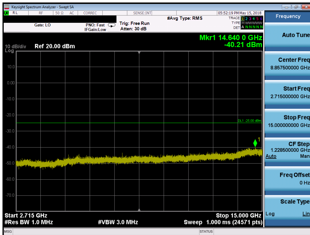
Plot 7-236. Conducted Spurious Plot (Band 41 - 20.0MHz QPSK - RB Size 1, RB Offset 0 - High Channel)
