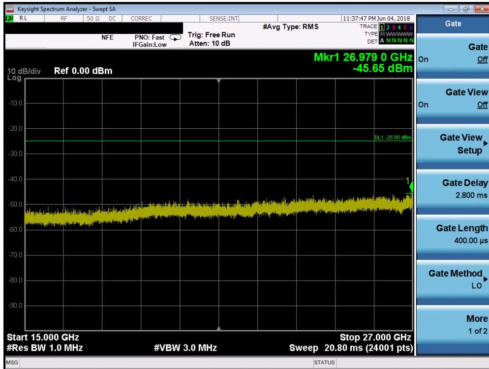
Plot 7-228. Conducted Spurious Plot (Band 41/38 - 20.0MHz QPSK - RB Size 1, RB Offset 0 - High Channel)
