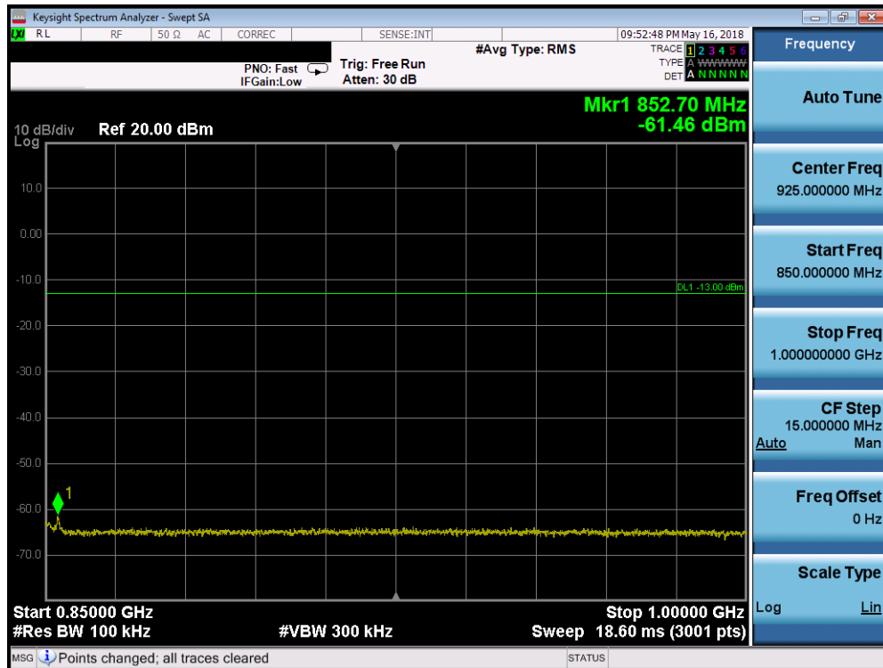
Plot 7-170. Conducted Spurious Plot (Band 26/5 - 10.0MHz QPSK - RB Size 1, RB Offset 0 - High Channel)
