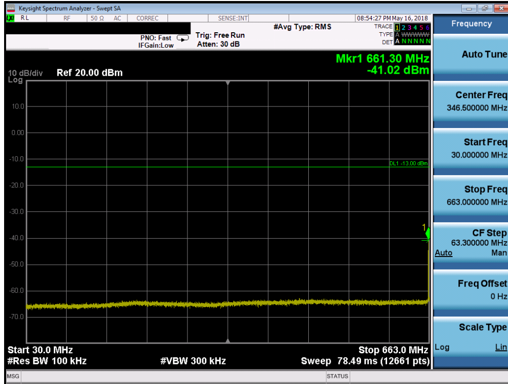
Plot 7-148. Conducted Spurious Plot (Band 71 - 20.0MHz QPSK - RB Size 1, RB Offset 0 - High Channel)
