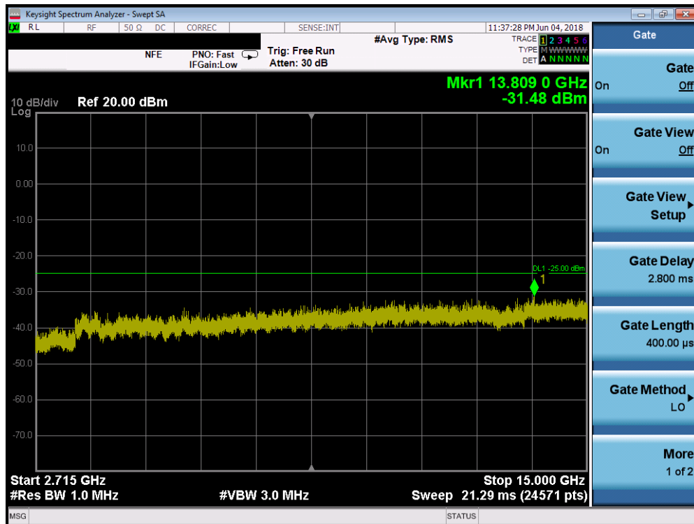
Plot 7-227. Conducted Spurious Plot (Band 41/38 - 20.0MHz QPSK - RB Size 1, RB Offset 0 - High Channel)
