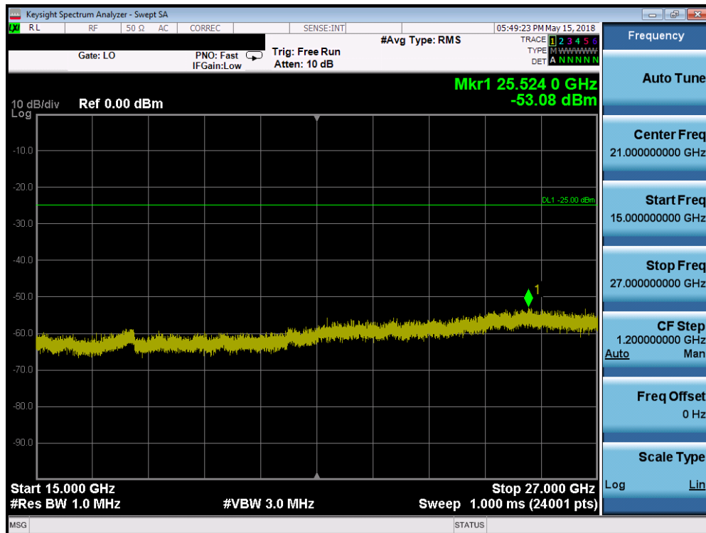
Plot 7-234. Conducted Spurious Plot (Band 41 - 20.0MHz QPSK - RB Size 1, RB Offset 0 - Mid Channel)
