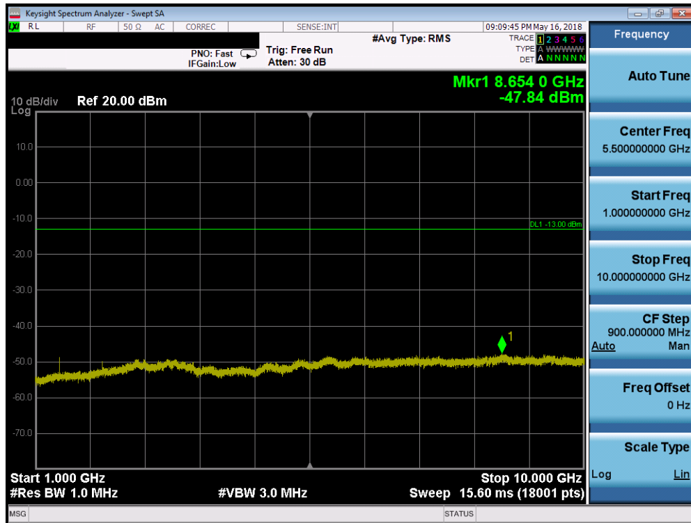
Plot 7-153. Conducted Spurious Plot (Band 12/17 - 10.0MHz QPSK - RB Size 1, RB Offset 0 - Low Channel)
