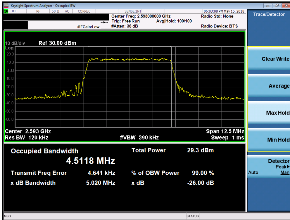
Plot 7-120. Occupied Bandwidth Plot (Band 41/38- 5.0MHz 64-QAM - Full RB Configuration)
