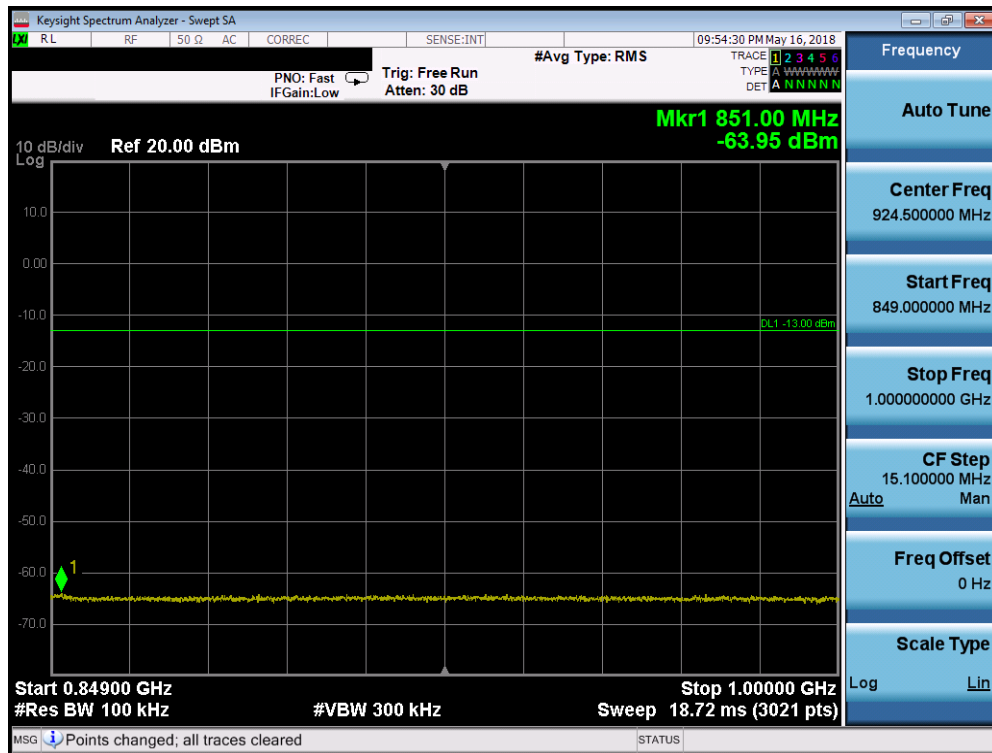
Plot 7-164. Conducted Spurious Plot (Band 26/5 - 10.0MHz QPSK - RB Size 1, RB Offset 0 - Low Channel)
