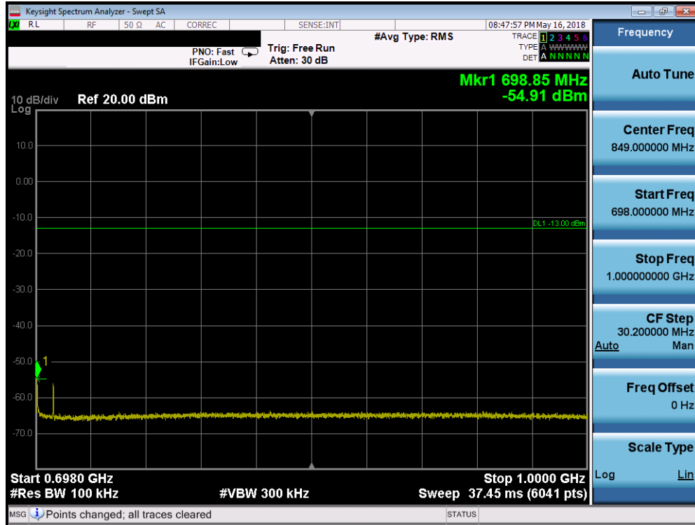
Plot 7-146. Conducted Spurious Plot (Band 71 - 20.0MHz QPSK - RB Size 1, RB Offset 0 - Mid Channel)
