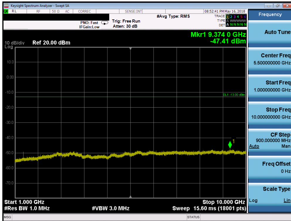
Plot 7-144. Conducted Spurious Plot (Band 71 - 20.0MHz QPSK - RB Size 1, RB Offset 0 - Low Channel)
