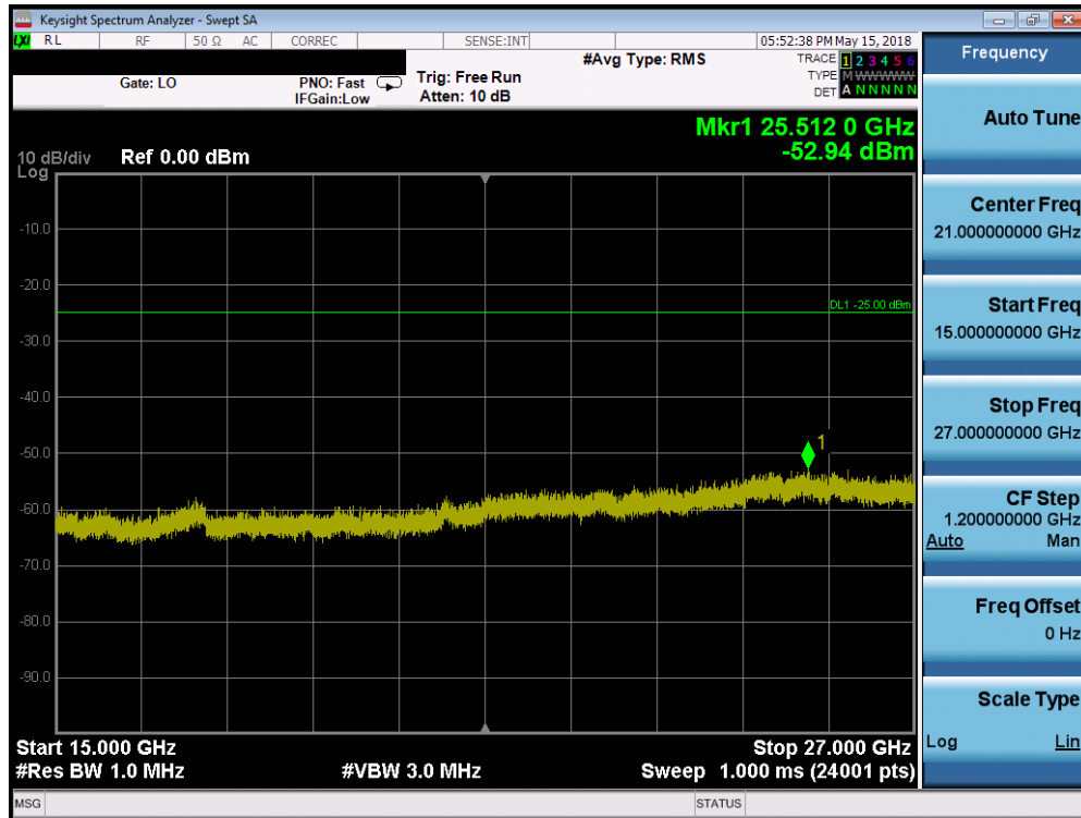
Plot 7-237. Conducted Spurious Plot (Band 41 - 20.0MHz QPSK - RB Size 1, RB Offset 0 - High Channel)
