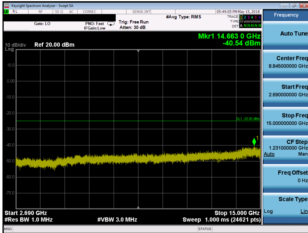
Plot 7-233. Conducted Spurious Plot (Band 41 - 20.0MHz QPSK - RB Size 1, RB Offset 0 - Mid Channel)
