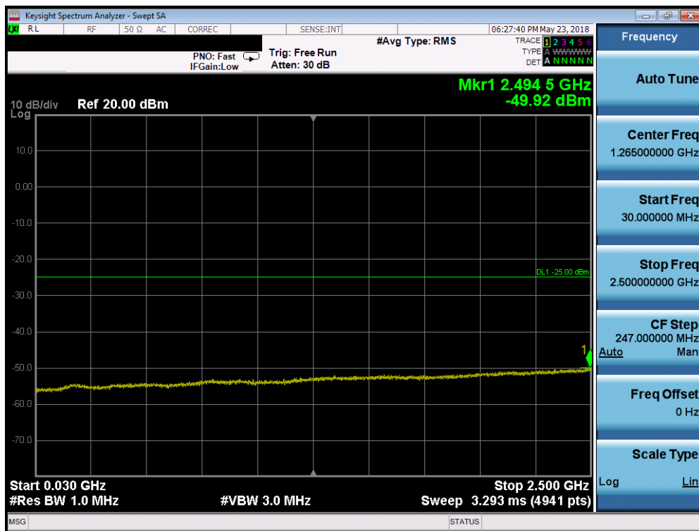
Plot 7-205. Conducted Spurious Plot (Band 7 - 15.0MHz QPSK - RB Size 1, RB Offset 0 - Mid Channel)
