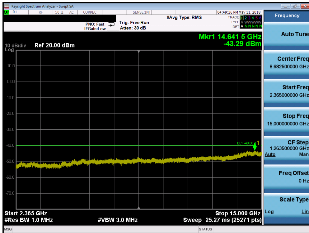
Plot 7-191. Conducted Spurious Plot (Band 30 - 10.0MHz QPSK - RB Size 1, RB Offset 0 - Mid Channel)
