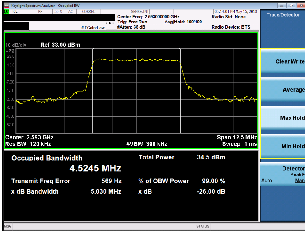
Plot 7-130. Occupied Bandwidth Plot (Band 41 - 5.0MHz QPSK - Full RB Configuration)
