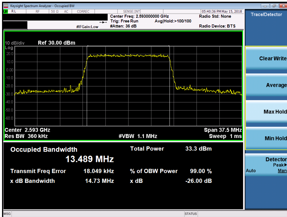
Plot 7-137. Occupied Bandwidth Plot (Band 41 - 15.0MHz 16-QAM - Full RB Configuration)
