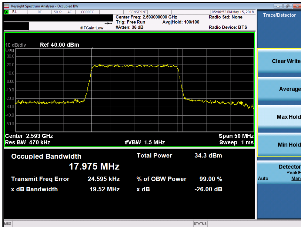
Plot 7-139. Occupied Bandwidth Plot (Band 41 - 20.0MHz QPSK - Full RB Configuration)
