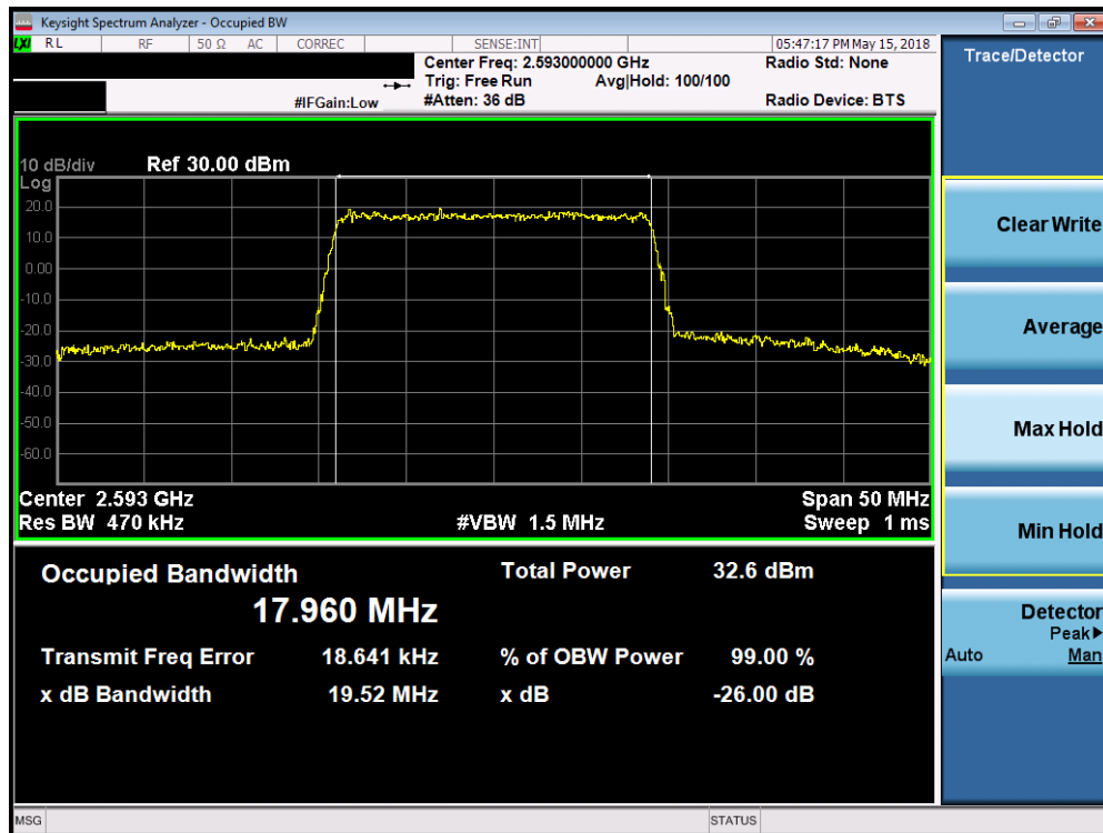
Plot 7-141. Occupied Bandwidth Plot (Band 41 - 20.0MHz 64-QAM - Full RB Configuration)
