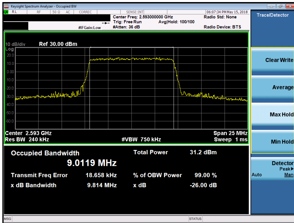
Plot 7-121. Occupied Bandwidth Plot (Band 41/38 - 10.0MHz QPSK - Full RB Configuration)
