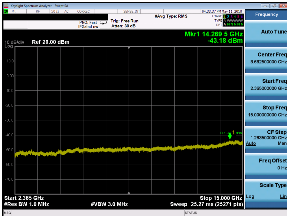
Plot 7-200. Conducted Spurious Plot (Band 30 - 5.0MHz QPSK - RB Size 1, RB Offset 0 - High Channel)
