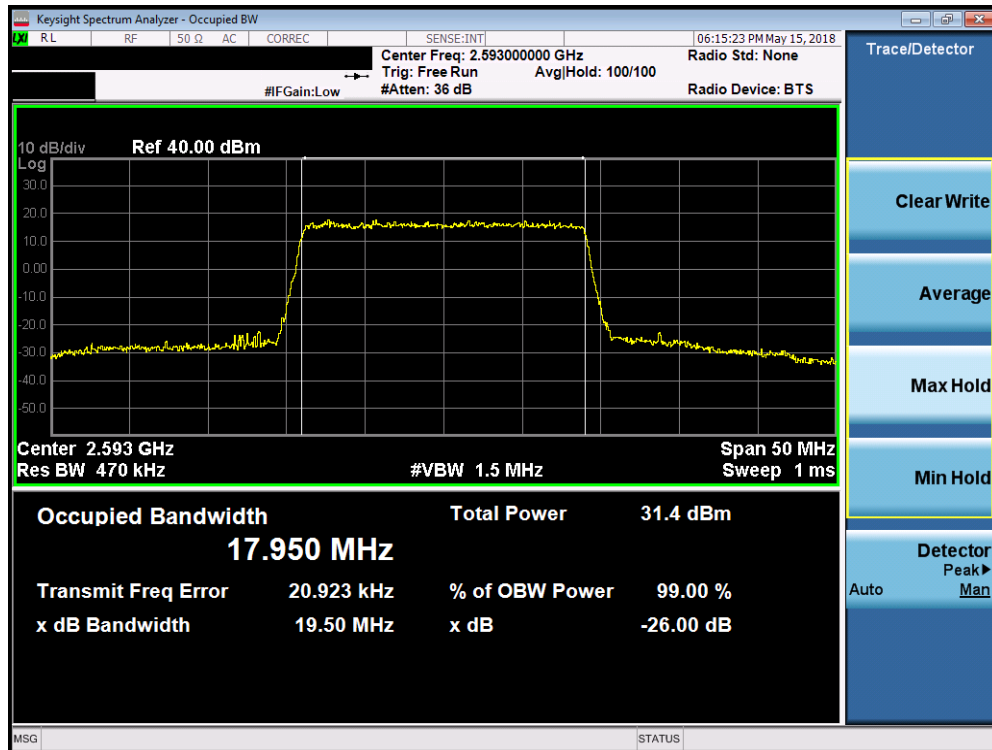
Plot 7-127. Occupied Bandwidth Plot (Band 41/38 - 20.0MHz QPSK - Full RB Configuration)
