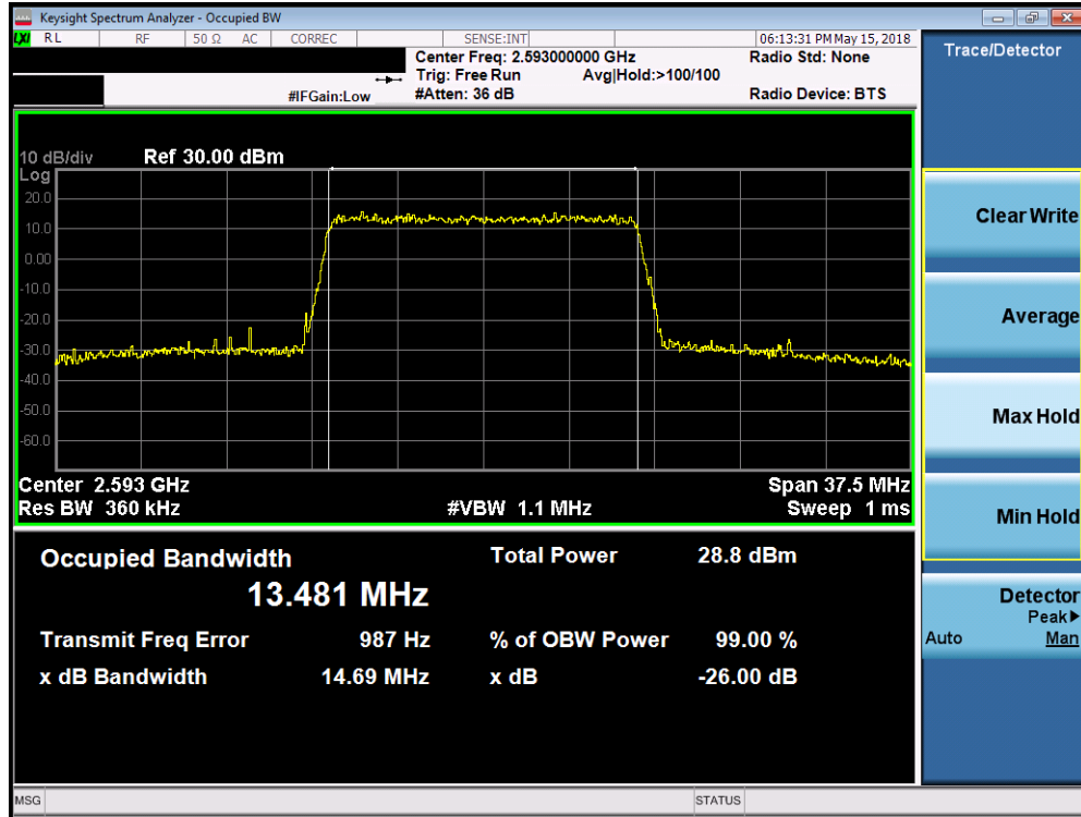
Plot 7-126. Occupied Bandwidth Plot (Band 41/38 - 15.0MHz 64-QAM - Full RB Configuration)
