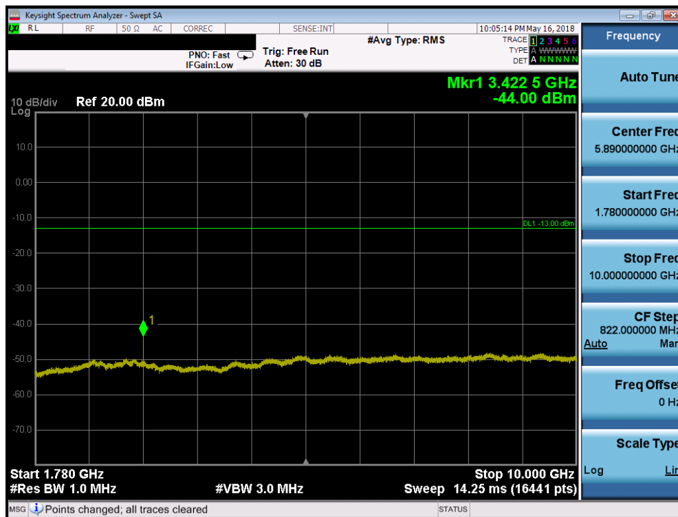
Plot 7-173. Conducted Spurious Plot (Band 66/4 - 20.0MHz QPSK - RB Size 1, RB Offset 0 - Low Channel)
