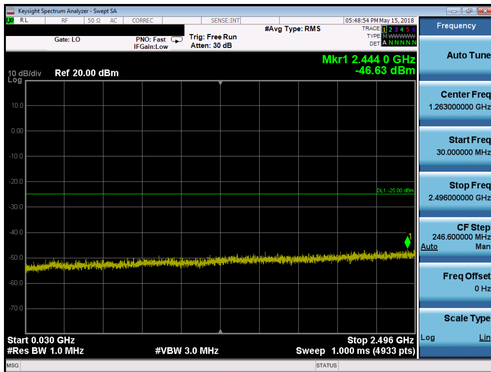
Plot 7-232. Conducted Spurious Plot (Band 41 - 20.0MHz QPSK - RB Size 1, RB Offset 0 - Mid Channel)
