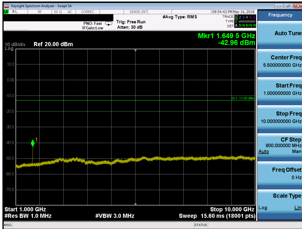
Plot 7-165. Conducted Spurious Plot (Band 26/5 - 10.0MHz QPSK - RB Size 1, RB Offset 0 - Low Channel)
