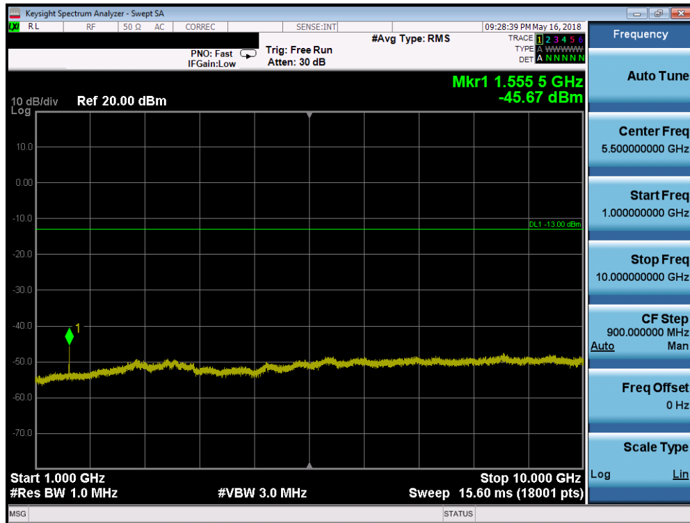
Plot 7-162. Conducted Spurious Plot (Band 13 - 10.0MHz QPSK - RB Size 1, RB Offset 0)
