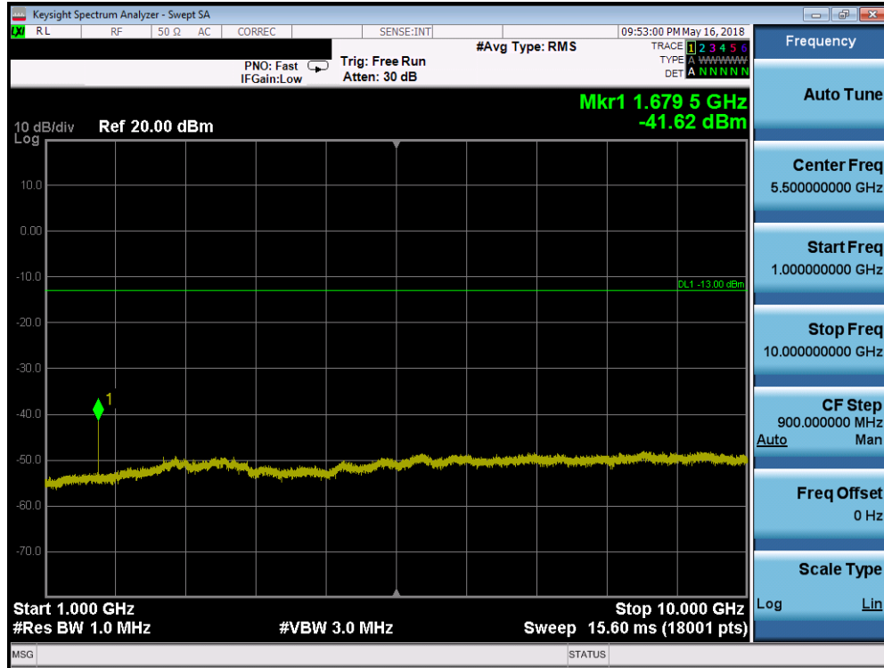
Plot 7-171. Conducted Spurious Plot (Band 26/5 - 10.0MHz QPSK - RB Size 1, RB Offset 0 - High Channel)
