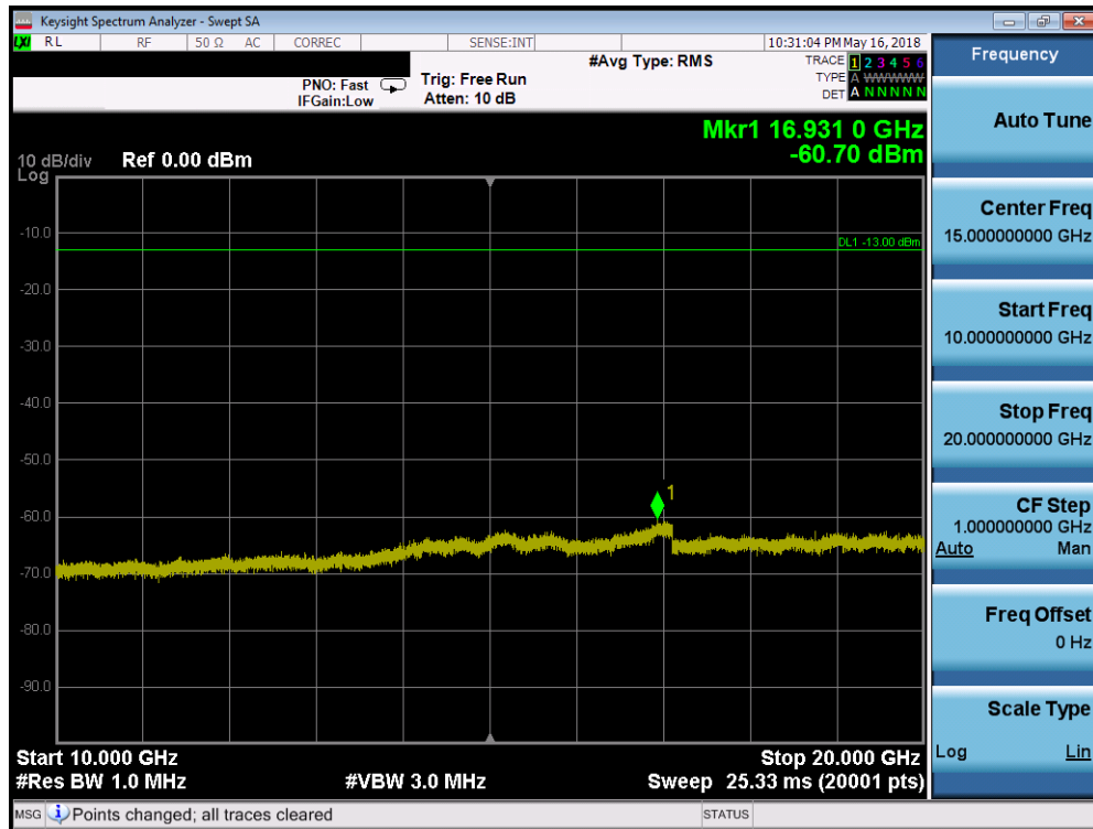
Plot 7-183. Conducted Spurious Plot (Band 25/2 - 20.0MHz QPSK - RB Size 1, RB Offset 0 - Low Channel)
