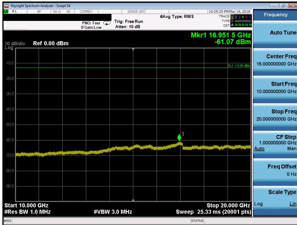
Plot 7-186. Conducted Spurious Plot (Band 25/2 - 20.0MHz QPSK - RB Size 1, RB Offset 0 - Mid Channel)
