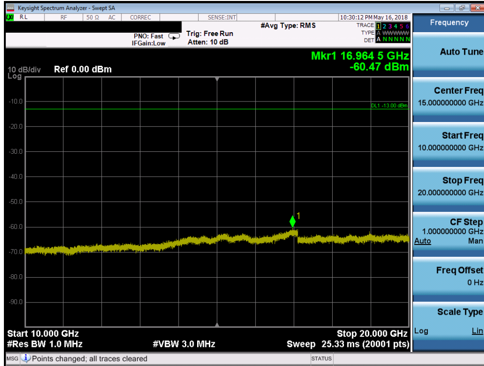
Plot 7-189. Conducted Spurious Plot (Band 25/2 - 20.0MHz QPSK - RB Size 1, RB Offset 0 - High Channel)
