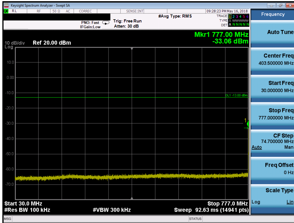
Plot 7-160. Conducted Spurious Plot (Band 13 - 10.0MHz QPSK - RB Size 1, RB Offset 0)
