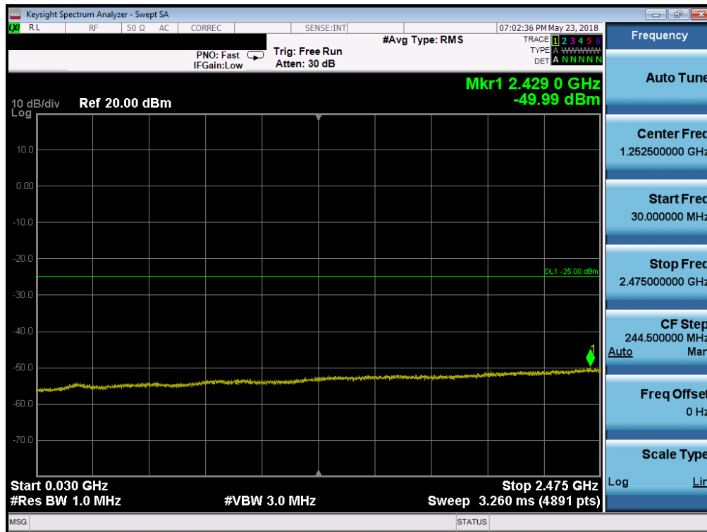
Plot 7-211. Conducted Spurious Plot (Band 7 - 15.0MHz QPSK - RB Size 1, RB Offset 0 - Low Channel)
