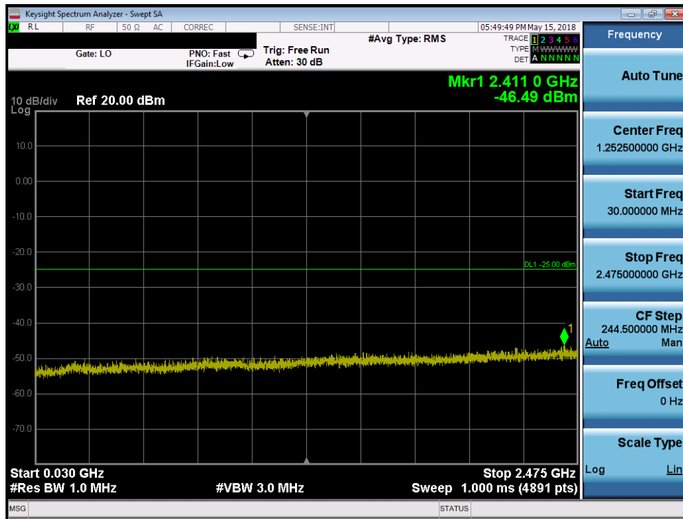
Plot 7-229. Conducted Spurious Plot (Band 41 - 20.0MHz QPSK - RB Size 1, RB Offset 0 - Low Channel)
