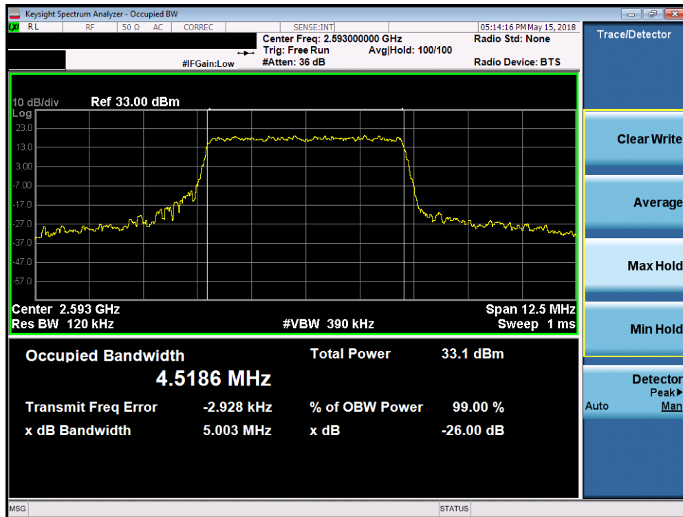
Plot 7-131. Occupied Bandwidth Plot (Band 41 - 5.0MHz 16-QAM - Full RB Configuration)
