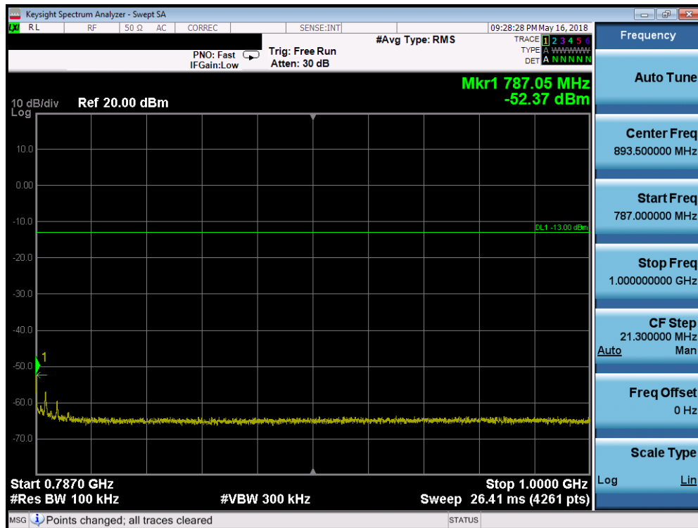
Plot 7-161. Conducted Spurious Plot (Band 13 - 10.0MHz QPSK - RB Size 1, RB Offset 0)
