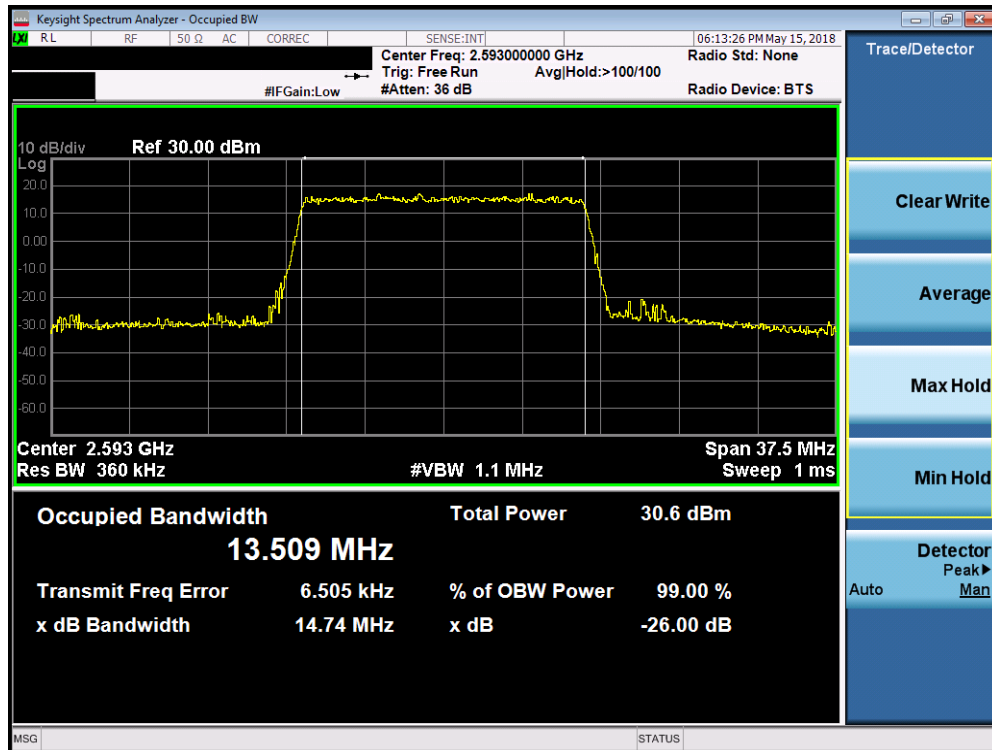
Plot 7-125. Occupied Bandwidth Plot (Band 41/38 - 15.0MHz 16-QAM - Full RB Configuration)
