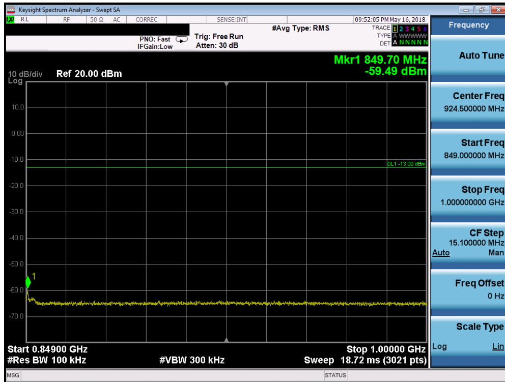
Plot 7-167. Conducted Spurious Plot (Band 26/5 - 10.0MHz QPSK - RB Size 1, RB Offset 0 - Mid Channel)
