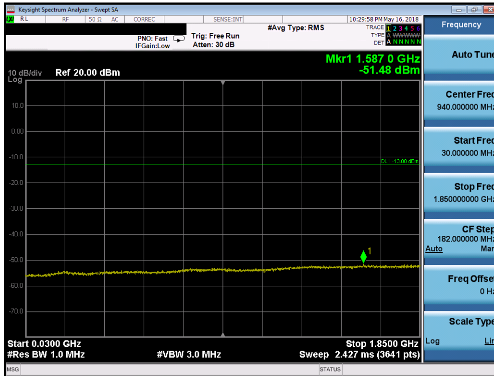
Plot 7-187. Conducted Spurious Plot (Band 25/2 - 20.0MHz QPSK - RB Size 1, RB Offset 0 - High Channel)
