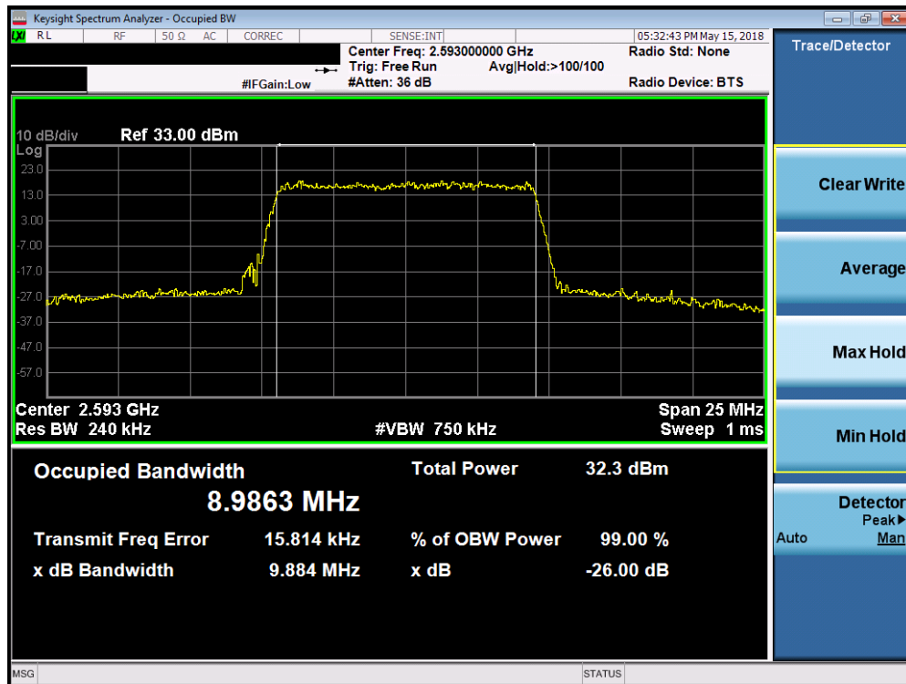
Plot 7-135. Occupied Bandwidth Plot (Band 41 - 10.0MHz 64-QAM - Full RB Configuration)
