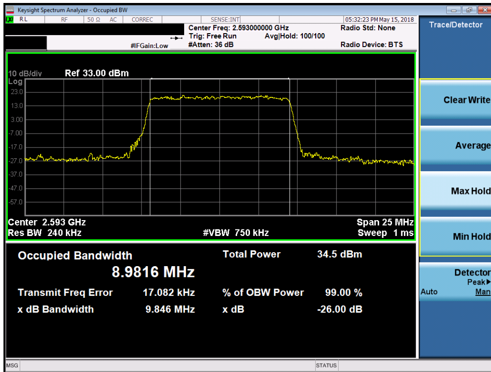
Plot 7-133. Occupied Bandwidth Plot (Band 41 - 10.0MHz QPSK - Full RB Configuration)
