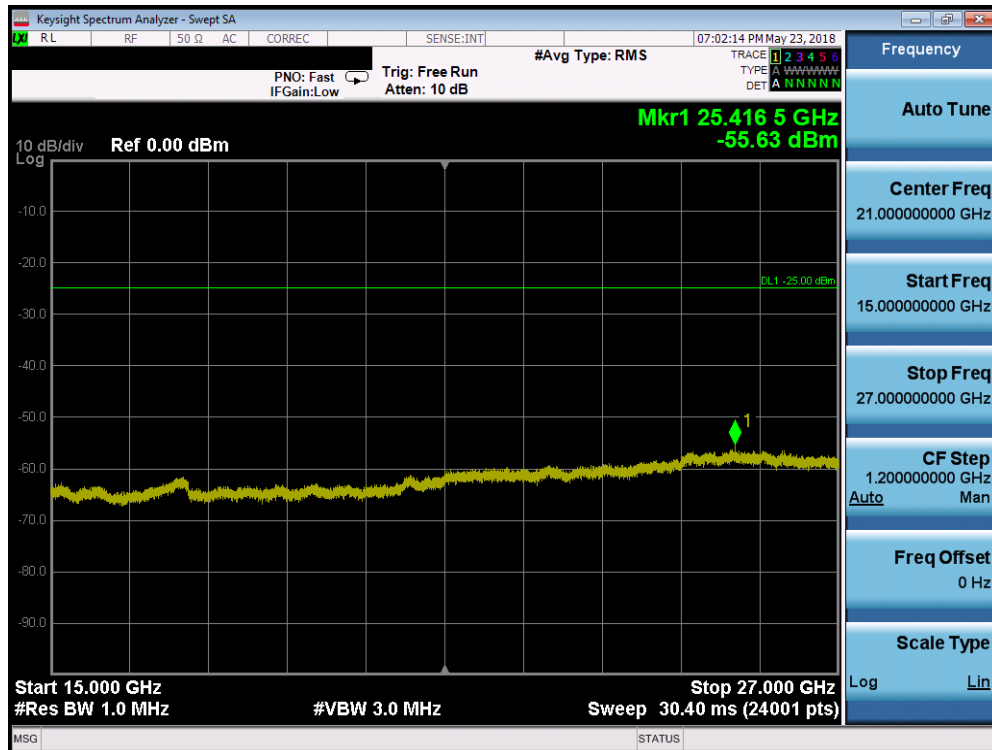
Plot 7-216. Conducted Spurious Plot (Band 7 - 15.0MHz QPSK - RB Size 1, RB Offset 0 - Mid Channel)
