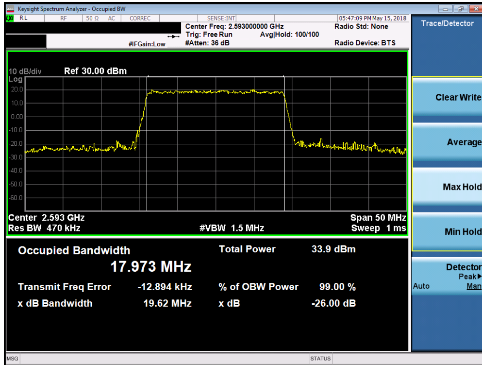
Plot 7-140. Occupied Bandwidth Plot (Band 41 - 20.0MHz 16-QAM - Full RB Configuration)
