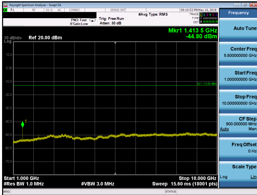
Plot 7-159. Conducted Spurious Plot (Band 12/17 - 10.0MHz QPSK - RB Size 1, RB Offset 0 - High Channel)
