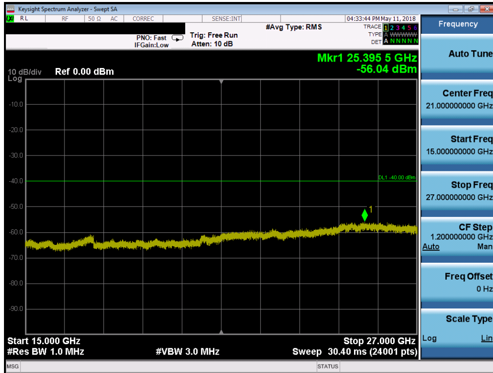
Plot 7-201. Conducted Spurious Plot (Band 30 - 5.0MHz QPSK - RB Size 1, RB Offset 0 - High Channel)
