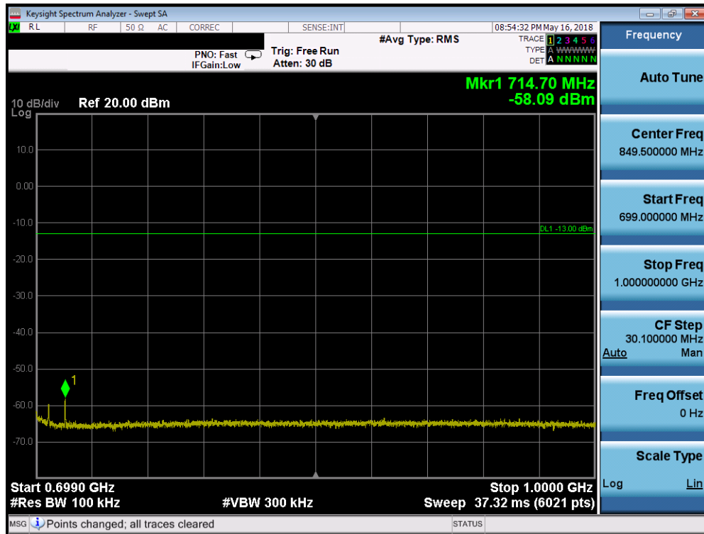
Plot 7-149. Conducted Spurious Plot (Band 71 - 20.0MHz QPSK - RB Size 1, RB Offset 0 - High Channel)
