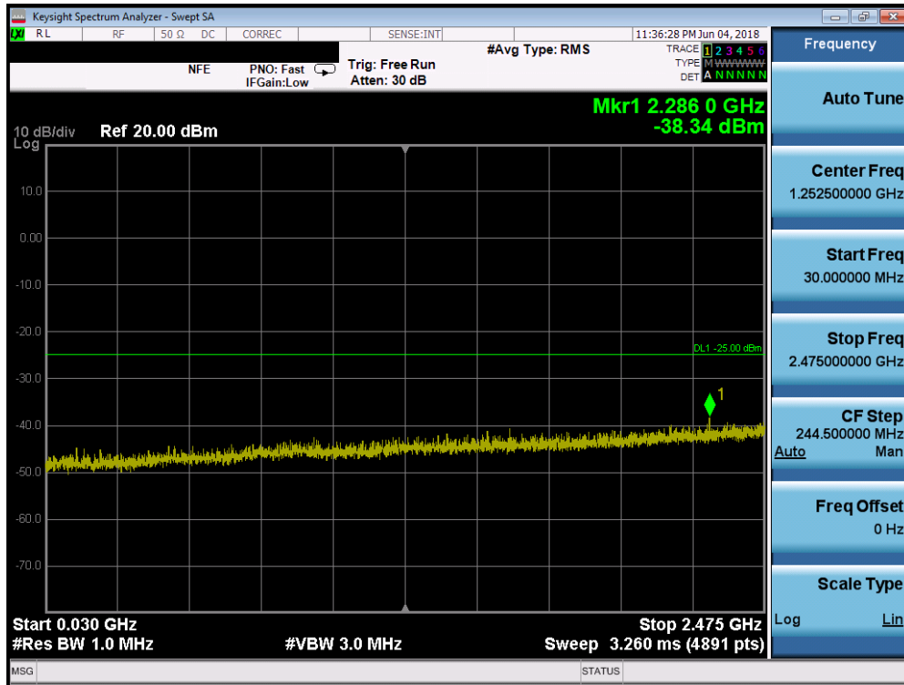
Plot 7-220. Conducted Spurious Plot (Band 41/38 - 20.0MHz QPSK - RB Size 1, RB Offset 0 - Low Channel)
