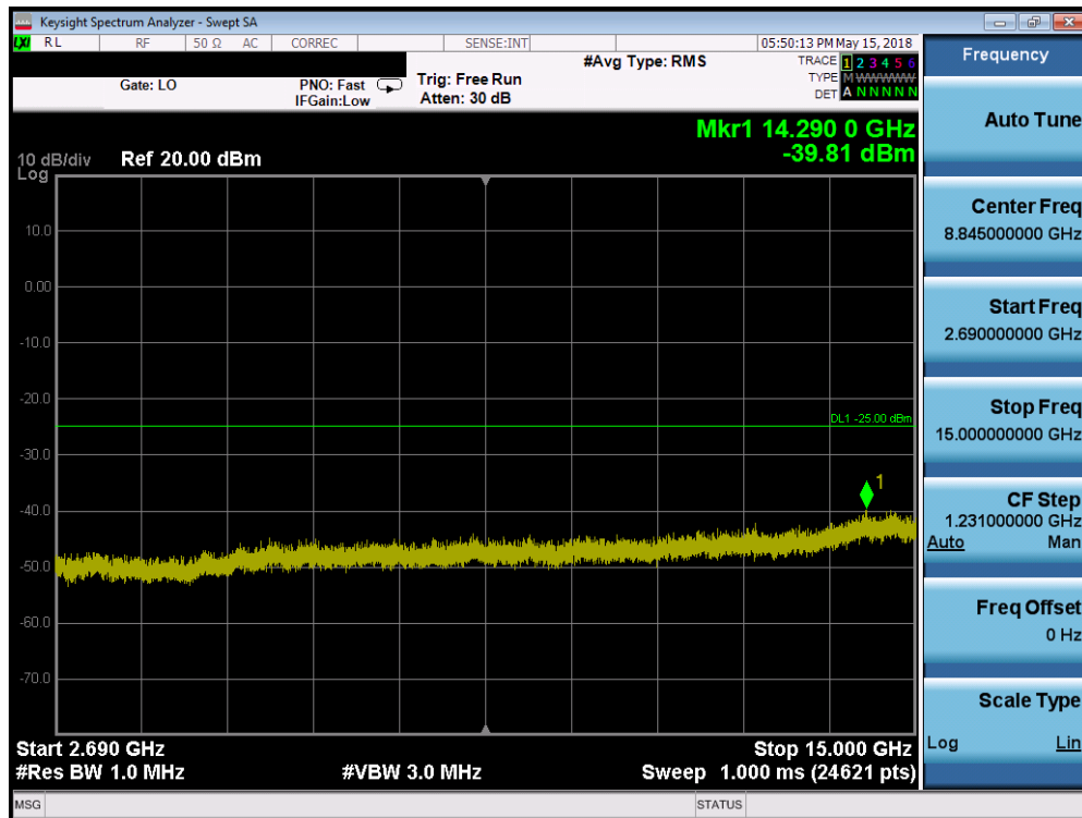
Plot 7-230. Conducted Spurious Plot (Band 41 - 20.0MHz QPSK - RB Size 1, RB Offset 0 - Low Channel)
