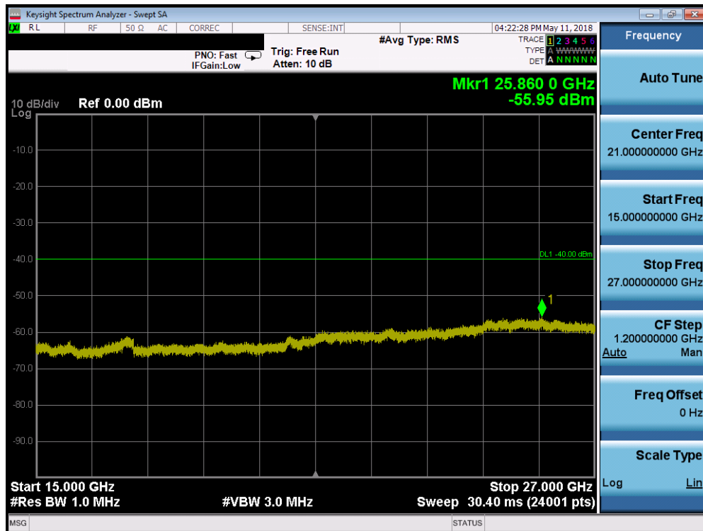
Plot 7-198. Conducted Spurious Plot (Band 30 - 5.0MHz QPSK - RB Size 1, RB Offset 0 - Mid Channel)
