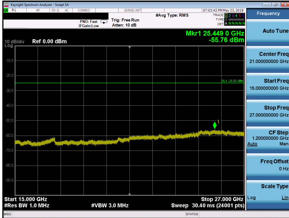
Plot 7-219. Conducted Spurious Plot (Band 7 - 15.0MHz QPSK - RB Size 1, RB Offset 0 - High Channel)
