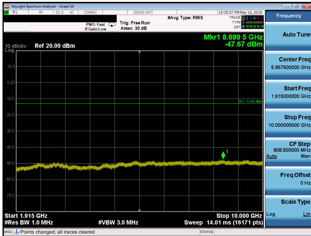
Plot 7-182. Conducted Spurious Plot (Band 25/2 - 20.0MHz QPSK - RB Size 1, RB Offset 0 - Low Channel)
