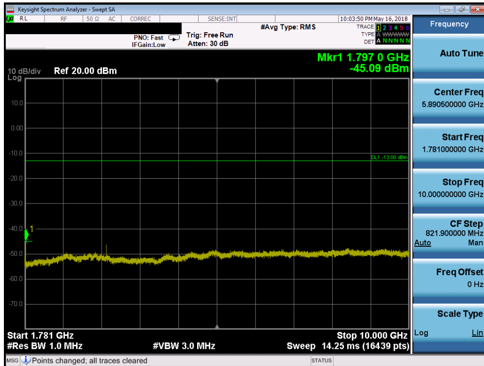
Plot 7-179. Conducted Spurious Plot (Band 66/4 - 20.0MHz QPSK - RB Size 1, RB Offset 0 - High Channel)
