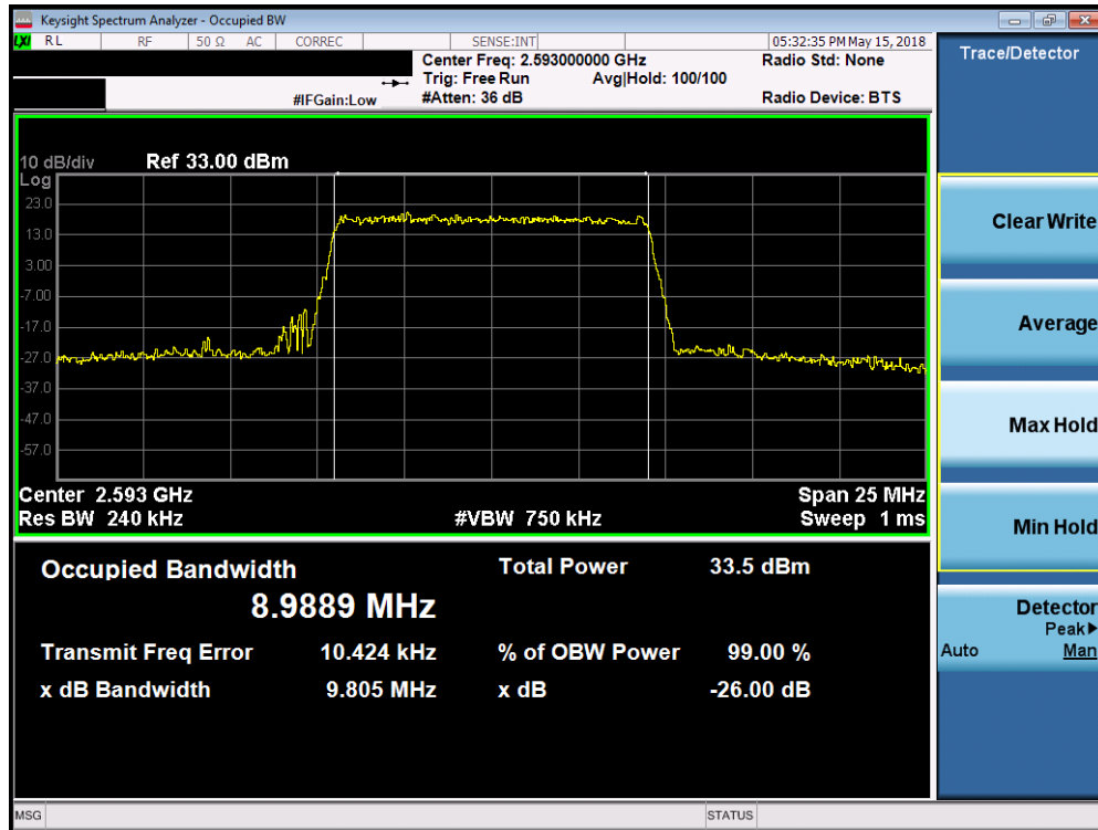
Plot 7-134. Occupied Bandwidth Plot (Band 41 - 10.0MHz 16-QAM - Full RB Configuration)
