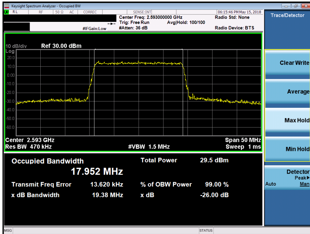
Plot 7-129. Occupied Bandwidth Plot (Band 41/38 - 20.0MHz 64-QAM - Full RB Configuration)
