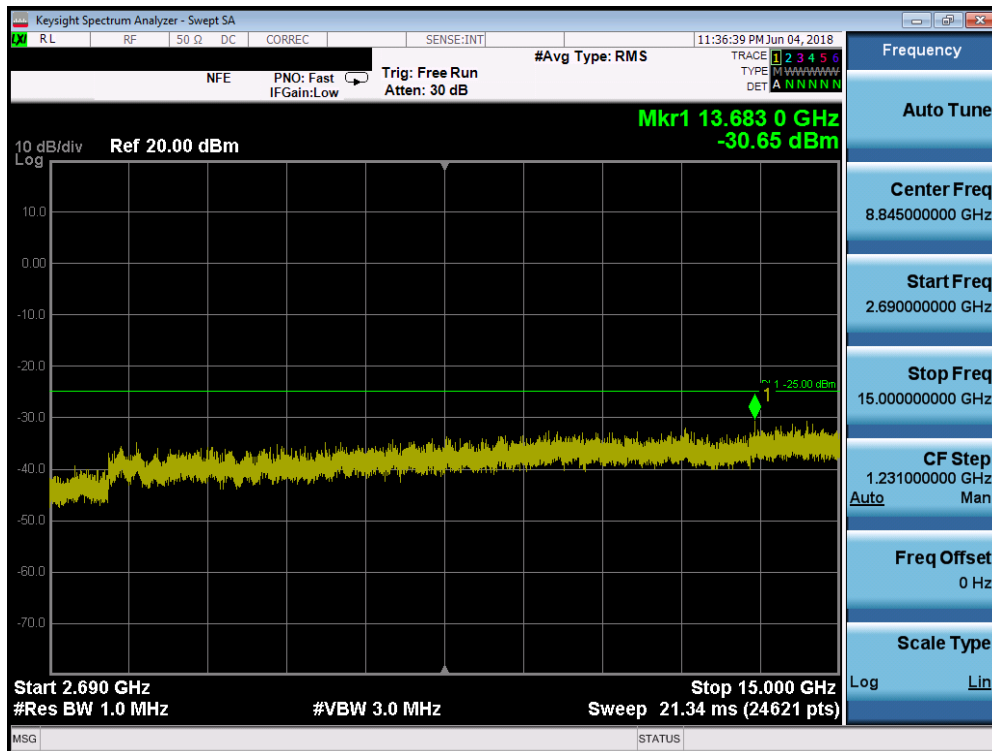
Plot 7-221. Conducted Spurious Plot (Band 41/38 - 20.0MHz QPSK - RB Size 1, RB Offset 0 - Low Channel)
