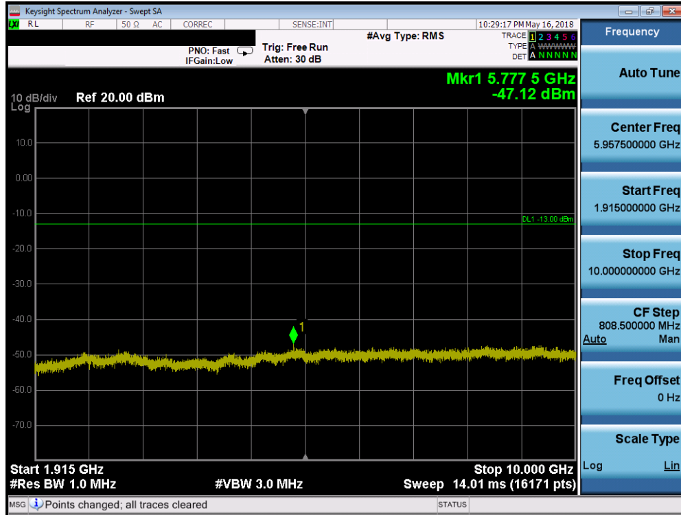
Plot 7-185. Conducted Spurious Plot (Band 25/2 - 20.0MHz QPSK - RB Size 1, RB Offset 0 - Mid Channel)
