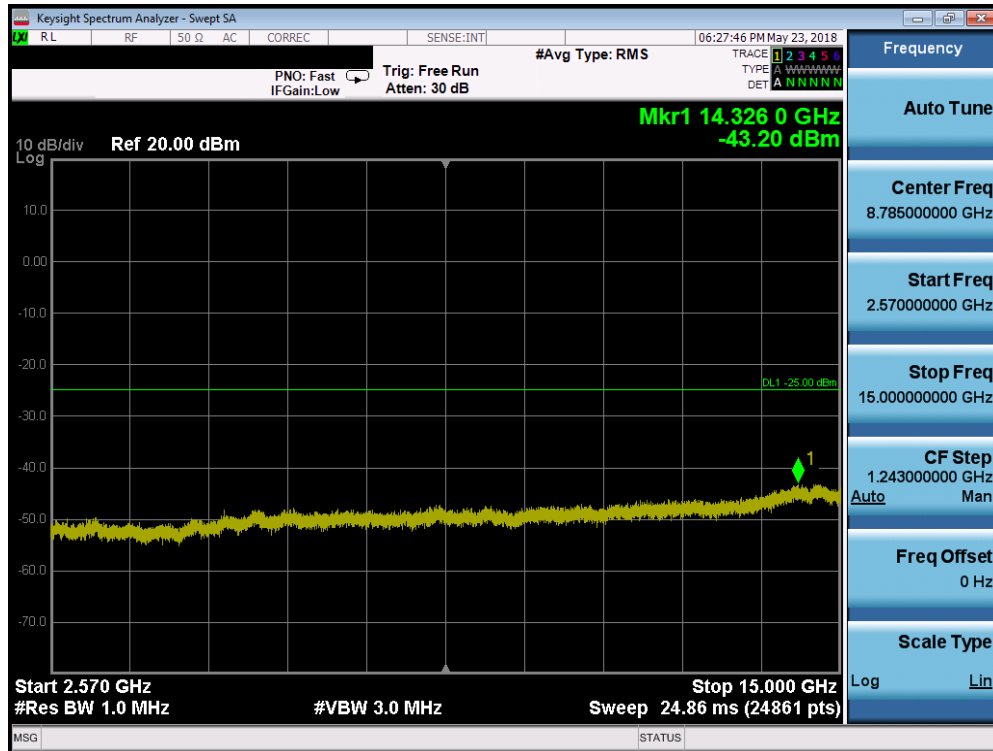
Plot 7-206. Conducted Spurious Plot (Band 7 - 15.0MHz QPSK - RB Size 1, RB Offset 0 - Mid Channel)
