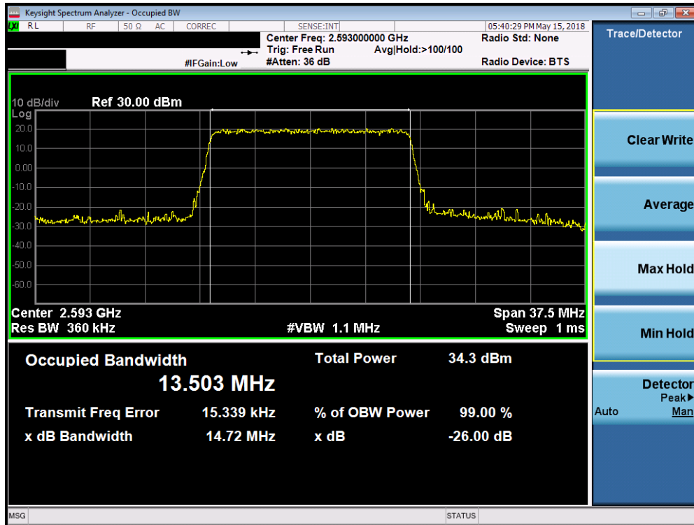
Plot 7-136. Occupied Bandwidth Plot (Band 41 - 15.0MHz QPSK - Full RB Configuration)
