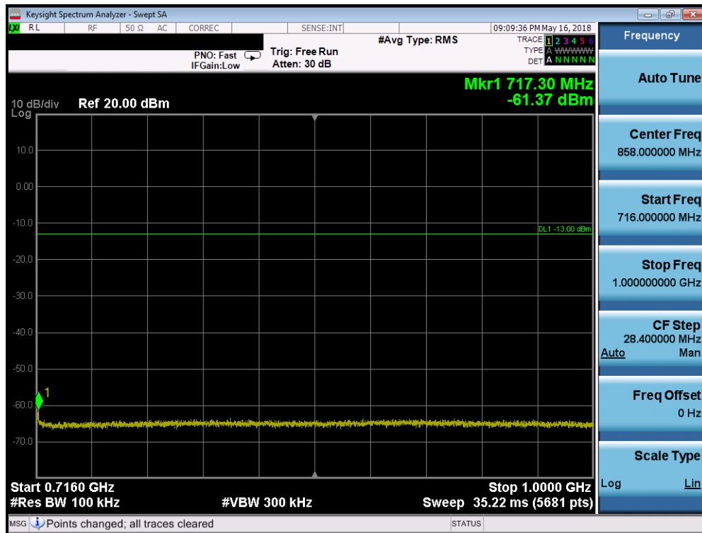
Plot 7-152. Conducted Spurious Plot (Band 12/17 - 10.0MHz QPSK - RB Size 1, RB Offset 0 - Low Channel)
