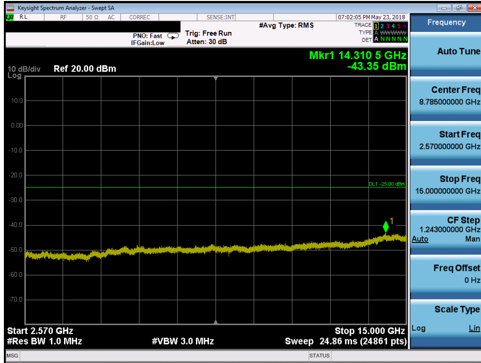
Plot 7-215. Conducted Spurious Plot (Band 7 - 15.0MHz QPSK - RB Size 1, RB Offset 0 - Mid Channel)
