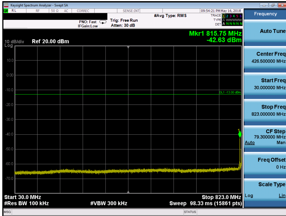
Plot 7-163. Conducted Spurious Plot (Band 26/5 - 10.0MHz QPSK - RB Size 1, RB Offset 0 - Low Channel)
