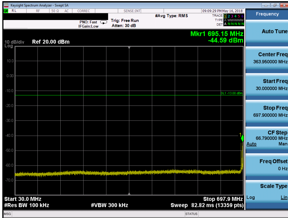
Plot 7-151. Conducted Spurious Plot (Band 12/17 - 10.0MHz QPSK - RB Size 1, RB Offset 0 - Low Channel)
