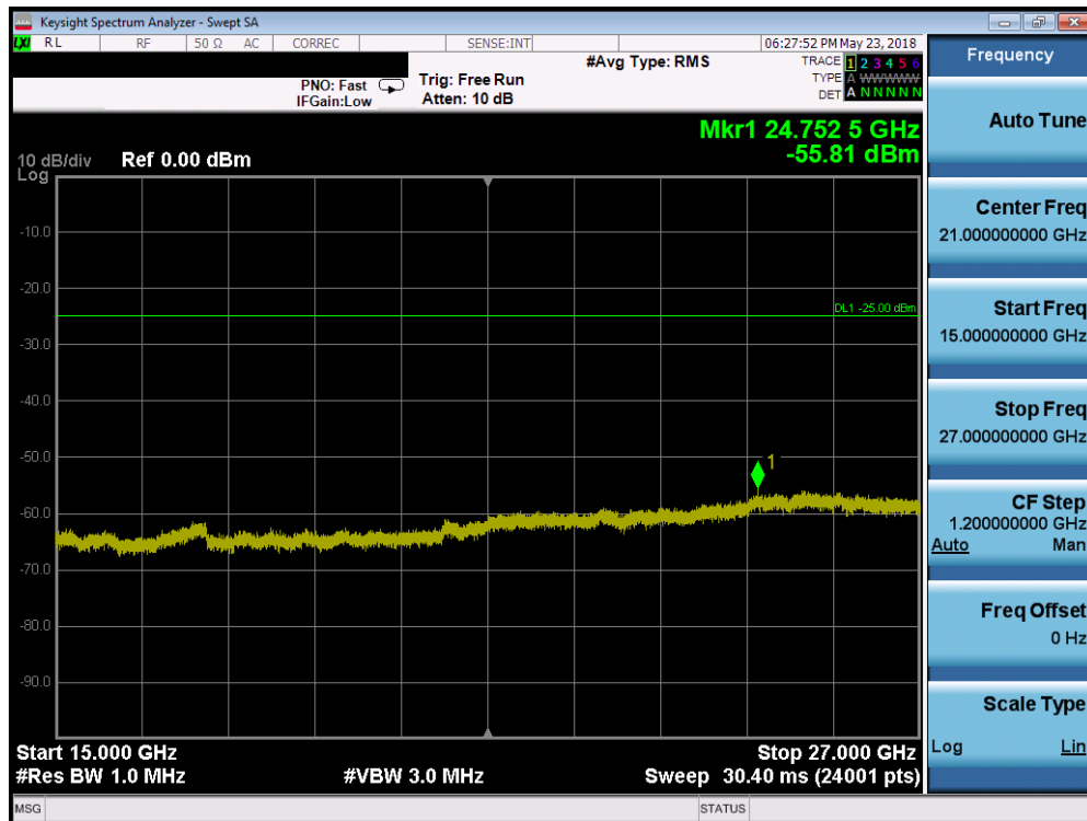
Plot 7-207. Conducted Spurious Plot (Band 7 - 15.0MHz QPSK - RB Size 1, RB Offset 0 - Mid Channel)
