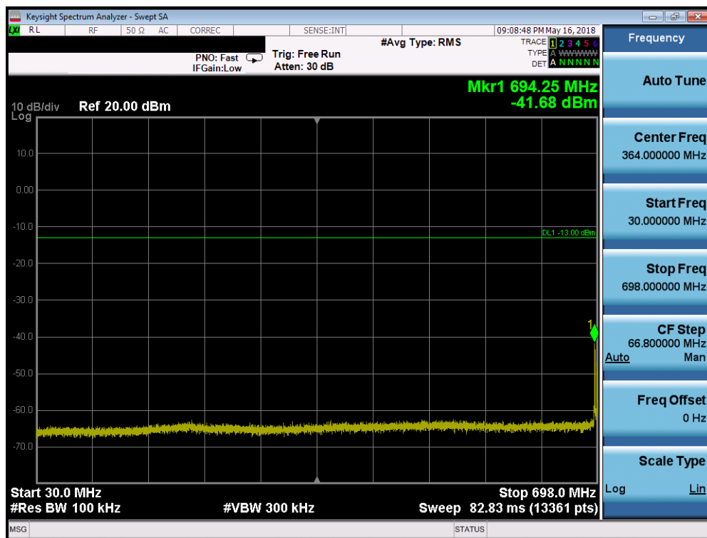
Plot 7-154. Conducted Spurious Plot (Band 12/17 - 10.0MHz QPSK - RB Size 1, RB Offset 0 - Mid Channel)
