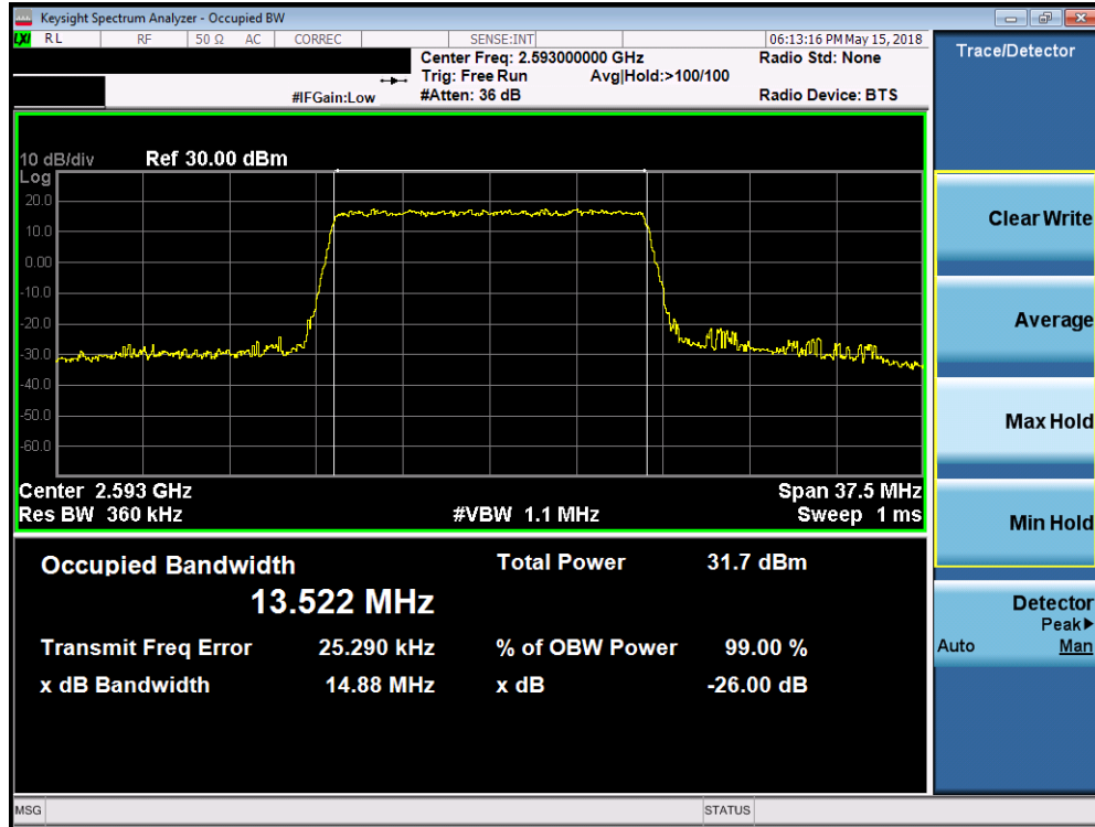
Plot 7-124. Occupied Bandwidth Plot (Band 41/38 - 15.0MHz QPSK - Full RB Configuration)
