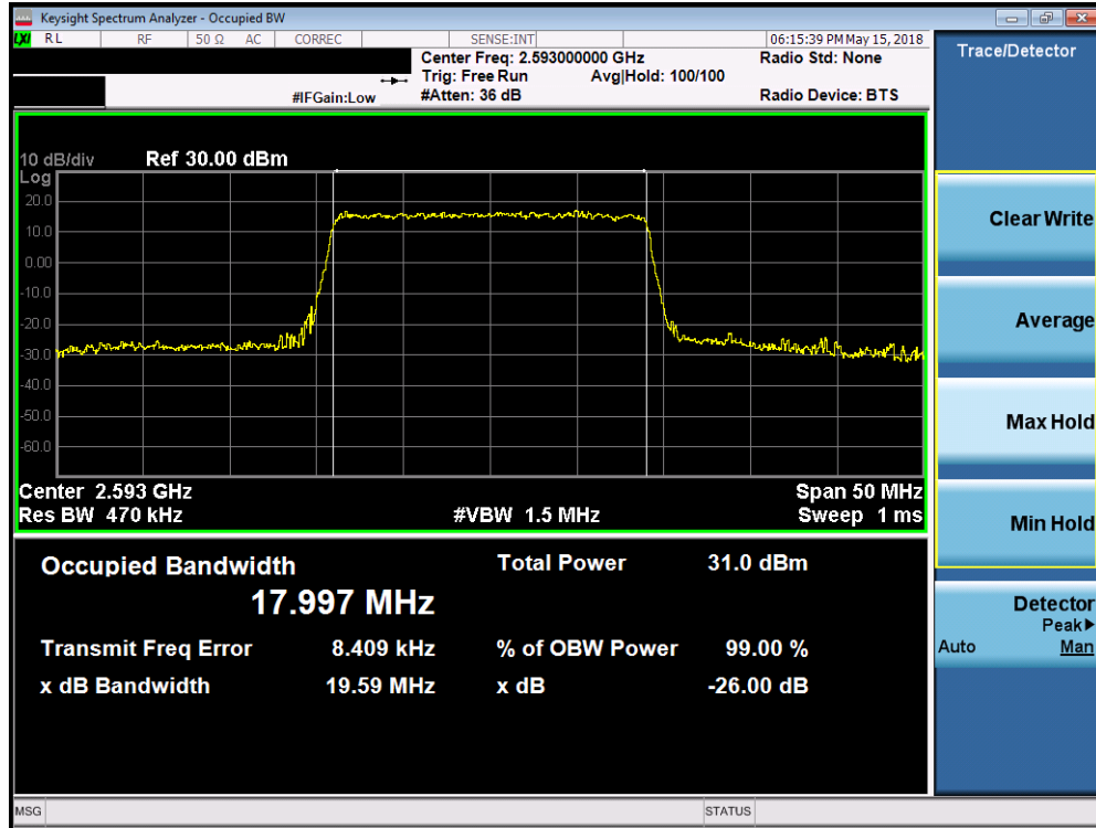
Plot 7-128. Occupied Bandwidth Plot (Band 41/38 - 20.0MHz 16-QAM - Full RB Configuration)
