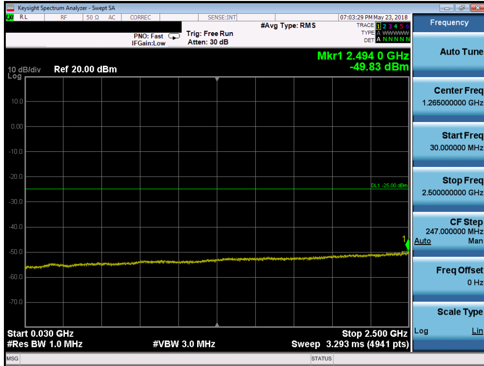
Plot 7-217. Conducted Spurious Plot (Band 7 - 15.0MHz QPSK - RB Size 1, RB Offset 0 - High Channel)
