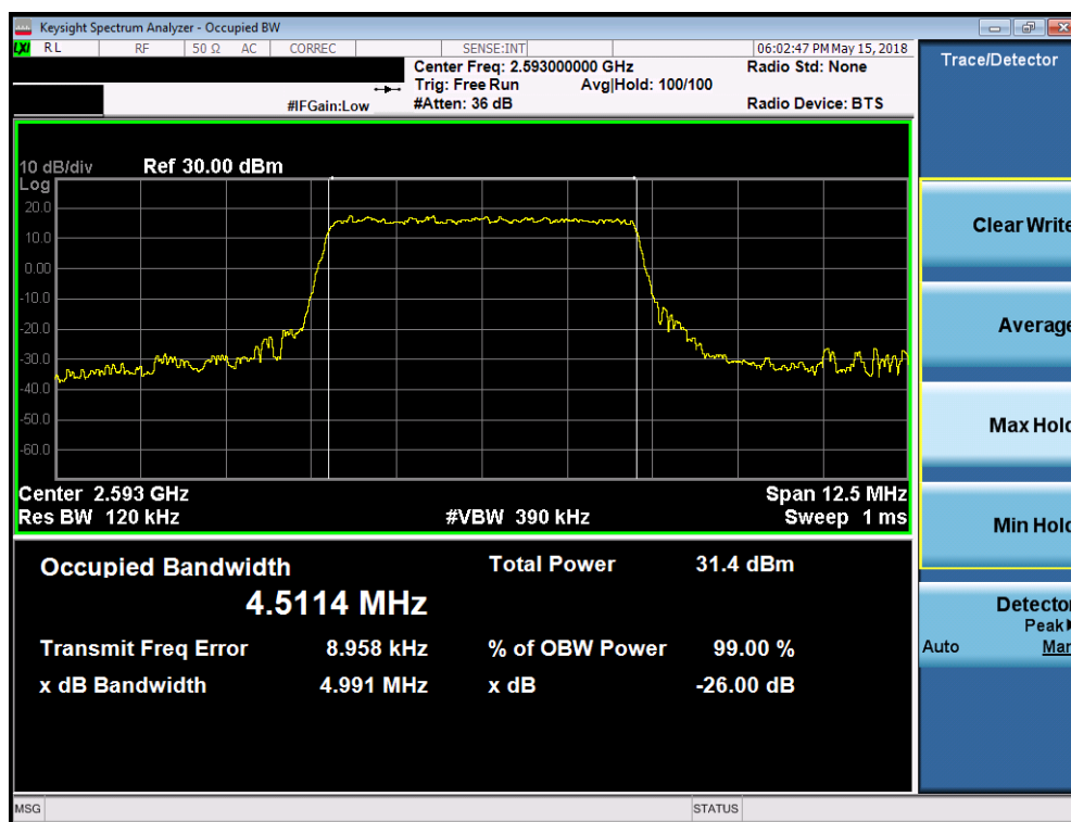
Plot 7-118. Occupied Bandwidth Plot (Band 41/38 - 5.0MHz QPSK - Full RB Configuration)
