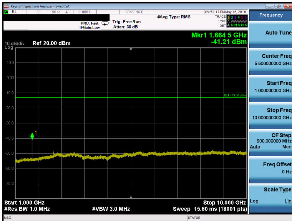
Plot 7-168. Conducted Spurious Plot (Band 26/5 - 10.0MHz QPSK - RB Size 1, RB Offset 0 - Mid Channel)
