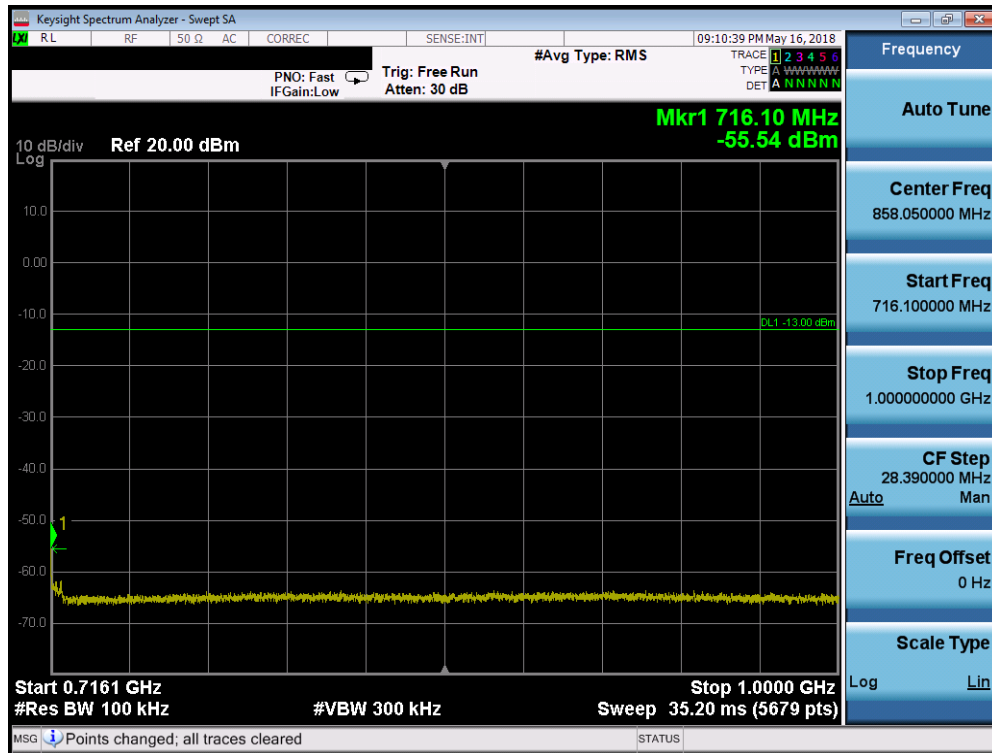
Plot 7-158. Conducted Spurious Plot (Band 12/17 - 10.0MHz QPSK - RB Size 1, RB Offset 0 - High Channel)
