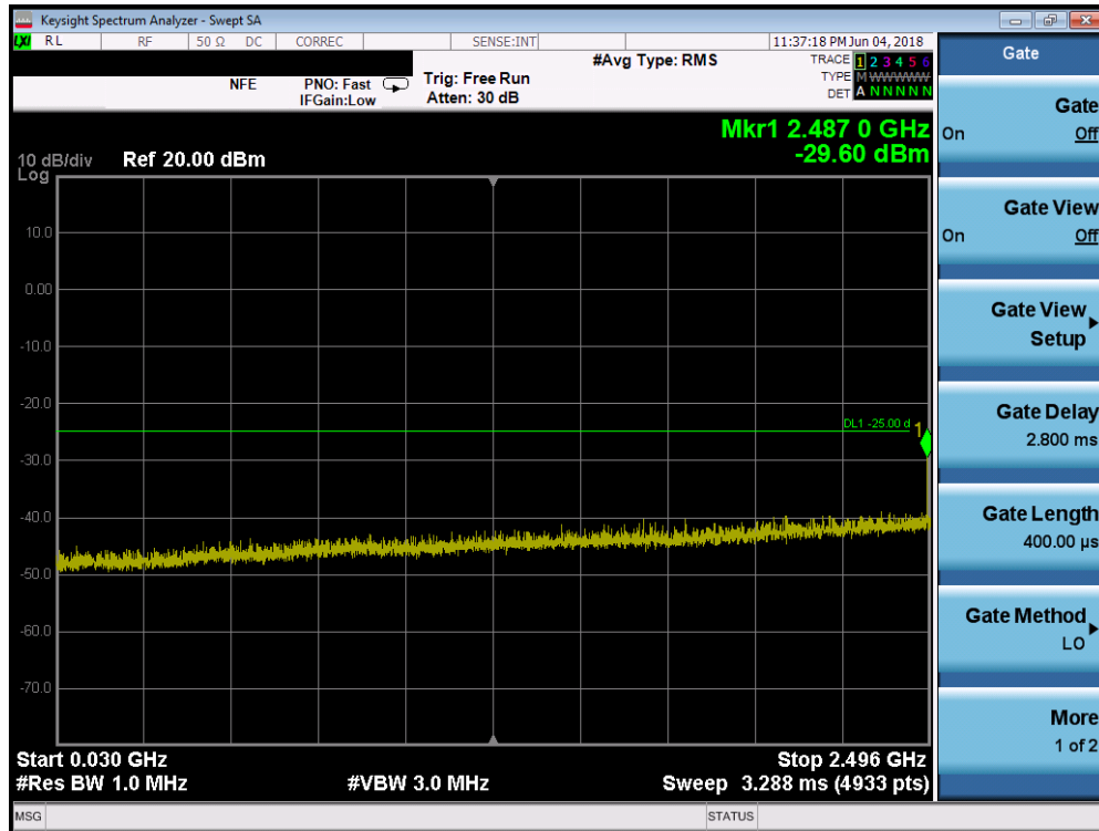
Plot 7-226. Conducted Spurious Plot (Band 41/38 - 20.0MHz QPSK - RB Size 1, RB Offset 0 - High Channel)
