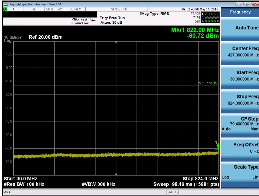
Plot 7-169. Conducted Spurious Plot (Band 26/5 - 10.0MHz QPSK - RB Size 1, RB Offset 0 - High Channel)
