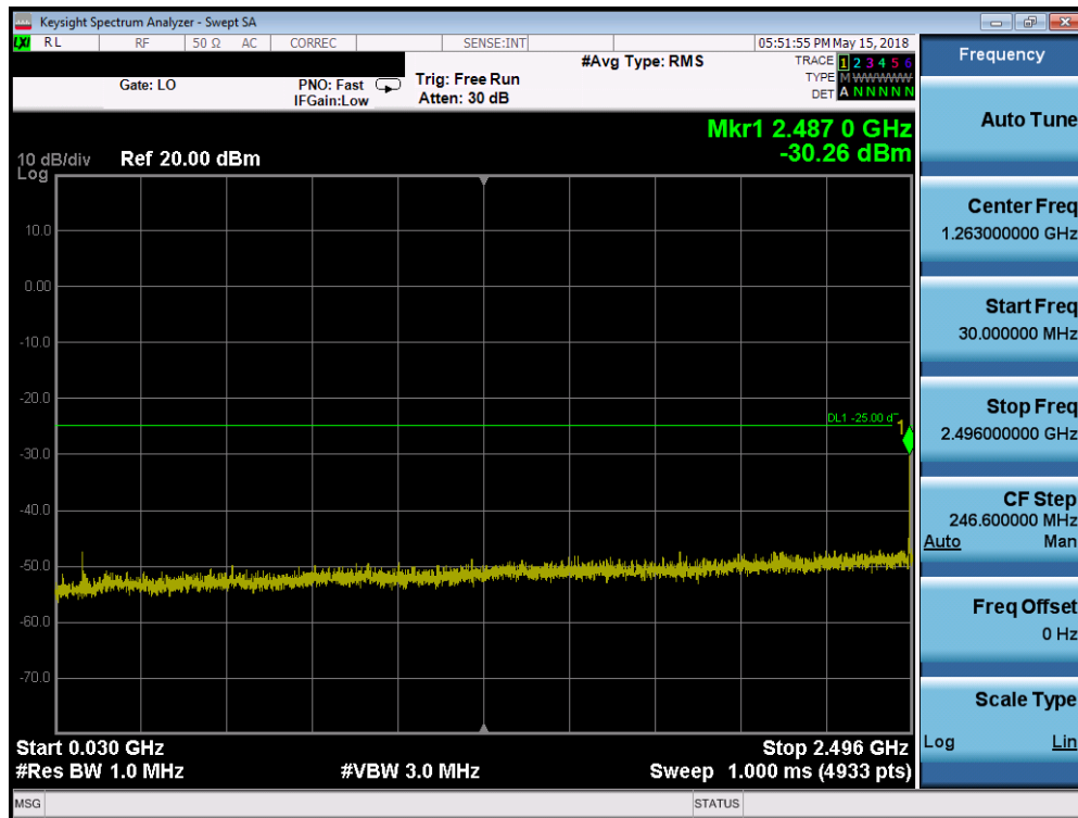
Plot 7-235. Conducted Spurious Plot (Band 41 - 20.0MHz QPSK - RB Size 1, RB Offset 0 - High Channel)
