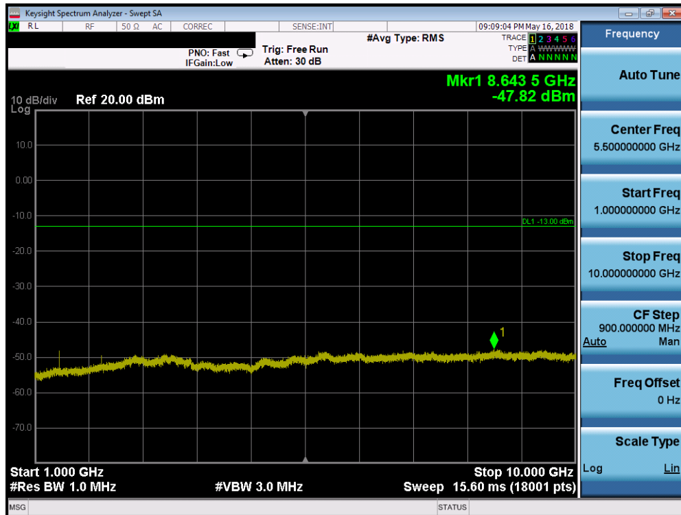
Plot 7-156. Conducted Spurious Plot (Band 12/17 - 10.0MHz QPSK - RB Size 1, RB Offset 0 - Mid Channel)
