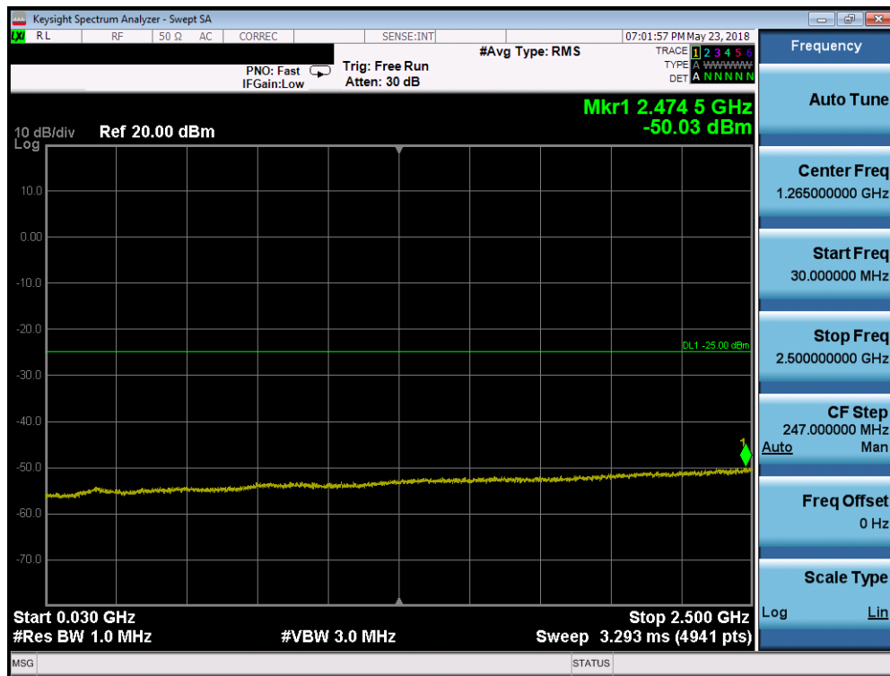
Plot 7-214. Conducted Spurious Plot (Band 7 - 15.0MHz QPSK - RB Size 1, RB Offset 0 - Mid Channel)
