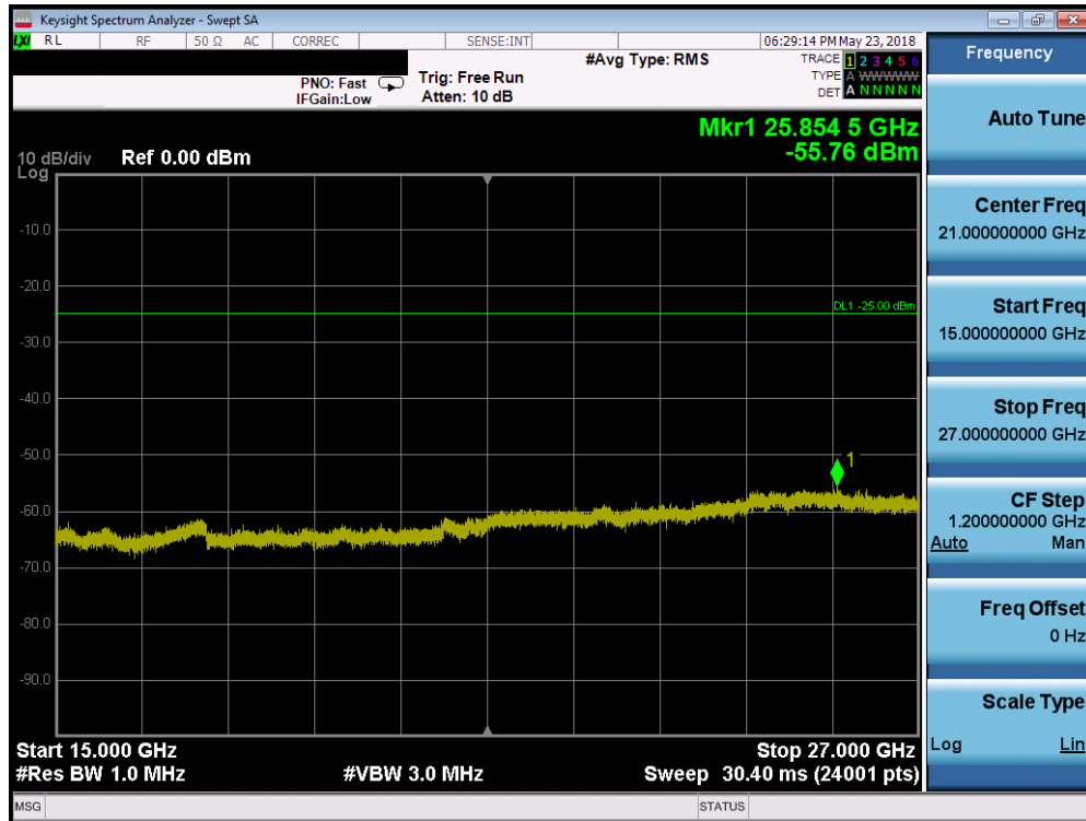
Plot 7-210. Conducted Spurious Plot (Band 7 - 15.0MHz QPSK - RB Size 1, RB Offset 0 - High Channel)
