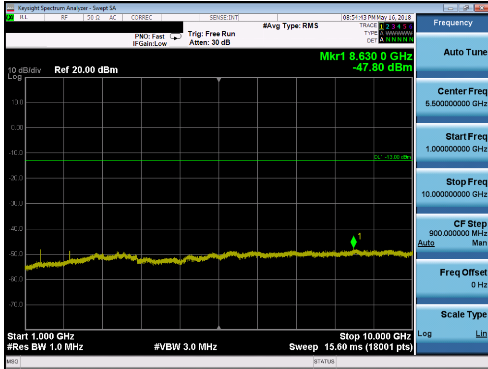
Plot 7-150. Conducted Spurious Plot (Band 71 - 20.0MHz QPSK - RB Size 1, RB Offset 0 - High Channel)
