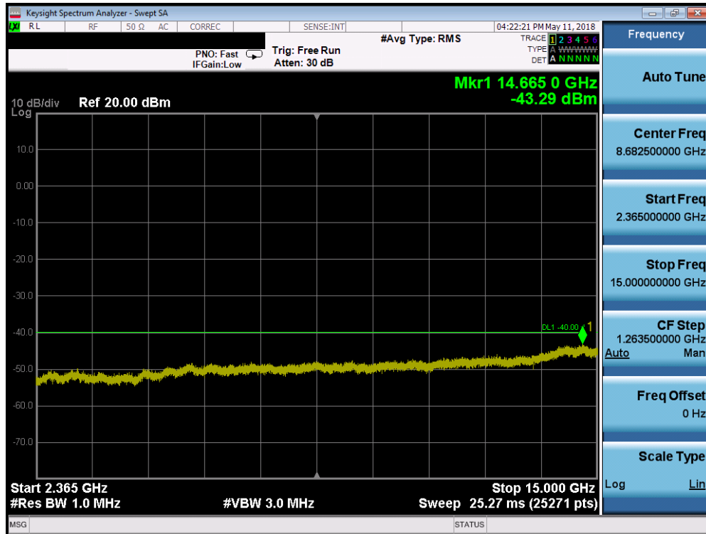
Plot 7-197. Conducted Spurious Plot (Band 30 - 5.0MHz QPSK - RB Size 1, RB Offset 0 - Mid Channel)
