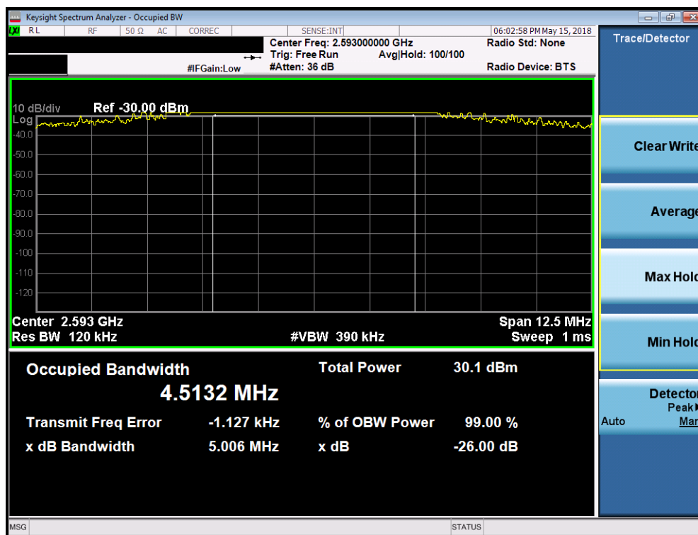
Plot 7-119. Occupied Bandwidth Plot (Band 41/38 - 5.0MHz 16-QAM - Full RB Configuration)
