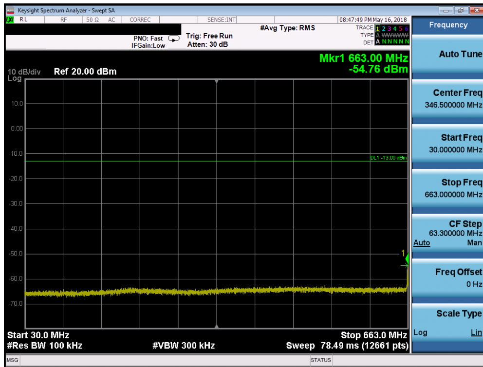
Plot 7-145. Conducted Spurious Plot (Band 71 - 20.0MHz QPSK - RB Size 1, RB Offset 0 - Mid Channel)
