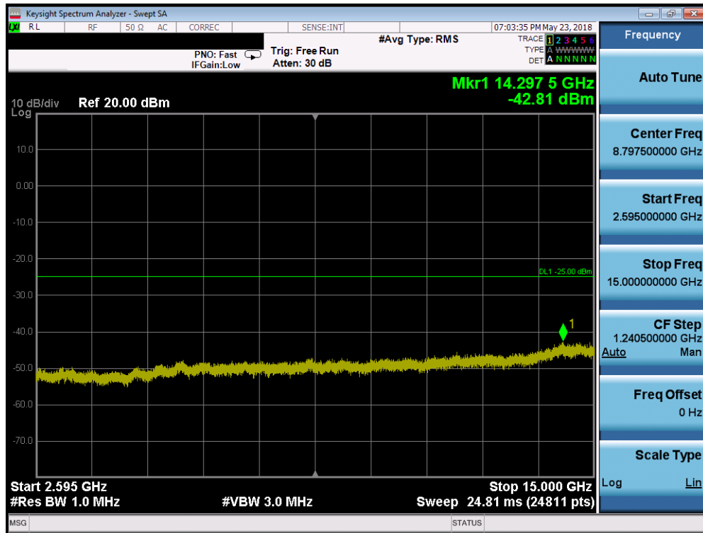
Plot 7-218. Conducted Spurious Plot (Band 7 - 15.0MHz QPSK - RB Size 1, RB Offset 0 - High Channel)
