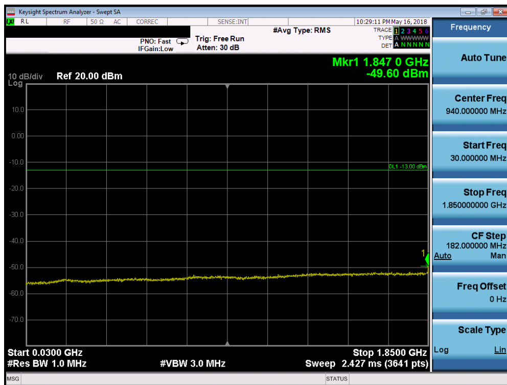
Plot 7-184. Conducted Spurious Plot (Band 25/2 - 20.0MHz QPSK - RB Size 1, RB Offset 0 - Mid Channel)
