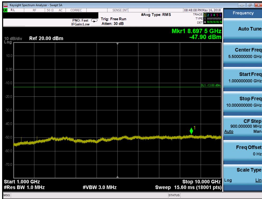
Plot 7-147. Conducted Spurious Plot (Band 71 - 20.0MHz QPSK - RB Size 1, RB Offset 0 - Mid Channel)
