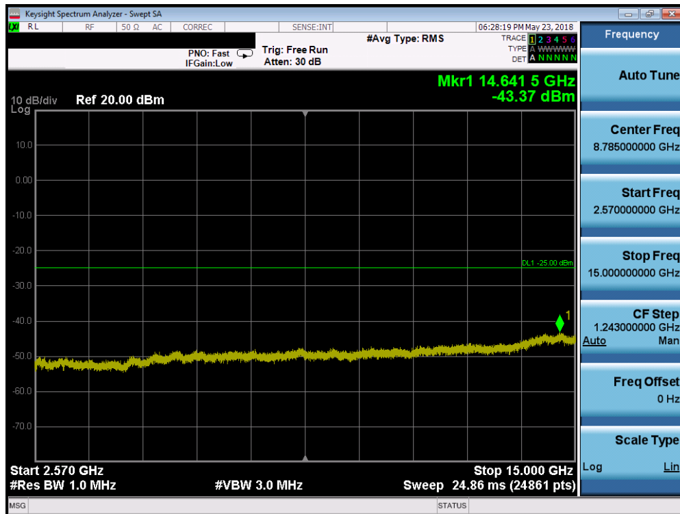
Plot 7-203. Conducted Spurious Plot (Band 7 - 15.0MHz QPSK - RB Size 1, RB Offset 0 - Low Channel)
