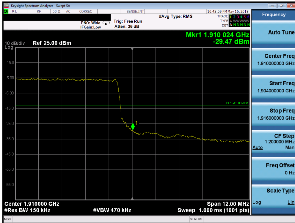
Plot 7-332. Upper Band Edge Plot (Band 2 - 15.0MHz QPSK - Full RB Configuration)
