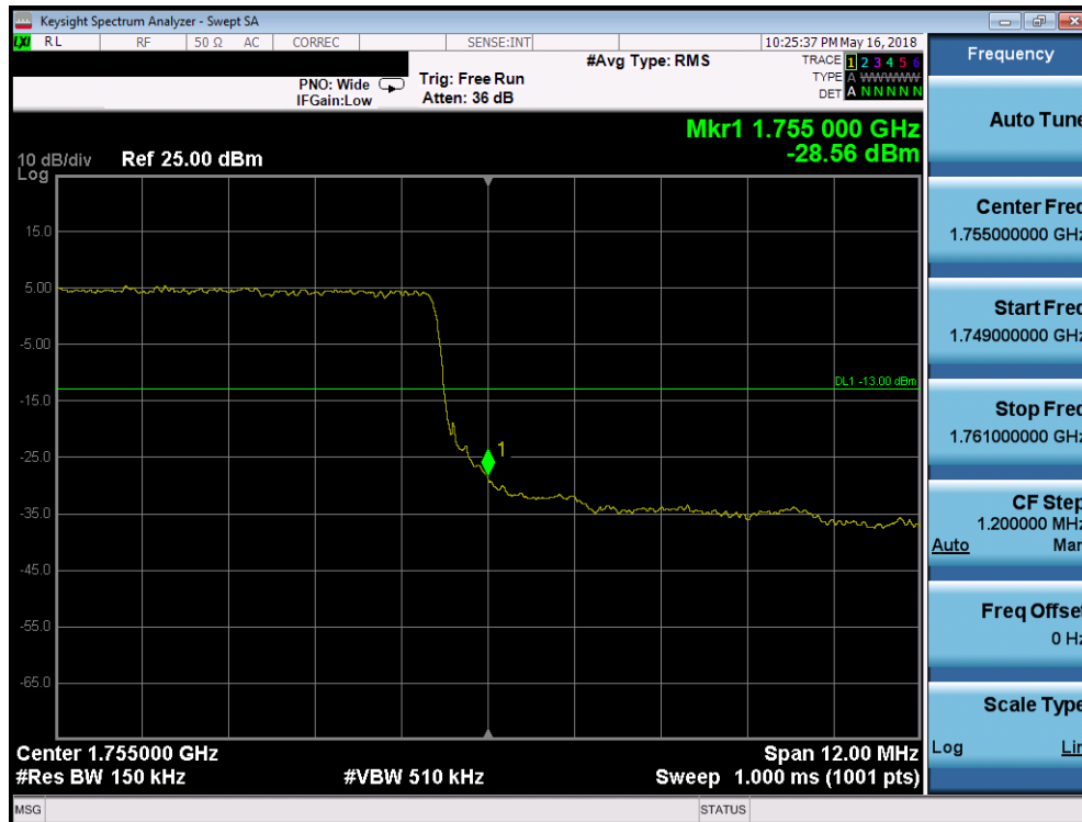
Plot 7-296. Upper Band Edge Plot (Band 4 - 15.0MHz QPSK - Full RB Configuration)
