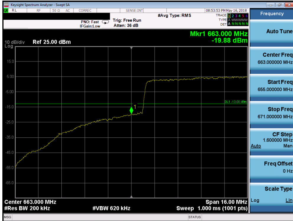
Plot 7-244. Lower Band Edge Plot (Band 71 - 20.0MHz QPSK - Full RB Configuration)
