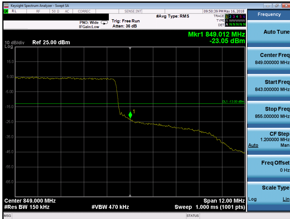
Plot 7-269. Upper Band Edge Plot (Band 26 - 15.0MHz QPSK - Full RB Configuration)
