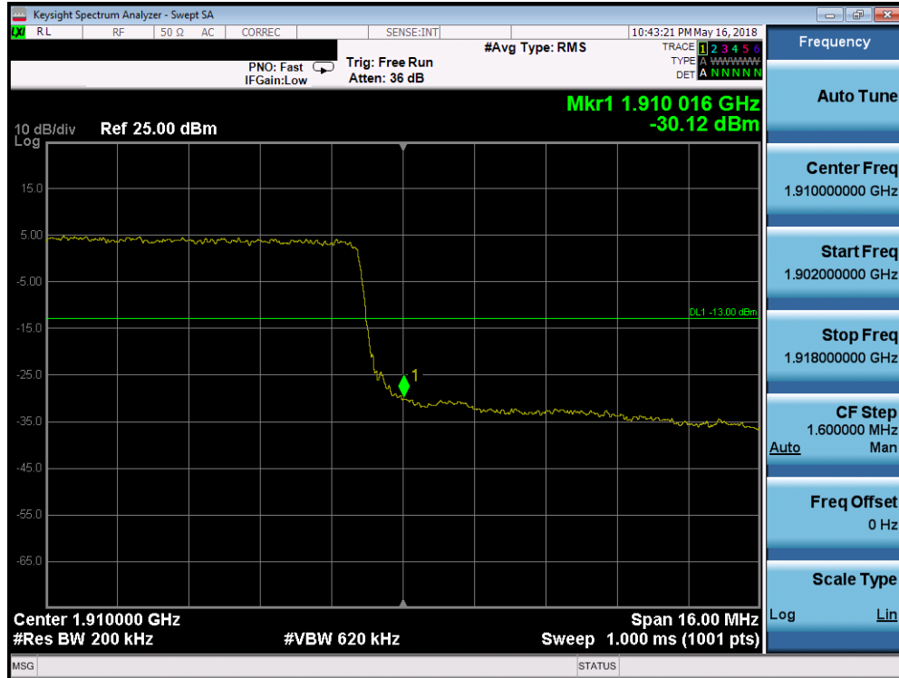
Plot 7-338. Upper Band Edge Plot (Band 2 - 20.0MHz QPSK - Full RB Configuration)
