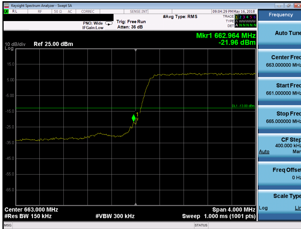
Plot 7-238. Lower Band Edge Plot (Band 71 - 5.0MHz QPSK - Full RB Configuration)
