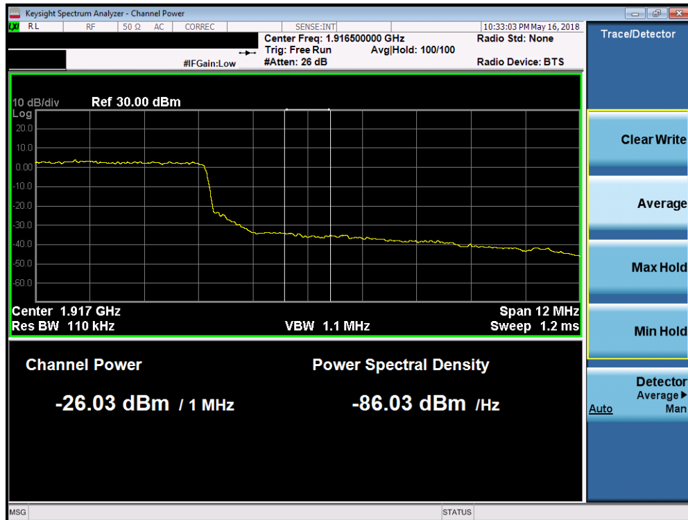
Plot 7-335. Upper Extended Band Edge Plot (Band 25 - 15.0MHz QPSK - Full RB Configuration)
