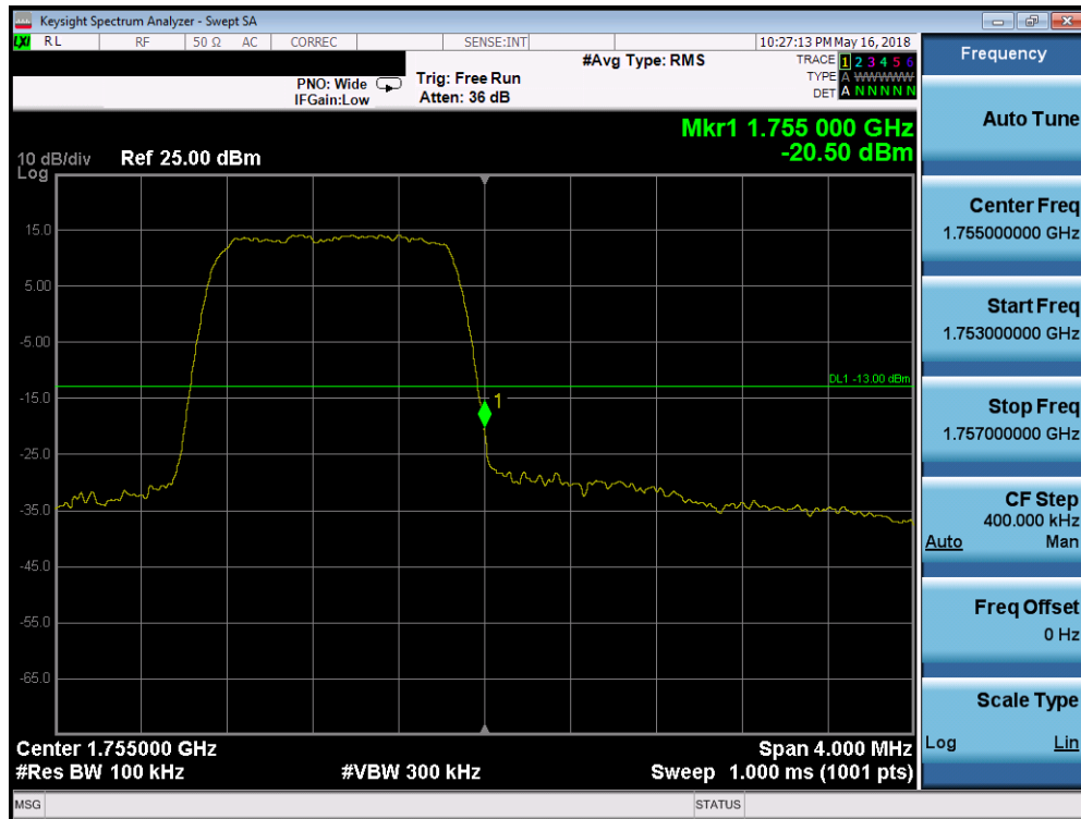
Plot 7-272. Upper Band Edge Plot (Band 4 - 1.4MHz QPSK - Full RB Configuration)
