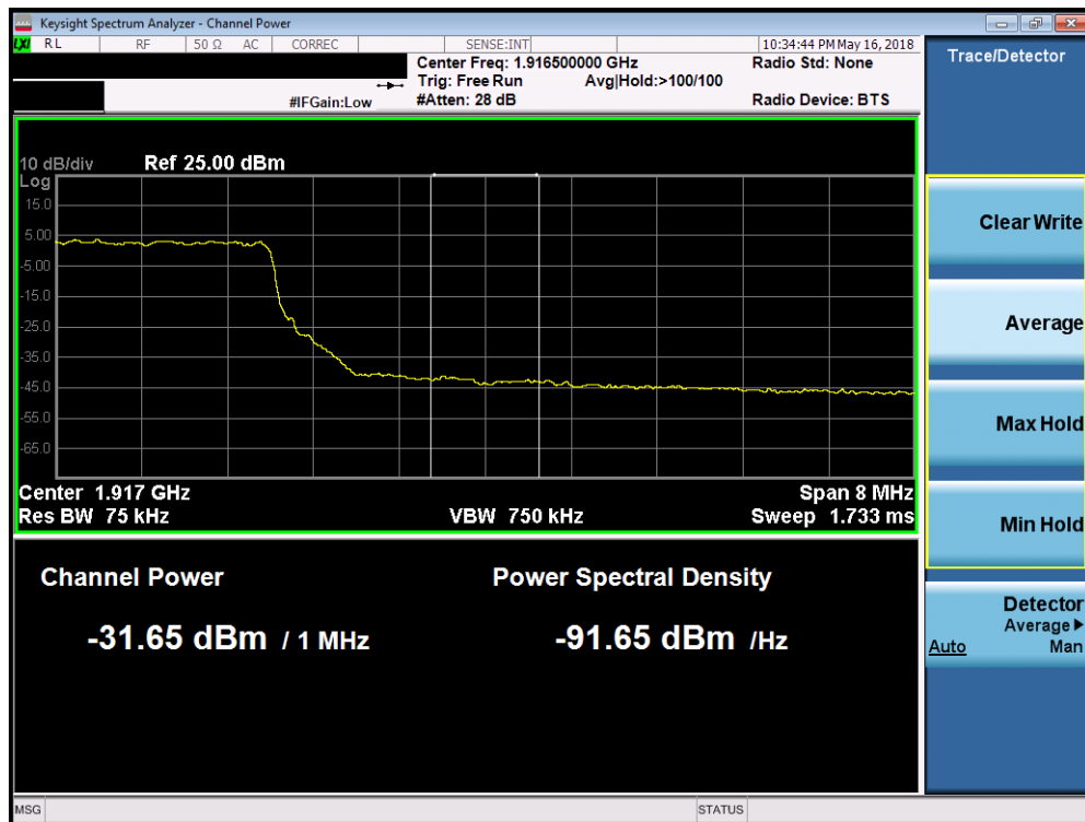
Plot 7-329. Upper Extended Band Edge Plot (Band 25 - 10.0MHz QPSK - Full RB Configuration)
