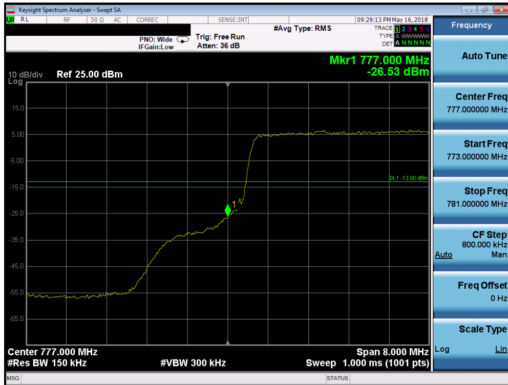
Plot 7-258. Lower Band Edge Plot (Band 13 - 10.0MHz QPSK - Full RB Configuration)
