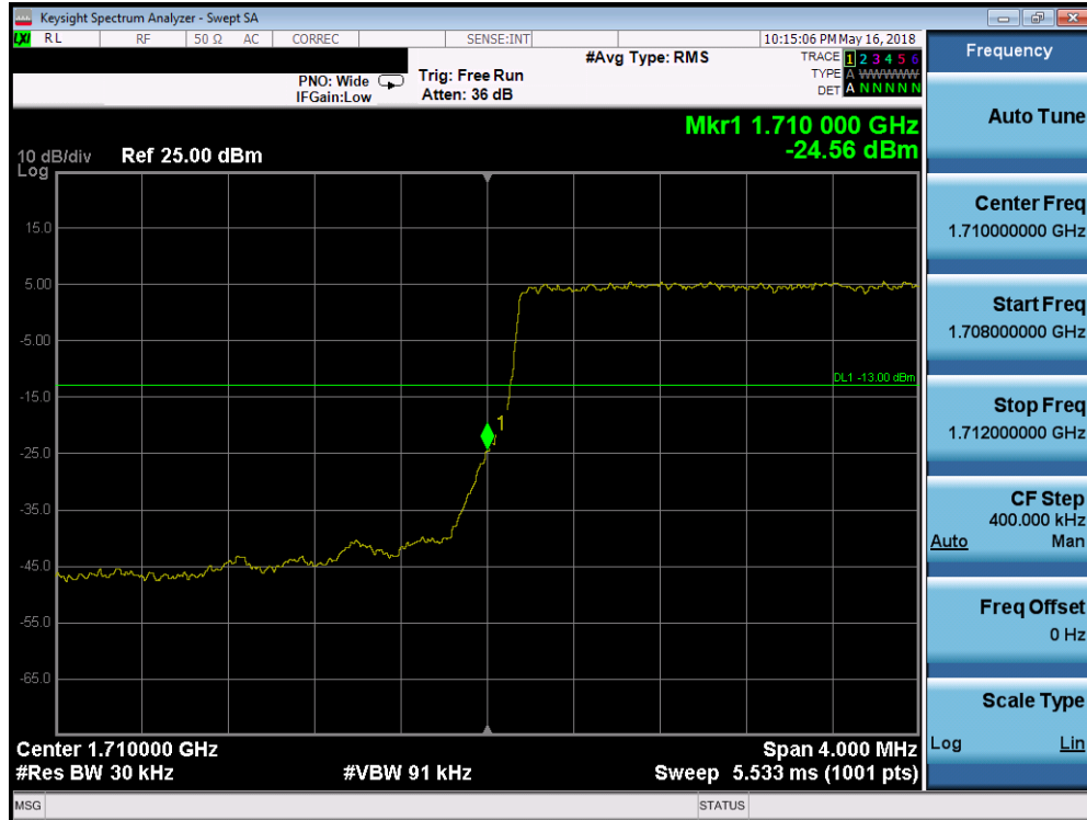
Plot 7-276. Lower Band Edge Plot (Band 66/4 - 3.0MHz QPSK - Full RB Configuration)
