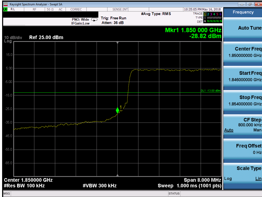
Plot 7-324. Lower Band Edge Plot (Band 25/2 - 10.0MHz QPSK - Full RB Configuration)
