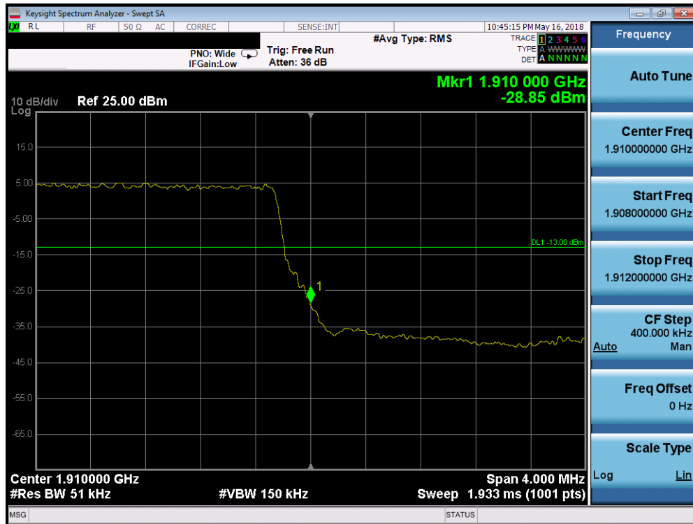
Plot 7-320. Upper Band Edge Plot (Band 2 - 5.0MHz QPSK - Full RB Configuration)
