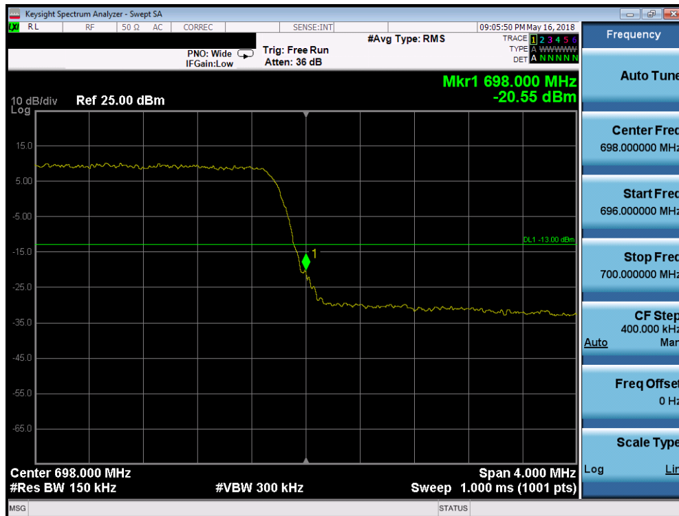
Plot 7-239. Upper Band Edge Plot (Band 71 - 5.0MHz QPSK - Full RB Configuration)
