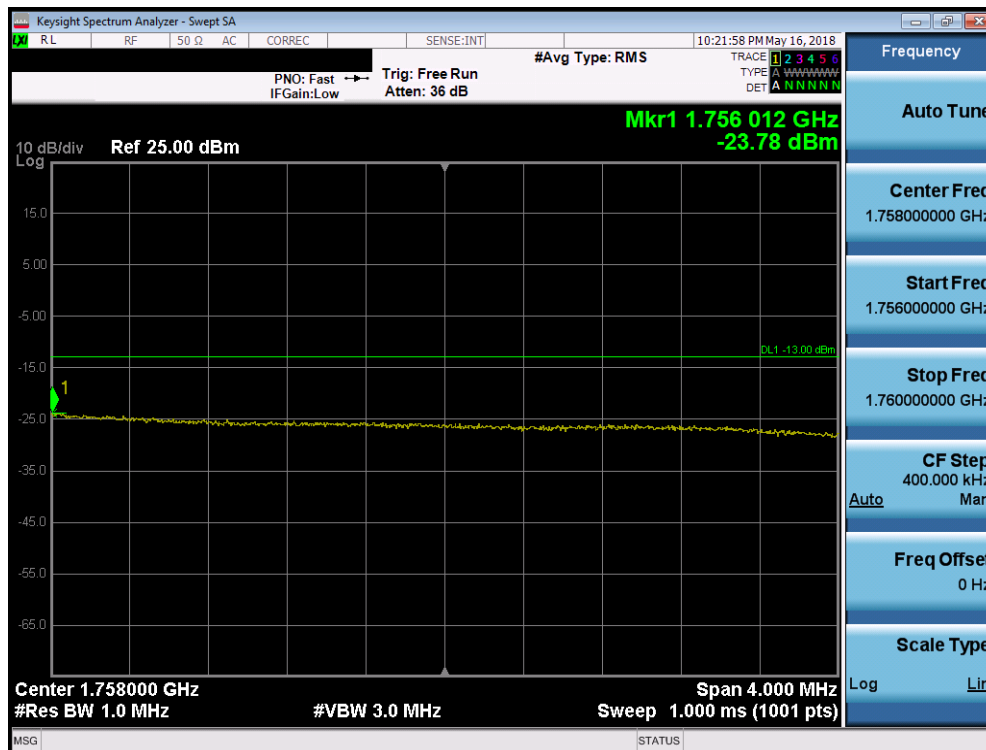
Plot 7-297. Upper Extended Band Edge Plot (Band 4 - 15.0MHz QPSK - Full RB Configuration)
