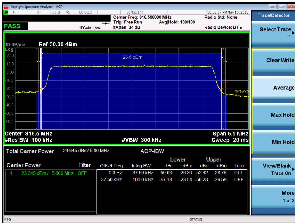
Plot 7-50. Channel Edge Plot (LTE Band 26 – 5MHz QPSK – RB Size 25– Low Channel)
