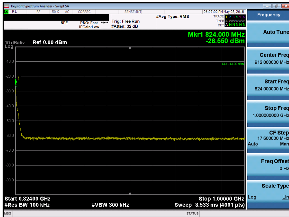
Plot 7-28. Conducted Spurious Plot (CDMA – Ch. 684)
