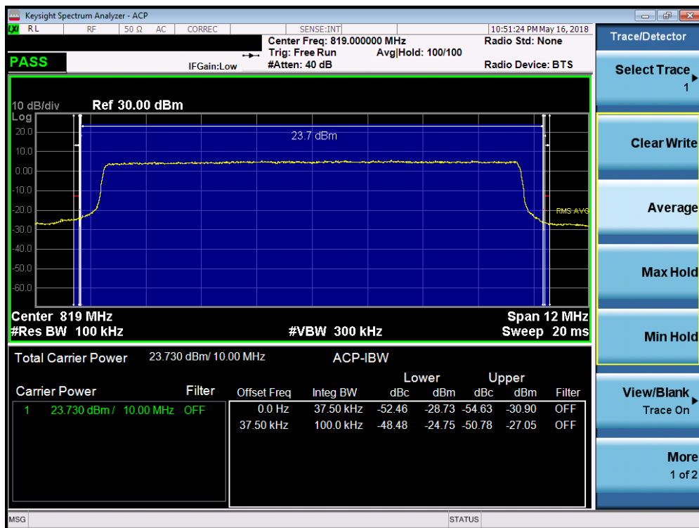
Plot 7-52. Channel Edge Plot (LTE Band 26 – 10MHz QPSK – RB Size 50)
