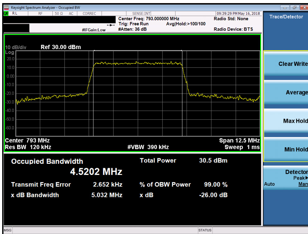
Plot 7-5. Occupied Bandwidth Plot (LTE Band 14 – 5MHz 64QAM – Full RB Configuration)
