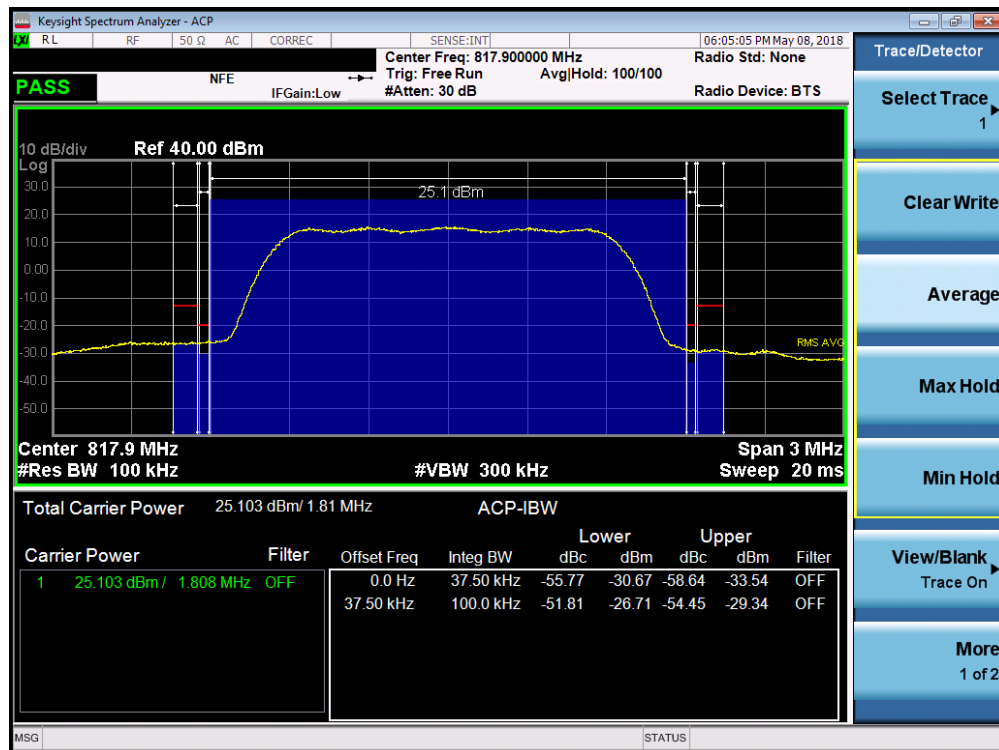
Plot 7-36. Channel Edge Plot (CDMA BC10 - Ch. 476)
