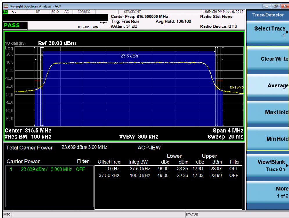
Plot 7-48. Channel Edge Plot (LTE Band 26 – 3MHz QPSK – RB Size 15– Low Channel)
