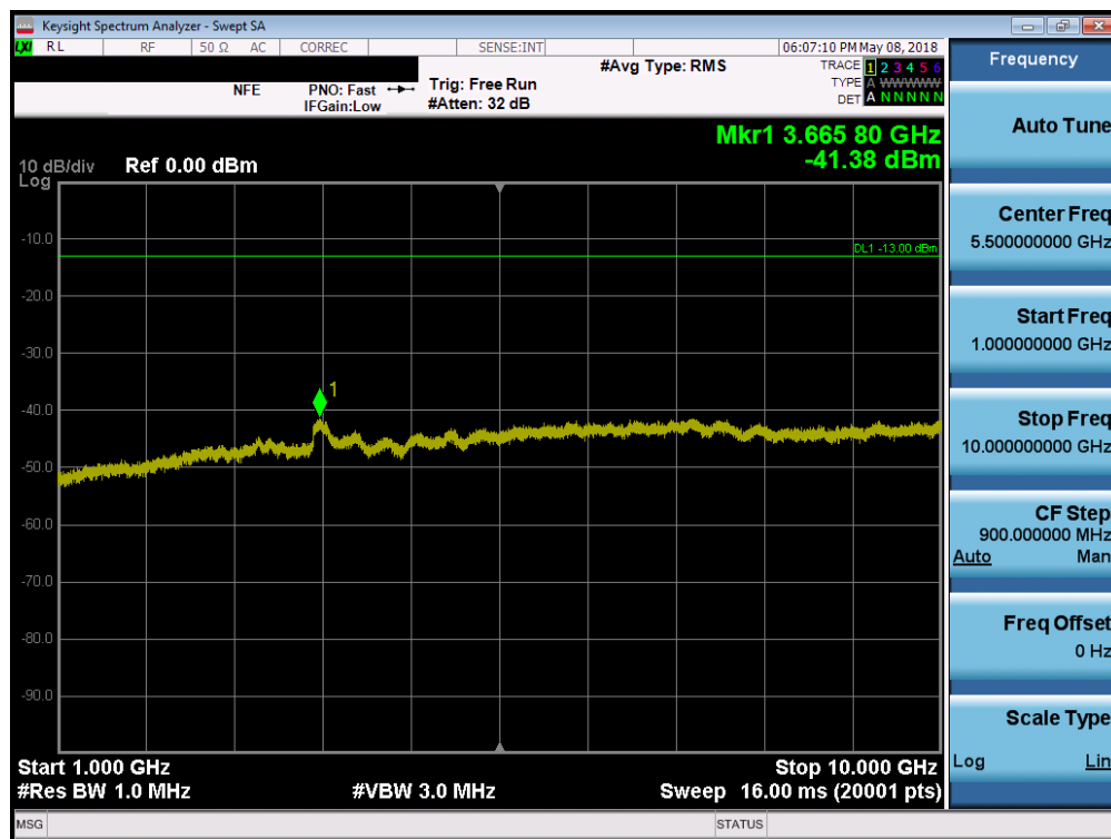
Plot 7-29. Conducted Spurious Plot (CDMA – Ch. 684)
