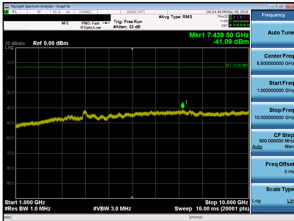
Plot 7-26. Conducted Spurious Plot (CDMA – Ch. 476)
