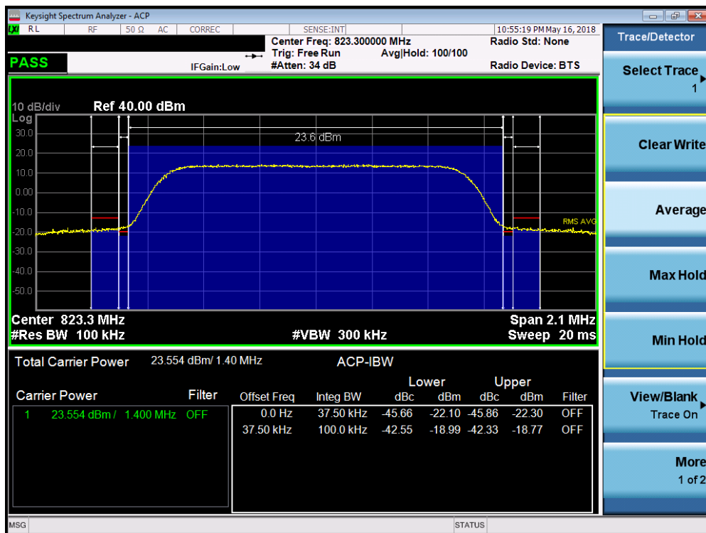
Plot 7-47. Channel Edge Plot (LTE Band 26 – 1.4MHz QPSK – RB Size 6 – High Channel)
