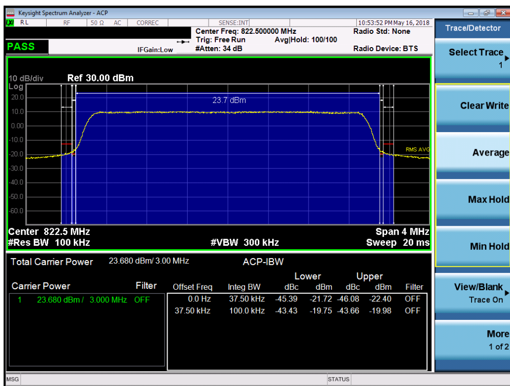
Plot 7-49. Channel Edge Plot (LTE Band 26 – 3MHz QPSK – RB Size 15 – High Channel)
