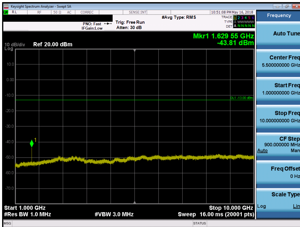
Plot 7-35. Conducted Spurious Plot (LTE B26 – 10MHz QPSK – RB Size 1, RB Offset 0)
