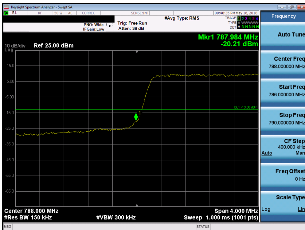
Plot 7-38. Lower Band Edge Plot (LTE Band 14 – 5MHz QPSK – Full RB Configuration)
