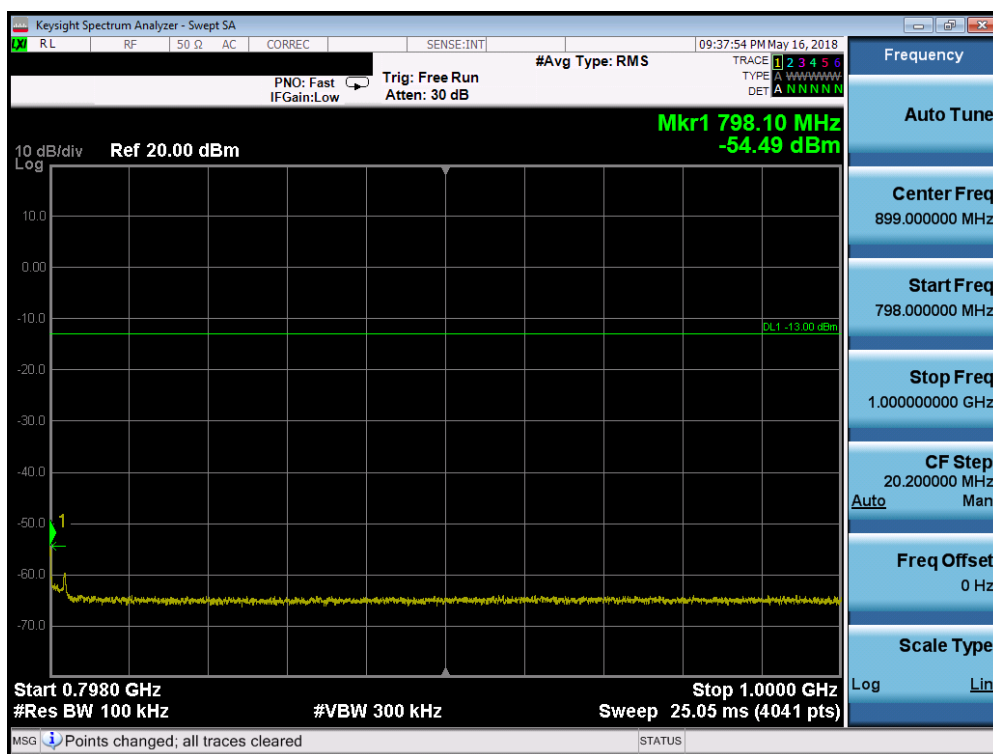
Plot 7-31. Conducted Spurious Plot (LTE B14 – 10MHz QPSK – RB Size 1, RB Offset 0)
