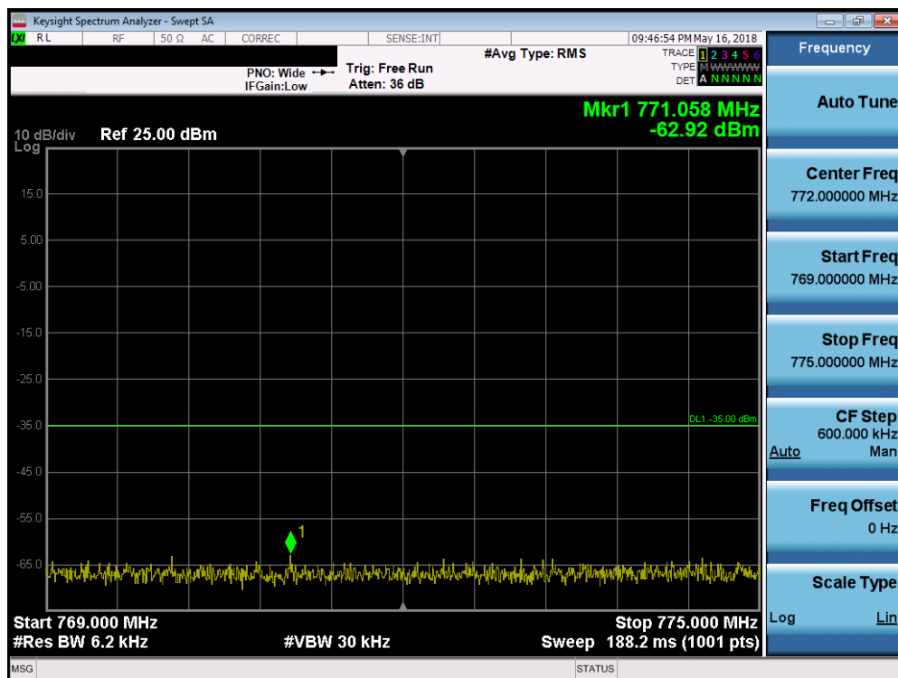
Plot 7-43. Lower Emission Mask Edge Plot (LTE Band 14 – 10MHz QPSK – Full RB Configuration)
