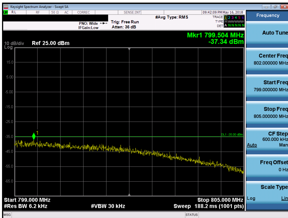
Plot 7-45. Upper Emission Mask Edge Plot (LTE Band 14 – 10MHz QPSK – Full RB Configuration)
