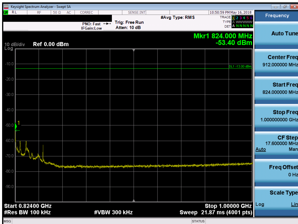
Plot 7-34. Conducted Spurious Plot (LTE B26 – 10MHz QPSK – RB Size 1, RB Offset 0)
