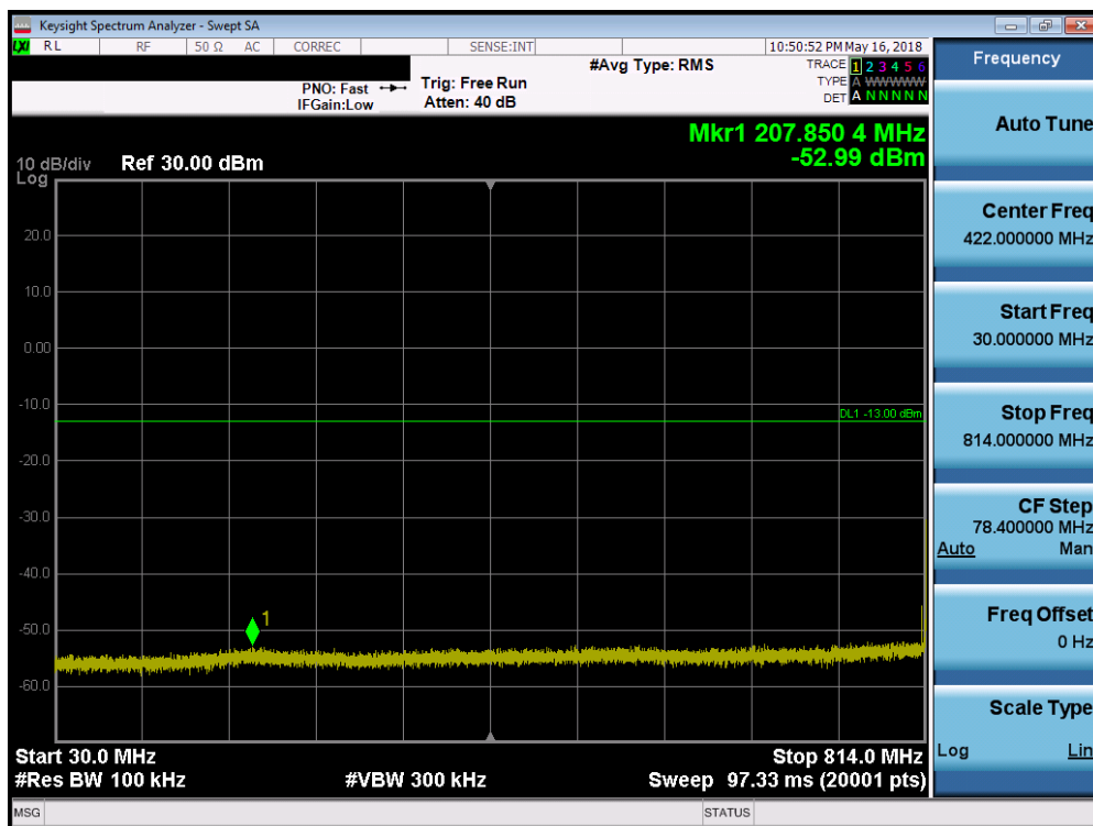
Plot 7-33. Conducted Spurious Plot (LTE B26 – 10MHz QPSK – RB Size 1, RB Offset 0)
