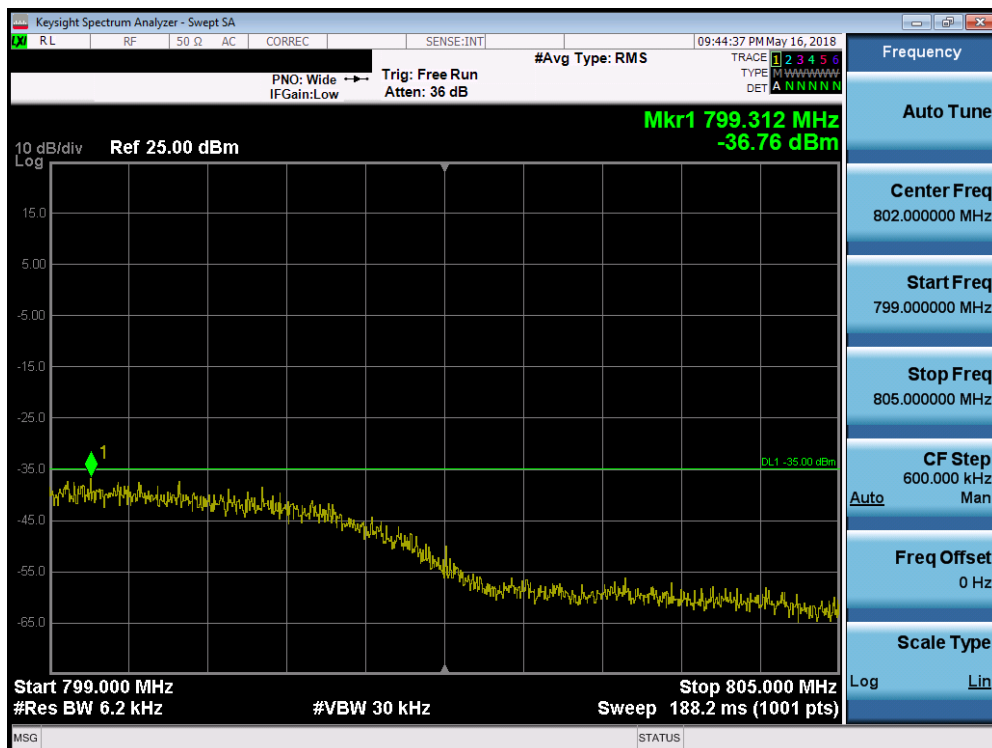
Plot 7-41. Upper Emission Mask Edge Plot (LTE Band 14 – 5MHz QPSK – Full RB Configuration)
