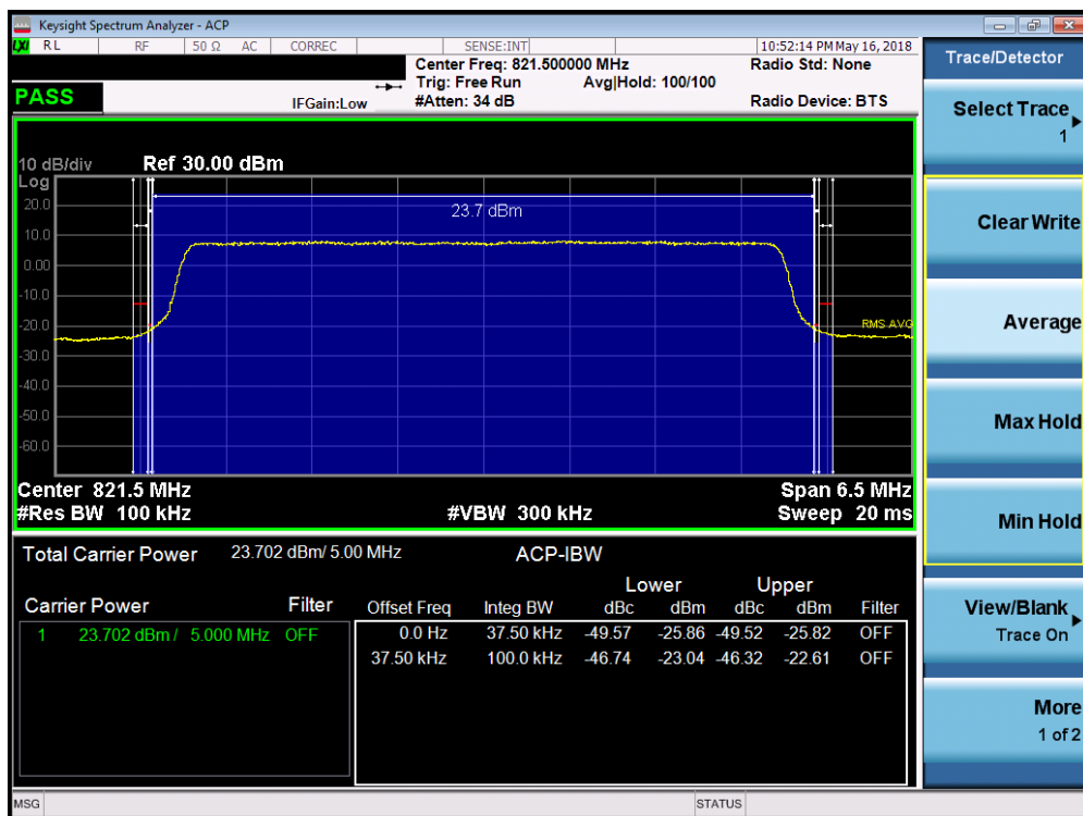
Plot 7-51. Channel Edge Plot (LTE Band 26 – 5MHz QPSK – RB Size 25 – High Channel)
