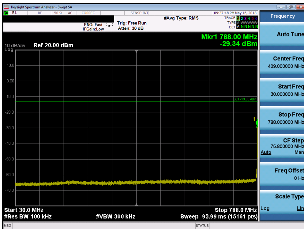
Plot 7-30. Conducted Spurious Plot (LTE B14 – 10MHz QPSK – RB Size 1, RB Offset 0)
