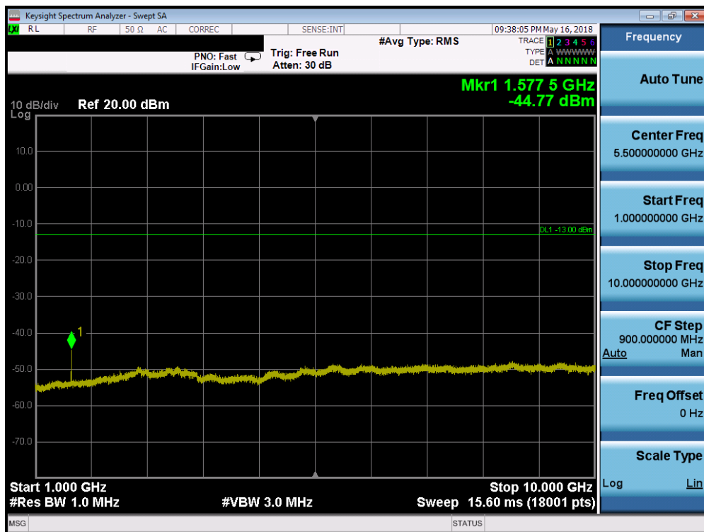
Plot 7-32. Conducted Spurious Plot (LTE B14 – 10MHz QPSK – RB Size 1, RB Offset 0)
