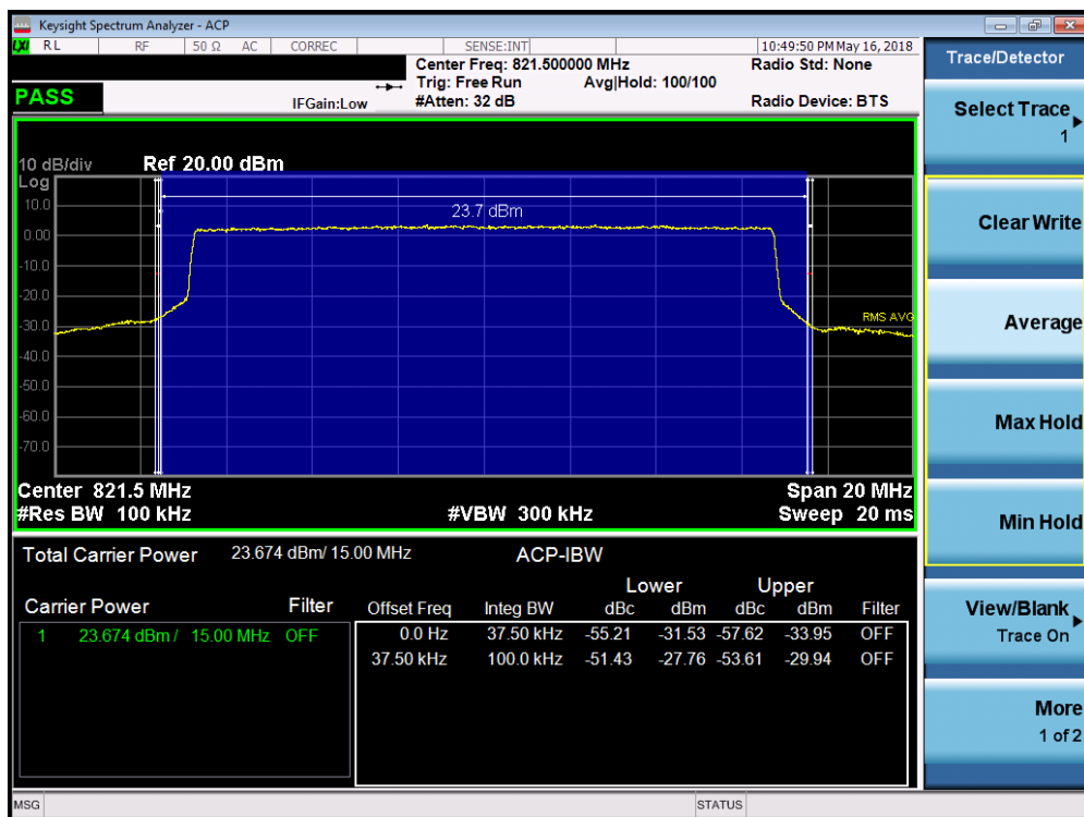
Plot 7-53. Channel Edge Plot (LTE Band 26 – 15MHz QPSK – RB Size 75)
