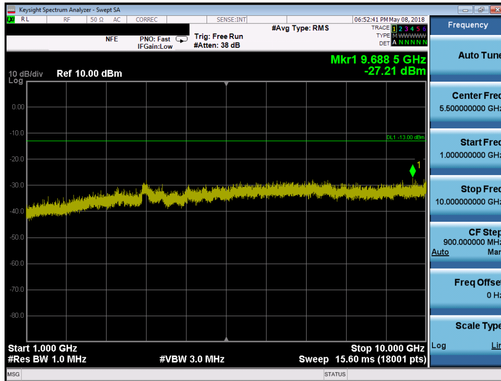
Plot 7-18. Conducted Spurious Plot (Cellular GPRS Mode - High Channel)
