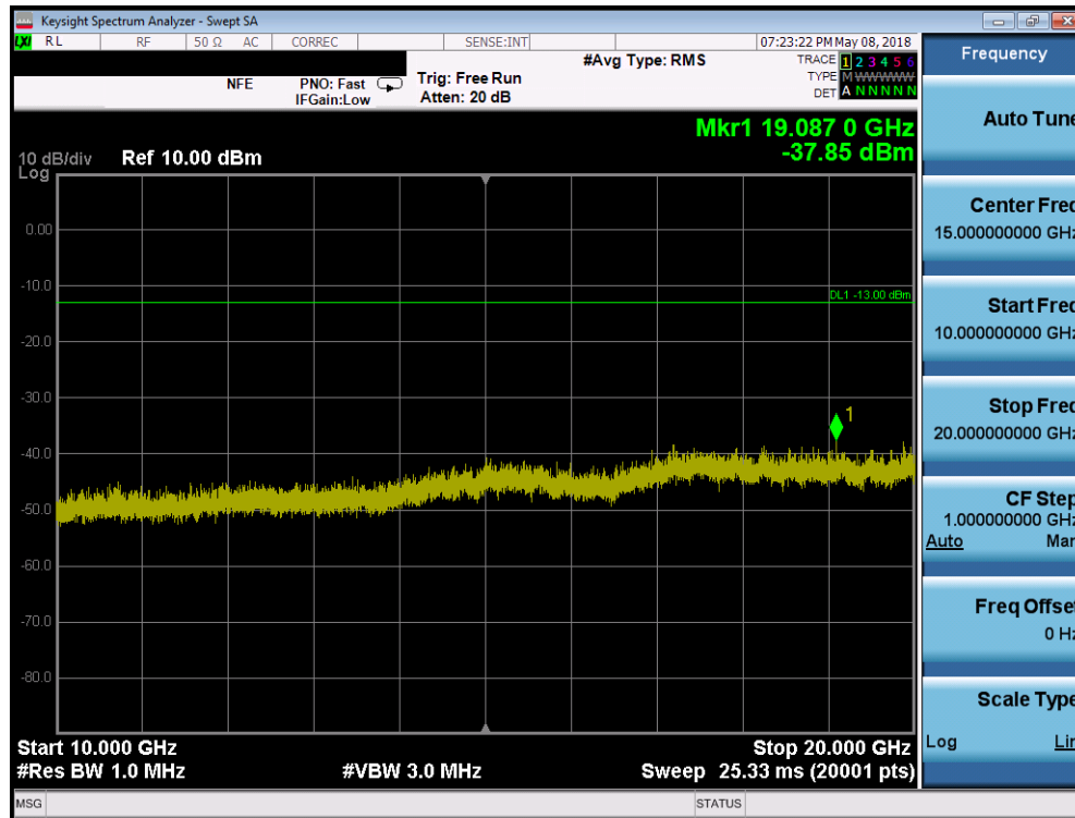
Plot 7-27. Conducted Spurious Plot (PCS GPRS Mode - High Channel)
