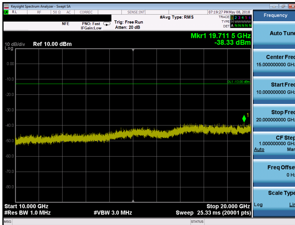
Plot 7-24. Conducted Spurious Plot (PCS GPRS Mode - Mid Channel)
