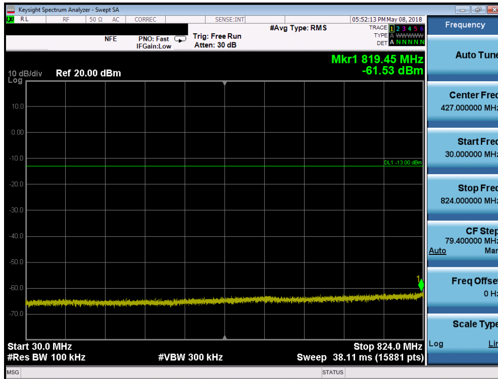
Plot 7-34. Conducted Spurious Plot (Cellular CDMA Mode - High Channel)
