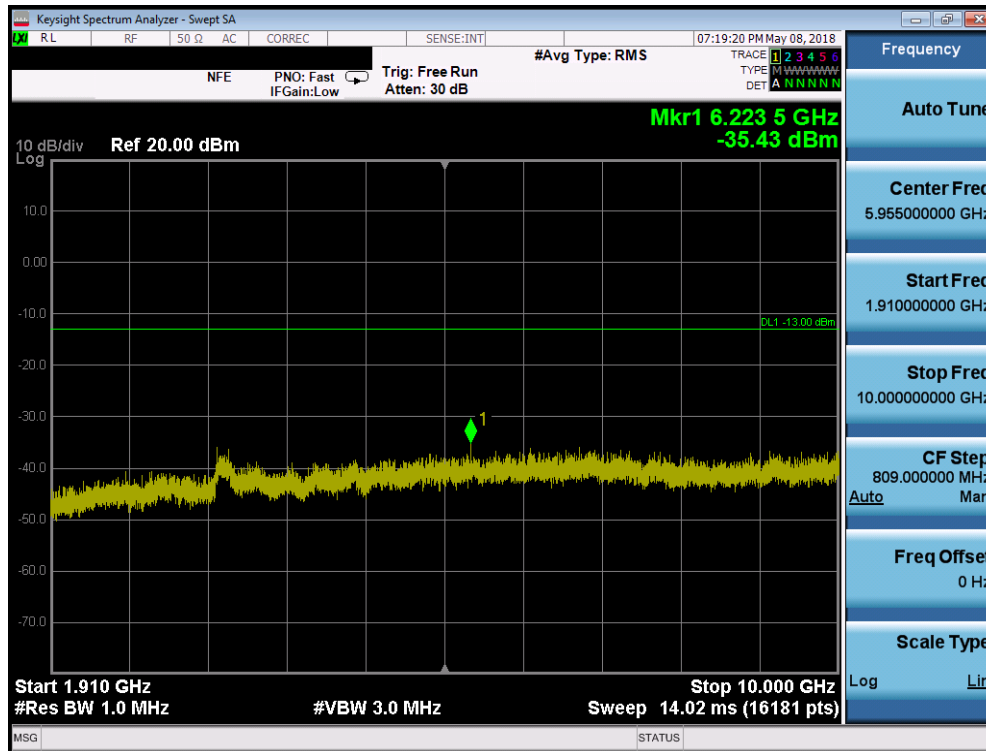
Plot 7-23. Conducted Spurious Plot (PCS GPRS Mode - Mid Channel)
