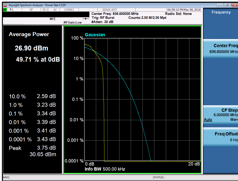
Plot 7-99. Peak-Average Ratio Plot (Cellular EDGE Mode)
