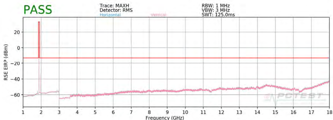
Plot 7-111. Radiated Spurious Plot Above 1GHz (PCS CDMA Mode)
