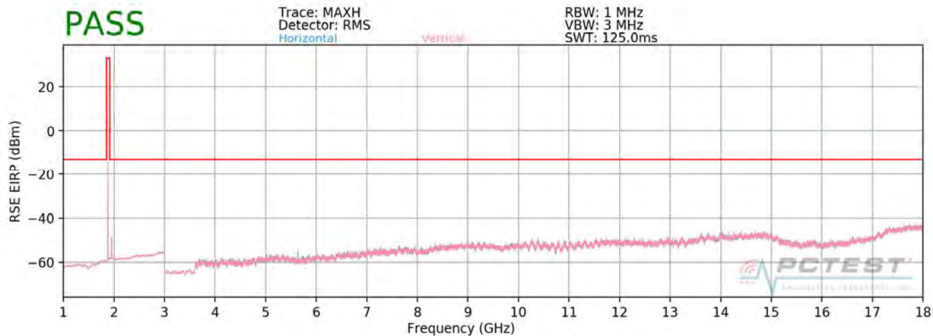
Plot 7-110. Radiated Spurious Plot Above 1GHz (PCS GPRS Mode)
