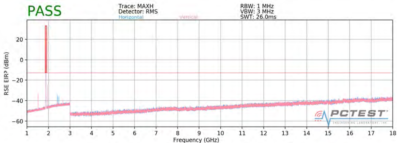
Plot 7-112. Radiated Spurious Plot Above 1GHz (PCS WCDMA Mode)
