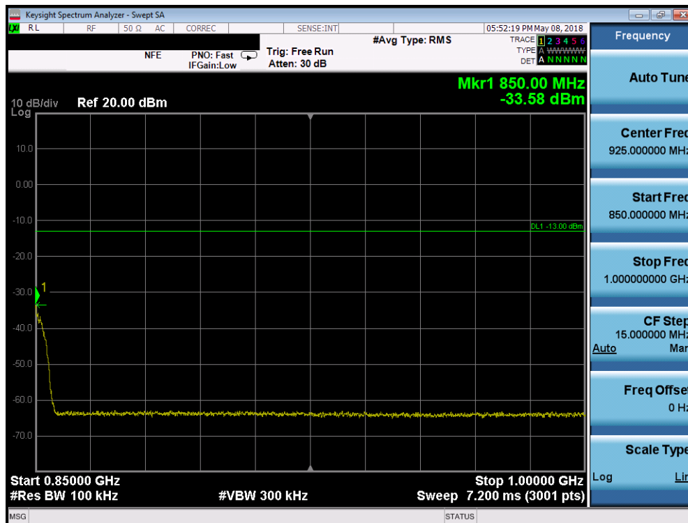
Plot 7-35. Conducted Spurious Plot (Cellular CDMA Mode - High Channel)
