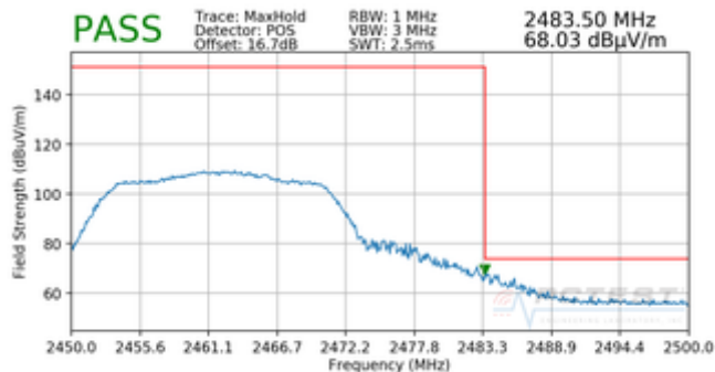
Plot 7-90. Radiated Restricted Upper Band Edge Measurement MIMO (Peak)
