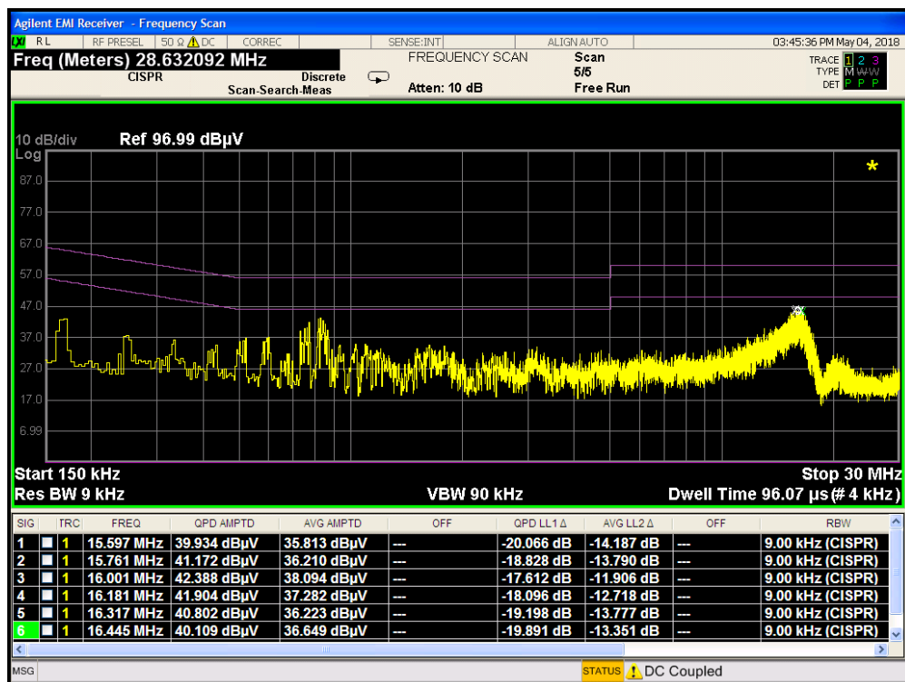
Plot 7-96. Line Conducted Plot with 802.11b (N) with Travel Adapter
