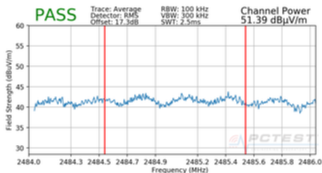
Plot 7-85. Radiated Restricted Band Edge Measurement CDD with WCP (Average)
