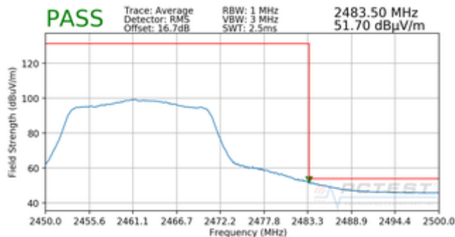
Plot 7-89. Radiated Restricted Upper Band Edge Measurement MIMO (Average)
