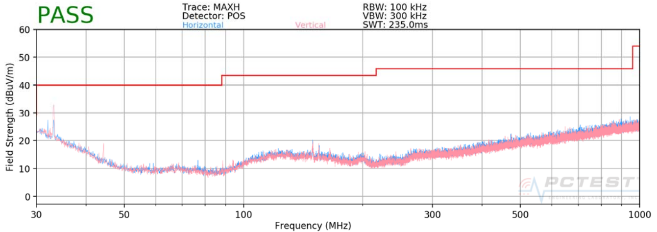
Plot 7-93. Radiated Spurious Plot below 1GHz SISO ANT1
