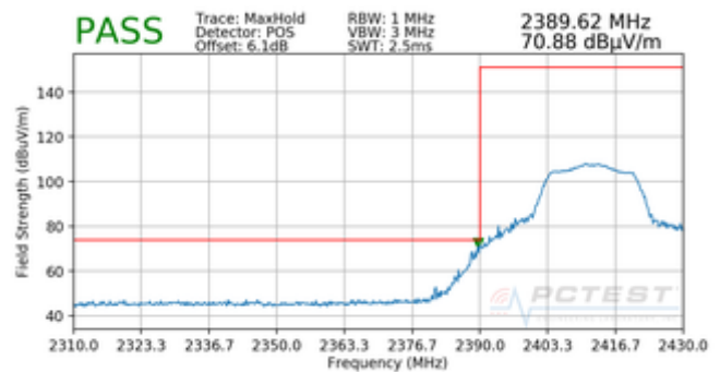
Plot 7-76. Radiated Restricted Lower Band Edge Measurement SISO ANT2 (Peak)
