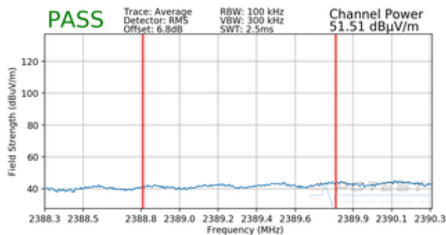
Plot 7-75. Radiated Restricted Lower Band Edge Measurement SISO ANT2 (Average)
