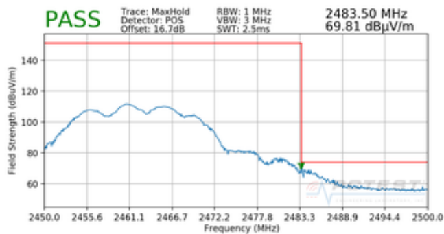
Plot 7-84. Radiated Restricted Upper Band Edge Measurement CDD (Peak)
