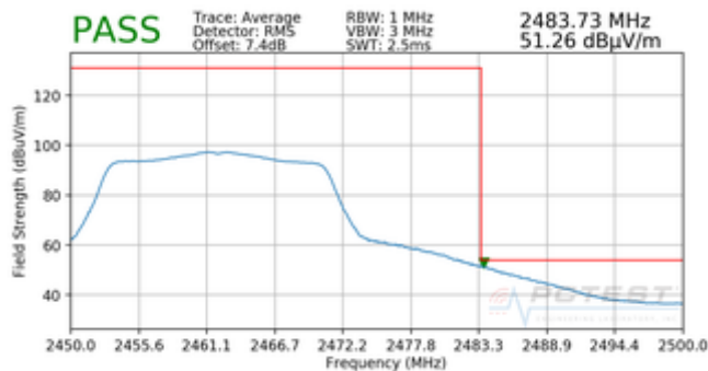
Plot 7-77. Radiated Restricted Upper Band Edge Measurement SISO ANT2 (Average)
