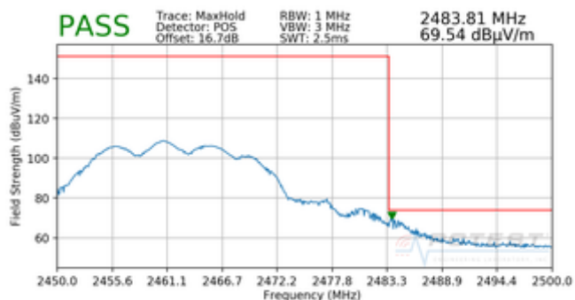
Plot 7-86. Radiated Restricted Band Edge Measurement CDD with WCP (Peak)
