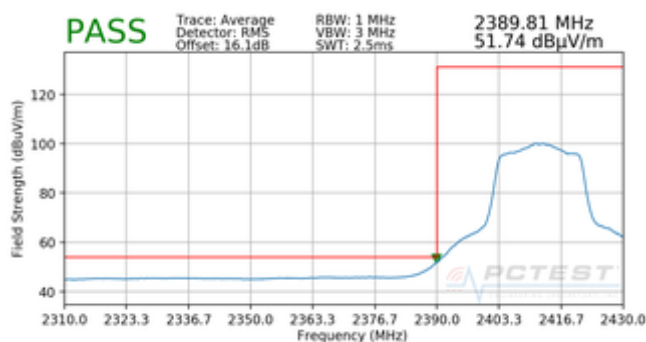
Plot 7-87. Radiated Restricted Lower Band Edge Measurement MIMO (Average)
