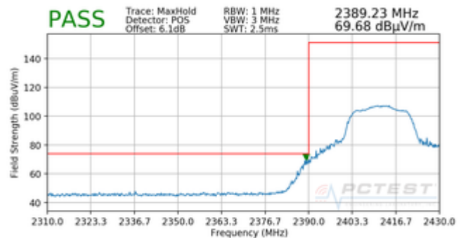
Plot 7-80. Radiated Restricted Band Edge Measurement SISO ANT2 with WCP (Peak)
