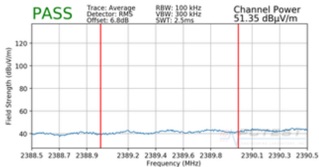
Plot 7-79. Radiated Restricted Band Edge Measurement SISO ANT2 with WCP (Average)
