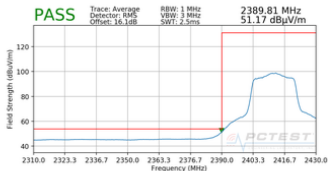
Plot 7-91. Radiated Restricted Band Edge Measurement MIMO with WCP (Average)
