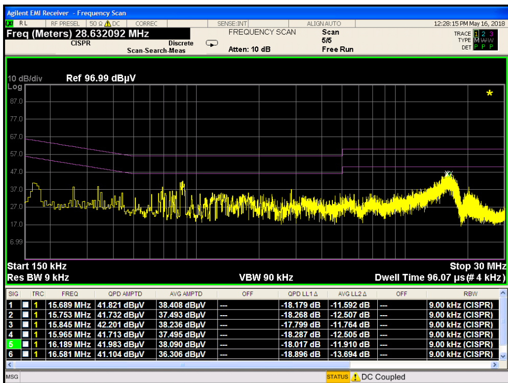
Plot 7-98. Line Conducted Plot with 802.11b (N) with Wireless Charging Pad
