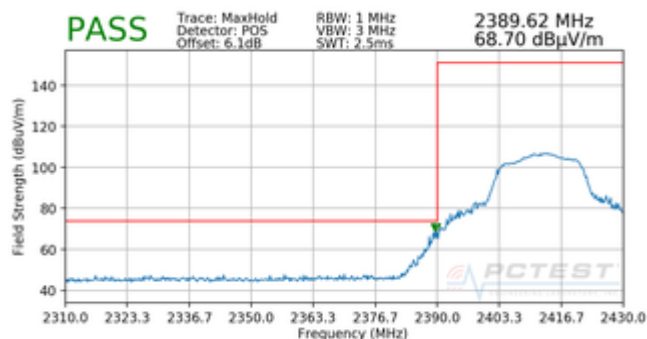
Plot 7-74. Radiated Restricted Band Edge Measurement SISO ANT1 with WCP (Peak)
