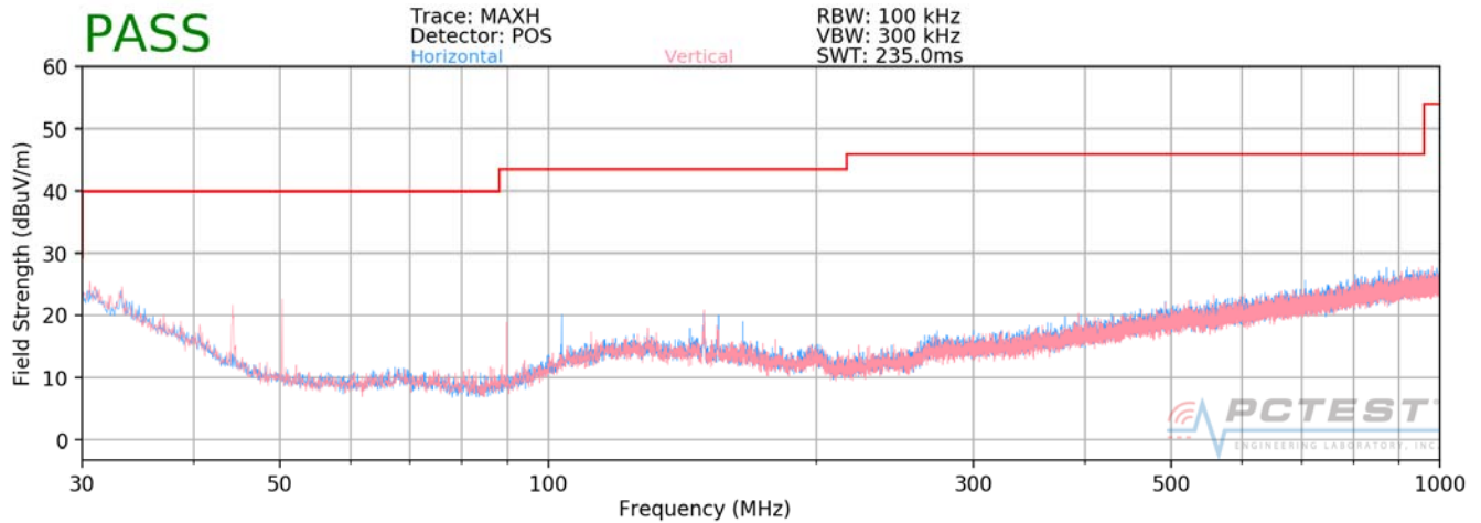
Plot 7-94. Radiated Spurious Plot below 1GHz SISO ANT2
