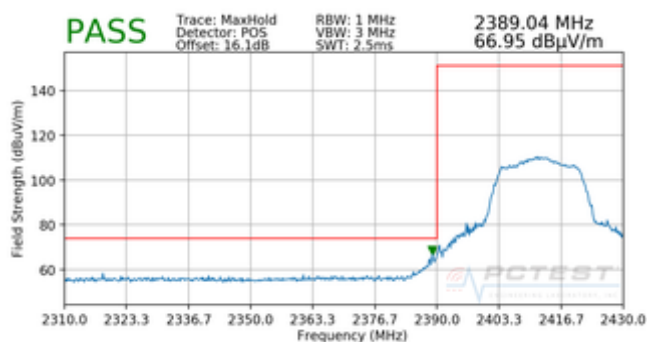
Plot 7-88. Radiated Restricted Lower Band Edge Measurement MIMO (Peak)
