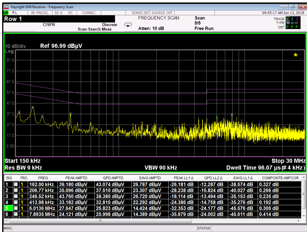
Plot 7-97. Line Conducted Plot with 802.11b (L1) with Wireless Charging Pad
