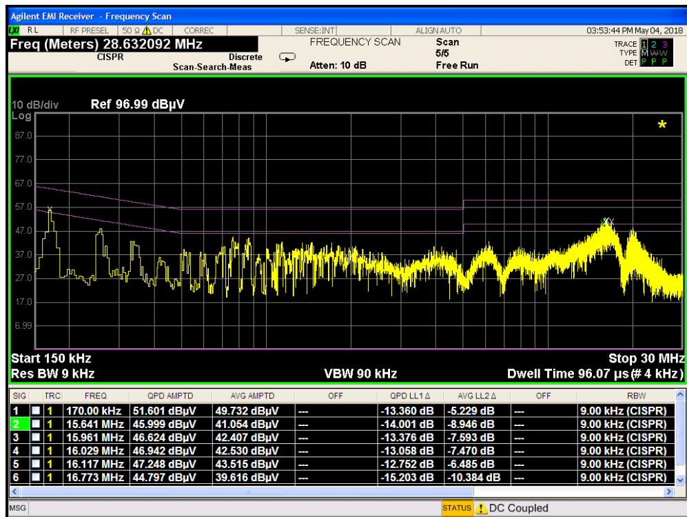
Plot 7-95. Line Conducted Plot with 802.11b (L1) with Travel Adapter
