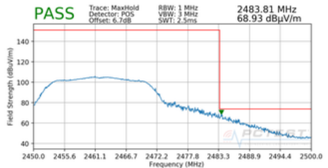
Plot 7-78. Radiated Restricted Upper Band Edge Measurement SISO ANT2 (Peak)
