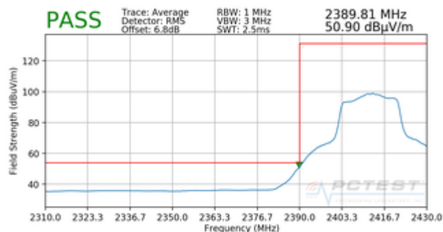
Plot 7-73. Radiated Restricted Band Edge Measurement SISO ANT1 with WCP (Average)
