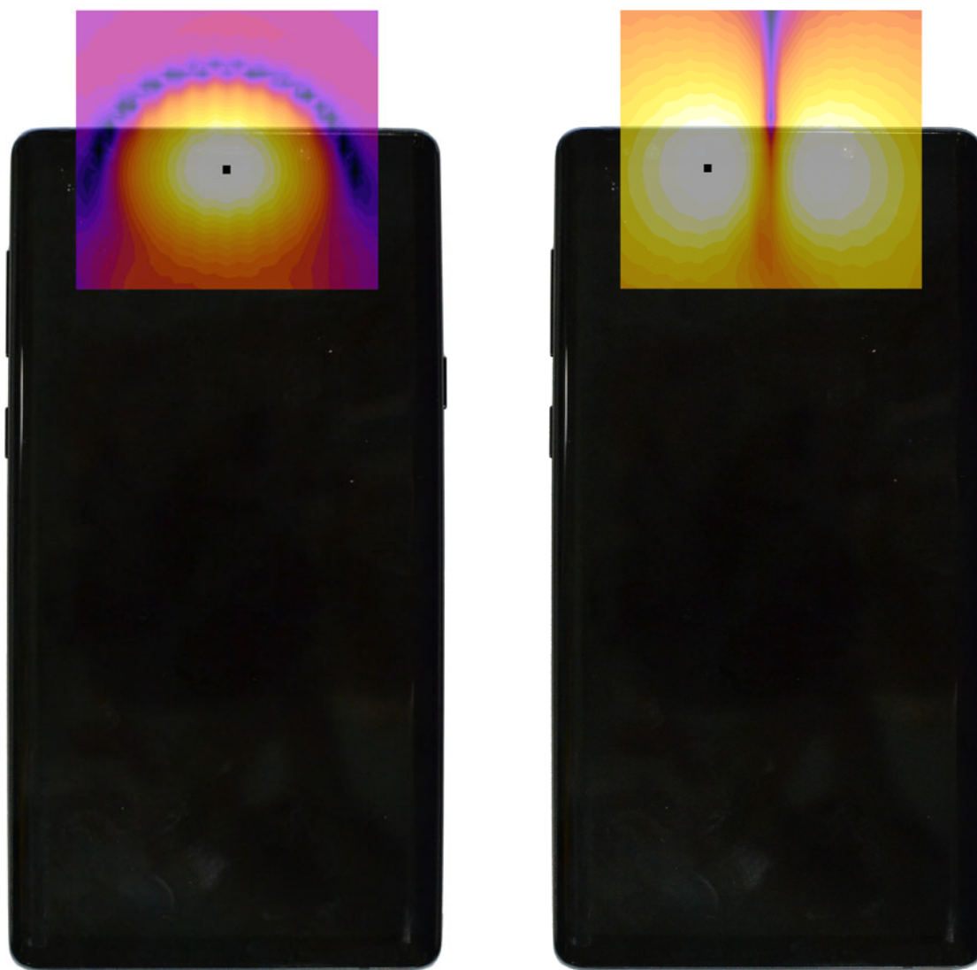
Figure 16-3 T-Coil Scan Overlay Magnetic Field Distributions
