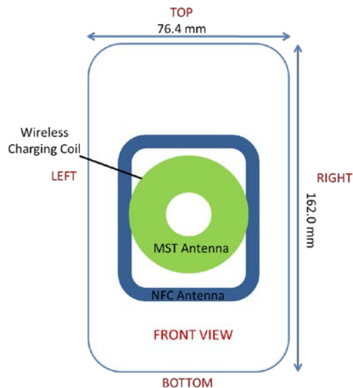
Figure F-2 NFC Antenna Locations
