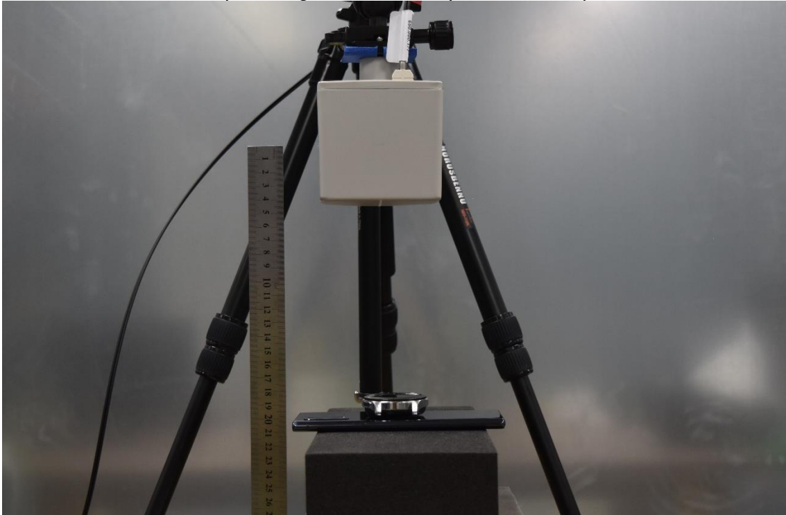
Edge 3 with USB cable (15cm distance)
