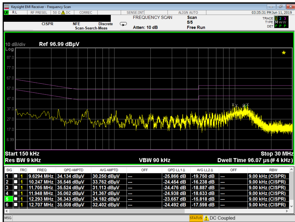
Plot 7-9. Line-Conducted Test Plot with WCP (N)
