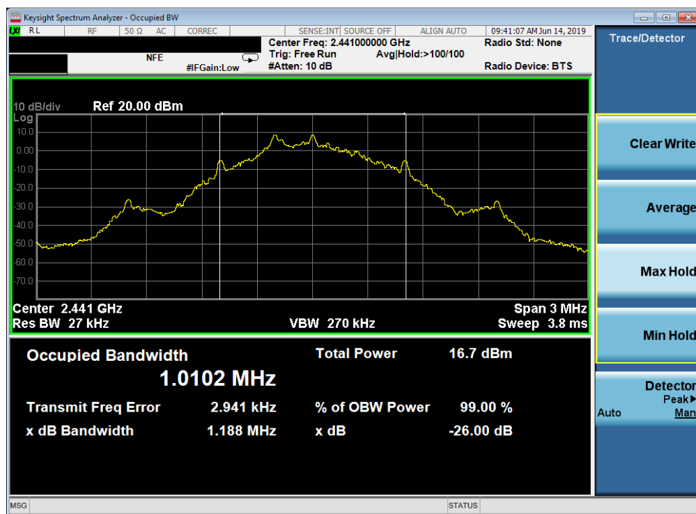
Plot 7-1. Occupied Bandwidth Plot (ANT+ – Ch. 39)
