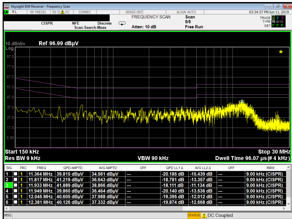
Plot 7-8. Line-Conducted Test Plot with WCP (L1)
