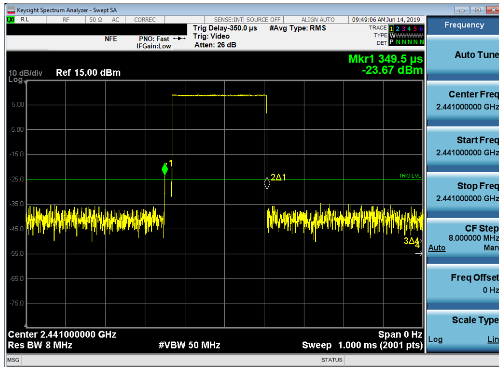
Plot 7-2. Pulse Width Measurement
