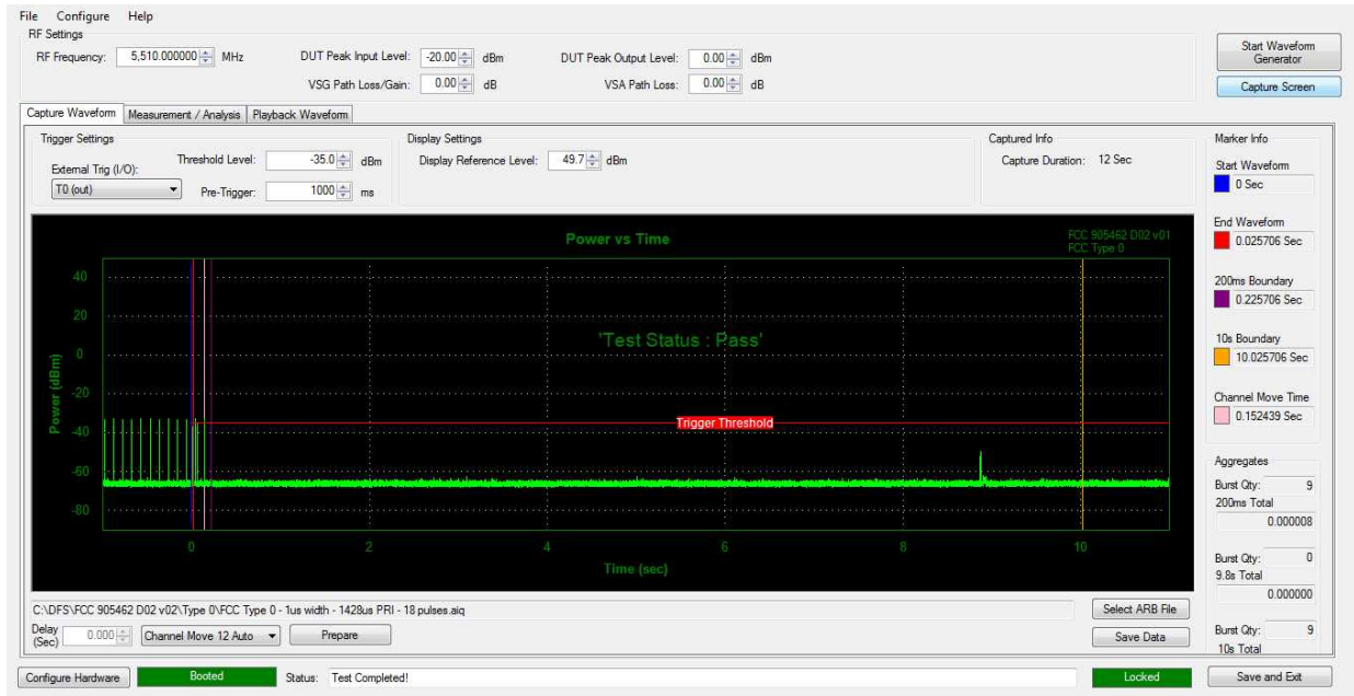
Figure 5-2. Band 2C Move Time and Aggregate Time
