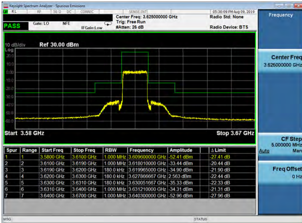
Plot 7-37. Mid Channel Edge Plot (Band 48 - 10.0MHz QPSK - Full RB Configuration)
