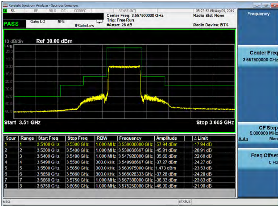
Plot 7-39. Lower Channel Edge Plot (Band 48 - 15.0MHz QPSK - Full RB Configuration)
