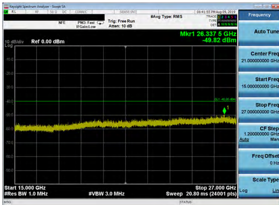
Plot 7-32. Conducted Spurious Plot (Band 48 - 20.0MHz QPSK - RB Size 1, RB Offset 0 - High Channel)
