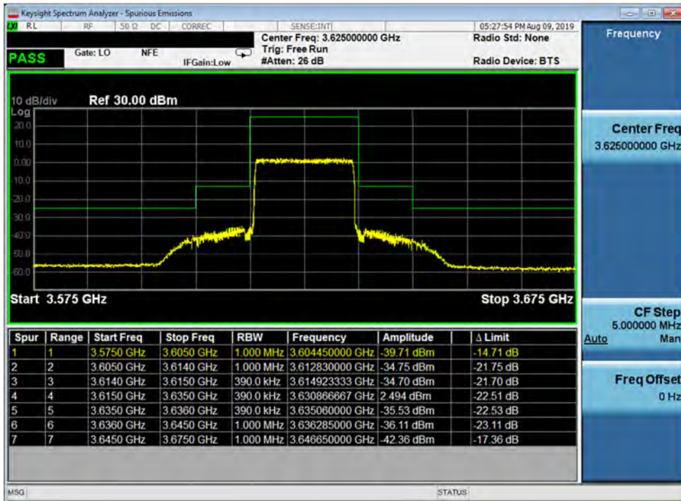
Plot 7-43. Mid Channel Edge Plot (Band 48 - 20.0MHz QPSK - Full RB Configuration)
