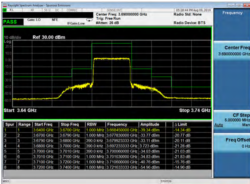
Plot 7-44. Upper Channel Edge Plot (Band 48 - 20.0MHz QPSK - Full RB Configuration)
