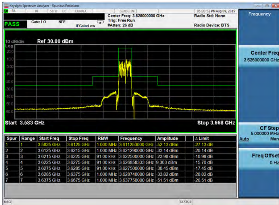
Plot 7-34. Mid Channel Edge Plot (Band 48 - 5.0MHz QPSK - Full RB Configuration)
