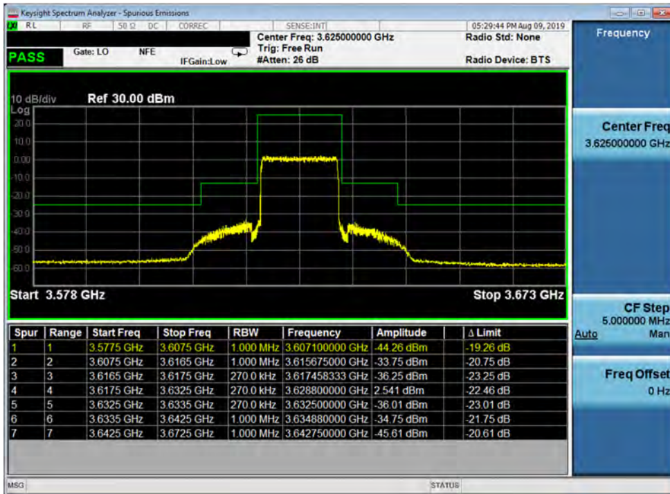
Plot 7-40. Mid Channel Edge Plot (Band 48 - 15.0MHz QPSK - Full RB Configuration)
