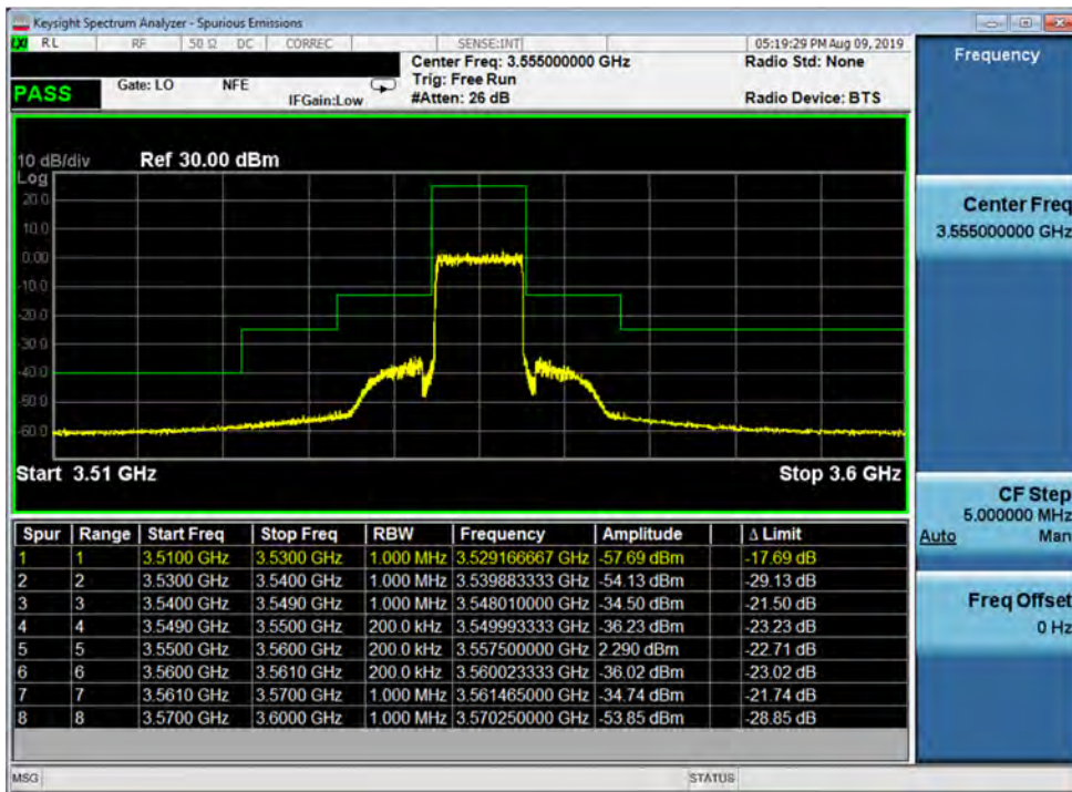
Plot 7-36. Lower Channel Edge Plot (Band 48 - 10.0MHz QPSK - Full RB Configuration)
