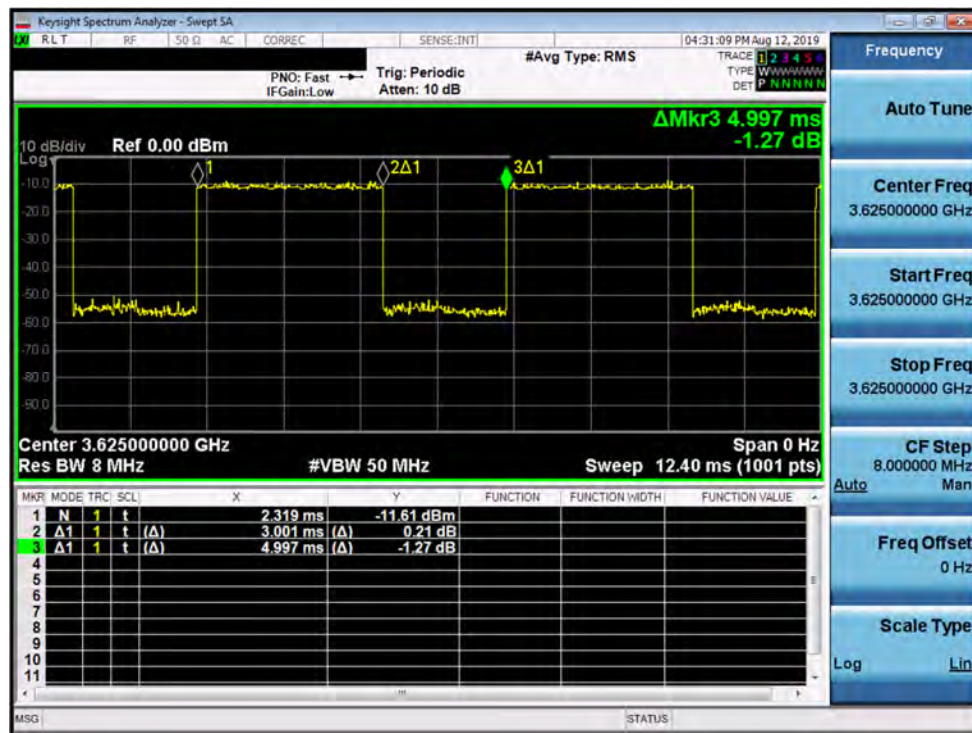
Plot 7-17. Duty Cycle Plot
