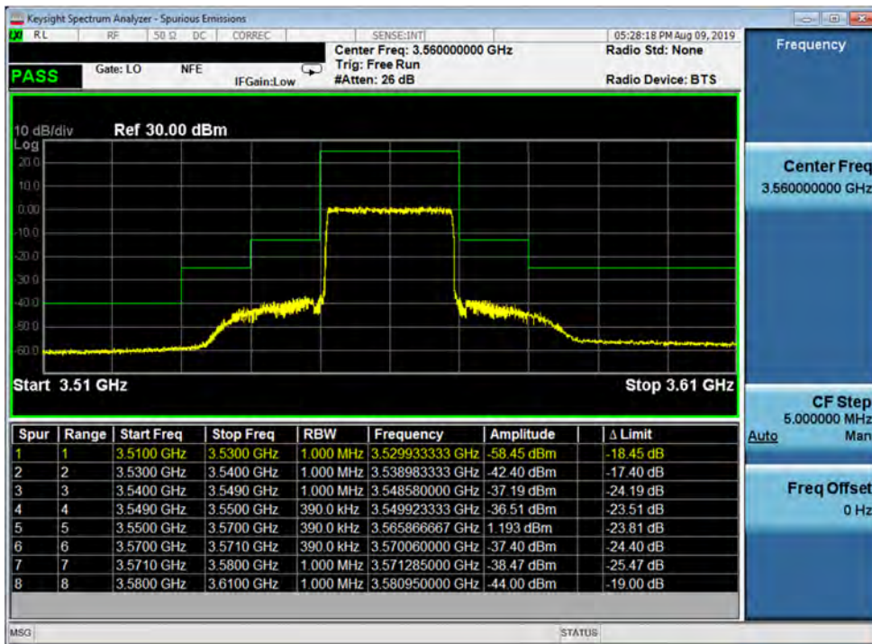
Plot 7-42. Lower Channel Edge Plot (Band 48 - 20.0MHz QPSK - Full RB Configuration)
