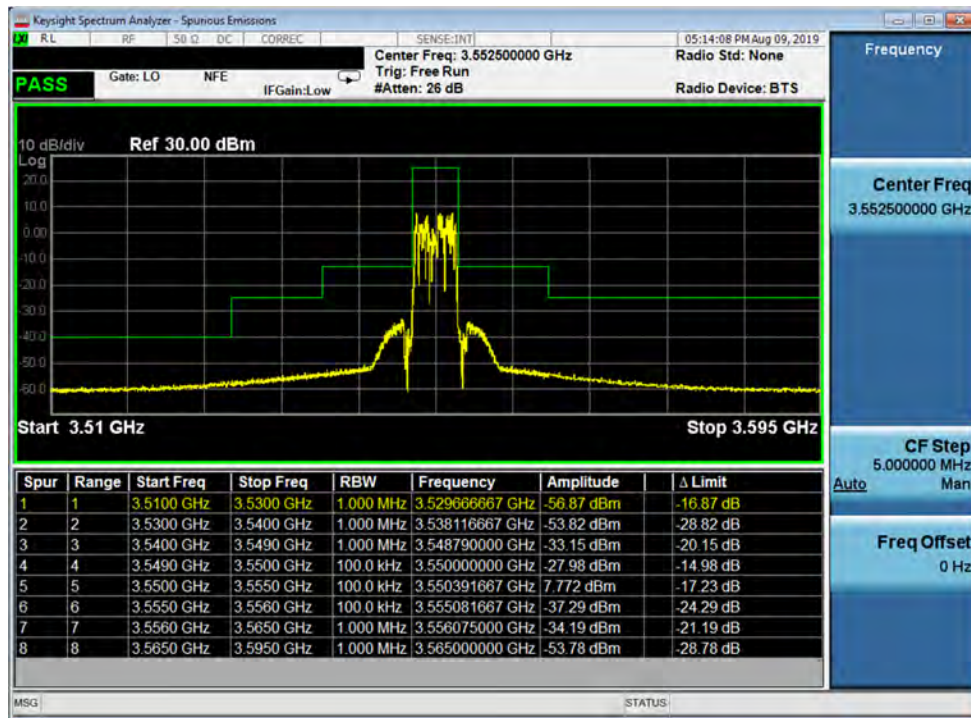
Plot 7-33. Lower Channel Edge Plot (Band 48 - 5.0MHz QPSK - Full RB Configuration)
