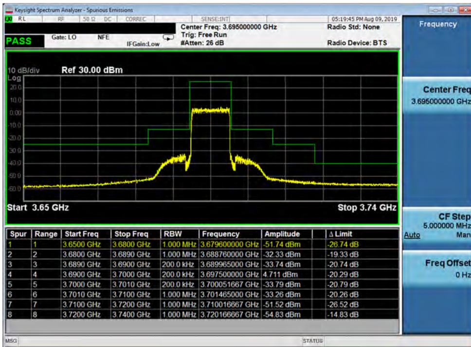
Plot 7-38. Upper Channel Edge Plot (Band 48 - 10.0MHz QPSK - Full RB Configuration)
