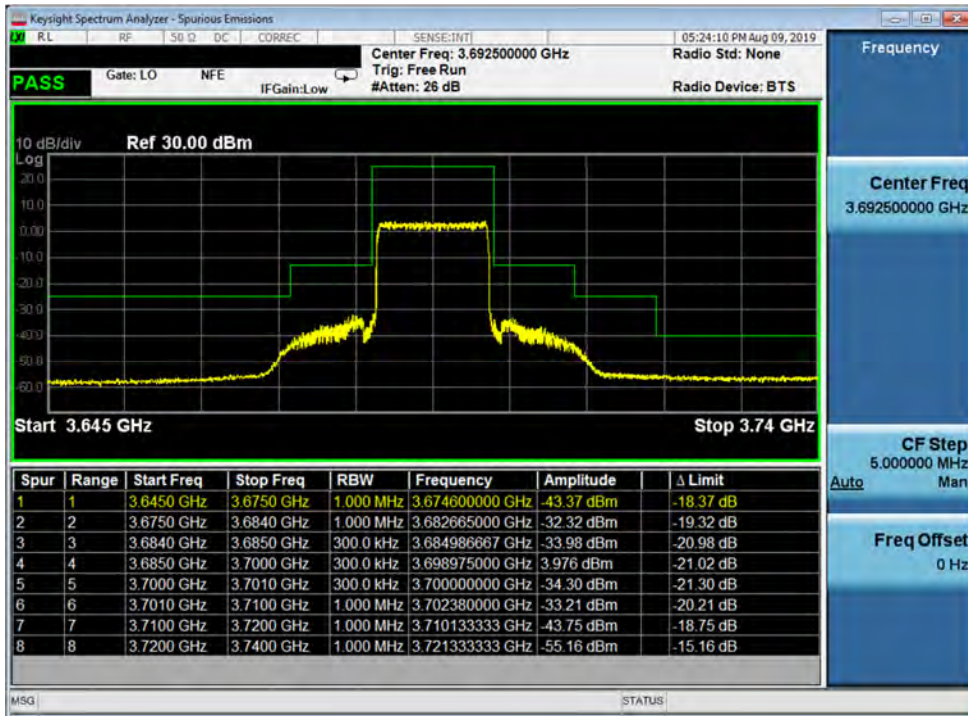
Plot 7-41. Upper Channel Edge Plot (Band 48 - 15.0MHz QPSK - Full RB Configuration)
