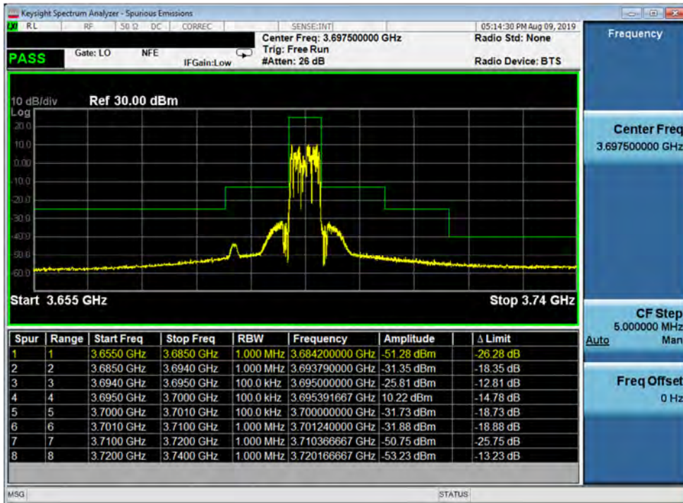
Plot 7-35. Upper Channel Edge Plot (Band 48 - 5.0MHz QPSK - Full RB Configuration)
