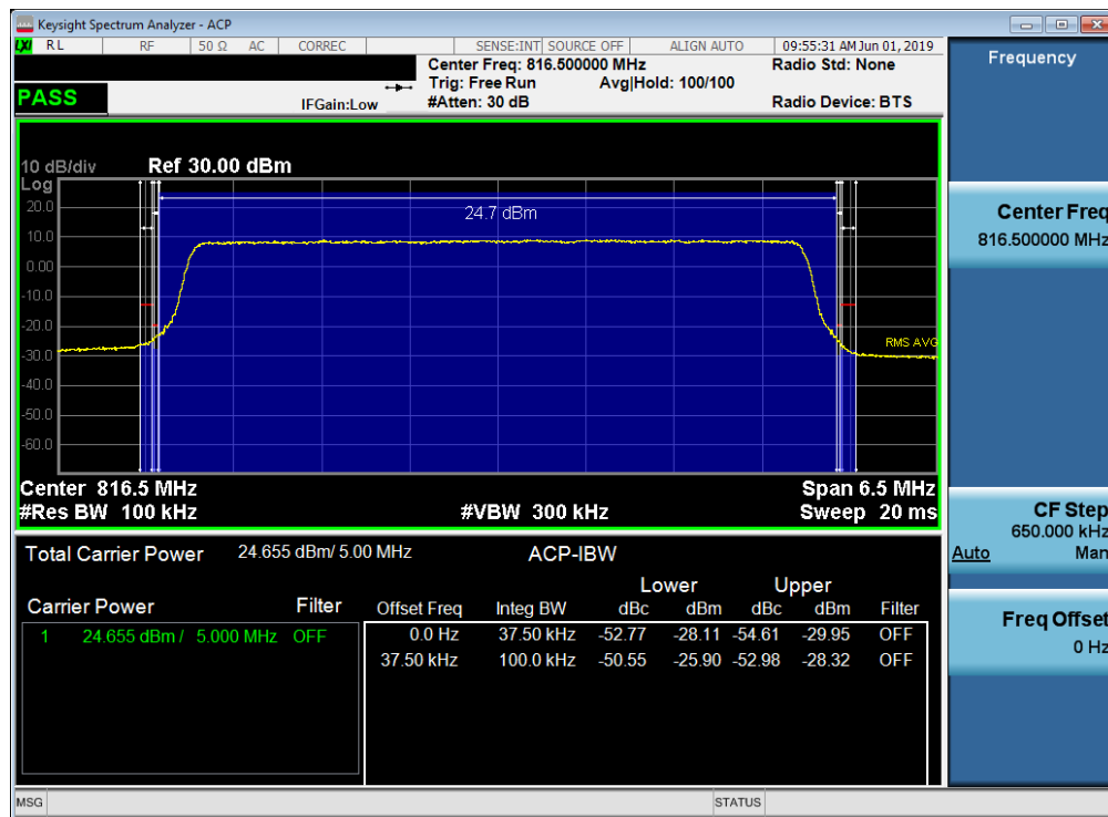
Plot 7-49. Channel Edge Plot (LTE Band 26, 5MHz QPSK – RB Size 25– Low Channel)
