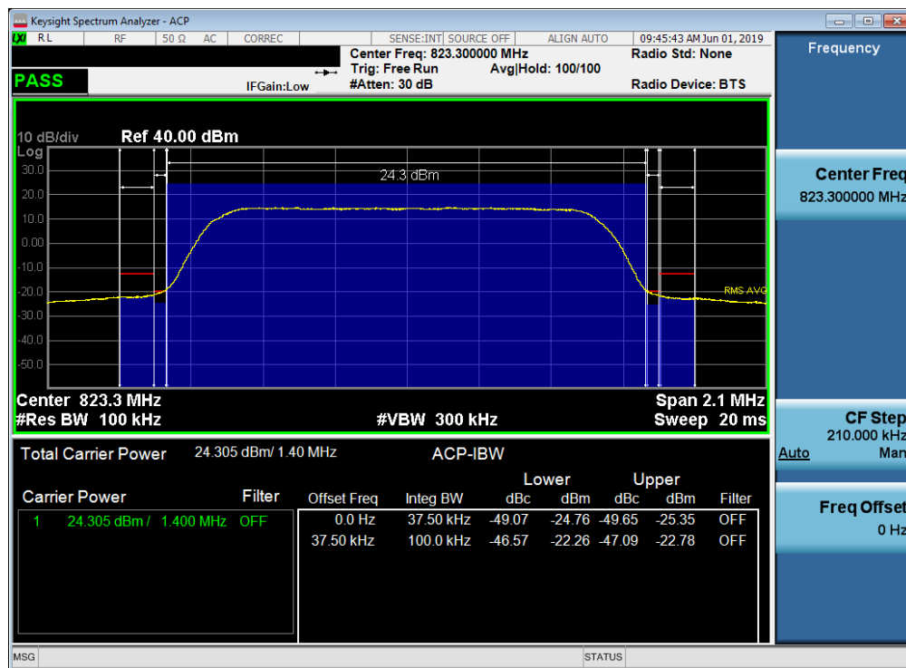
Plot 7-46. Channel Edge Plot (LTE Band 26, 1.4MHz QPSK – RB Size 6 – High Channel)
