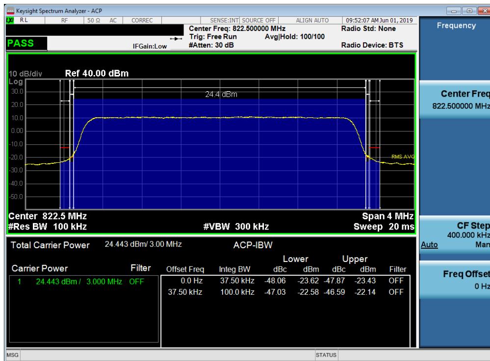
Plot 7-48. Channel Edge Plot (LTE Band 26, 3MHz QPSK – RB Size 15 – High Channel)
