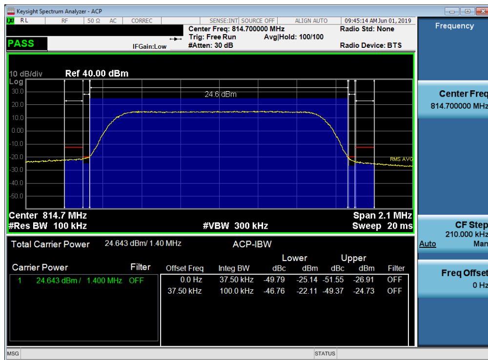
Plot 7-45. Channel Edge Plot (LTE Band 26, 1.4MHz QPSK – RB Size 6– Low Channel)
