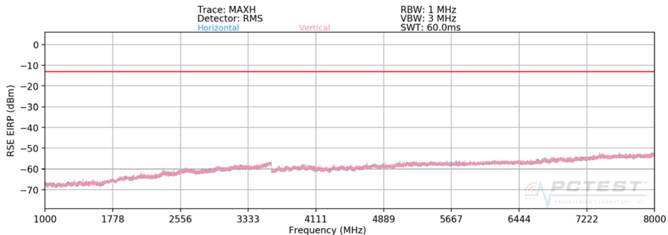
Plot 7-65. Radiated Spurious Plot above 1GHz (LTE Band 14)
