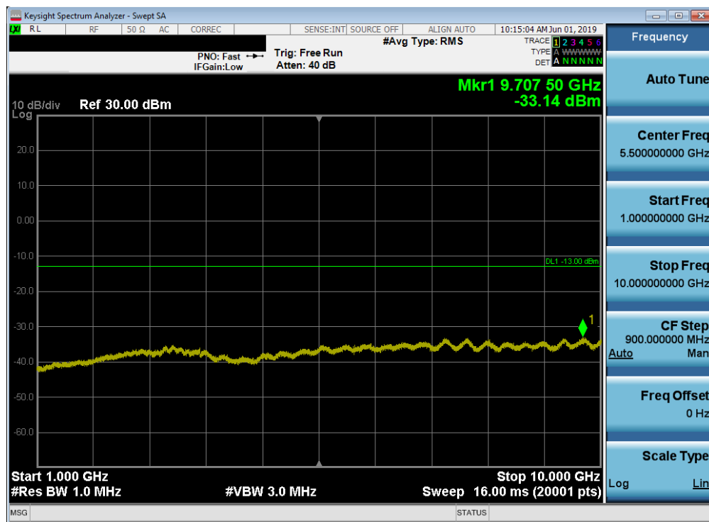
Plot 7-39. Conducted Spurious Plot (LTE Band 26, 15MHz QPSK – RB Size 1, RB Offset 0 – Mid Channel)
