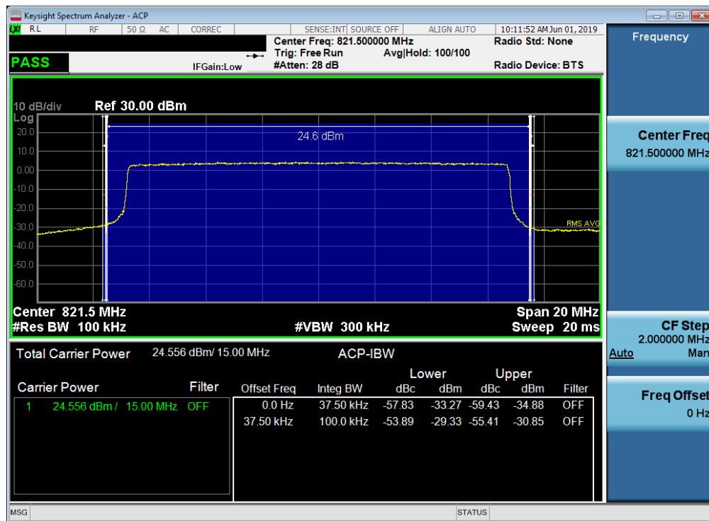
Plot 7-52. Channel Edge Plot (LTE Band 26, 15MHz QPSK – RB Size 75)
