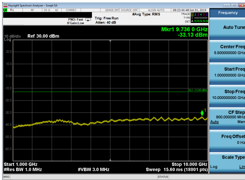
Plot 7-42. Conducted Spurious Plot (LTE Band 14, 10MHz QPSK – RB Size 1, RB Offset 0 – Mid Channel)
