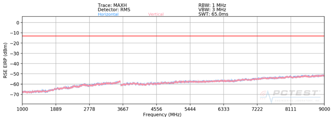
Plot 7-63. Radiated Spurious Plot above 1GHz (CDMA BC10)
