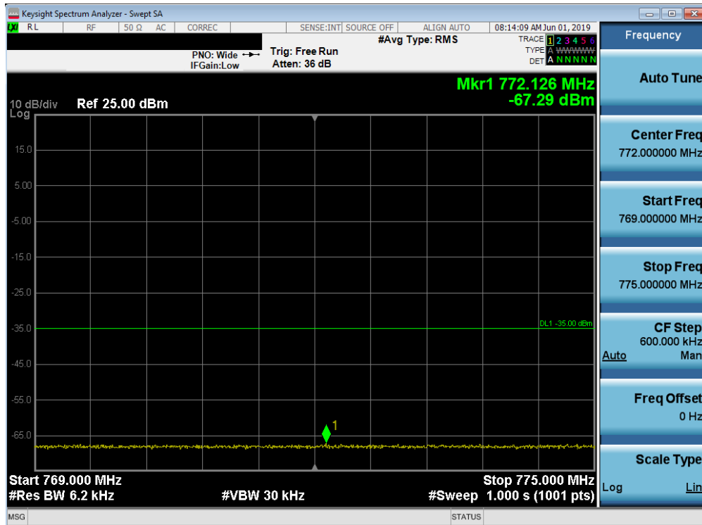
Plot 7-58. Lower Emission Mask Plot (LTE Band 14, 10MHz QPSK – RB Size 50)
