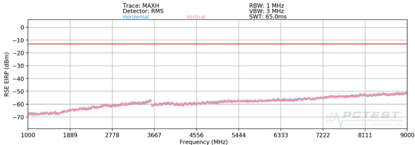
Plot 7-64. Radiated Spurious Plot above 1GHz (LTE Band 26)
