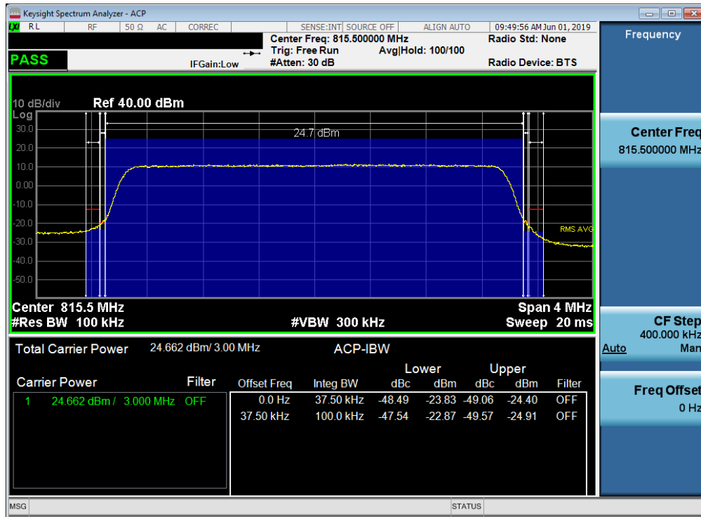
Plot 7-47. Channel Edge Plot (LTE Band 26, 3MHz QPSK – RB Size 15– Low Channel)
