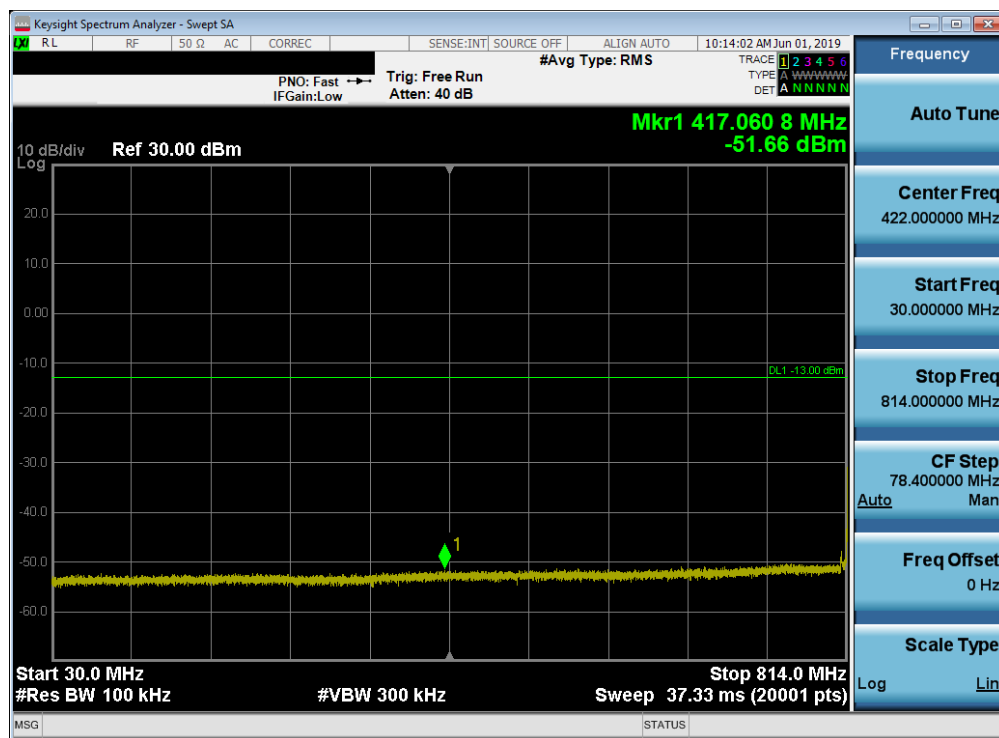
Plot 7-37. Conducted Spurious Plot (LTE Band 26, 15MHz QPSK – RB Size 1, RB Offset 0 – Mid Channel)
