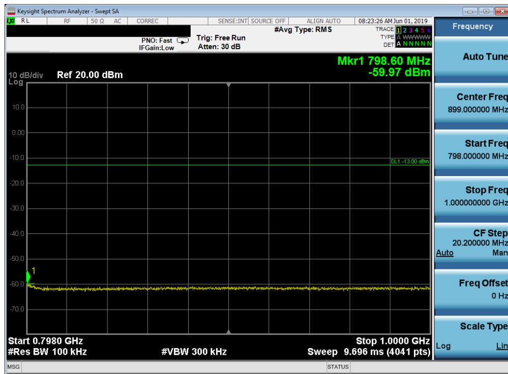
Plot 7-41. Conducted Spurious Plot (LTE Band 14, 10MHz QPSK – RB Size 1, RB Offset 0 – Mid Channel)
