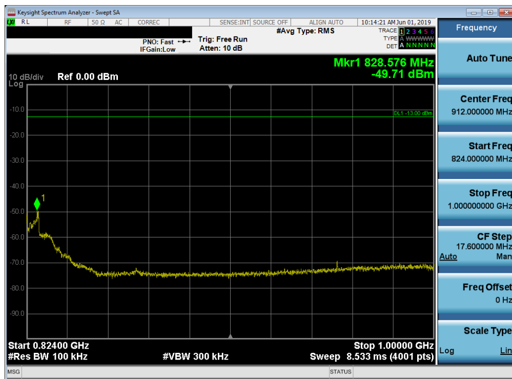
Plot 7-38. Conducted Spurious Plot (LTE Band 26, 15MHz QPSK – RB Size 1, RB Offset 0 – Mid Channel)
