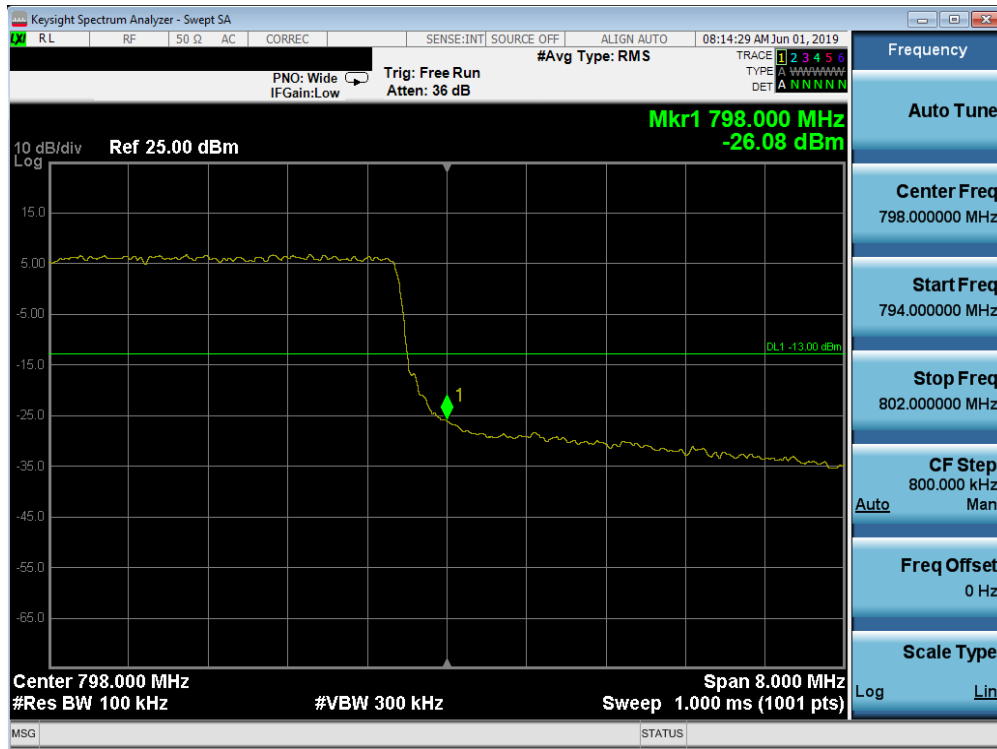
Plot 7-59. Upper Band Edge Plot (LTE Band 14, 10MHz QPSK – RB Size 50)
