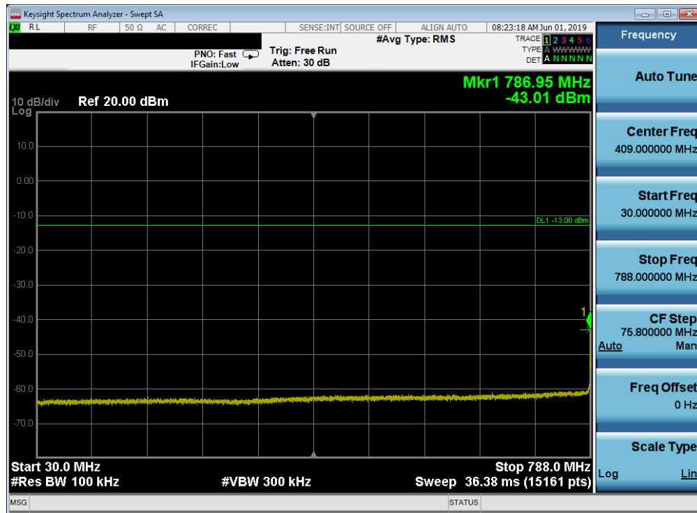
Plot 7-40. Conducted Spurious Plot (LTE Band 14, 10MHz QPSK – RB Size 1, RB Offset 0 – Mid Channel)
