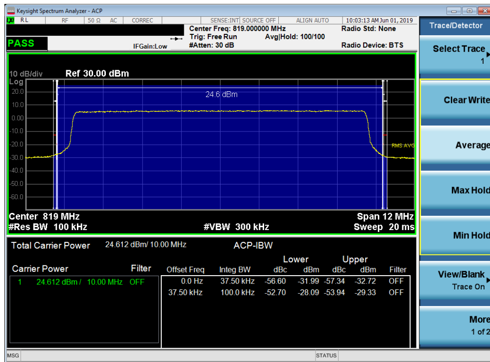
Plot 7-51. Channel Edge Plot (LTE Band 26, 10MHz QPSK – RB Size 50)
