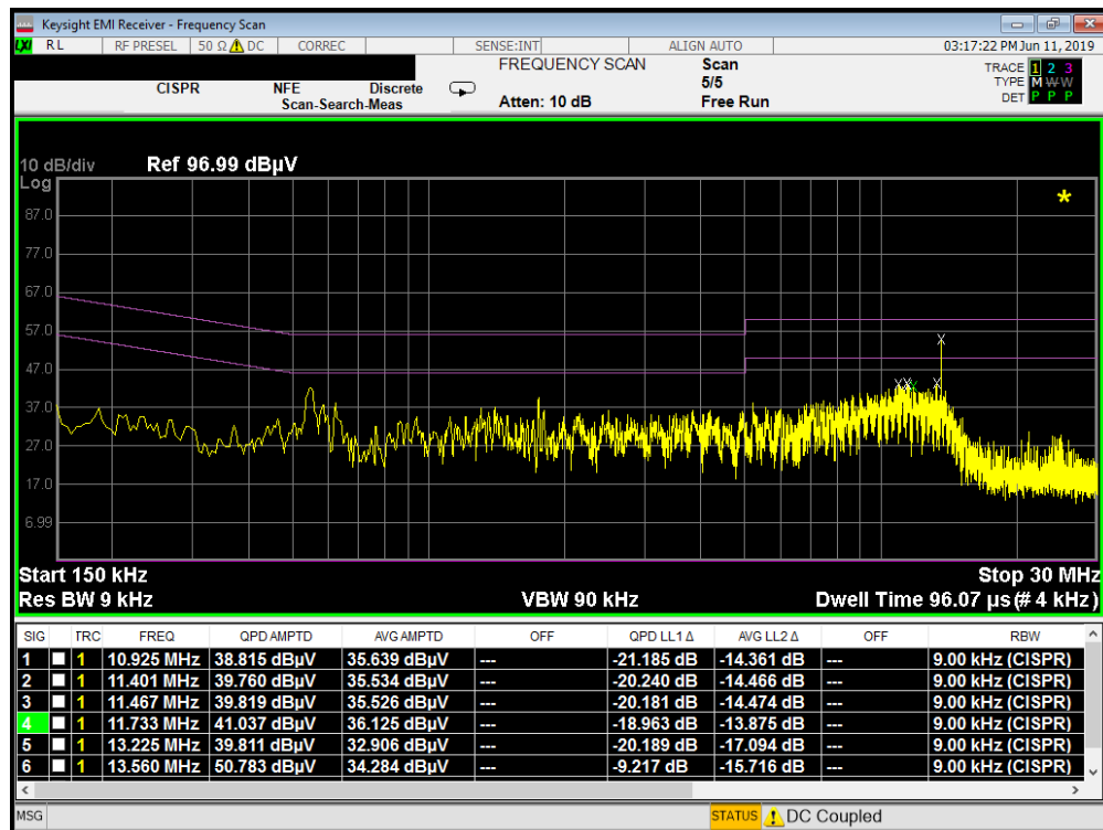
Plot 7-51. Line-Conducted Test Plot with WCP (L1)
