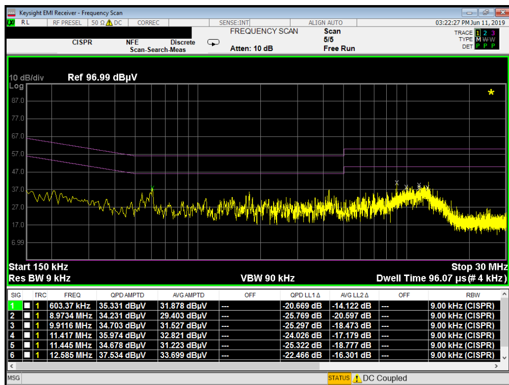
Plot 7-52. Line-Conducted Test Plot with WCP (N)
