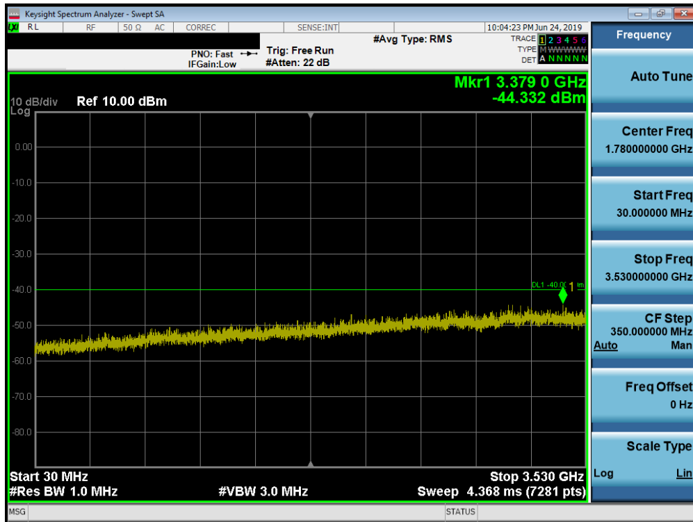
Plot 7-28. Conducted Spurious Plot (Band 48 - 20.0MHz QPSK - RB Size 1, RB Offset 99 - High Channel)
