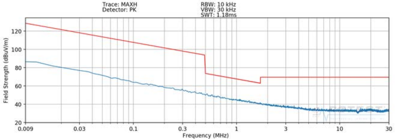
Plot 7-10. Radiated Spurious Plot 9kHz – 30MHz (Pol. X – Digitizer Mode 2)
