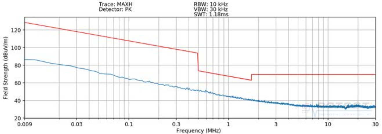
Plot 7-7. Radiated Spurious Plot 9kHz – 30MHz (Pol. X – Digitizer Mode 1)
