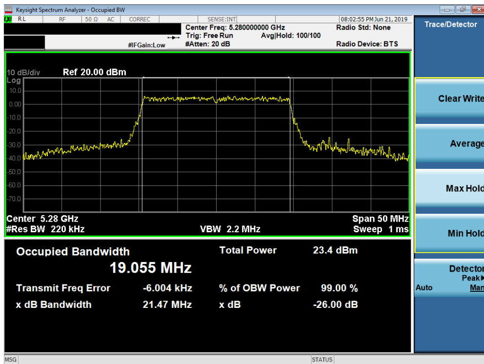
Plot 7-68. 26dB Bandwidth Plot SISO ANT2 (20MHz BW 802.11ac (UNII Band 1) – Ch. 56)
