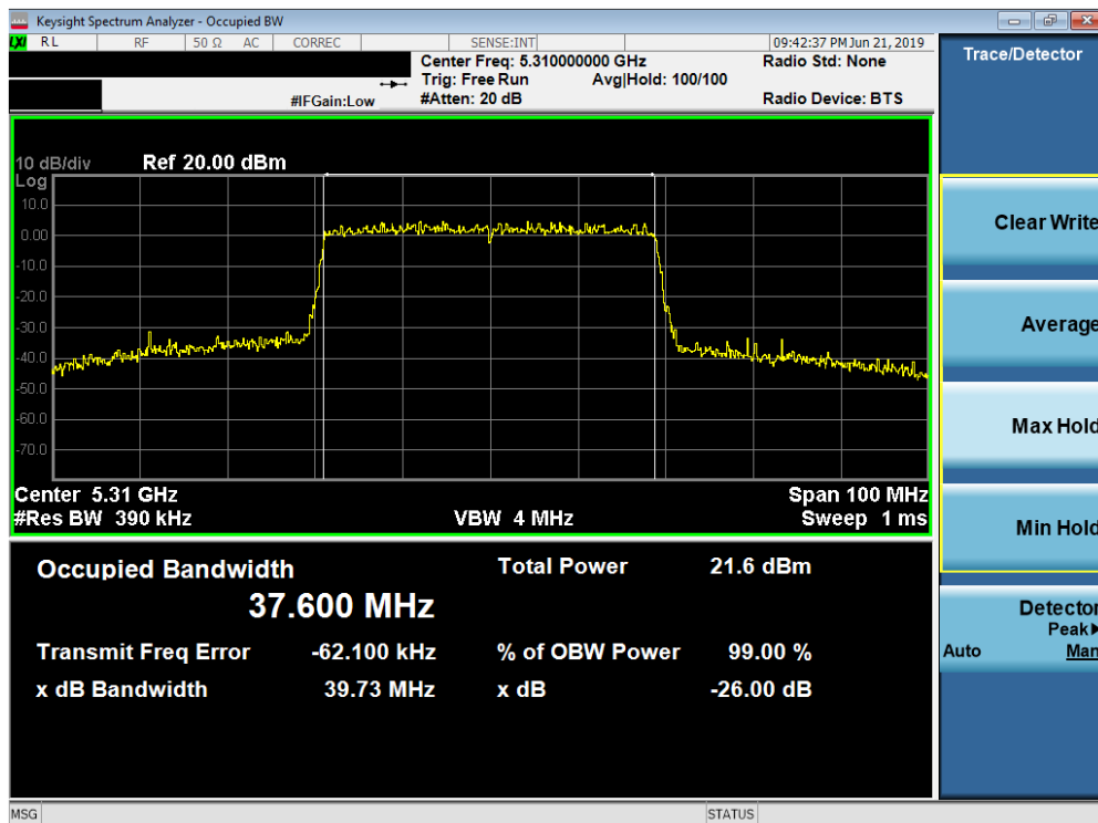
Plot 7-73. 26dB Bandwidth Plot SISO ANT2 (40MHz BW 802.11ax (UNII Band 1) – Ch. 62)
