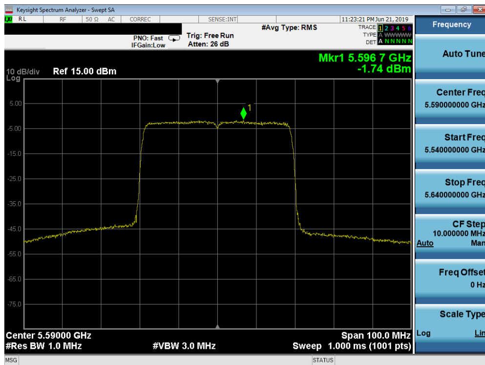
Plot 7-170. Power Spectral Density Plot SISO ANT1 (40MHz BW 802.11n (UNII Band 2C) – Ch. 118)
