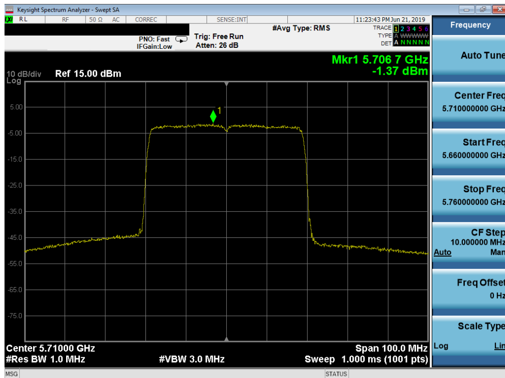
Plot 7-171. Power Spectral Density Plot SISO ANT1 (40MHz BW 802.11n (UNII Band 2C) – Ch. 142)
