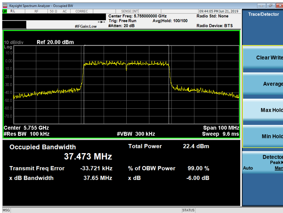
Plot 7-123. 6dB Bandwidth Plot SISO ANT2 (40MHz BW 802.11ax (UNII Band 3) – Ch. 151)
