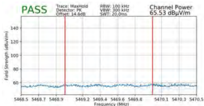
Plot 7-313. Radiated Lower Band Edge Plot SISO ANT2 (Peak – UNII Band 2C)
