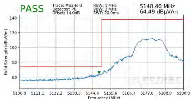
Plot 7-330. Radiated Lower Band Edge Plot MIMO (Peak – UNII Band 1)
