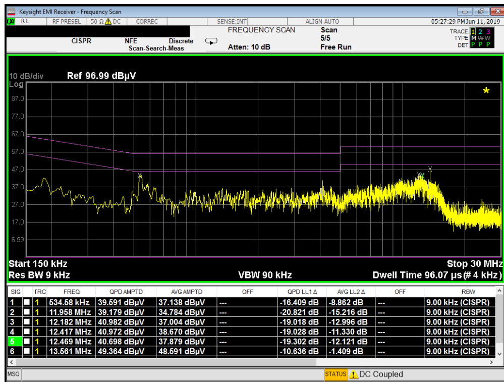
Plot 7-375. Line Conducted Plot with 802.11a UNII Band 3 with WCP (L1)
