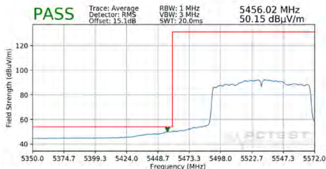
Plot 7-351. Radiated Lower Band Edge Plot MIMO (Average – UNII Band 2C)
