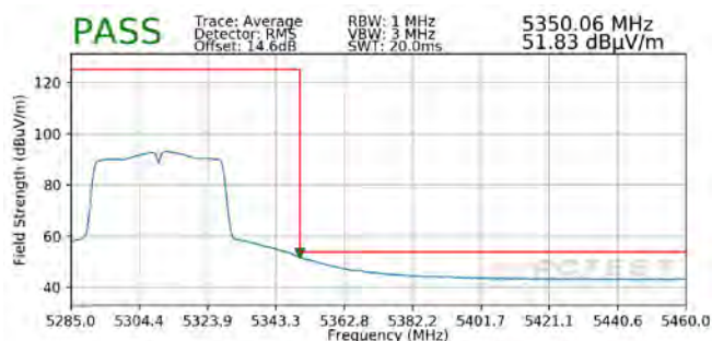
Plot 7-310. Radiated Upper Band Edge Plot SISO ANT2 (Average – UNII Band 2A)
