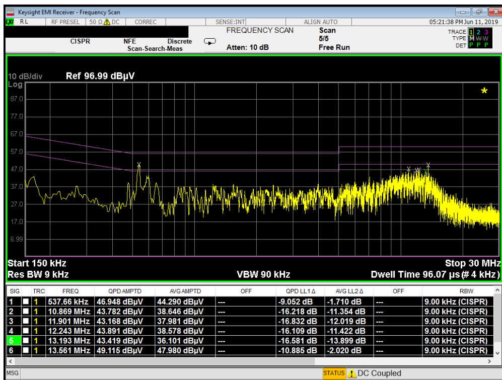
Plot 7-369. Line Conducted Plot with 802.11a UNII Band 2C (L1)
