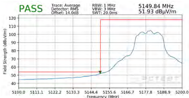
Plot 7-322. Radiated Lower Band Edge Plot MIMO (Average – UNII Band 1)
