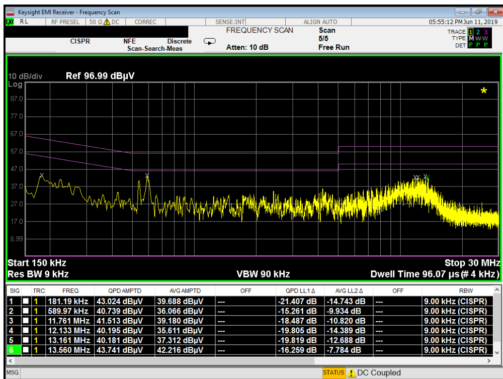
Plot 7-374. Line Conducted Plot with 802.11a UNII Band 3 (N)
