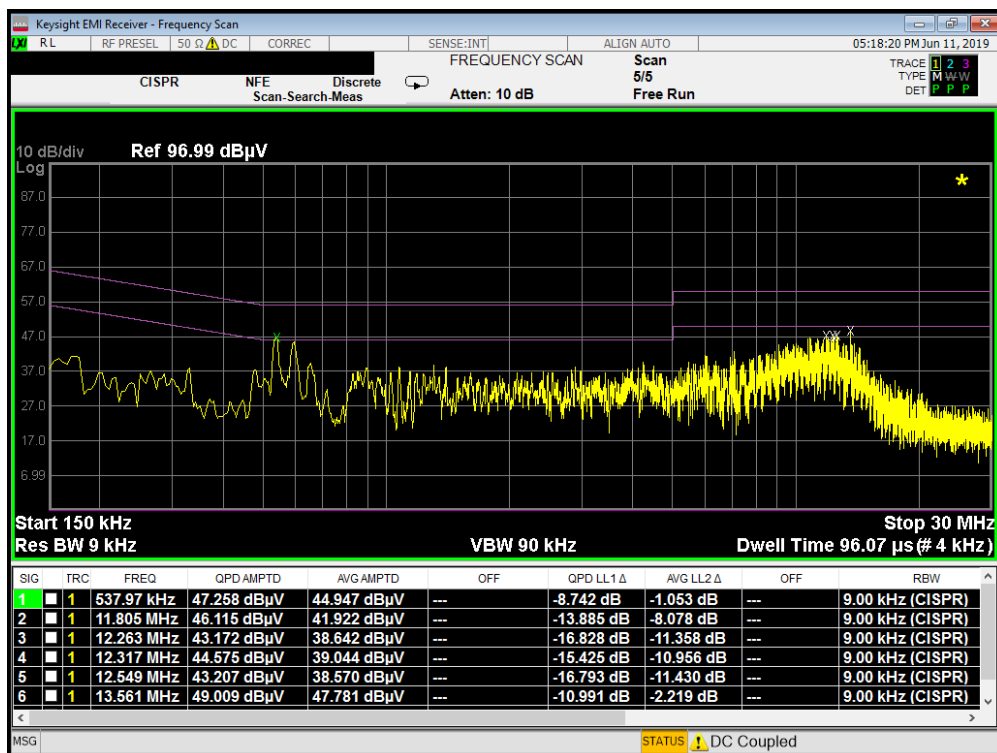
Plot 7-365. Line Conducted Plot with 802.11a UNII Band 2A (L1)
