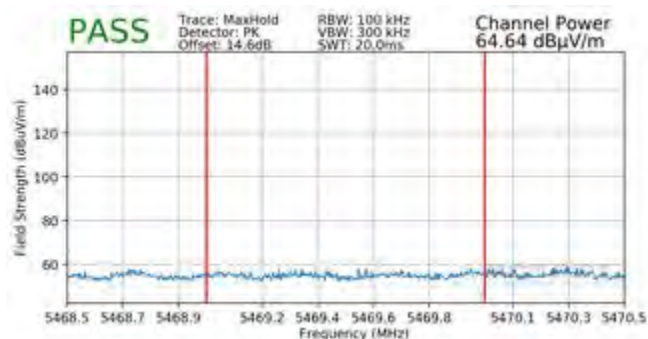
Plot 7-292. Radiated Lower Band Edge Plot SISO ANT1 (Peak – UNII Band 2C)
