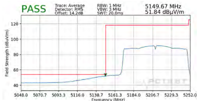
Plot 7-294. Radiated Lower Band Edge Plot SISO ANT1 (Average - UNII Band 1)
