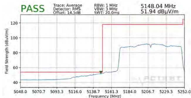
Plot 7-347. Radiated Lower Band Edge Plot MIMO (Average – UNII Band 1)
