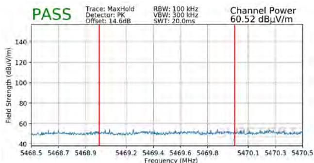
Plot 7-334. Radiated Lower Band Edge Plot MIMO (Peak – UNII Band 2C)
