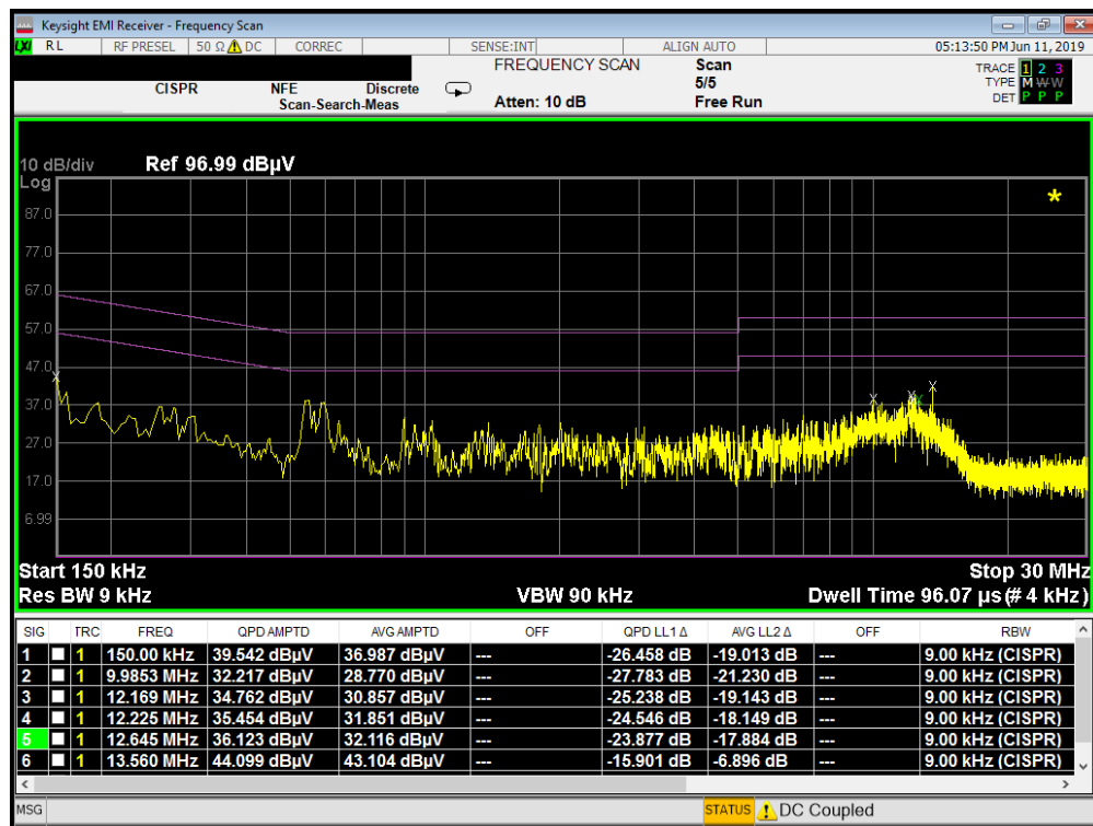
Plot 7-364. Line Conducted Plot with 802.11a UNII Band 1 with WCP (N)
