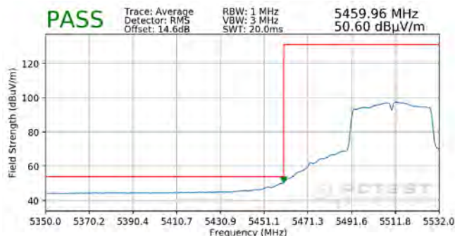
Plot 7-342. Radiated Lower Band Edge Plot MIMO (Average – UNII Band 2C)
