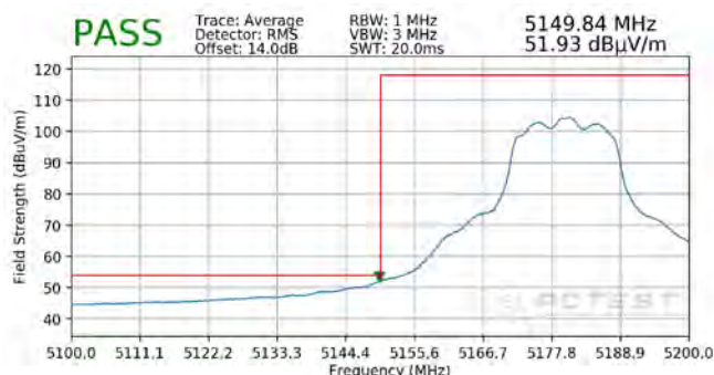
Plot 7-329. Radiated Lower Band Edge Plot MIMO (Average – UNII Band 1)
