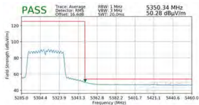
Plot 7-345. Radiated Band Edge Plot MIMO (Average – WCP)
