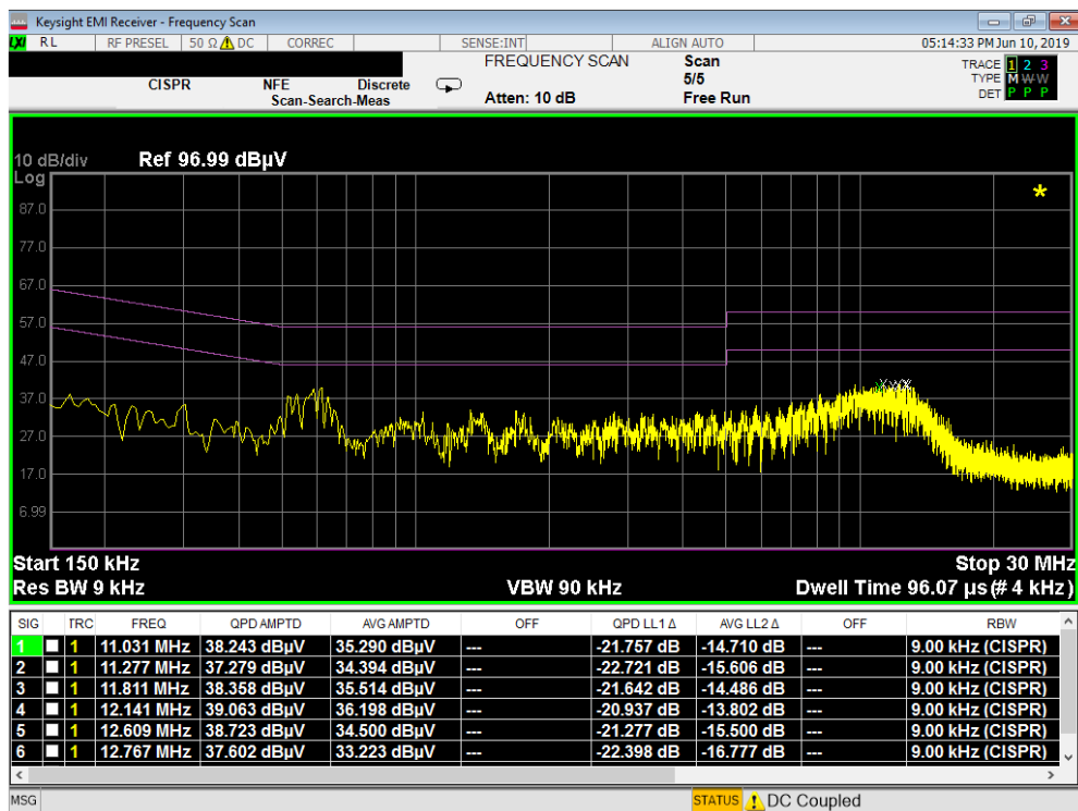
Plot 7-373. Line Conducted Plot with 802.11a UNII Band 3 (L1)
