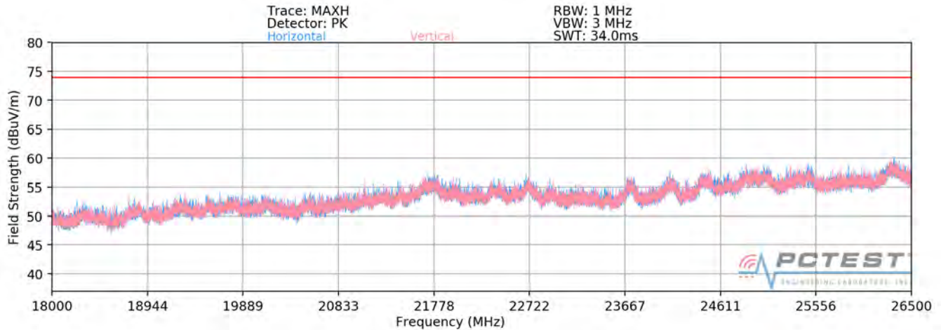
Plot 7-275. Radiated Spurious Plot 18GHz – 26.5GHz (5GHz – 2.4 GHz)
