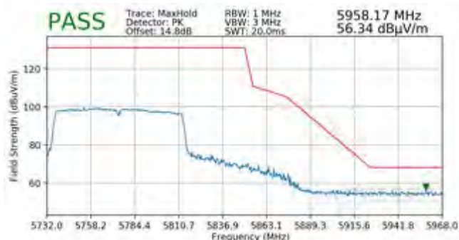
Plot 7-321. Radiated Upper Band Edge Plot SISO ANT2 (Peak – UNII Band 3)
