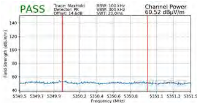
Plot 7-311. Radiated Upper Band Edge Plot SISO ANT2 (Peak – UNII Band 2A)
