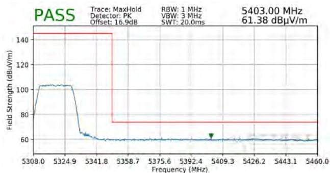
Plot 7-337. Radiated Band Edge Plot MIMO (Peak - WCP)
