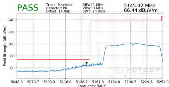
Plot 7-295. Radiated Lower Band Edge Plot SISO ANT1 (Peak - UNII Band 1)
