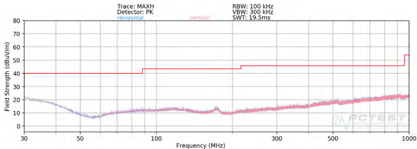
Plot 7-356. Radiated Spurious Plot below 1GHz SISO ANT1 (802.11a – U2A Ch. 56)
