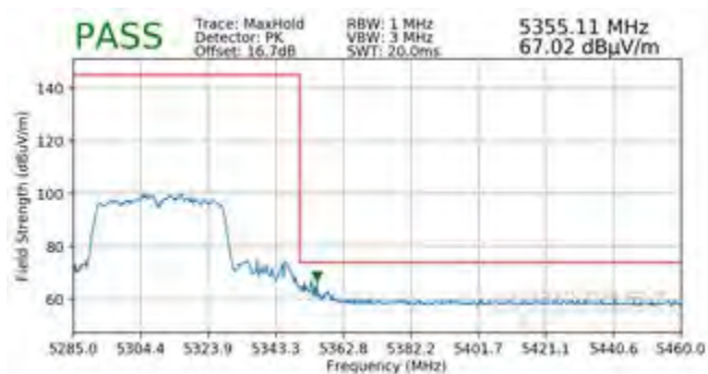
Plot 7-346. Radiated Band Edge Plot MIMO (Peak – WCP)
