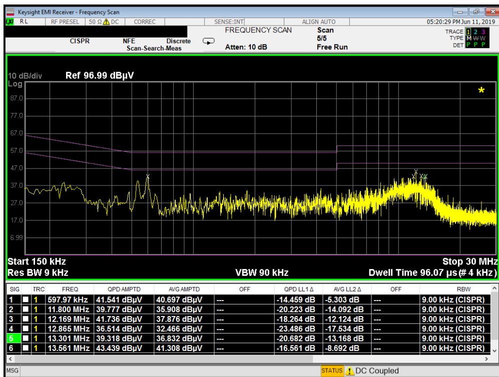
Plot 7-370. Line Conducted Plot with 802.11a UNII Band 2C (N)
