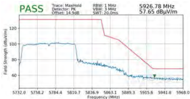
Plot 7-300. Radiated Upper Band Edge Plot SISO ANT1 (Peak – UNII Band 3)
