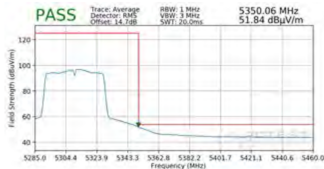
Plot 7-289. Radiated Upper Band Edge Plot SISO ANT1 (Average - UNII Band 2A)
