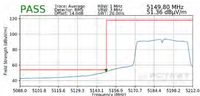
Plot 7-308. Radiated Lower Band Edge Plot SISO ANT2 (Average – UNII Band 1)
