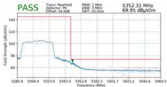
Plot 7-290. Radiated Upper Band Edge Plot SISO ANT1 (Peak - UNII Band 2A)
