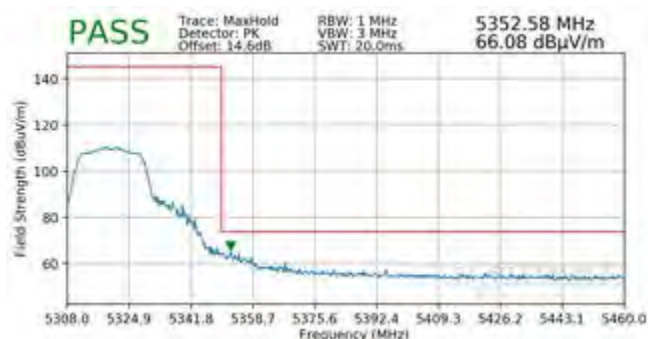
Plot 7-283. Radiated Upper Band Edge Plot SISO ANT1 (Peak – UNII Band 2A)
