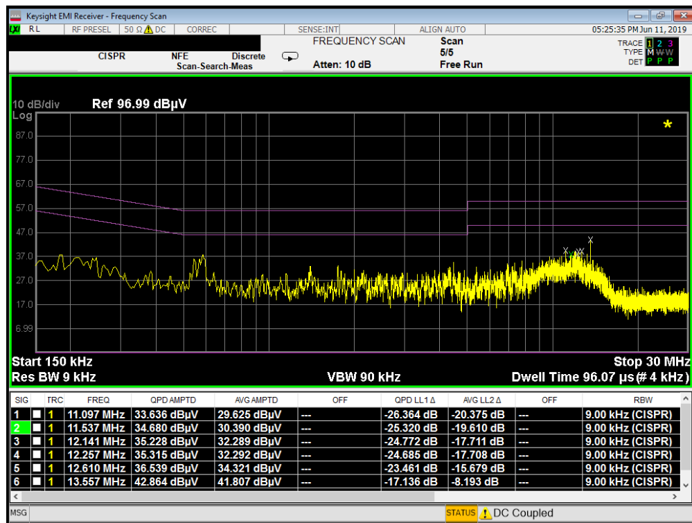
Plot 7-376. Line Conducted Plot with 802.11a UNII Band 3 with WCP (N)
