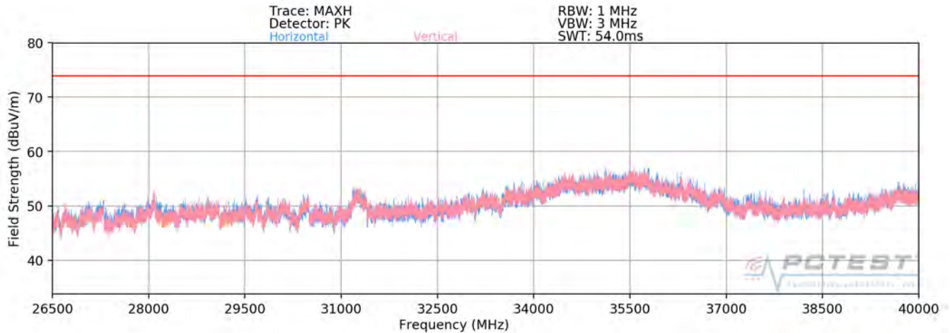
Plot 7-273. Radiated Spurious Plot above 26.5GHz (2.4GHz – 5GHz)
