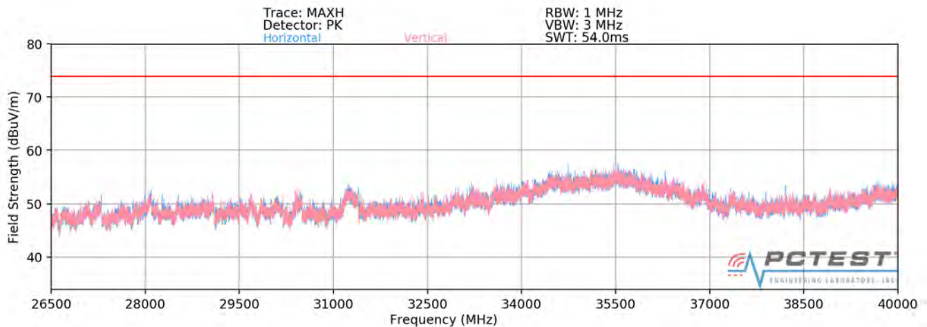
Plot 7-279. Radiated Spurious Plot above 26.5GHz (Dual Band Simult. Tx)
