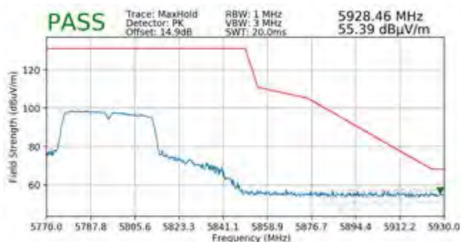
Plot 7-314. Radiated Upper Band Edge Plot SISO ANT2 (Peak – UNII Band 3)
