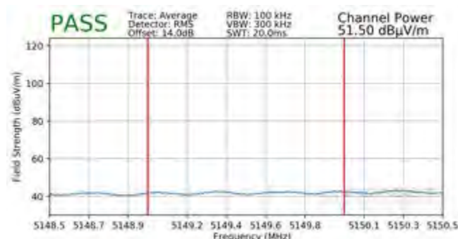
Plot 7-280. Radiated Lower Band Edge Plot SISO ANT1 (Average – UNII Band 1)
