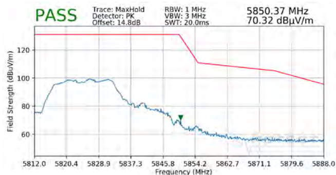
Plot 7-328. Radiated Upper Band Edge Plot MIMO (Peak – UNII Band 3)
