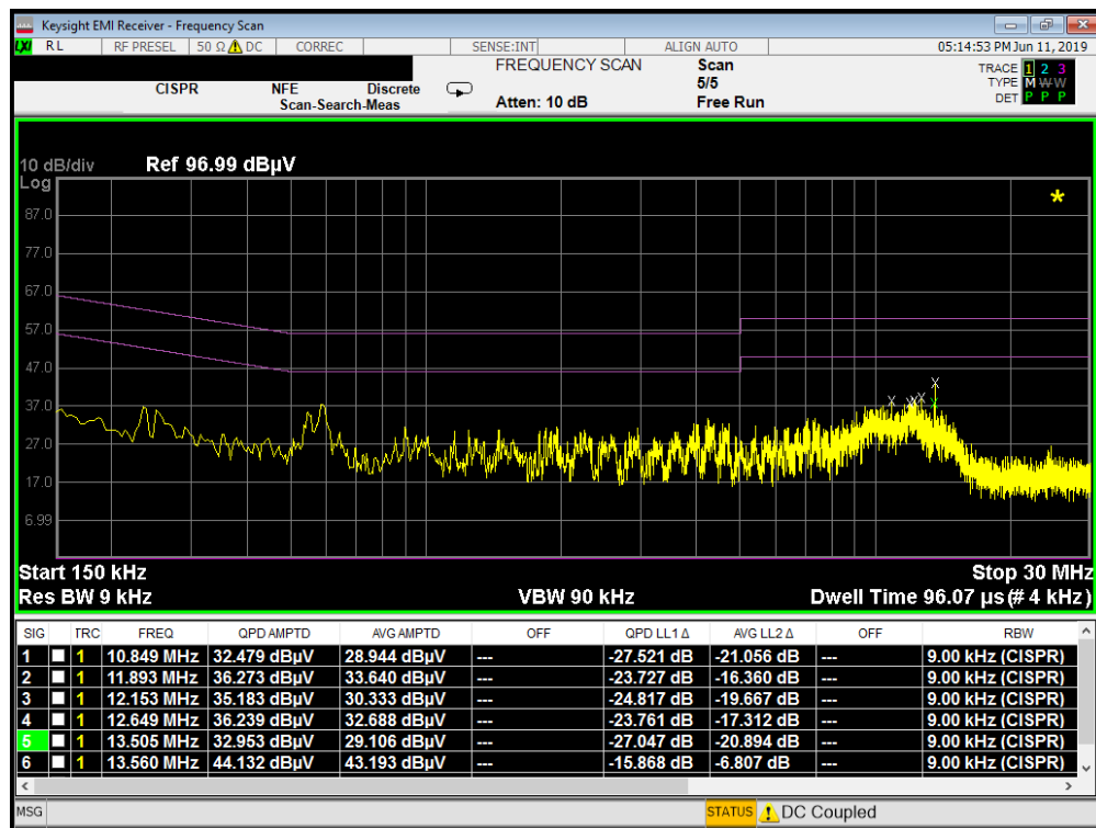
Plot 7-368. Line Conducted Plot with 802.11a UNII Band 2A with WCP (N)
