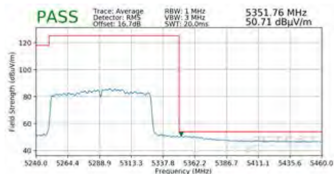
Plot 7-354. Radiated Band Edge Plot MIMO (Average - WCP)
