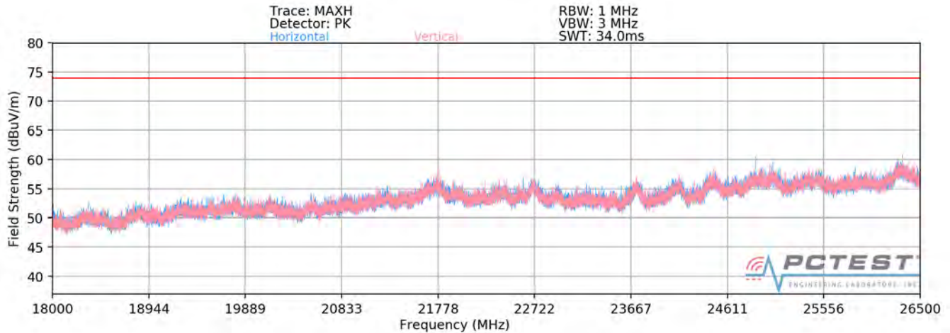
Plot 7-278. Radiated Spurious Plot 18GHz – 26.5GHz (Dual Band Simult. Tx)
