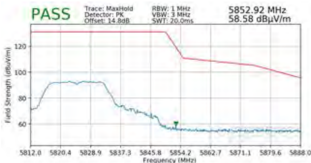
Plot 7-286. Radiated Upper Band Edge Plot SISO ANT1 (Peak - UNII Band 3)
