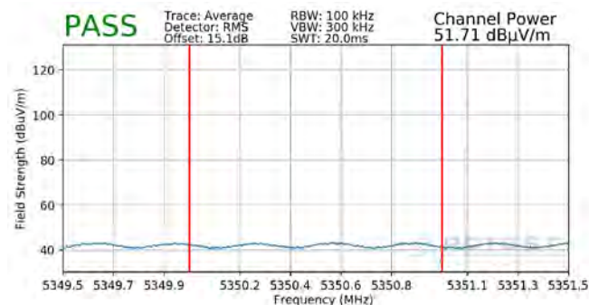
Plot 7-349. Radiated Upper Band Edge Plot MIMO (Average – UNII Band 2A)
