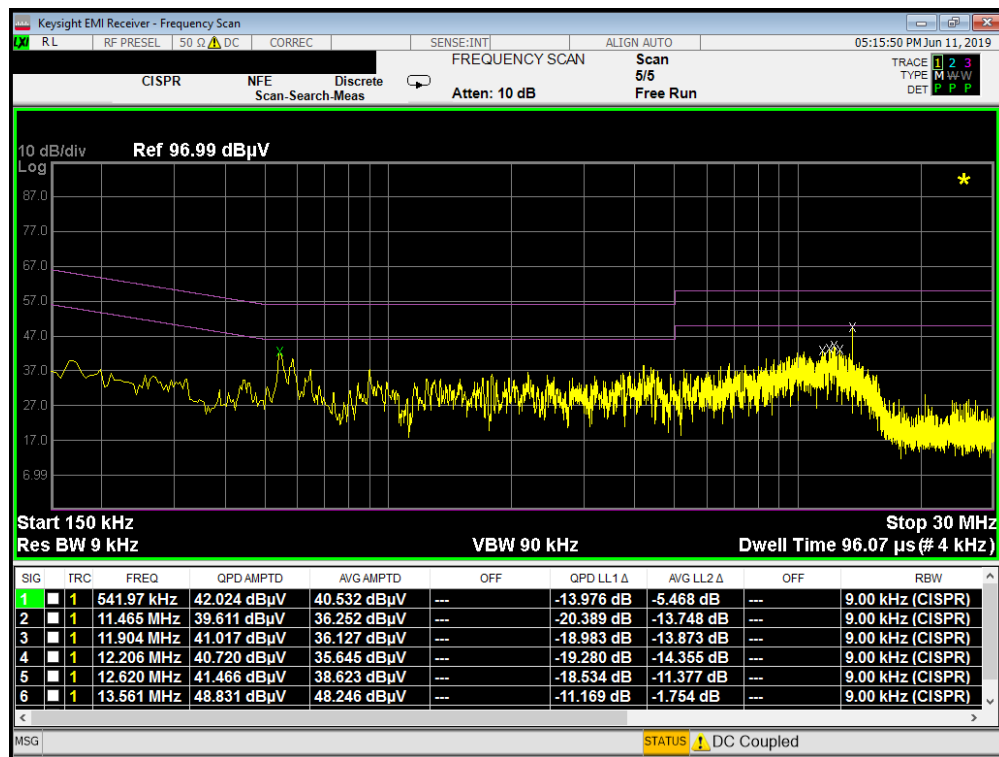
Plot 7-367. Line Conducted Plot with 802.11a UNII Band 2A with WCP (L1)
