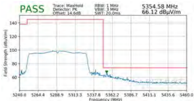
Plot 7-297. Radiated Upper Band Edge Plot SISO ANT1 (Peak - UNII Band 2A)
