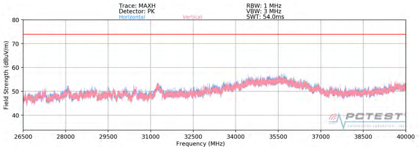
Plot 7-276. Radiated Spurious Plot above 26.5GHz (5GHz – 2.4 GHz)
