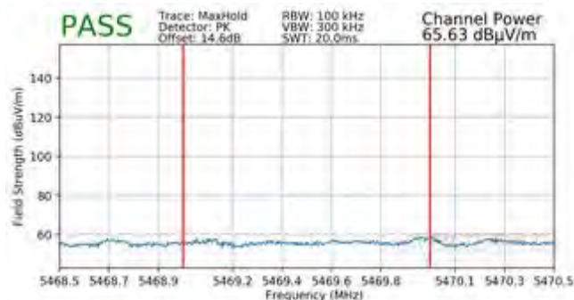
Plot 7-285. Radiated Lower Band Edge Plot SISO ANT1 (Peak - UNII Band 2C)
