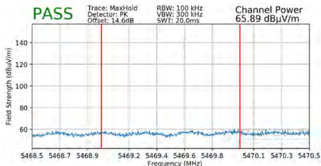
Plot 7-343. Radiated Lower Band Edge Plot MIMO (Peak – UNII Band 2C)
