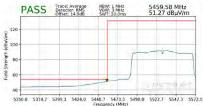
Plot 7-298. Radiated Lower Band Edge Plot SISO ANT1 (Average – UNII Band 2C)
