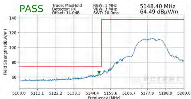
Plot 7-323. Radiated Lower Band Edge Plot MIMO (Peak – UNII Band 1)
