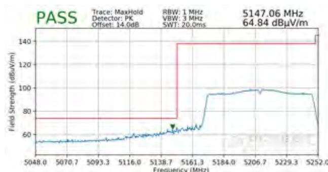
Plot 7-316. Radiated Lower Band Edge Plot SISO ANT2 (Peak – UNII Band 1)
