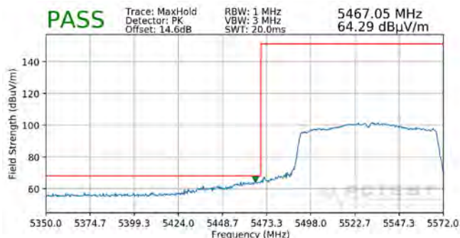
Plot 7-352. Radiated Lower Band Edge Plot MIMO (Peak – UNII Band 2C)
