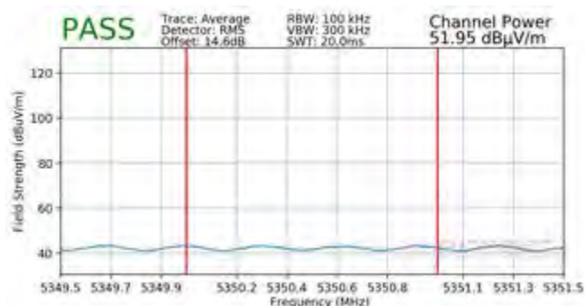
Plot 7-317. Radiated Upper Band Edge Plot SISO ANT2 (Average – UNII Band 2A)
