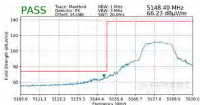
Plot 7-281. Radiated Lower Band Edge Plot SISO ANT1 (Peak – UNII Band 1)
