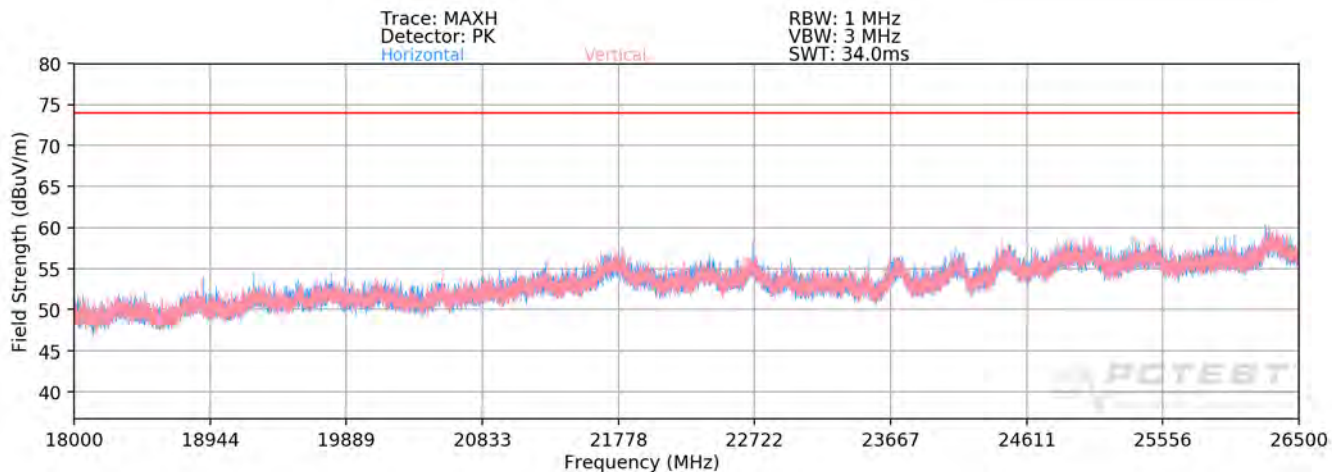
Plot 7-272. Radiated Spurious Plot 18GHz – 26.5GHz (2.4GHz – 5GHz)
