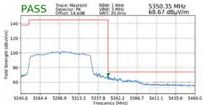
Plot 7-350. Radiated Upper Band Edge Plot MIMO (Peak – UNII Band 2A)
