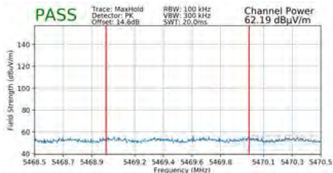
Plot 7-320. Radiated Lower Band Edge Plot SISO ANT2 (Peak – UNII Band 2C)
