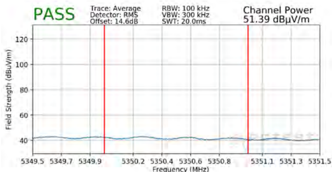
Plot 7-324. Radiated Upper Band Edge Plot MIMO (Average – UNII Band 2A)
