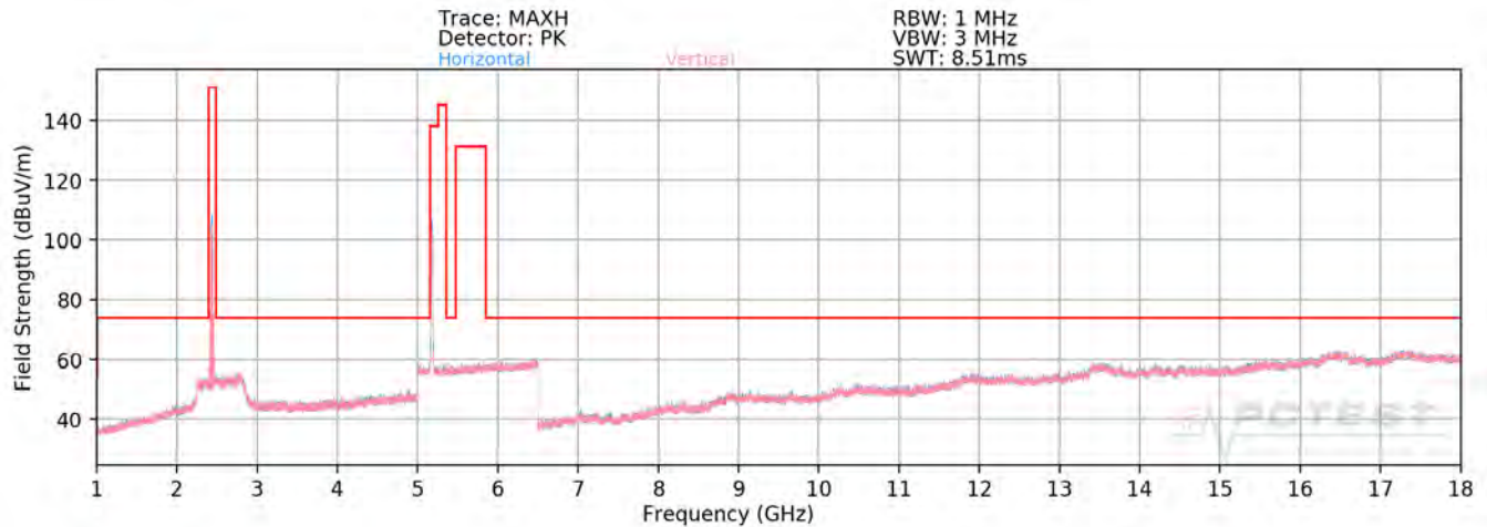
Plot 7-277. Radiated Spurious Plot above 1GHz (Dual Band Simult. Tx)
