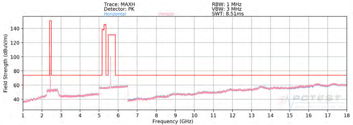
Plot 7-274. Radiated Spurious Plot above 1GHz (5GHz – 2.4 GHz)
