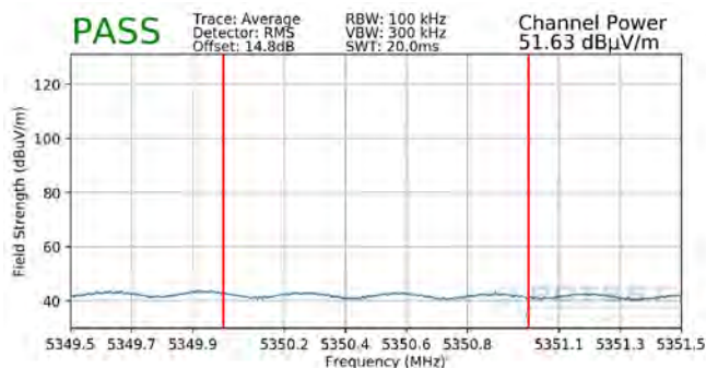
Plot 7-340. Radiated Upper Band Edge Plot MIMO (Average – UNII Band 2A)
