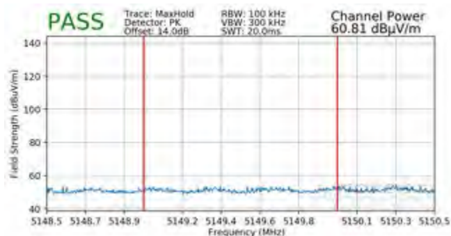
Plot 7-309. Radiated Lower Band Edge Plot SISO ANT2 (Peak – UNII Band 1)
