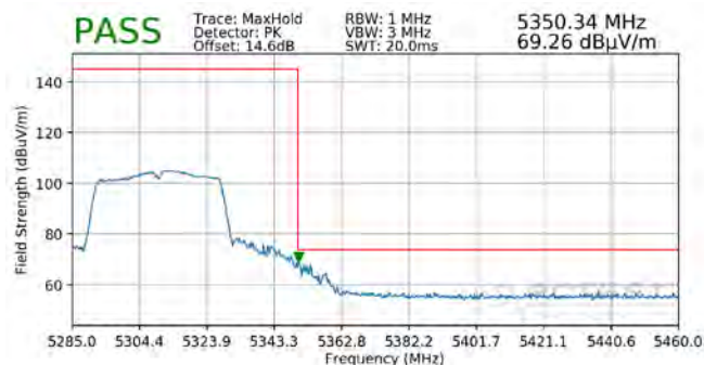
Plot 7-341. Radiated Upper Band Edge Plot MIMO (Peak – UNII Band 2A)
