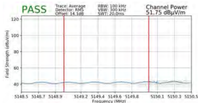
Plot 7-287. Radiated Lower Band Edge Plot SISO ANT1 (Average - UNII Band 1)
