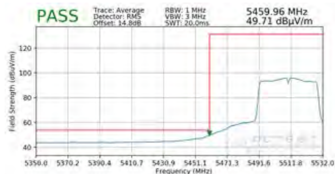
Plot 7-291. Radiated Lower Band Edge Plot SISO ANT1 (Average – UNII Band 2C)
