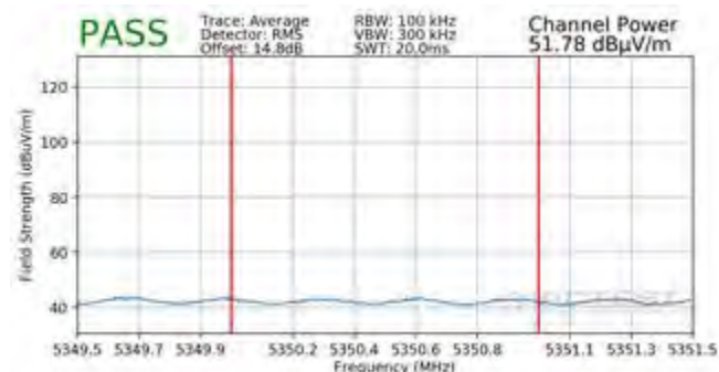
Plot 7-296. Radiated Upper Band Edge Plot SISO ANT1 (Average - UNII Band 2A)
