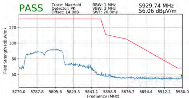
Plot 7-344. Radiated Upper Band Edge Plot MIMO (Peak – UNII Band 3)
