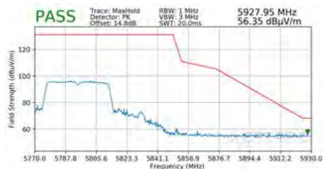
Plot 7-293. Radiated Upper Band Edge Plot SISO ANT1 (Peak – UNII Band 3)
