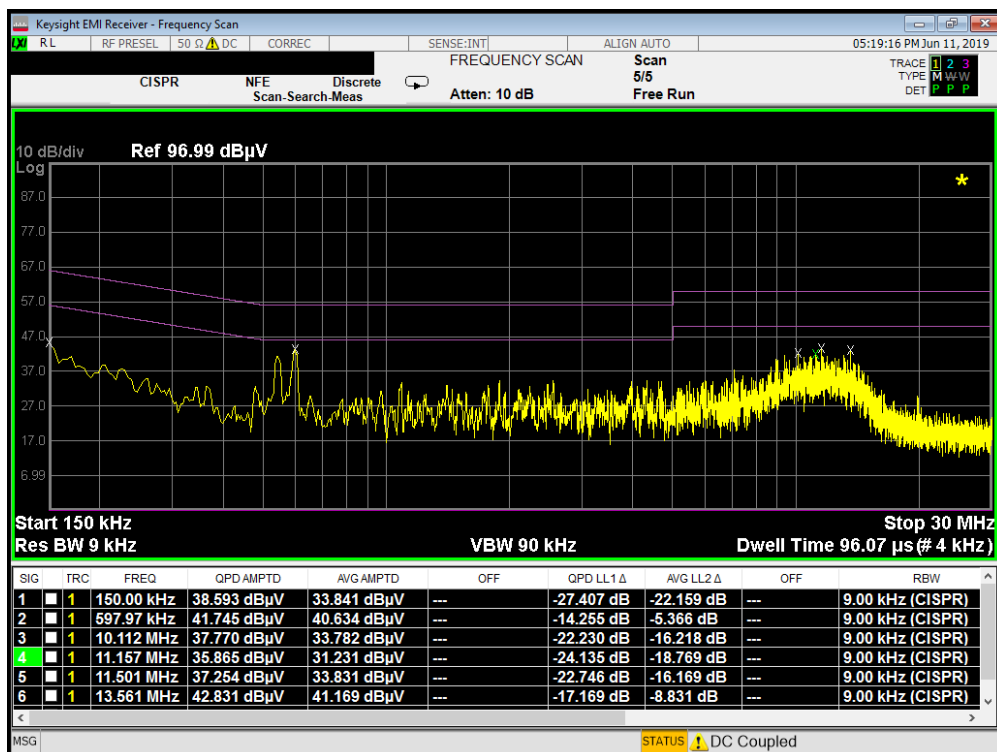
Plot 7-366. Line Conducted Plot with 802.11a UNII Band 2A (N)
