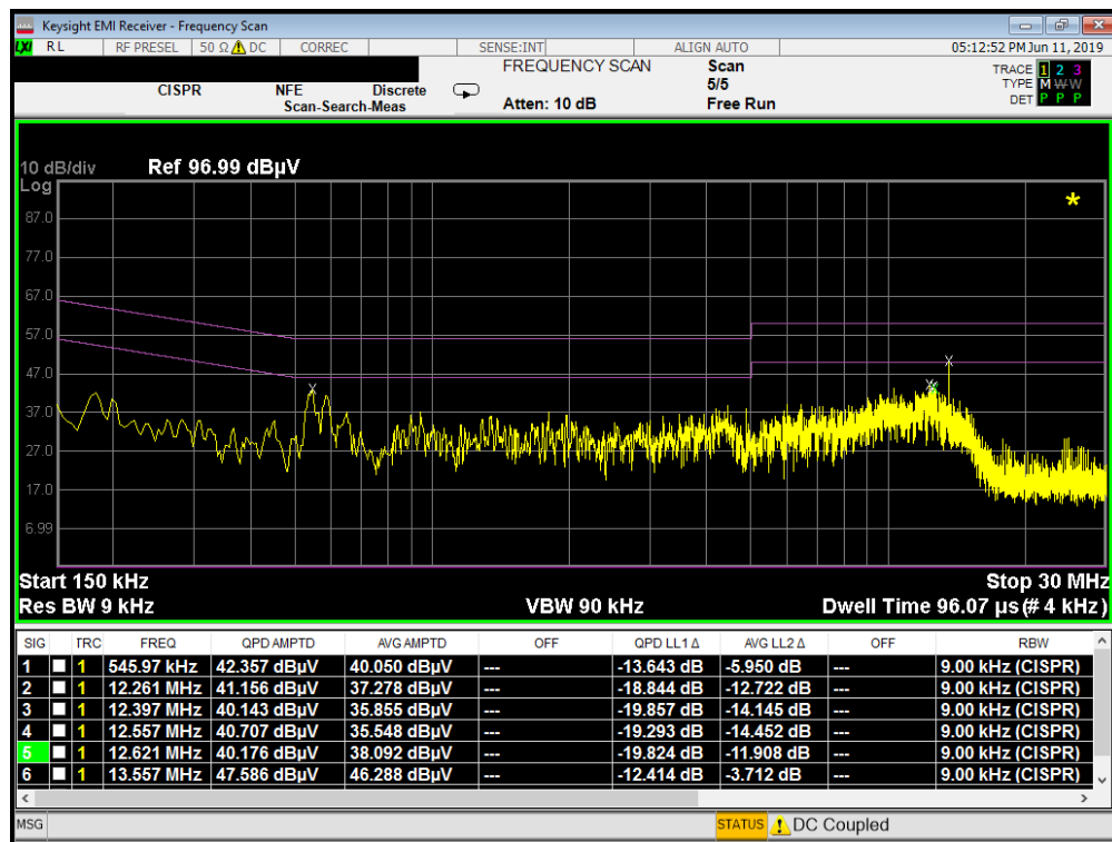
Plot 7-363. Line Conducted Plot with 802.11a UNII Band 1 with WCP (L1)
