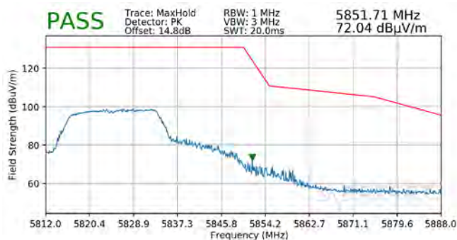
Plot 7-335. Radiated Upper Band Edge Plot MIMO (Peak – UNII Band 3)
