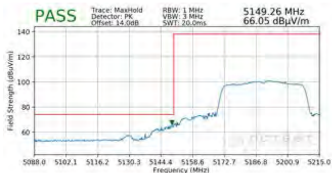
Plot 7-288. Radiated Lower Band Edge Plot SISO ANT1 (Peak - UNII Band 1)
