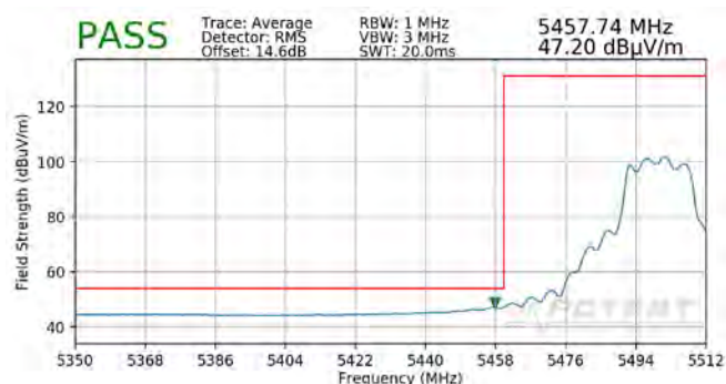
Plot 7-326. Radiated Lower Band Edge Plot MIMO (Average – UNII Band 2C)
