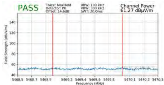
Plot 7-299. Radiated Lower Band Edge Plot SISO ANT1 (Peak – UNII Band 2C)
