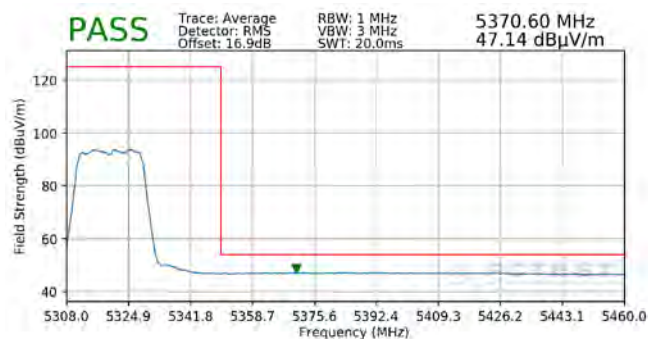
Plot 7-336. Radiated Band Edge Plot MIMO (Average - WCP)
