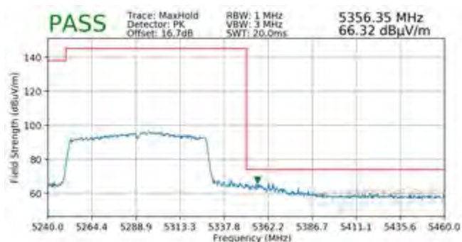
Plot 7-355. Radiated Band Edge Plot MIMO (Peak - WCP)
