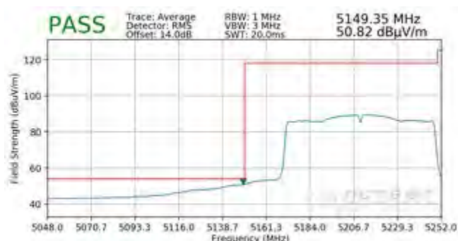
Plot 7-315. Radiated Lower Band Edge Plot SISO ANT2 (Average – UNII Band 1)
