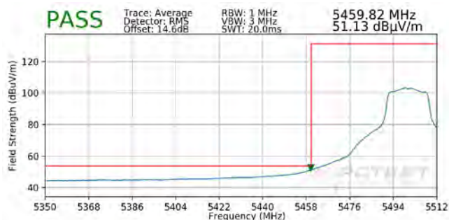
Plot 7-284. Radiated Lower Band Edge Plot SISO ANT1 (Average - UNII Band 2C)
