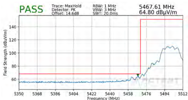
Plot 7-327. Radiated Lower Band Edge Plot MIMO (Peak – UNII Band 2C)
