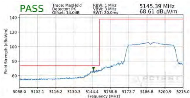
Plot 7-339. Radiated Lower Band Edge Plot MIMO (Peak – UNII Band 1)
