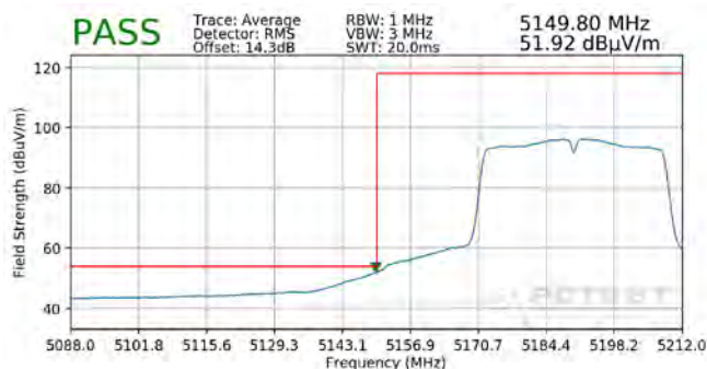
Plot 7-338. Radiated Lower Band Edge Plot MIMO (Average – UNII Band 1)
