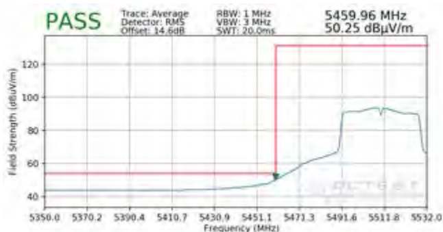
Plot 7-312. Radiated Lower Band Edge Plot SISO ANT2 (Average – UNII Band 2C)
