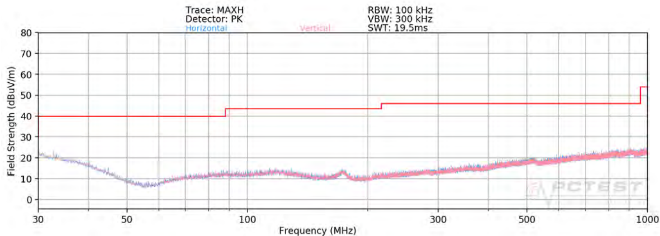
Plot 7-357. Radiated Spurious Plot below 1GHz SISO ANT2 (802.11a - U2A Ch. 64)
