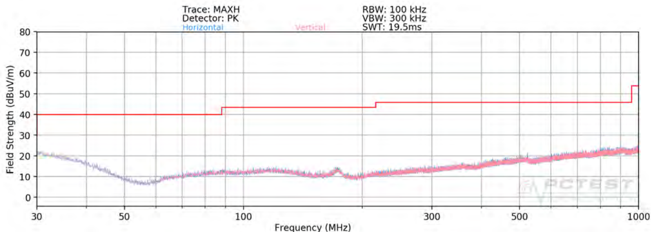
Plot 7-359. Radiated Spurious Plot below 1GHz (2.4GHz – 5GHz)
