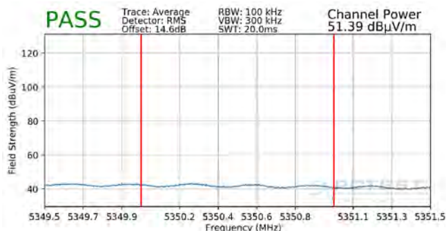
Plot 7-331. Radiated Upper Band Edge Plot MIMO (Average – UNII Band 2A)
