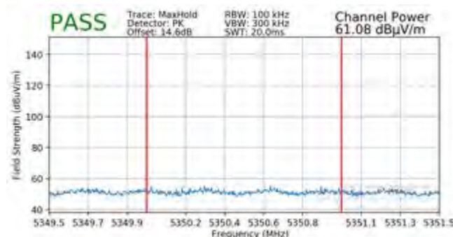
Plot 7-318. Radiated Upper Band Edge Plot SISO ANT2 (Peak – UNII Band 2A)
