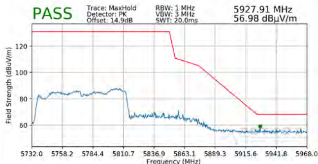
Plot 7-353. Radiated Upper Band Edge Plot MIMO (Peak – UNII Band 3)
