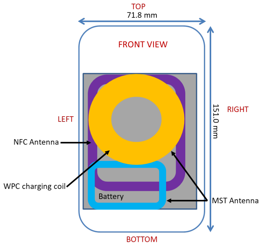
Figure F-2 NFC Antenna Locations
