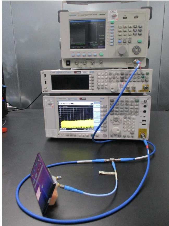
ANTENNA PORT CONDUCTED PHOTO
