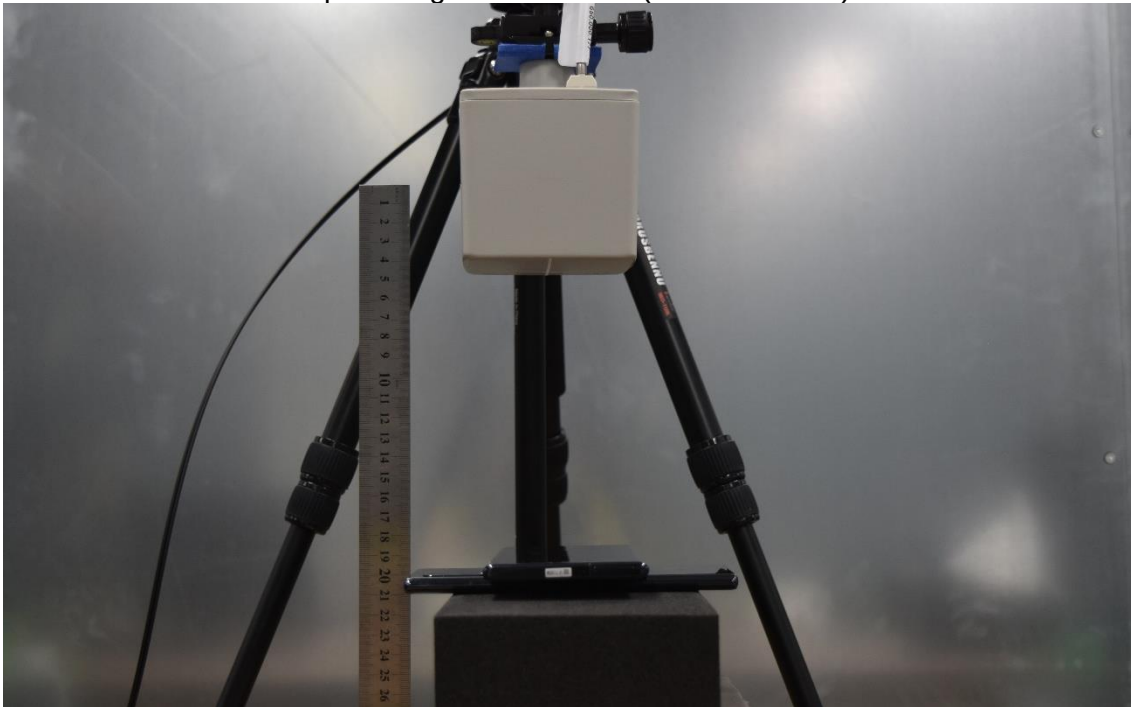
Top – charger below client (20cm distance)
