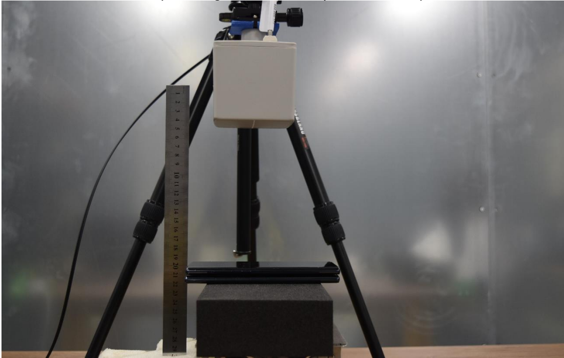
Top – charger below client (20cm distance)
