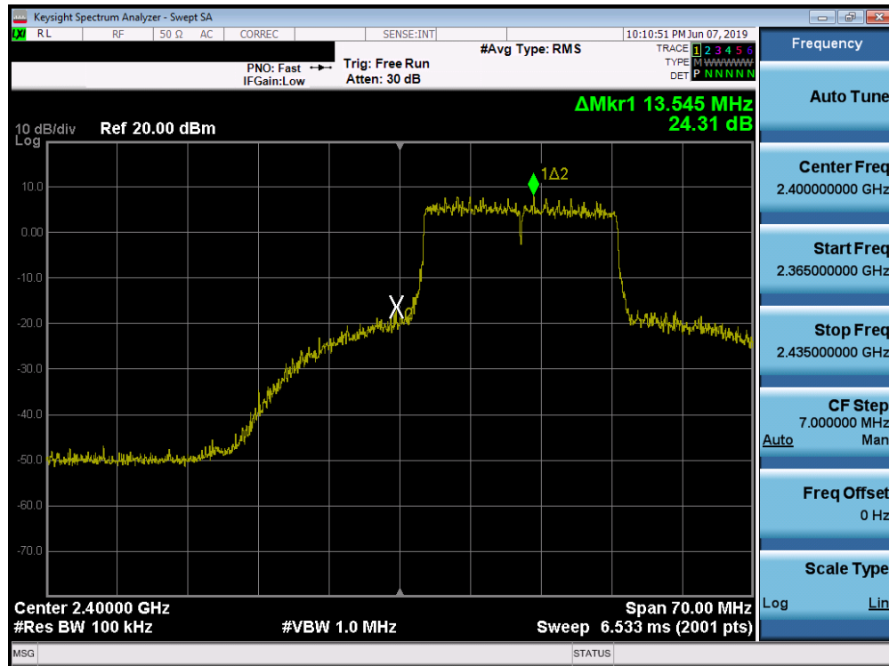
Plot 7-41. Band Edge Plot SISO ANT1 (802.11ax OFDMA – 242 Tones – Ch. 1)
