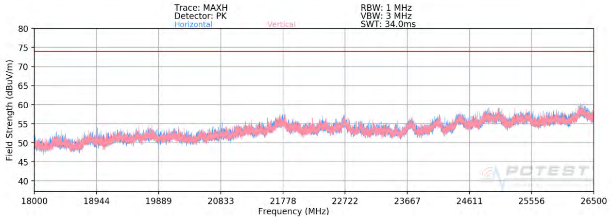
Plot 7-92. Radiated Spurious Plot above 18GHz SISO ANT2 (802.11ax OFDMA – 242 Tones)
