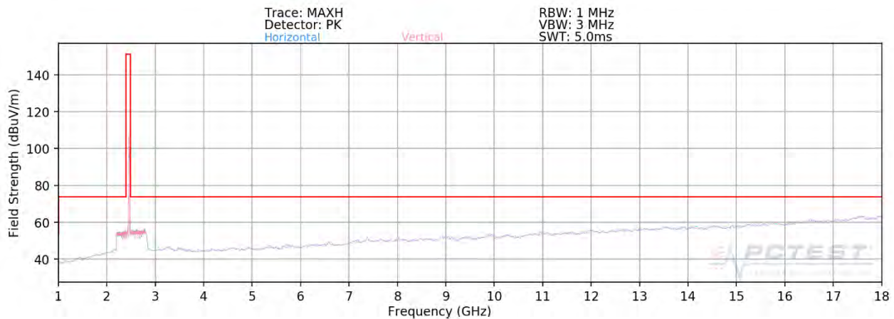
Plot 7-87. Radiated Spurious Plot above 1GHz SISO ANT2 (802.11ax OFDMA – 26 Tones – Ch. 11)
