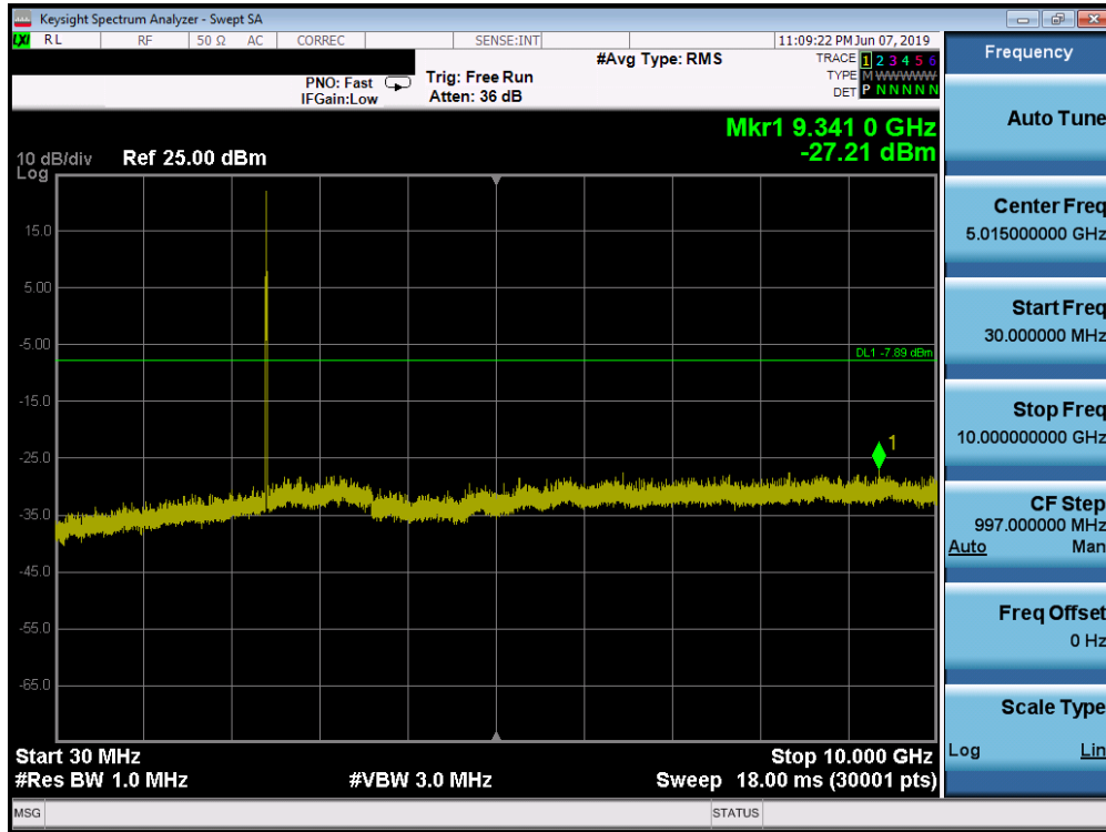
Plot 7-65. Conducted Spurious Plot SISO ANT2 (802.11ax OFDMA – 26 Tones – Ch. 1)
