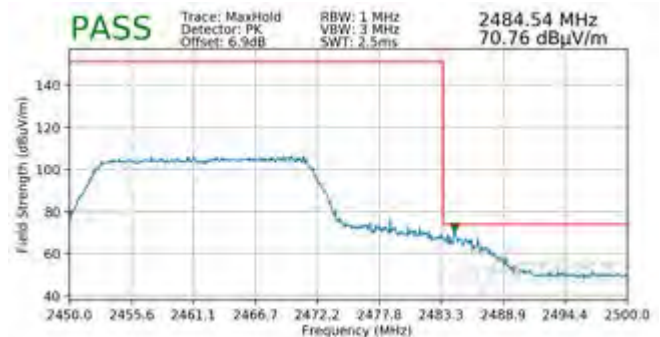
Plot 7-120. Radiated Restricted Upper Band Edge Measurement SISO ANT1 (Peak – 242 Tones)
