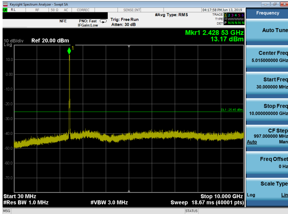
Plot 7-73. Conducted Spurious Plot SISO ANT2 (802.11ax OFDMA – 242 Tones – Ch. 6)
