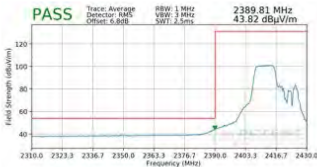
Plot 7-103. Radiated Restricted Lower Band Edge Measurement SISO ANT1 (Average – 106 Tones)
