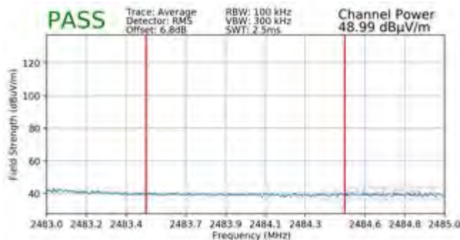
Plot 7-123. Radiated Restricted Upper Band Edge Measurement SISO ANT1 (Average – 242 Tones)
