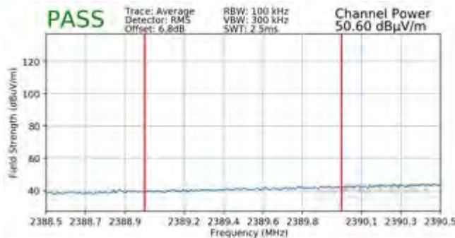
Plot 7-115. Radiated Restricted Lower Band Edge Measurement SISO ANT1 (Average – 242 Tones)
