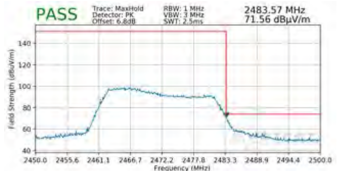
Plot 7-144. Radiated Restricted Upper Band Edge Measurement SISO ANT2 (Peak – 242 Tones)
