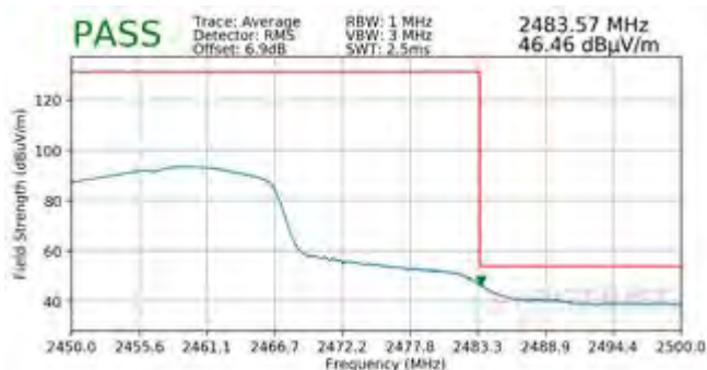
Plot 7-137. Radiated Restricted Upper Band Edge Measurement SISO ANT2 (Average – 242 Tones)
