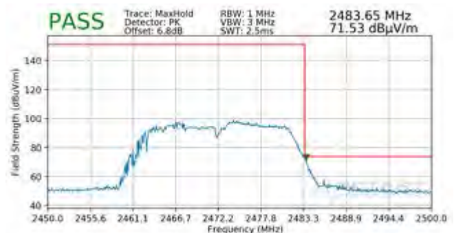
Plot 7-112. Radiated Restricted Upper Band Edge Measurement SISO ANT1 (Peak – 106 Tones)
