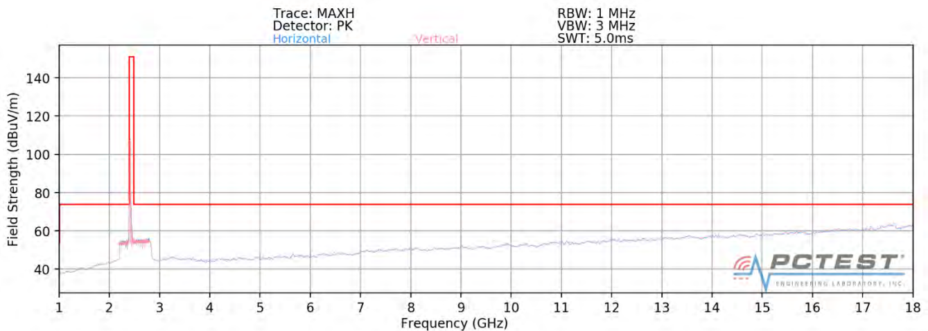
Plot 7-80. Radiated Spurious Plot above 1GHz SISO ANT1 (802.11ax OFDMA – 242 Tones – Ch. 1)
