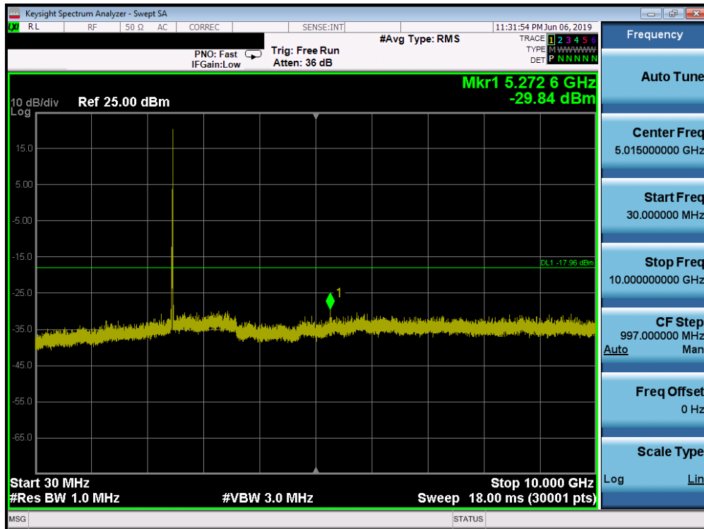
Plot 7-57. Conducted Spurious Plot SISO ANT1 (802.11ax OFDMA – 26 Tones – Ch. 11)
