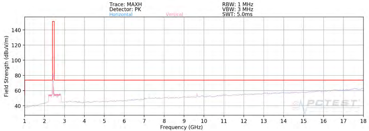
Plot 7-96. Radiated Spurious Plot above 1GHz MIMO (802.11ax OFDMA – 242 Tones – Ch. 1)
