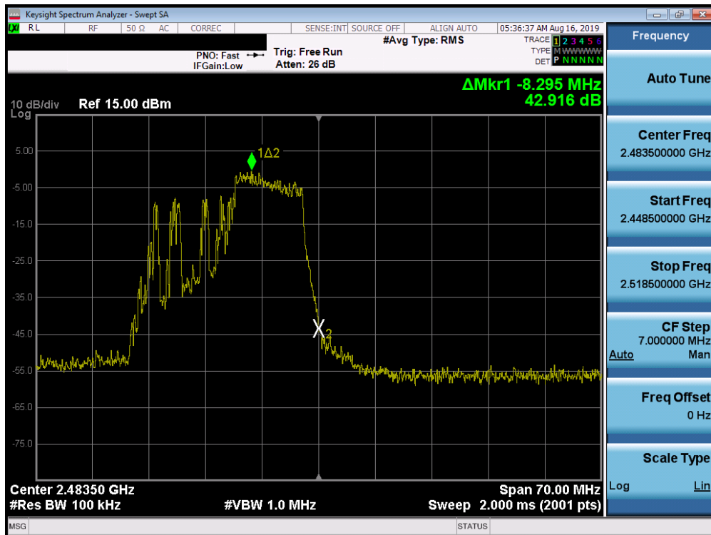
Plot 7-40. Band Edge Plot SISO ANT1 (802.11ax OFDMA – 106 Tones – Ch. 13)
