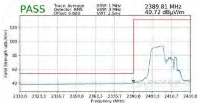
Plot 7-125. Radiated Restricted Lower Band Edge Measurement SISO ANT2 (Average – 106 Tones)
