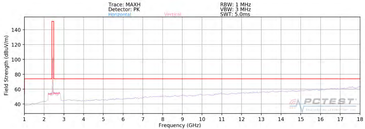
Plot 7-89. Radiated Spurious Plot above 1GHz SISO ANT2 (802.11ax OFDMA – 242 Tones – Ch. 6)
