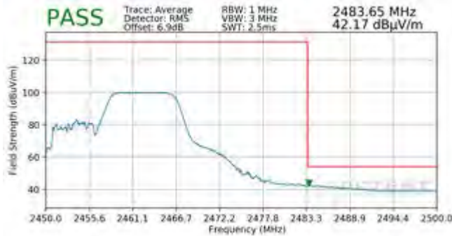
Plot 7-105. Radiated Restricted Upper Band Edge Measurement SISO ANT1 (Average – 106 Tones)
