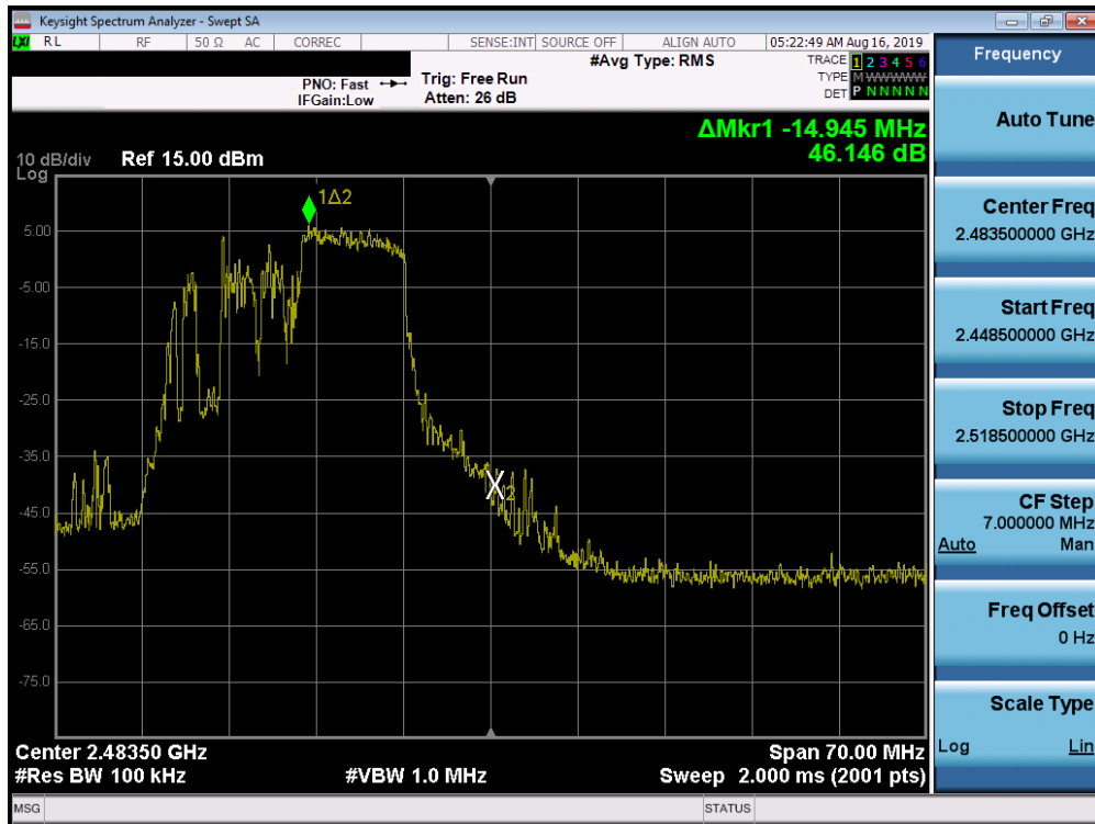
Plot 7-47. Band Edge Plot SISO ANT2 (802.11ax OFDMA - 106 Tones - Ch. 12)
