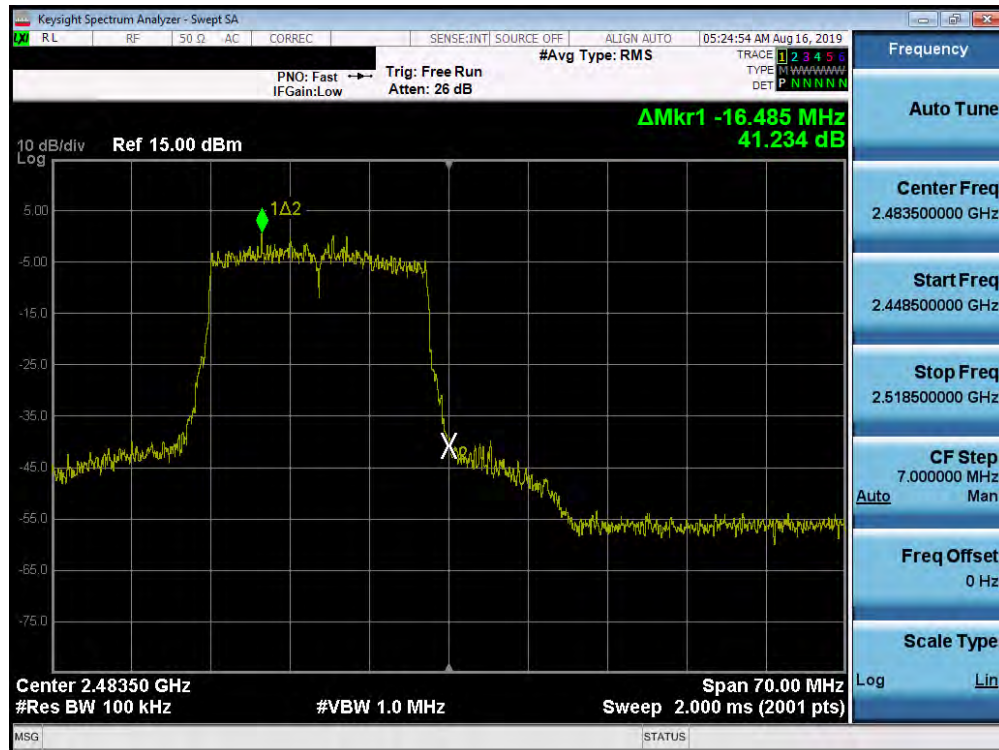
Plot 7-52. Band Edge Plot SISO ANT2 (802.11ax OFDMA - 242 Tones - Ch. 13)
