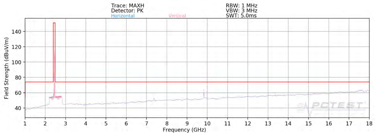
Plot 7-95. Radiated Spurious Plot above 1GHz MIMO (802.11ax OFDMA – 26 Tones – Ch. 11)
