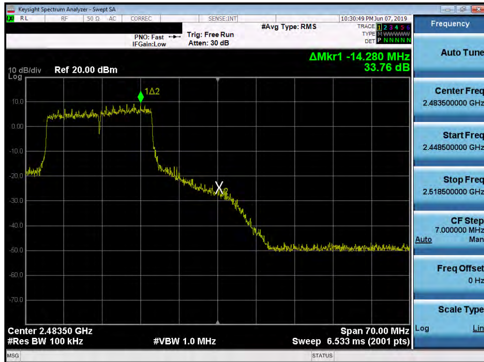
Plot 7-42. Band Edge Plot SISO ANT1 (802.11ax OFDMA – 242 Tones – Ch. 11)
