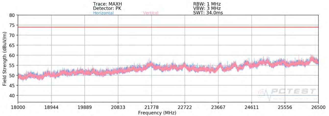
Plot 7-83. Radiated Spurious Plot above 18GHz SISO ANT1 (802.11ax OFDMA – 26 Tones)
