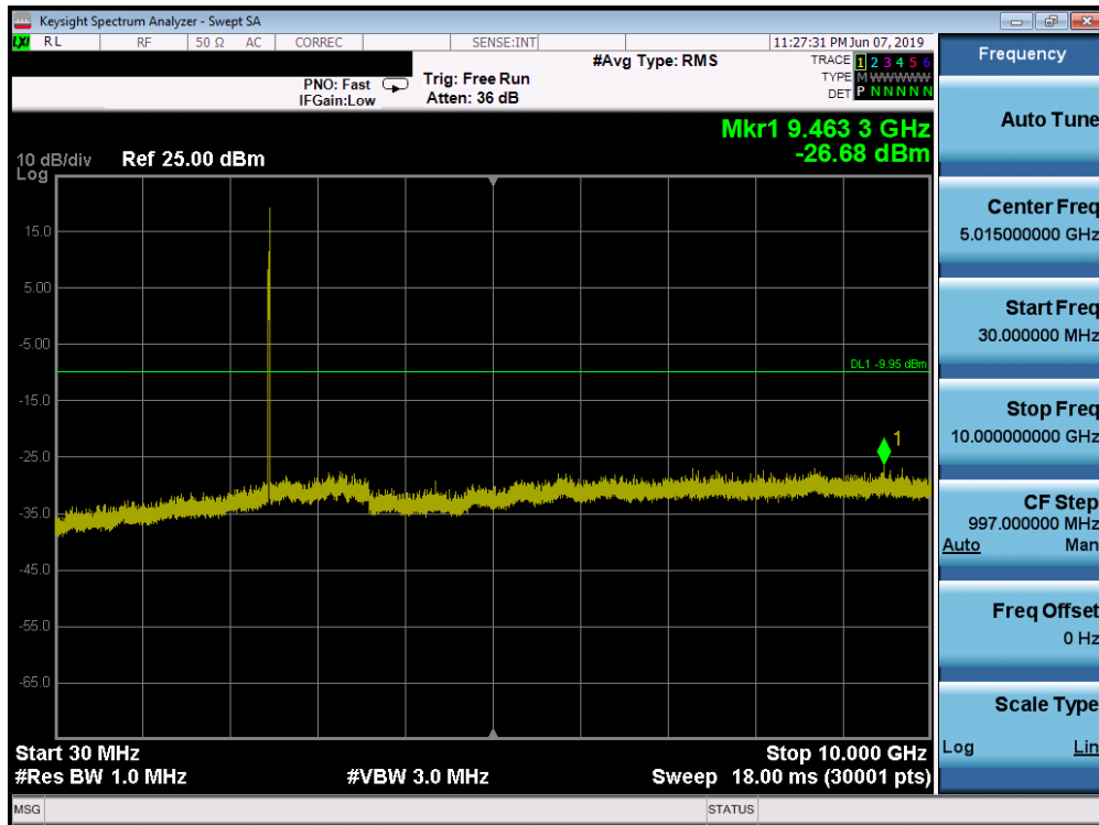
Plot 7-69. Conducted Spurious Plot SISO ANT2 (802.11ax OFDMA – 26 Tones – Ch. 11)
