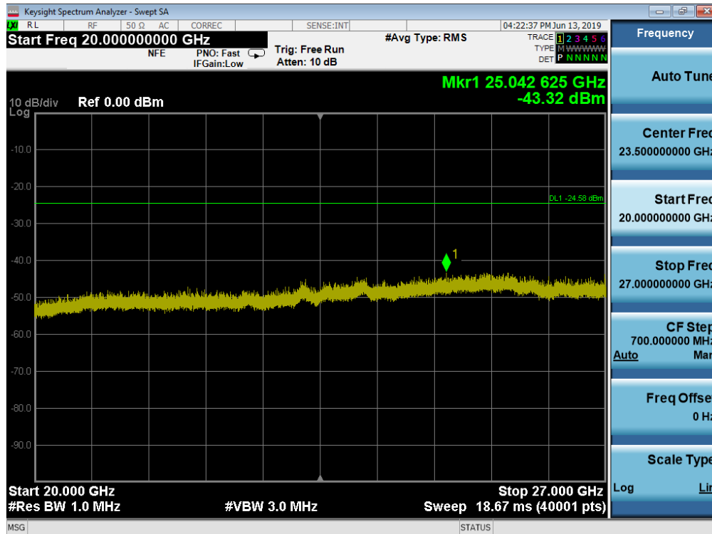
Plot 7-76. Conducted Spurious Plot SISO ANT2 (802.11ax OFDMA – 242 Tones – Ch. 11)
