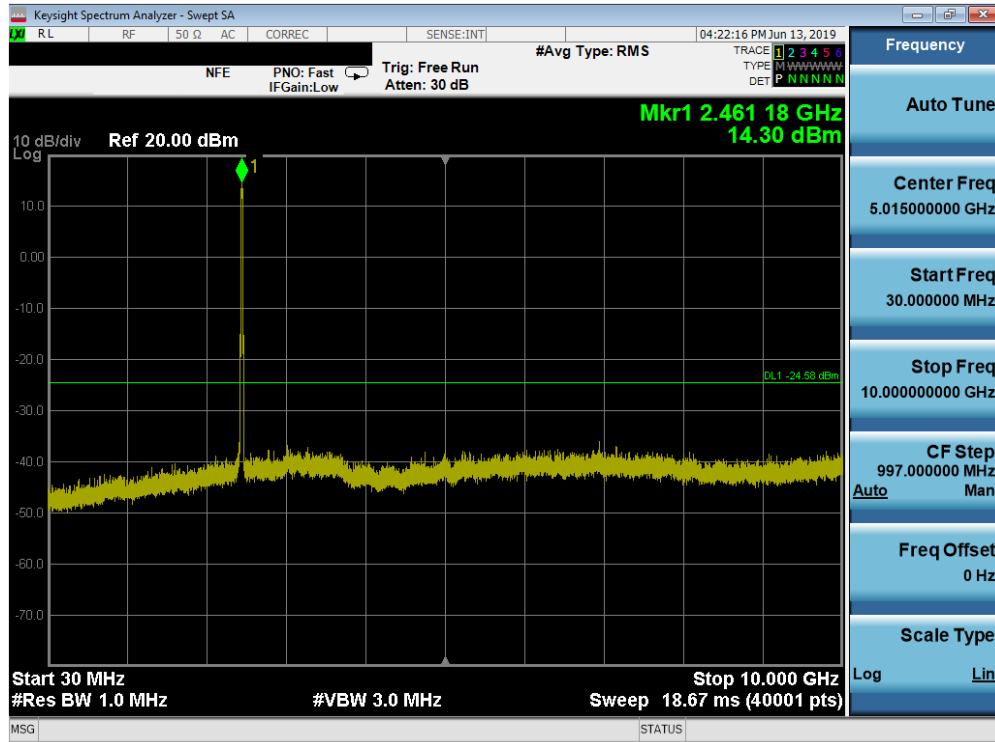
Plot 7-75. Conducted Spurious Plot SISO ANT2 (802.11ax OFDMA – 242 Tones – Ch. 11)
