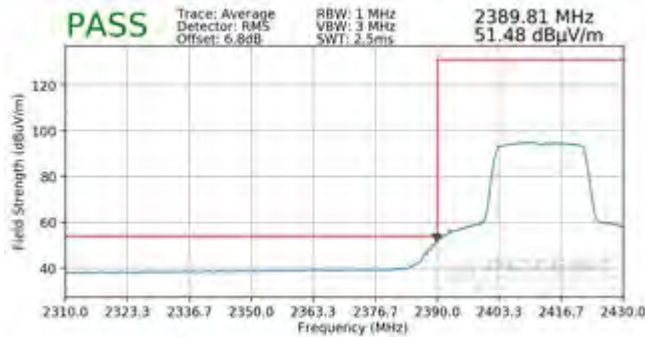
Plot 7-113. Radiated Restricted Lower Band Edge Measurement SISO ANT1 (Average – 242 Tones)
