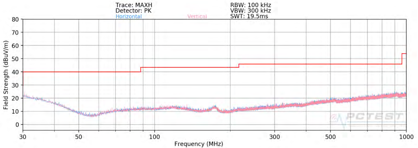
Plot 7-161. Radiated Spurious Plot below 1GHz MIMO (26 Tones)
