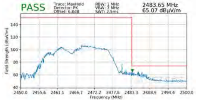
Plot 7-150. Radiated Restricted Upper Band Edge Measurement MIMO (Peak – 106 Tones)
