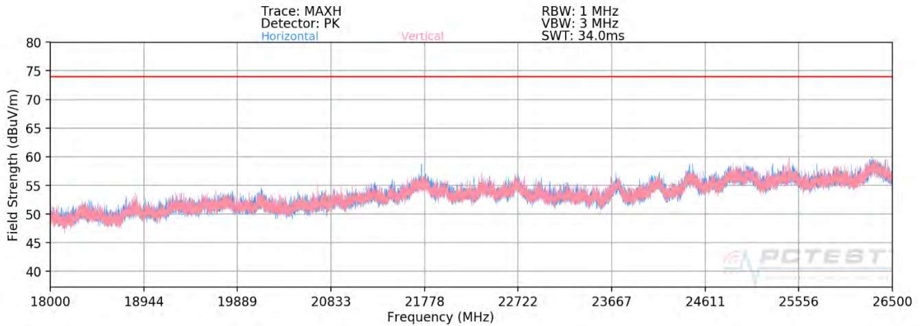
Plot 7-99. Radiated Spurious Plot above 18GHz MIMO (802.11ax OFDMA – 26 Tones)
