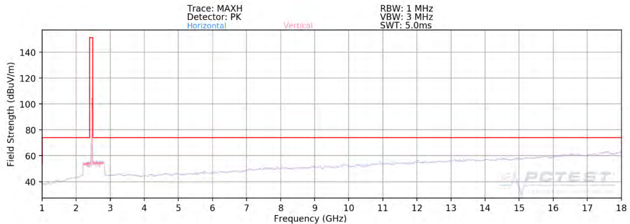
Plot 7-90. Radiated Spurious Plot above 1GHz SISO ANT2 (802.11ax OFDMA – 242 Tones – Ch. 11)
