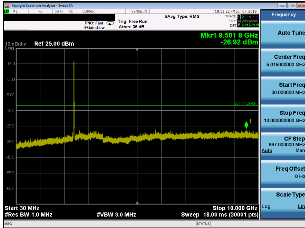
Plot 7-59. Conducted Spurious Plot SISO ANT1 (802.11ax OFDMA – 242 Tones – Ch. 1)
