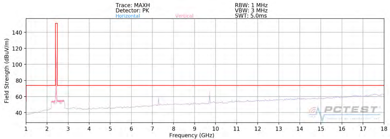
Plot 7-94. Radiated Spurious Plot above 1GHz MIMO (802.11ax OFDMA – 26 Tones – Ch. 6)
