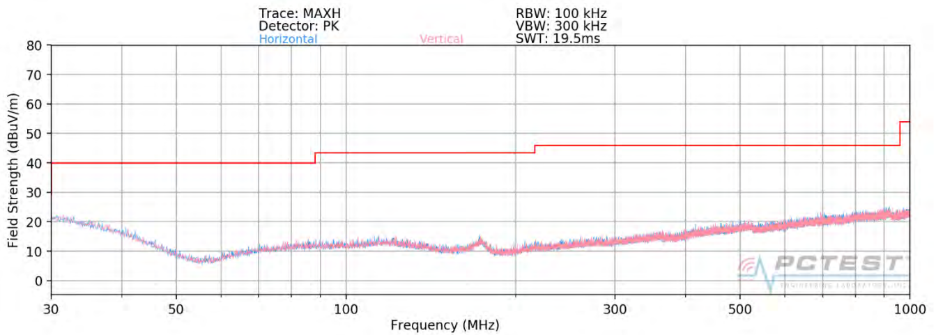
Plot 7-162. Radiated Spurious Plot below 1GHz MIMO (242 Tones)
