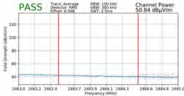
Plot 7-117. Radiated Restricted Upper Band Edge Measurement SISO ANT1 (Average – 242 Tones)
