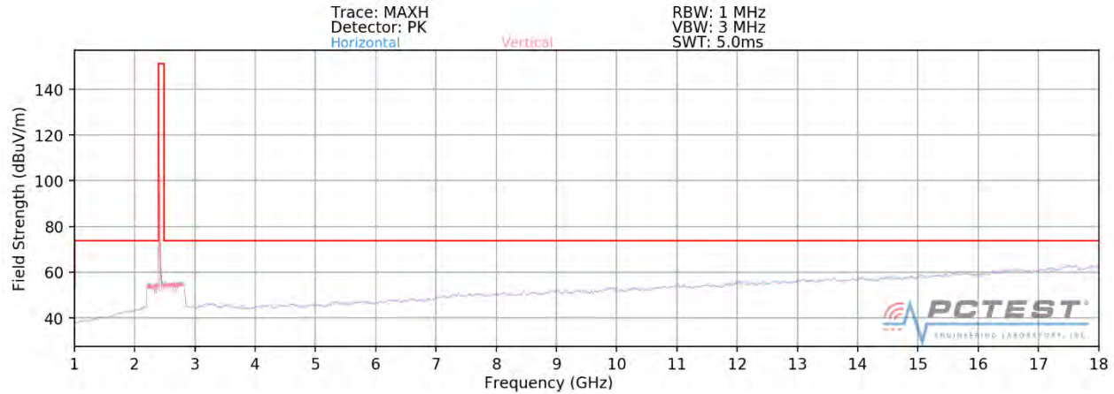
Plot 7-88. Radiated Spurious Plot above 1GHz SISO ANT2 (802.11ax OFDMA – 242 Tones – Ch. 1)
