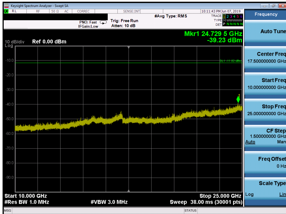
Plot 7-60. Conducted Spurious Plot SISO ANT1 (802.11ax OFDMA – 242 Tones – Ch. 1)
