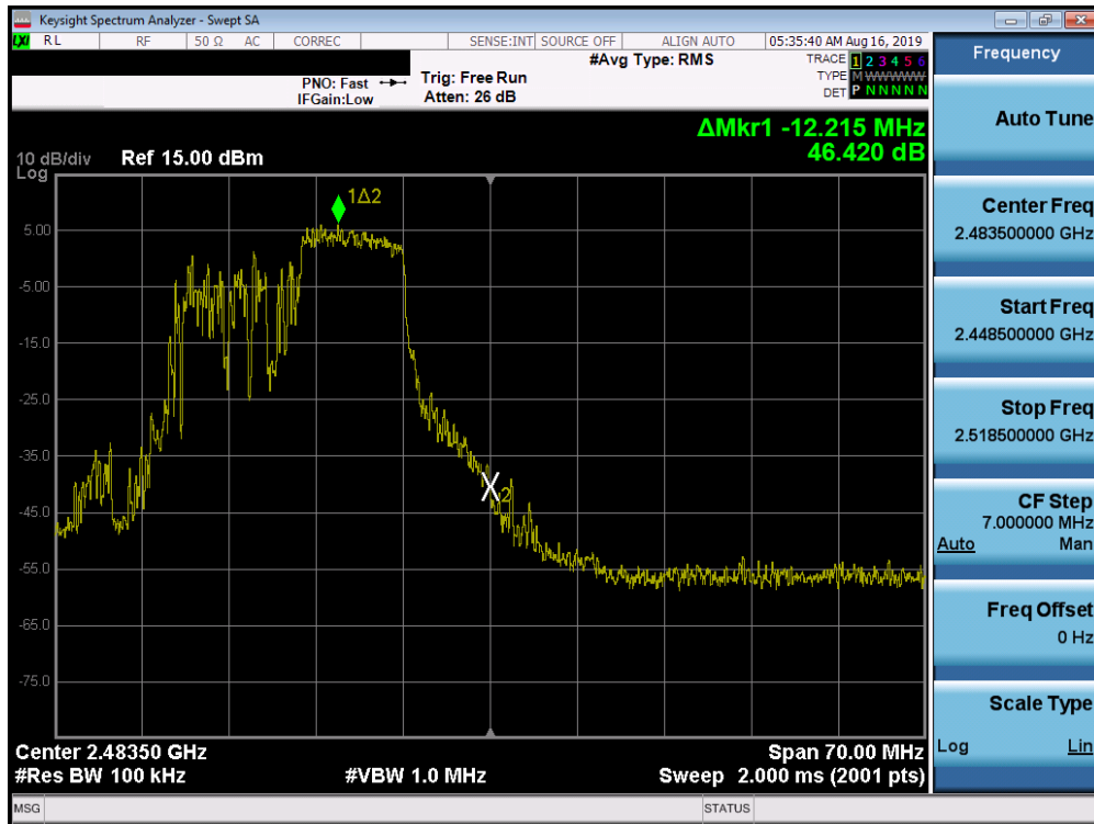
Plot 7-39. Band Edge Plot SISO ANT1 (802.11ax OFDMA – 106 Tones – Ch. 12)
