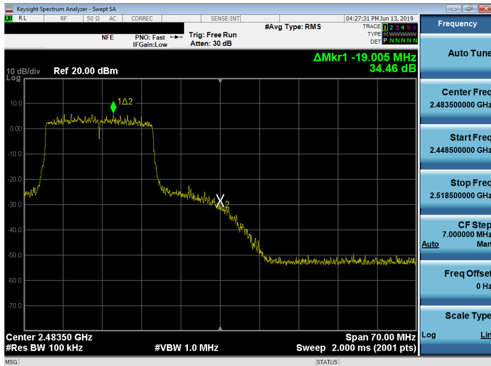
Plot 7-50. Band Edge Plot SISO ANT2 (802.11ax OFDMA - 242 Tones - Ch. 11)
