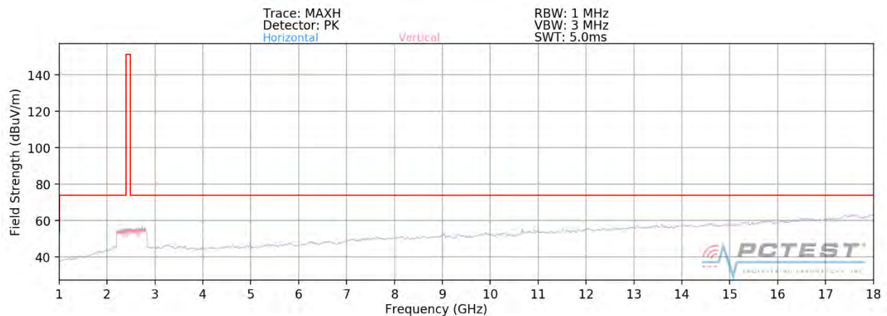
Plot 7-98. Radiated Spurious Plot above 1GHz MIMO (802.11ax OFDMA – 242 Tones – Ch. 11)
