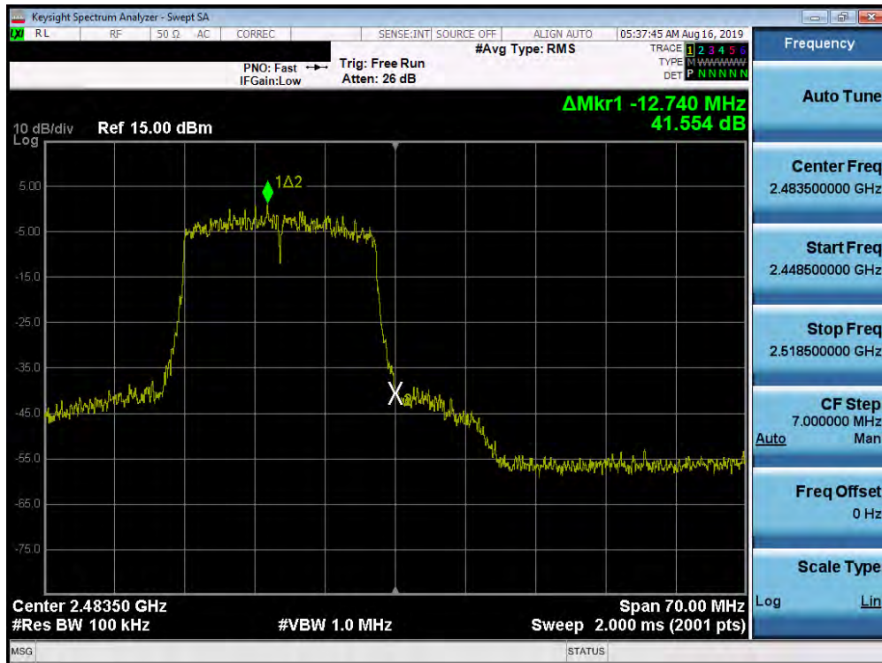
Plot 7-44. Band Edge Plot SISO ANT1 (802.11ax OFDMA - 242 Tones - Ch. 13)
