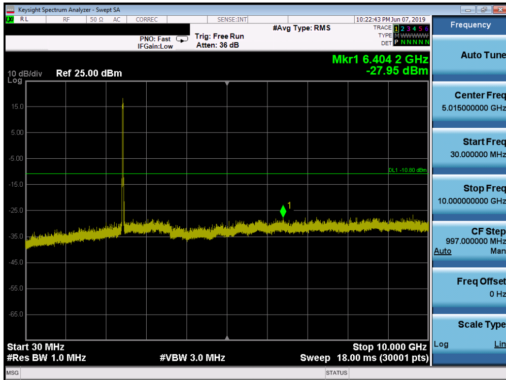
Plot 7-61. Conducted Spurious Plot SISO ANT1 (802.11ax OFDMA – 242 Tones – Ch. 6)
