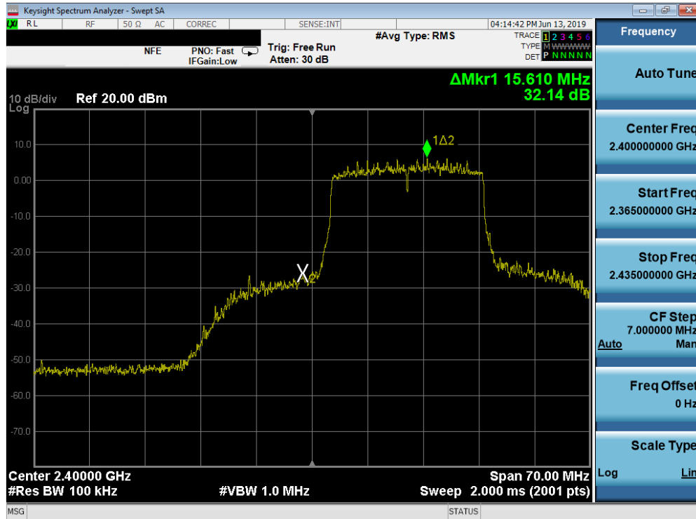
Plot 7-49. Band Edge Plot SISO ANT2 (802.11ax OFDMA - 242 Tones - Ch. 1)
