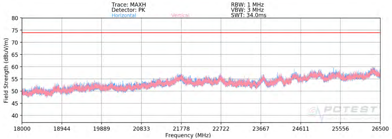
Plot 7-91. Radiated Spurious Plot above 18GHz SISO ANT2 (802.11ax OFDMA – 26 Tones)
