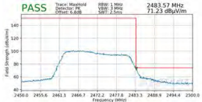
Plot 7-158. Radiated Restricted Upper Band Edge Measurement MIMO (Peak – 242 Tones)
