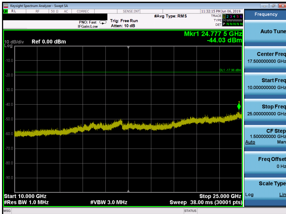
Plot 7-58. Conducted Spurious Plot SISO ANT1 (802.11ax OFDMA – 26 Tones – Ch. 11)
