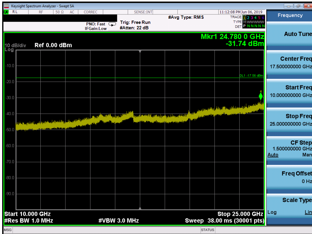
Plot 7-54. Conducted Spurious Plot SISO ANT1 (802.11ax OFDMA – 26 Tones – Ch. 1)
