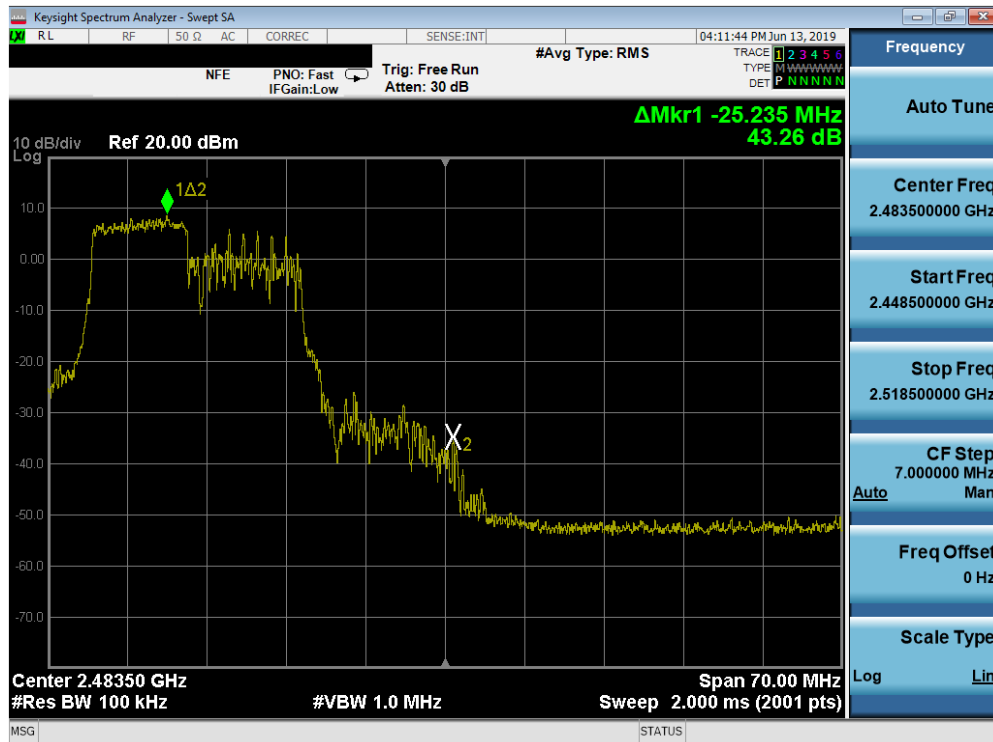
Plot 7-46. Band Edge Plot SISO ANT2 (802.11ax OFDMA - 106 Tones - Ch. 11)
