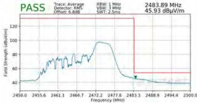
Plot 7-109. Radiated Restricted Upper Band Edge Measurement SISO ANT1 (Average – 52 Tones)
