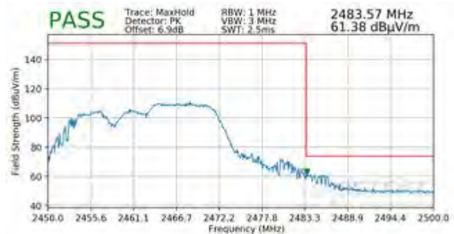
Plot 7-148. Radiated Restricted Upper Band Edge Measurement MIMO (Peak – 106 Tones)
