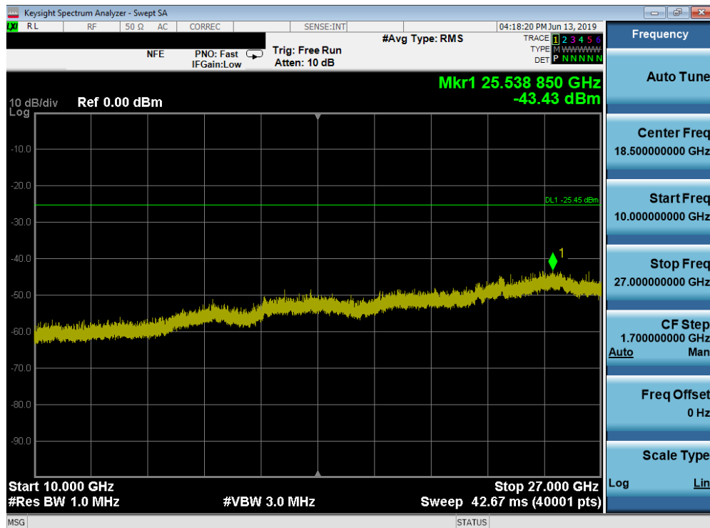
Plot 7-74. Conducted Spurious Plot SISO ANT2 (802.11ax OFDMA – 242 Tones – Ch. 6)
