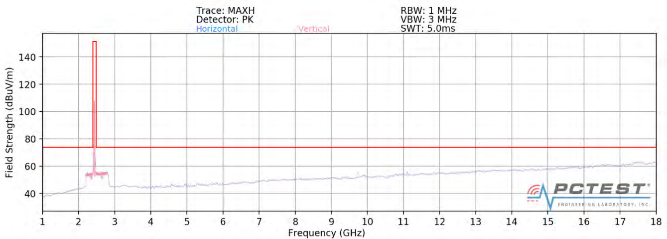
Plot 7-81. Radiated Spurious Plot above 1GHz SISO ANT1 (802.11ax OFDMA – 242 Tones – Ch. 6)
