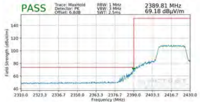
Plot 7-116. Radiated Restricted Lower Band Edge Measurement SISO ANT1 (Peak – 242 Tones)
