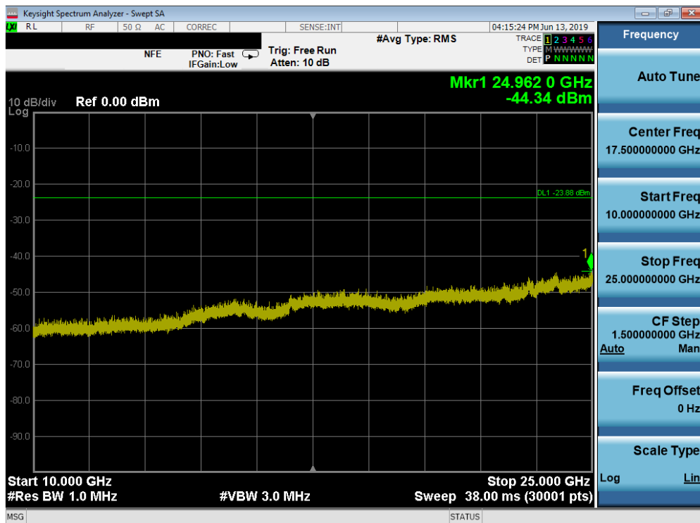
Plot 7-72. Conducted Spurious Plot SISO ANT2 (802.11ax OFDMA – 242 Tones – Ch. 1)
