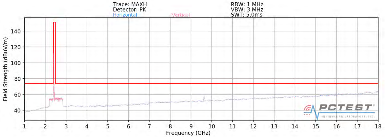
Plot 7-77. Radiated Spurious Plot above 1GHz SISO ANT1 (802.11ax OFDMA – 26 Tones – Ch. 1)
