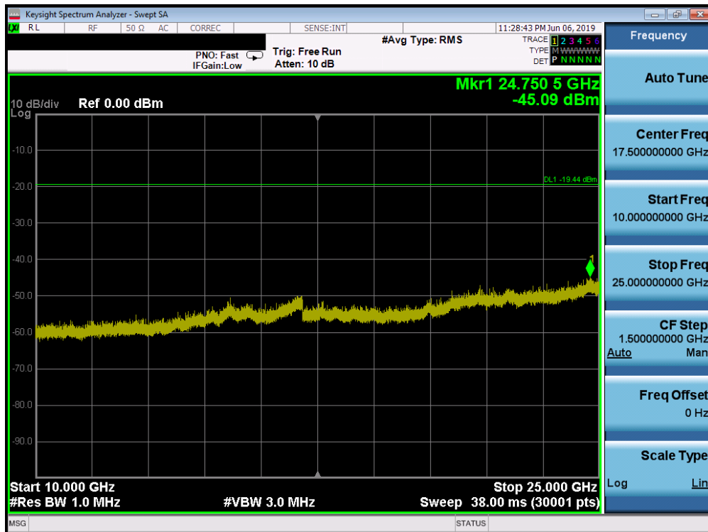
Plot 7-56. Conducted Spurious Plot SISO ANT1 (802.11ax OFDMA – 26 Tones – Ch. 6)
