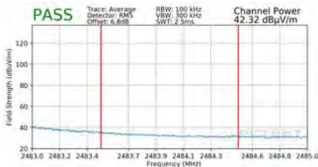
Plot 7-151. Radiated Restricted Upper Band Edge Measurement MIMO (Average – 52 Tones)
