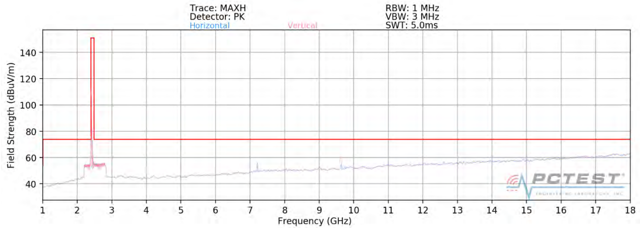
Plot 7-93. Radiated Spurious Plot above 1GHz MIMO (802.11ax OFDMA – 26 Tones – Ch. 1)
