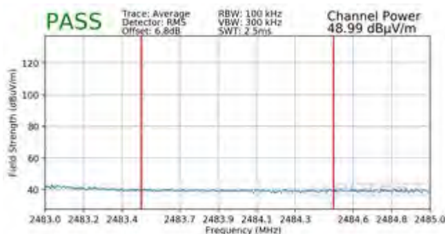
Plot 7-111. Radiated Restricted Upper Band Edge Measurement SISO ANT1 (Average – 106 Tones)
