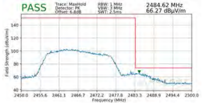
Plot 7-142. Radiated Restricted Upper Band Edge Measurement SISO ANT2 (Peak – 242 Tones)
