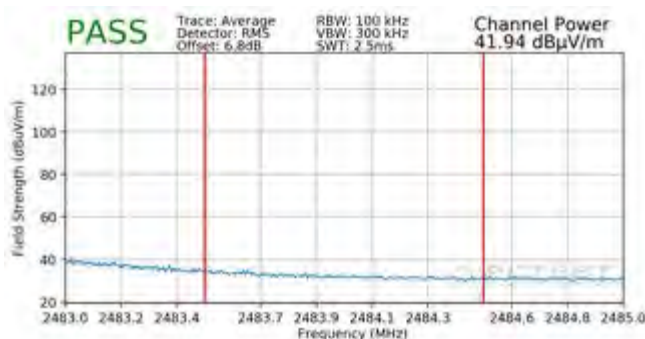
Plot 7-131. Radiated Restricted Upper Band Edge Measurement SISO ANT2 (Average – 26 Tones)
