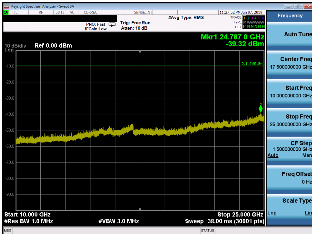
Plot 7-70. Conducted Spurious Plot SISO ANT2 (802.11ax OFDMA – 26 Tones – Ch. 11)
