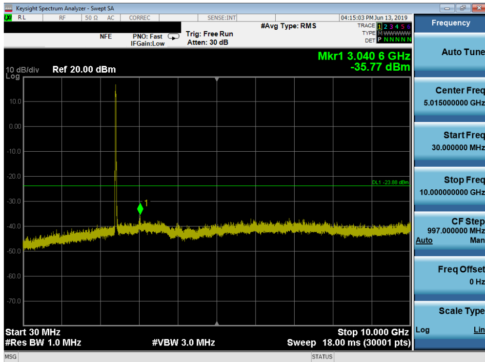
Plot 7-71. Conducted Spurious Plot SISO ANT2 (802.11ax OFDMA – 242 Tones – Ch. 1)
