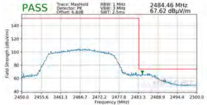
Plot 7-122. Radiated Restricted Upper Band Edge Measurement SISO ANT1 (Peak – 242 Tones)
