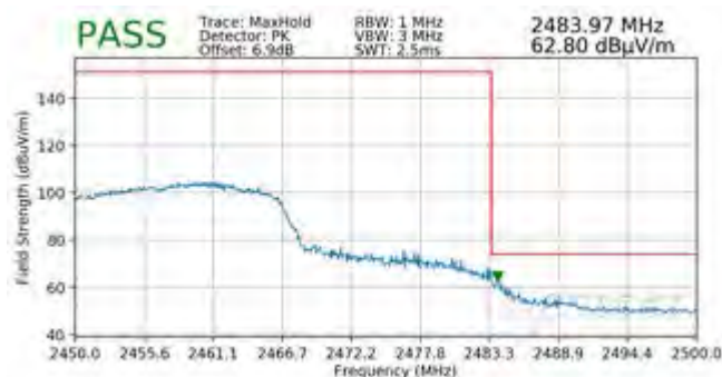
Plot 7-138. Radiated Restricted Upper Band Edge Measurement SISO ANT2 (Peak – 242 Tones)
