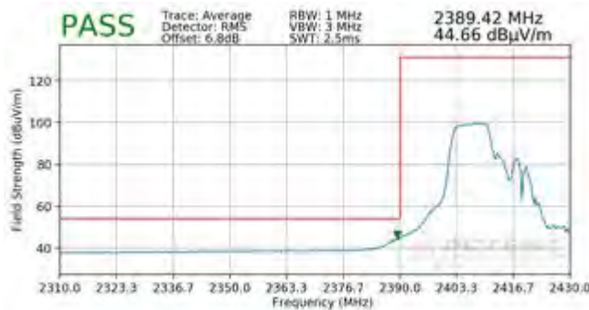
Plot 7-145. Radiated Restricted Lower Band Edge Measurement MIMO (Average – 106 Tones)
