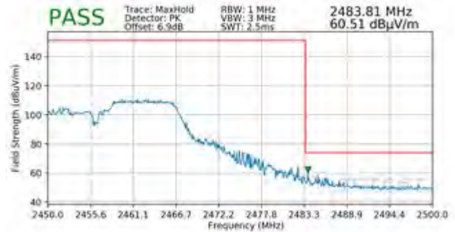
Plot 7-106. Radiated Restricted Upper Band Edge Measurement SISO ANT1 (Peak – 106 Tones)
