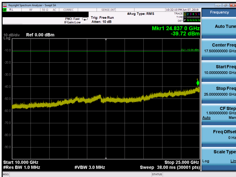
Plot 7-64. Conducted Spurious Plot SISO ANT1 (802.11ax OFDMA - 242 Tones - Ch. 11)
