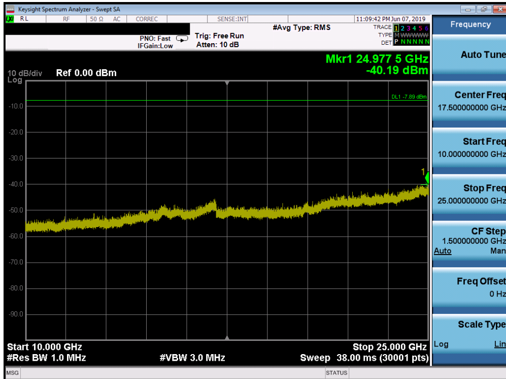
Plot 7-66. Conducted Spurious Plot SISO ANT2 (802.11ax OFDMA – 26 Tones – Ch. 1)
