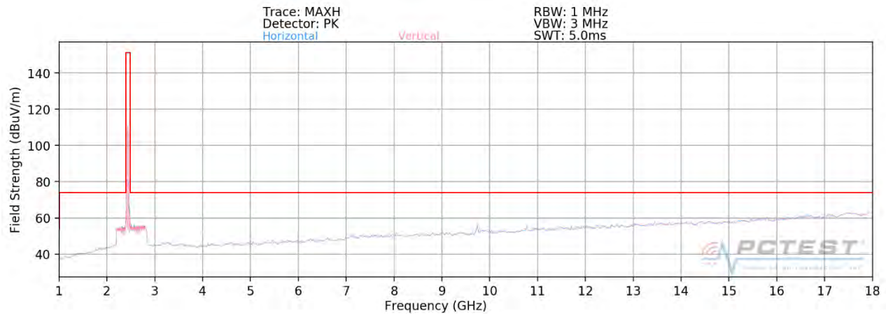
Plot 7-97. Radiated Spurious Plot above 1GHz MIMO (802.11ax OFDMA – 242 Tones – Ch. 6)
