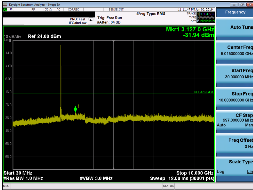
Plot 7-53. Conducted Spurious Plot SISO ANT1 (802.11ax OFDMA – 26 Tones – Ch. 1)
