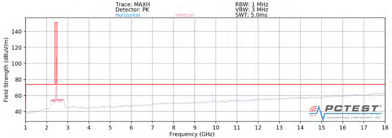
Plot 7-82. Radiated Spurious Plot above 1GHz SISO ANT1 (802.11ax OFDMA – 242 Tones – Ch. 11)
