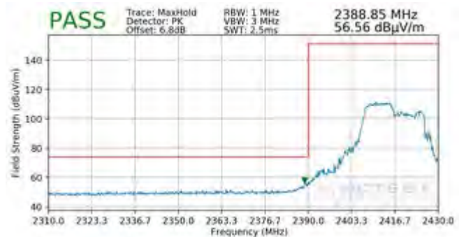
Plot 7-104. Radiated Restricted Lower Band Edge Measurement SISO ANT1 (Peak – 106 Tones)
