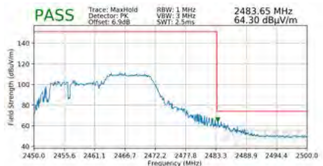
Plot 7-108. Radiated Restricted Upper Band Edge Measurement SISO ANT1 (Peak – 106 Tones)
