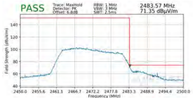
Plot 7-124. Radiated Restricted Upper Band Edge Measurement SISO ANT1 (Peak – 242 Tones)
