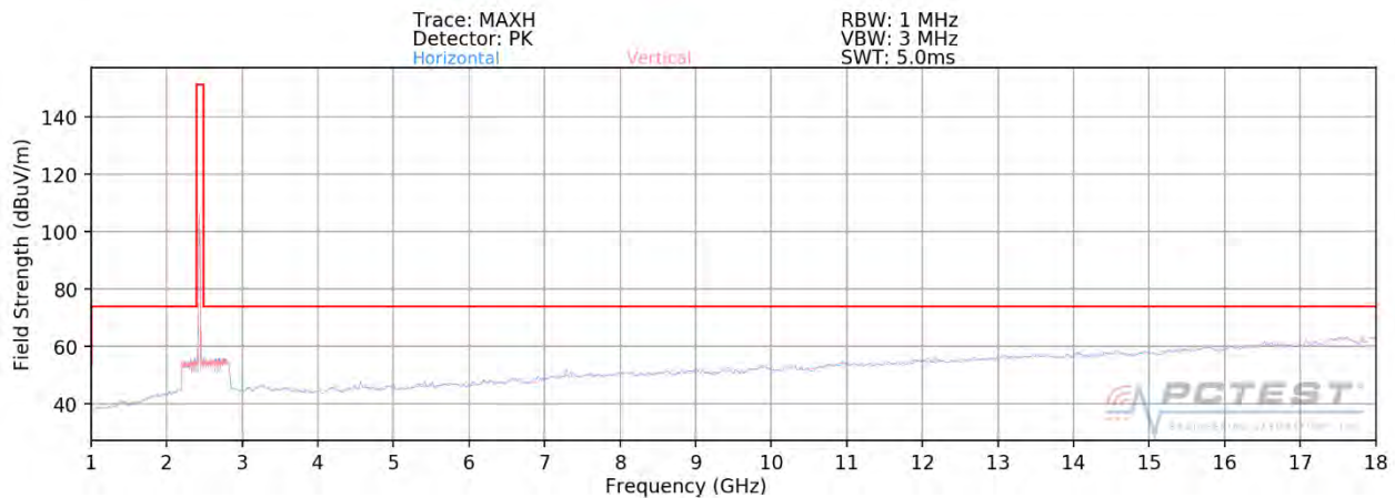
Plot 7-86. Radiated Spurious Plot above 1GHz SISO ANT2 (802.11ax OFDMA – 26 Tones – Ch. 6)
