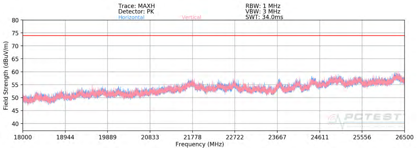
Plot 7-100. Radiated Spurious Plot above 18GHz MIMO (802.11ax OFDMA – 242 Tones)
