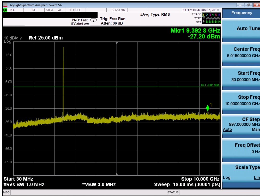
Plot 7-67. Conducted Spurious Plot SISO ANT2 (802.11ax OFDMA – 26 Tones – Ch. 6)
