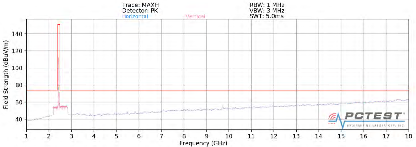
Plot 7-78. Radiated Spurious Plot above 1GHz SISO ANT1 (802.11ax OFDMA – 26 Tones – Ch. 6)
