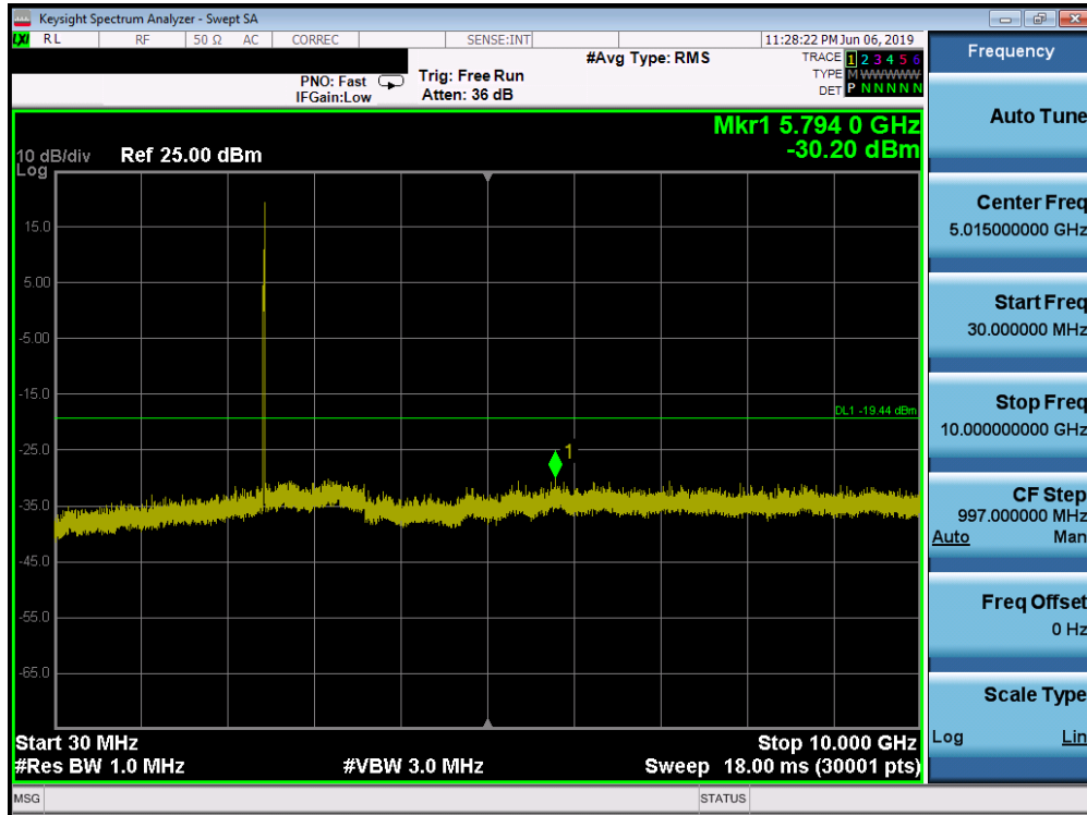
Plot 7-55. Conducted Spurious Plot SISO ANT1 (802.11ax OFDMA – 26 Tones – Ch. 6)
