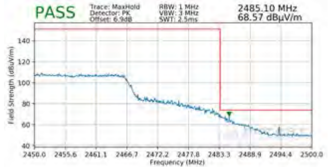
Plot 7-118. Radiated Restricted Upper Band Edge Measurement SISO ANT1 (Peak – 242 Tones)
