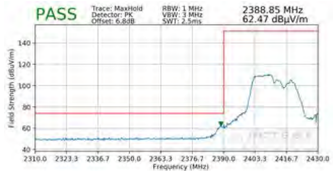
Plot 7-146. Radiated Restricted Lower Band Edge Measurement MIMO (Peak – 106 Tones)
