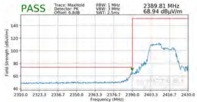
Plot 7-102. Radiated Restricted Lower Band Edge Measurement SISO ANT1 (Peak – 106 Tones)
