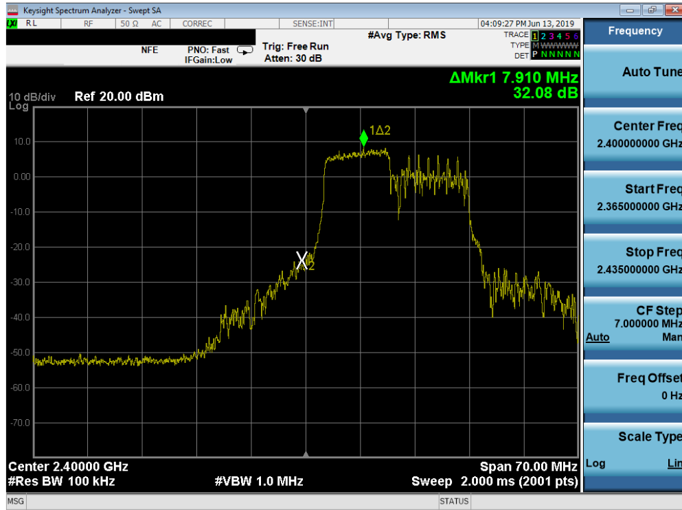
Plot 7-45. Band Edge Plot SISO ANT2 (802.11ax OFDMA - 106 Tones - Ch. 1)
