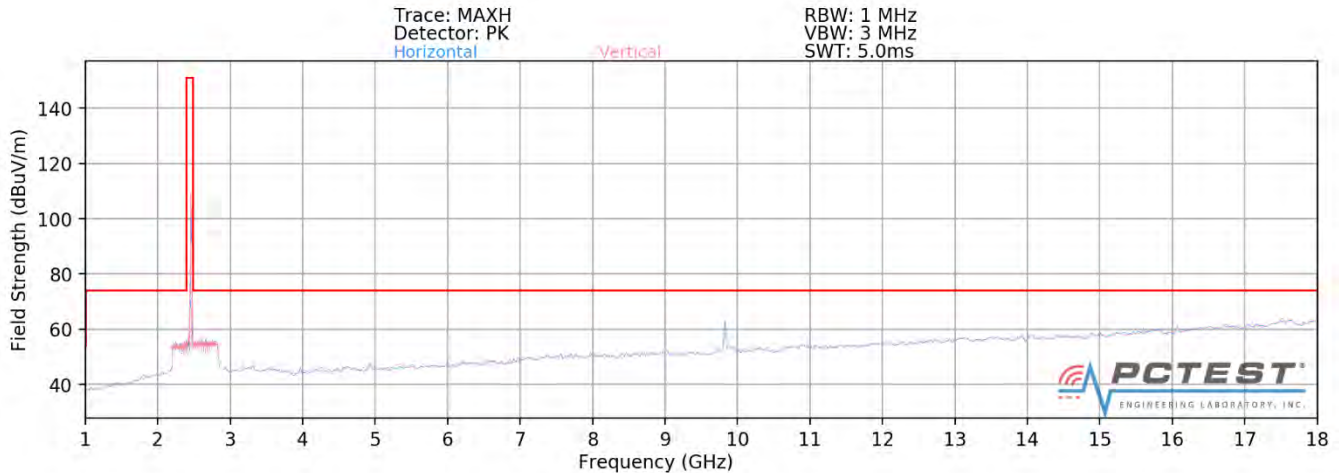
Plot 7-79. Radiated Spurious Plot above 1GHz SISO ANT1 (802.11ax OFDMA – 26 Tones – Ch. 11)
