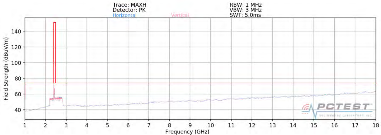
Plot 7-85. Radiated Spurious Plot above 1GHz SISO ANT2 (802.11ax OFDMA – 26 Tones – Ch. 1)
