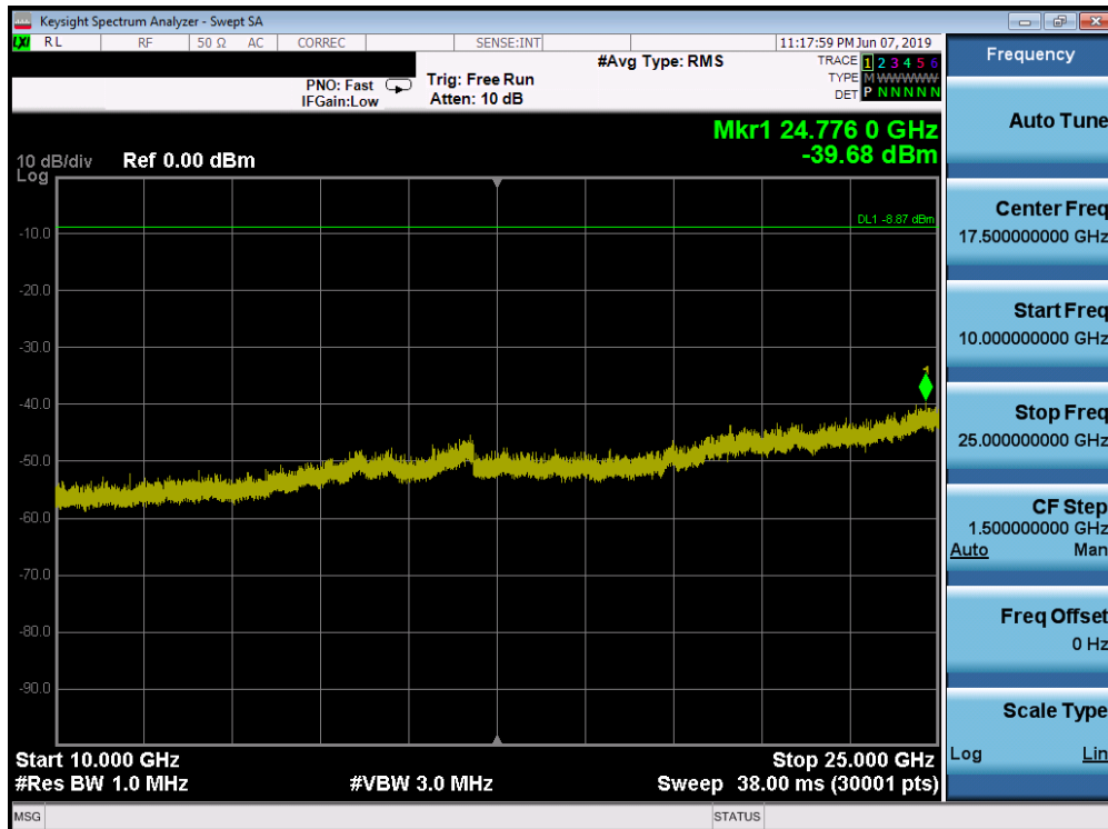
Plot 7-68. Conducted Spurious Plot SISO ANT2 (802.11ax OFDMA – 26 Tones – Ch. 6)
