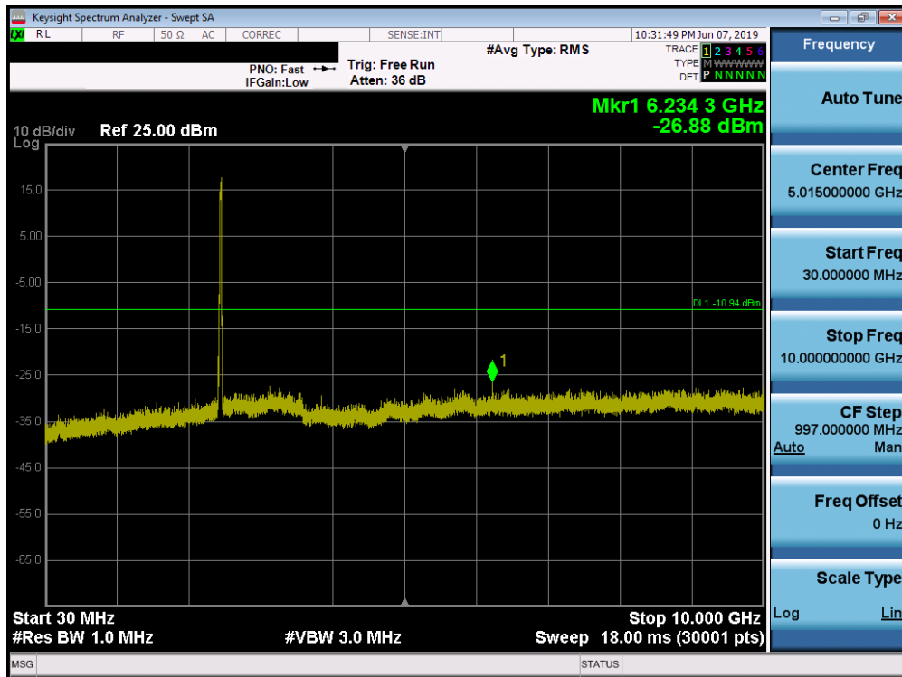
Plot 7-63. Conducted Spurious Plot SISO ANT1 (802.11ax OFDMA - 242 Tones - Ch. 11)
