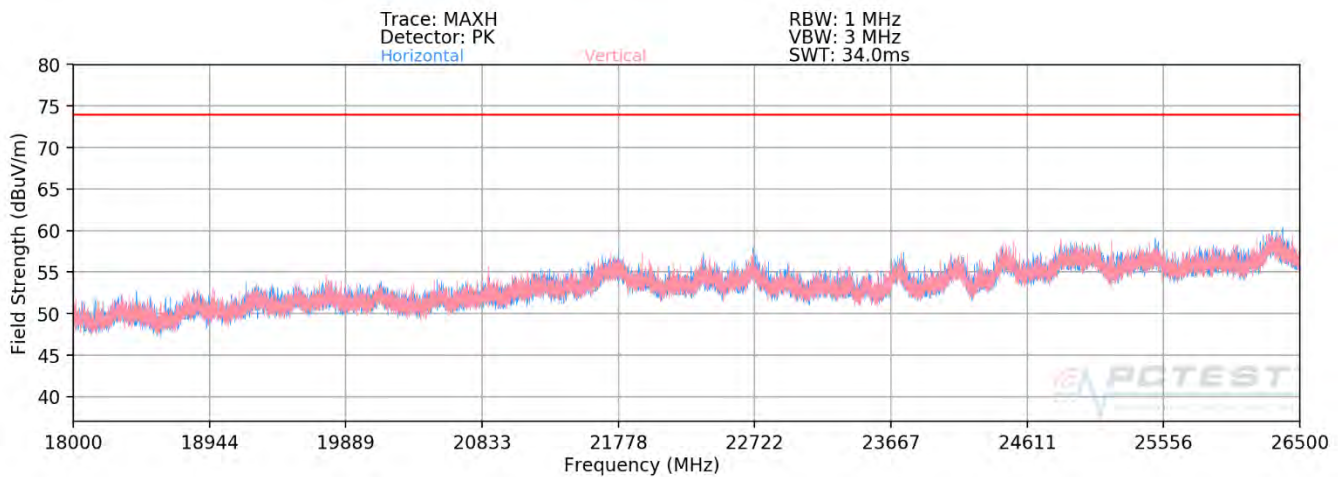
Plot 7-84. Radiated Spurious Plot above 18GHz SISO ANT1 (802.11ax OFDMA – 242 Tones)
