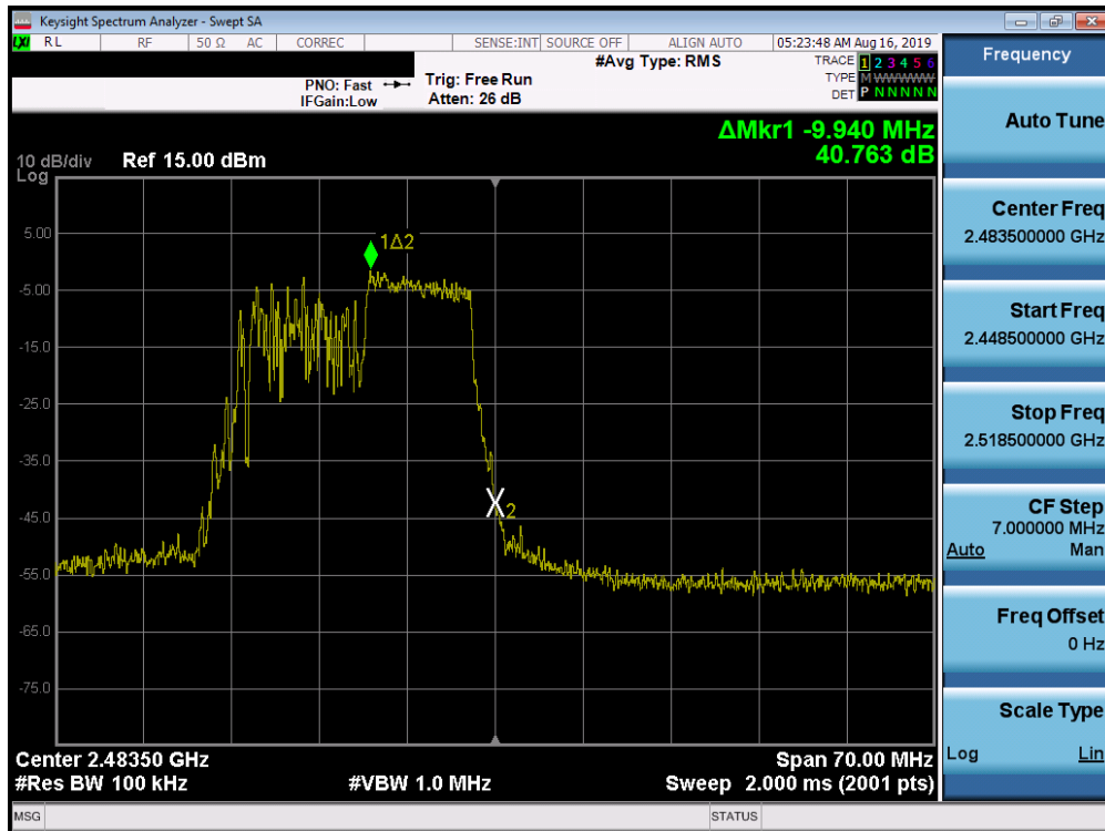
Plot 7-48. Band Edge Plot SISO ANT2 (802.11ax OFDMA - 106 Tones - Ch. 13)
