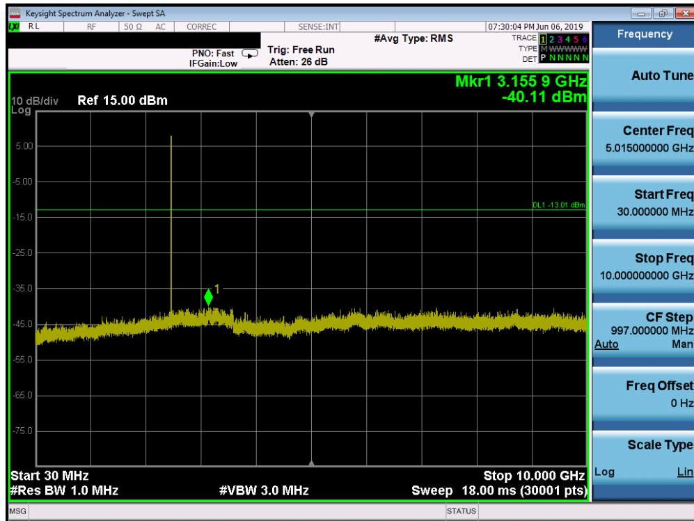
Plot 7-49. Conducted Spurious Plot (Bluetooth (LE), 2Mbps - Ch. 39)
