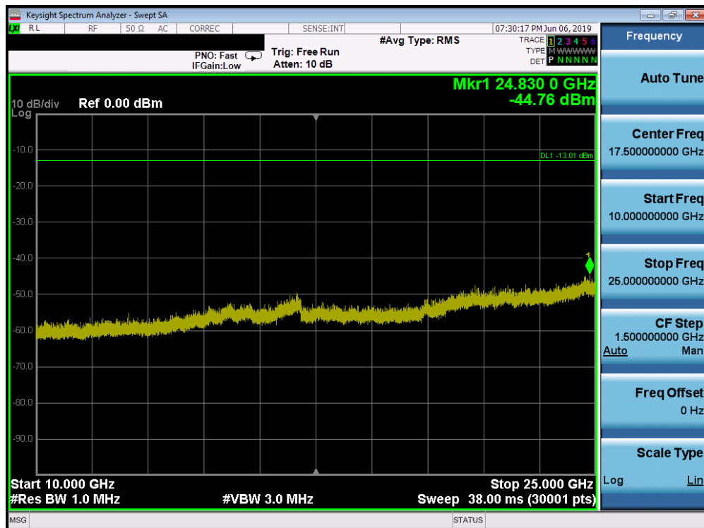
Plot 7-50. Conducted Spurious Plot (Bluetooth (LE), 2Mbps - Ch. 39)
