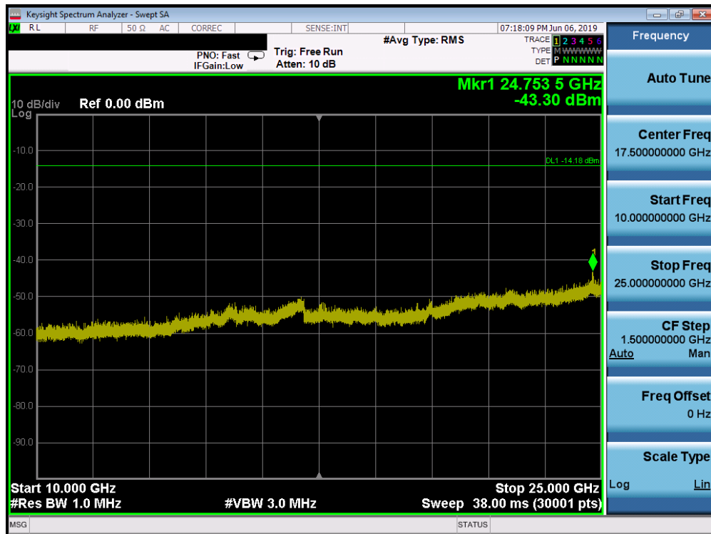
Plot 7-46. Conducted Spurious Plot (Bluetooth (LE), 2Mbps - Ch. 0)
