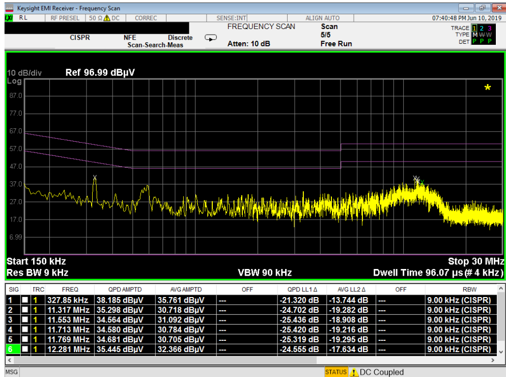
Plot 7-56. Line Conducted Plot with Bluetooth LE with WCP (N)
