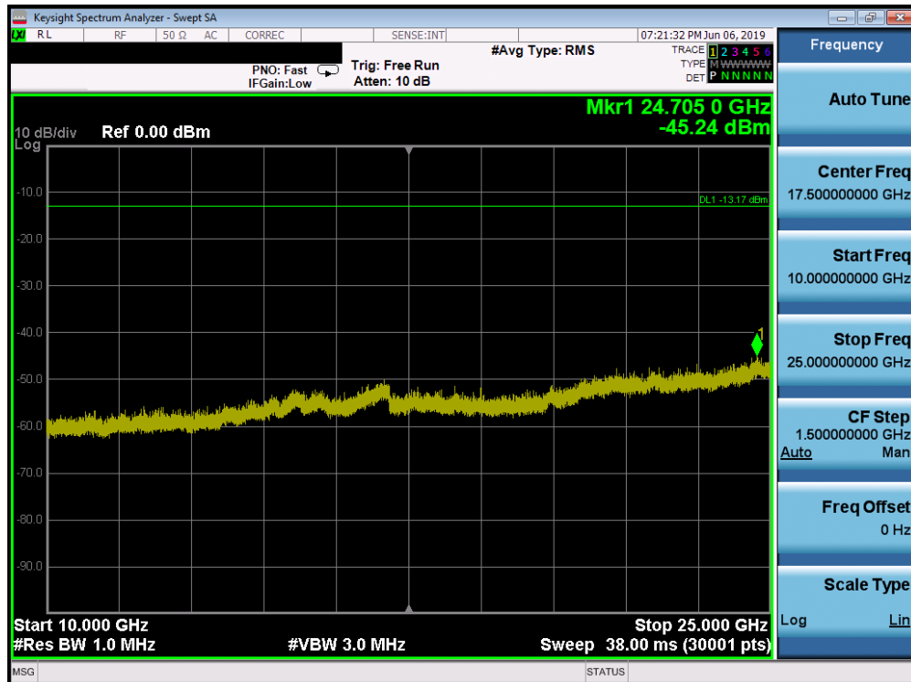
Plot 7-48. Conducted Spurious Plot (Bluetooth (LE), 2Mbps – Ch. 19)
