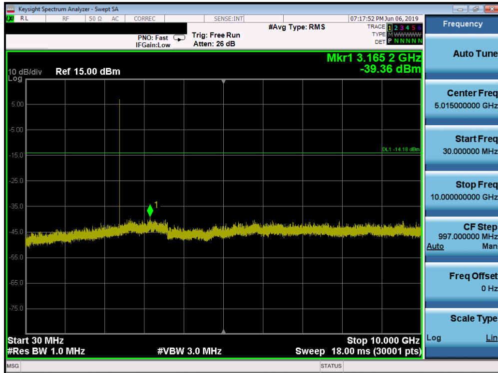
Plot 7-45. Conducted Spurious Plot (Bluetooth (LE), 2Mbps - Ch. 0)
