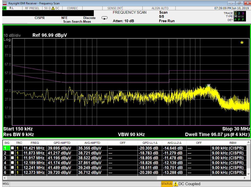
Plot 7-55. Line Conducted Plot with Bluetooth LE with WCP (L1)
