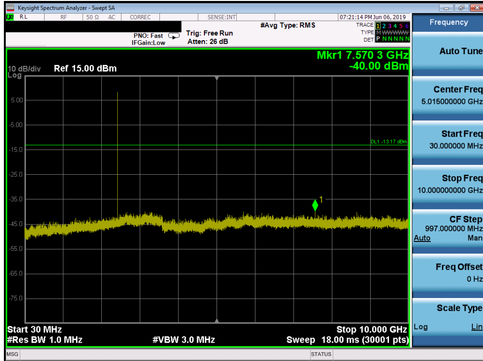
Plot 7-47. Conducted Spurious Plot (Bluetooth (LE), 2Mbps – Ch. 19)
