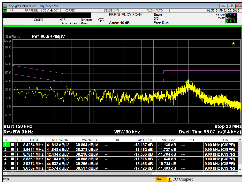
Plot 7-7. Line-Conducted Test Plot (L1) Antenna Terminated in 50 Ω
