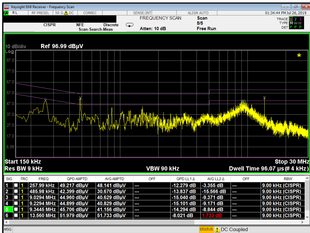
Plot 7-6. Line-Conducted Test Plot (N)
