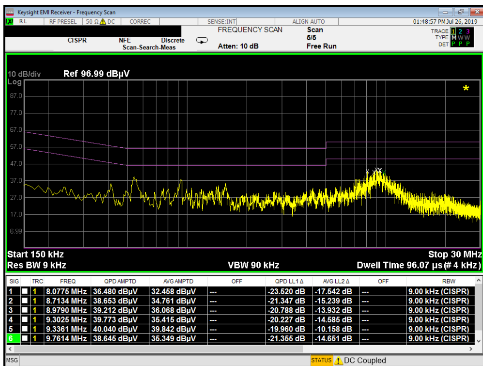
Plot 7-8. Line-Conducted Test Plot (N) Antenna Terminated in 50 Ω
