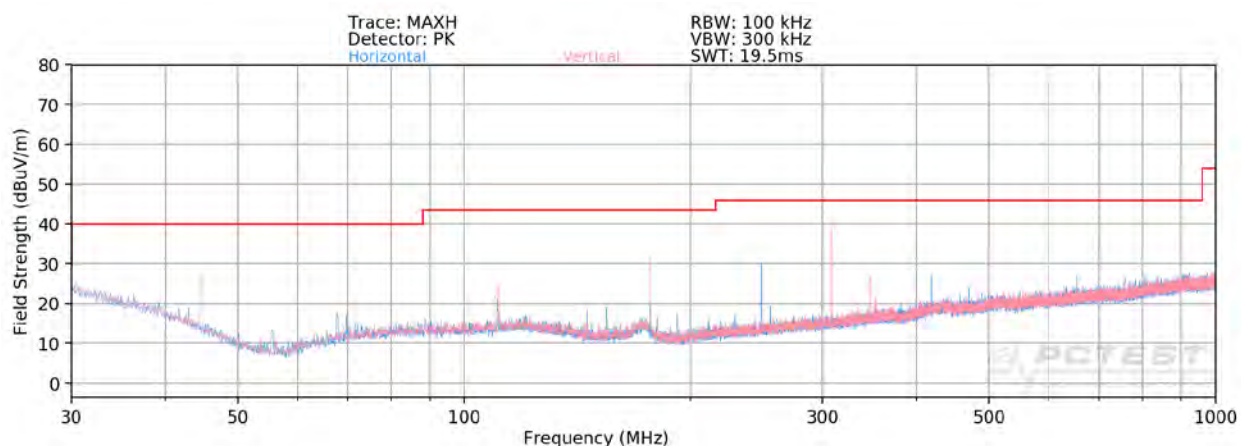
Plot 7-359. Radiated Spurious Plot below 1GHz (Dual Band Simult. Tx)
