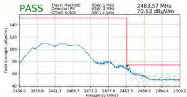
Plot 7-164. Radiated Restricted Upper Band Edge Measurement CDD (Peak)
