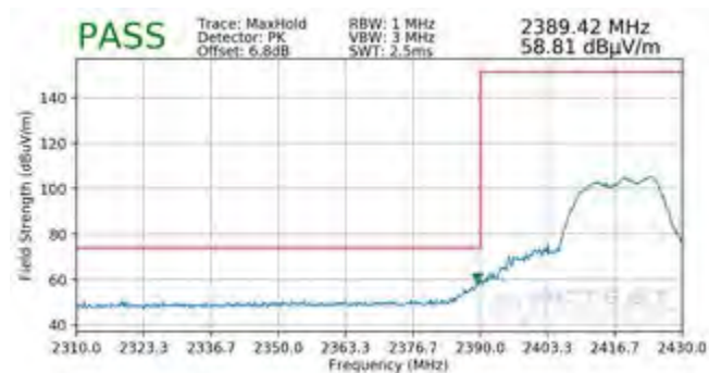
Plot 7-170. Radiated Restricted Band Edge Measurement CDD with WCP (Peak)
