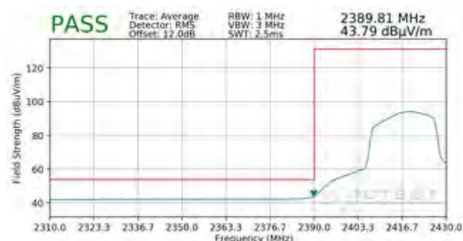
Plot 7-133. Radiated Restricted Lower Band Edge Measurement SISO ANT2 (Average)
