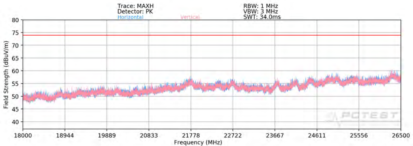
Plot 7-114. Radiated Spurious Plot above 18GHz SISO ANT2
