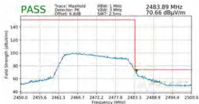
Plot 7-142. Radiated Restricted Upper Band Edge Measurement SISO ANT2 (Peak)
