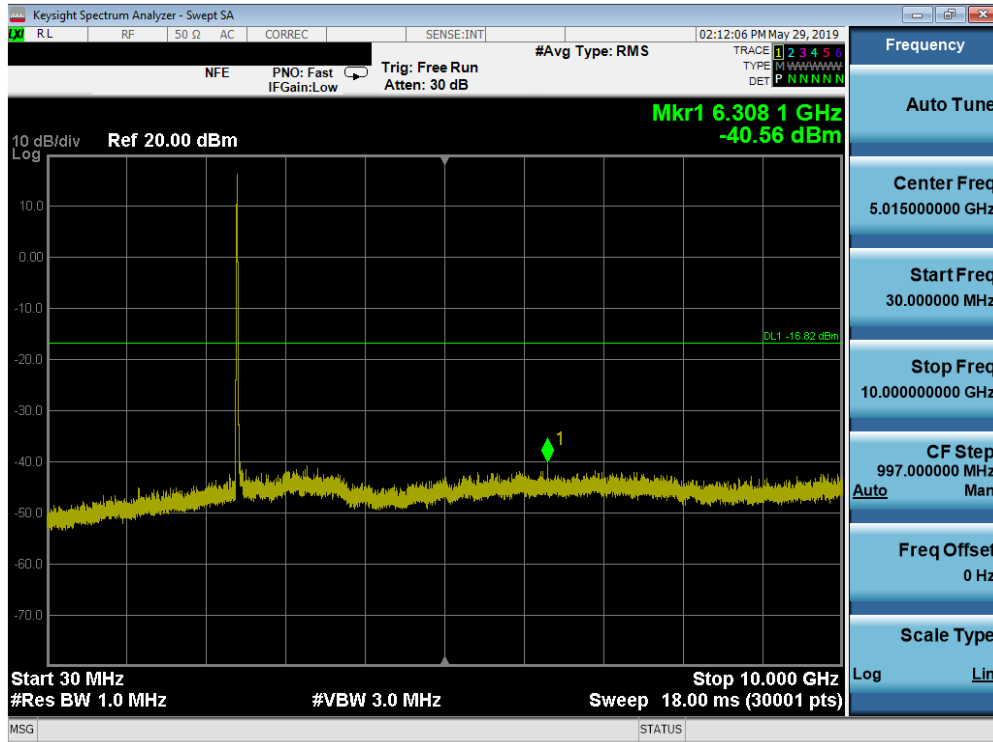
Plot 7-95. Conducted Spurious Plot SISO ANT1 (802.11b - Ch. 1)
