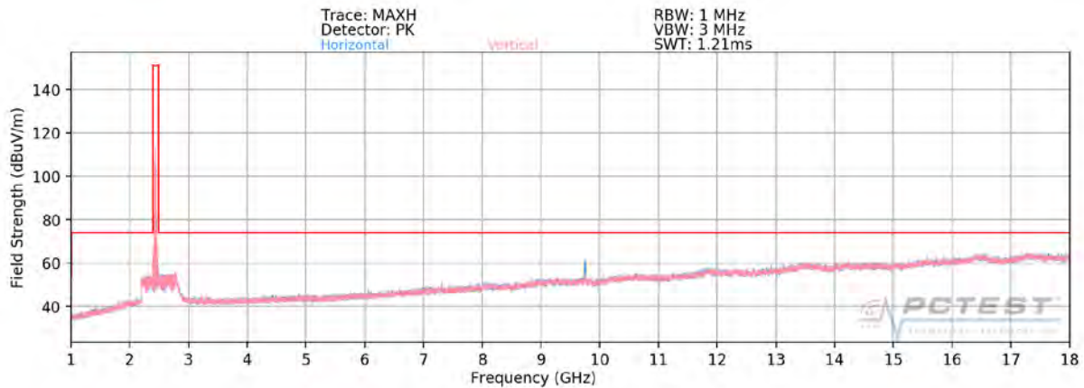
Plot 7-116. Radiated Spurious Plot above 1GHz MIMO/CDD (802.11g – Ch. 6)
