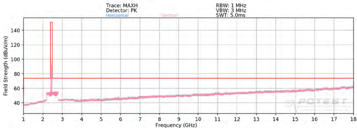
Plot 7-108. Radiated Spurious Plot above 1GHz SISO ANT1 (802.11b – Ch. 6)
