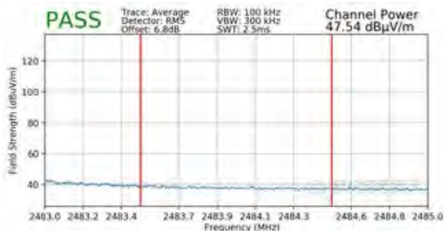
Plot 7-153. Radiated Restricted Upper Band Edge Measurement MIMO (Average)
