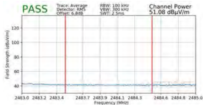
Plot 7-129. Radiated Restricted Upper Band Edge Measurement SISO ANT1 (Average)
