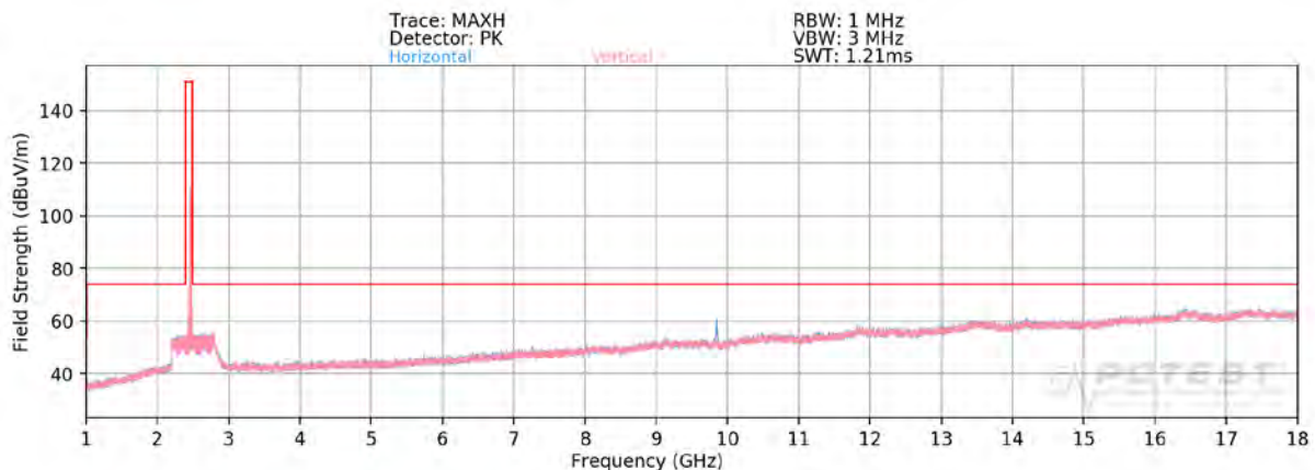
Plot 7-117. Radiated Spurious Plot above 1GHz MIMO/CDD (802.11g – Ch. 11)
