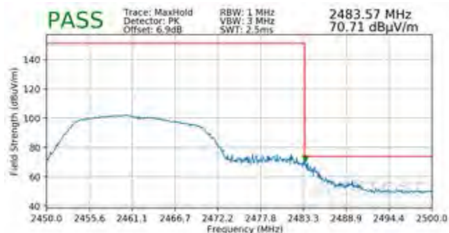
Plot 7-138. Radiated Restricted Upper Band Edge Measurement SISO ANT2 (Peak)
