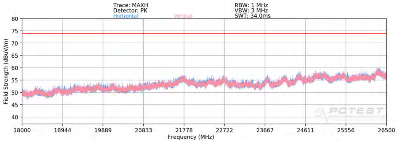
Plot 7-118. Radiated Spurious Plot above 18GHz MIMO/CDD
