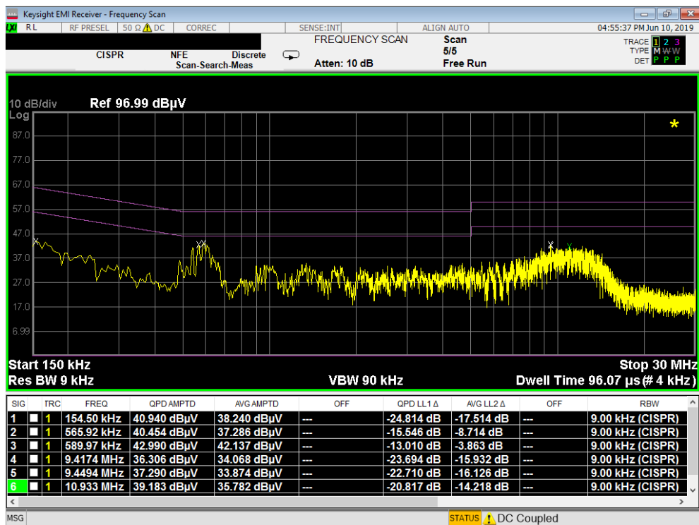
Plot 7-172. Line Conducted Plot with 802.11b (L1) with Travel Adapter
