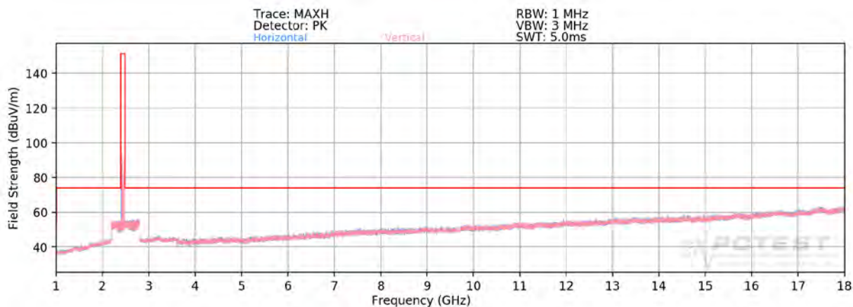
Plot 7-107. Radiated Spurious Plot above 1GHz SISO ANT1 (802.11b – Ch. 1)
