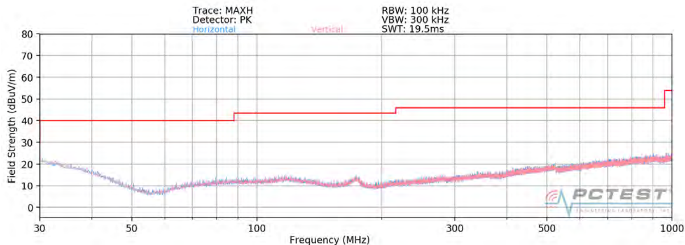
Plot 7-171. Radiated Spurious Plot below 1GHz MIMO
