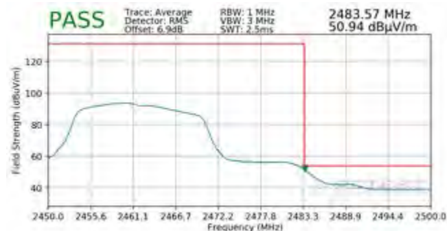
Plot 7-137. Radiated Restricted Upper Band Edge Measurement SISO ANT2 (Average)
