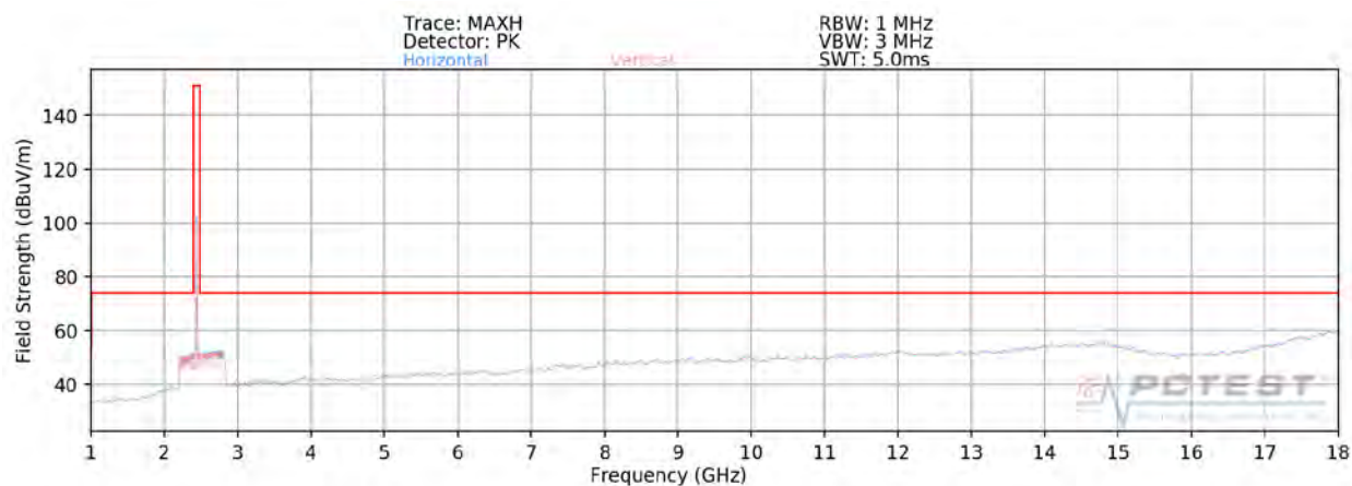
Plot 7-112. Radiated Spurious Plot above 1GHz SISO ANT2 (802.11b – Ch. 6)
