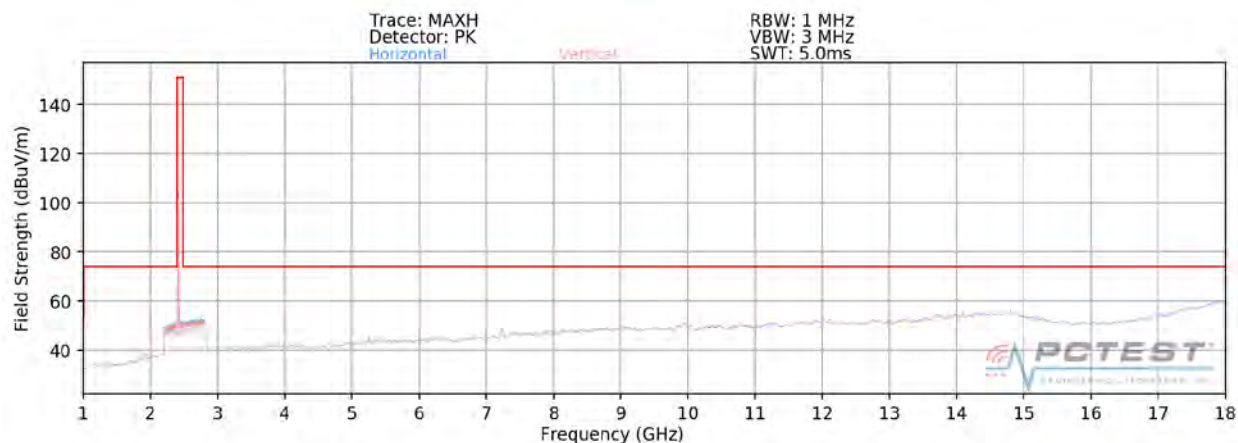
Plot 7-111. Radiated Spurious Plot above 1GHz SISO ANT2 (802.11b – Ch. 1)
