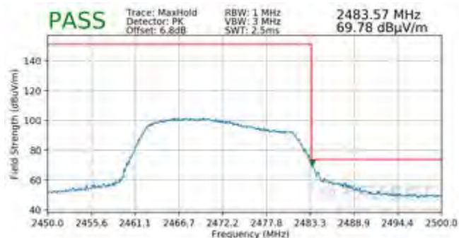
Plot 7-154. Radiated Restricted Upper Band Edge Measurement MIMO (Peak)
