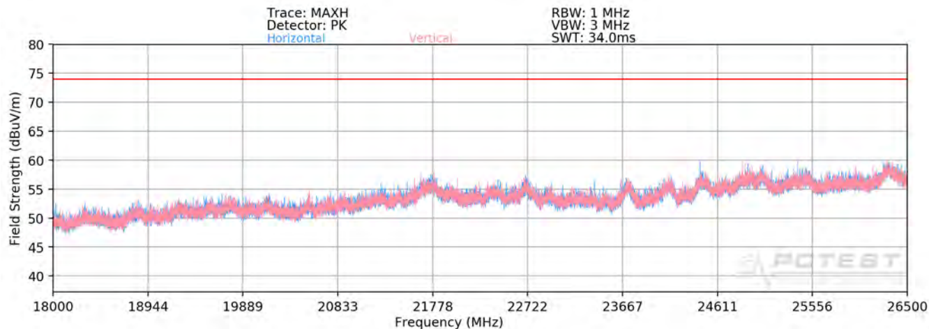
Plot 7-110. Radiated Spurious Plot above 18GHz SISO ANT1
