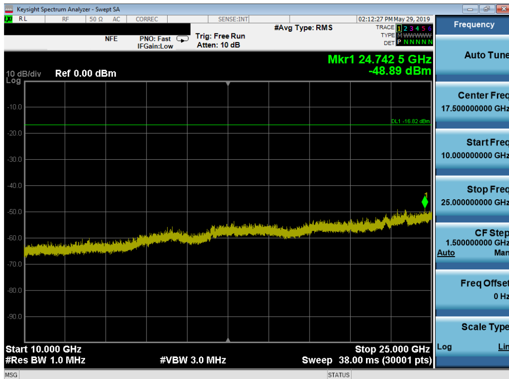
Plot 7-96. Conducted Spurious Plot SISO ANT1 (802.11b - Ch. 1)
