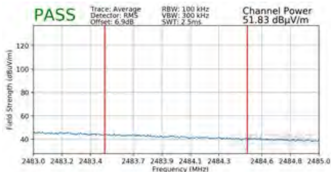
Plot 7-123. Radiated Restricted Upper Band Edge Measurement SISO ANT1 (Average)
