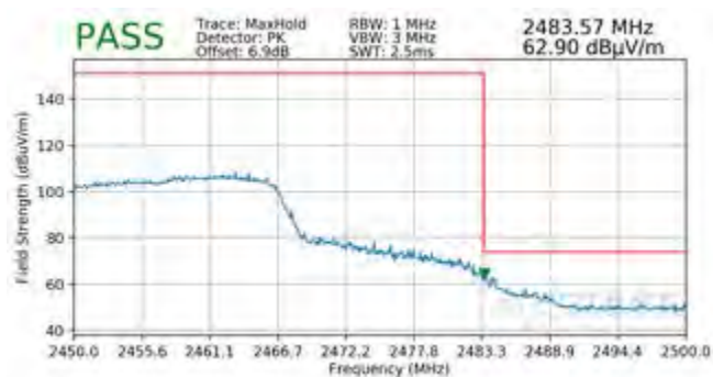
Plot 7-156. Radiated Restricted Band Edge Measurement MIMO with WCP (Peak)
