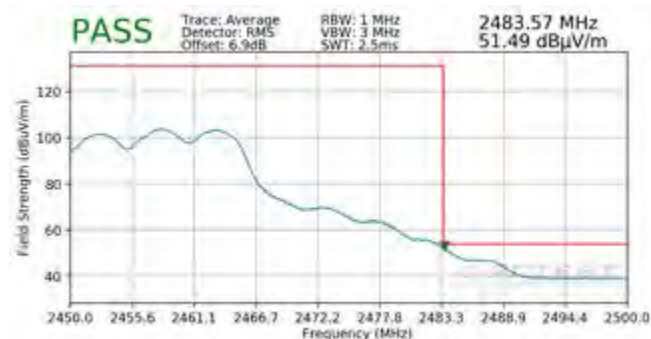
Plot 7-161. Radiated Restricted Upper Band Edge Measurement CDD (Average)
