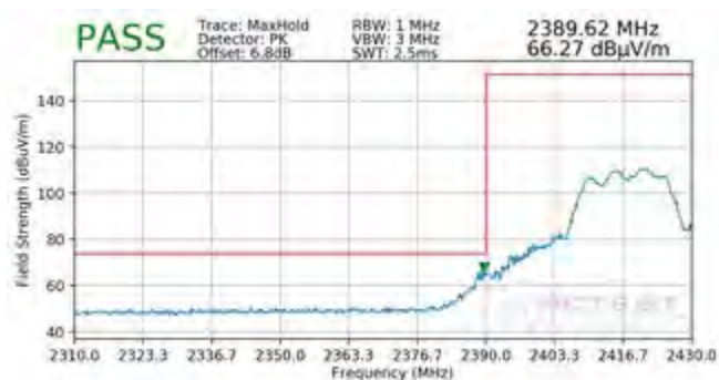
Plot 7-160. Radiated Restricted Lower Band Edge Measurement CDD (Peak)
