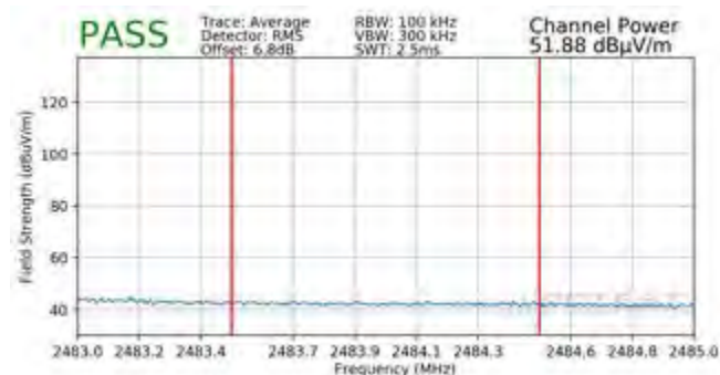
Plot 7-141. Radiated Restricted Upper Band Edge Measurement SISO ANT2 (Average)
