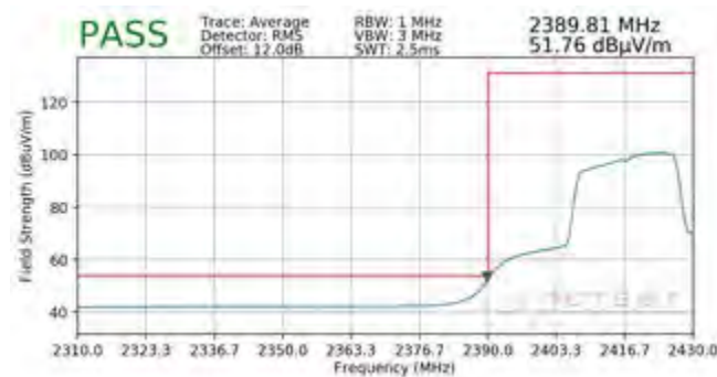
Plot 7-121. Radiated Restricted Lower Band Edge Measurement SISO ANT1 (Average)
