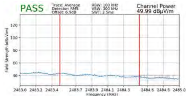
Plot 7-163. Radiated Restricted Upper Band Edge Measurement CDD (Average)
