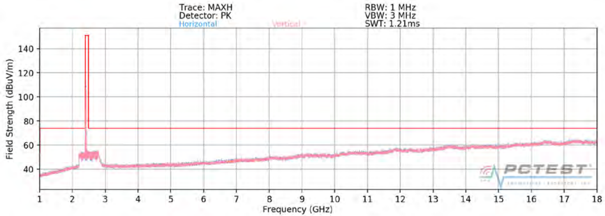
Plot 7-115. Radiated Spurious Plot above 1GHz MIMO/CDD (802.11g – Ch. 1)
