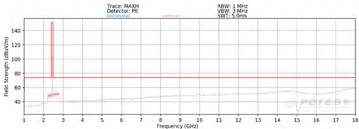
Plot 7-113. Radiated Spurious Plot above 1GHz SISO ANT2 (802.11b – Ch. 11)
