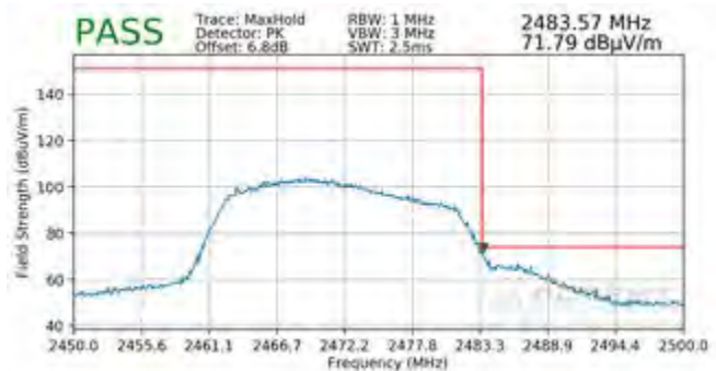
Plot 7-130. Radiated Restricted Upper Band Edge Measurement SISO ANT1 (Peak)
