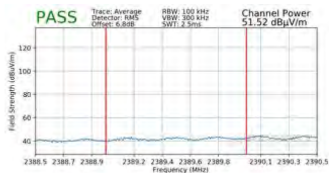
Plot 7-159. Radiated Restricted Lower Band Edge Measurement CDD (Average)
