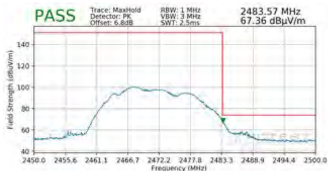
Plot 7-168. Radiated Restricted Upper Band Edge Measurement CDD (Peak)
