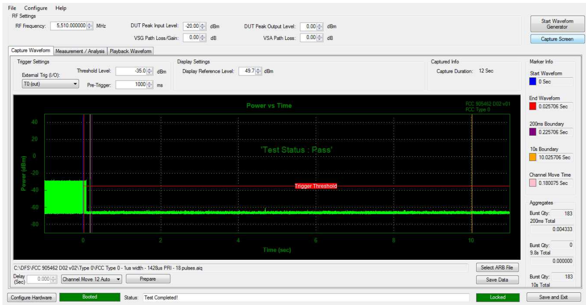
Figure 5-2. Band 2C Move Time and Aggregate Time
