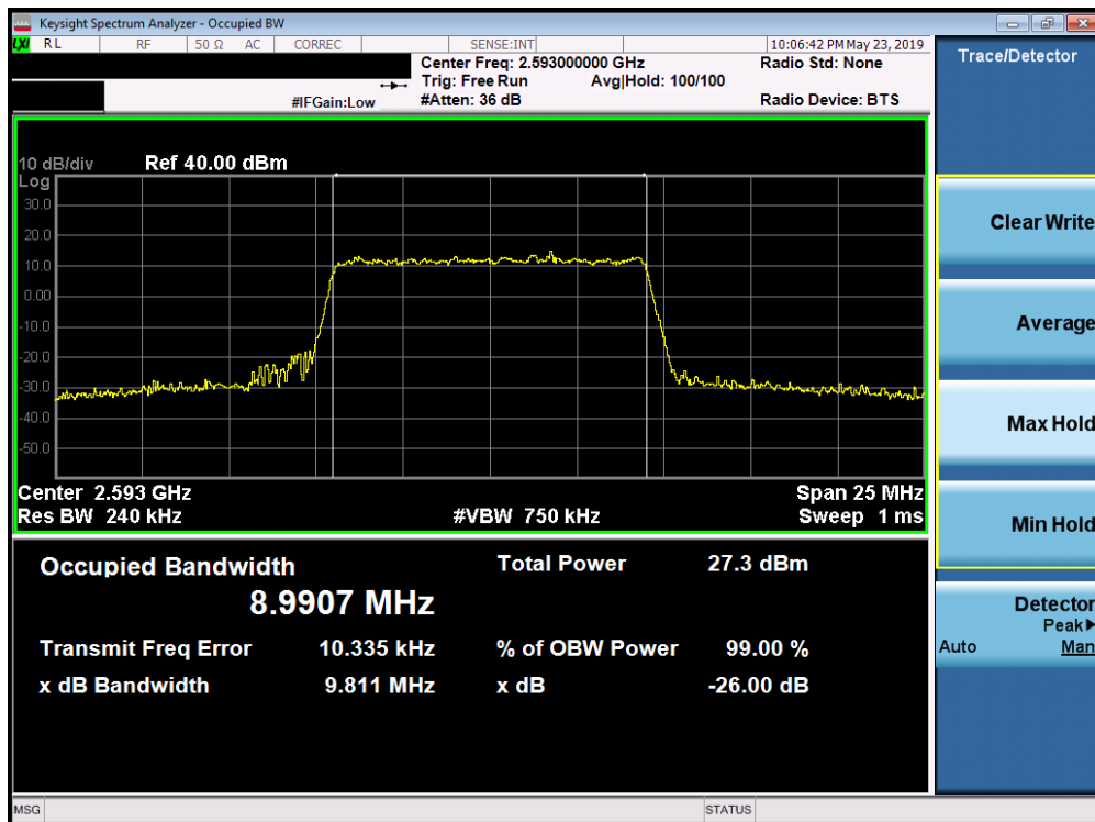
Plot 7-140. Occupied Bandwidth Plot (Band 41/38 (PC3) - 10.0MHz 256-QAM - Full RB Configuration)
