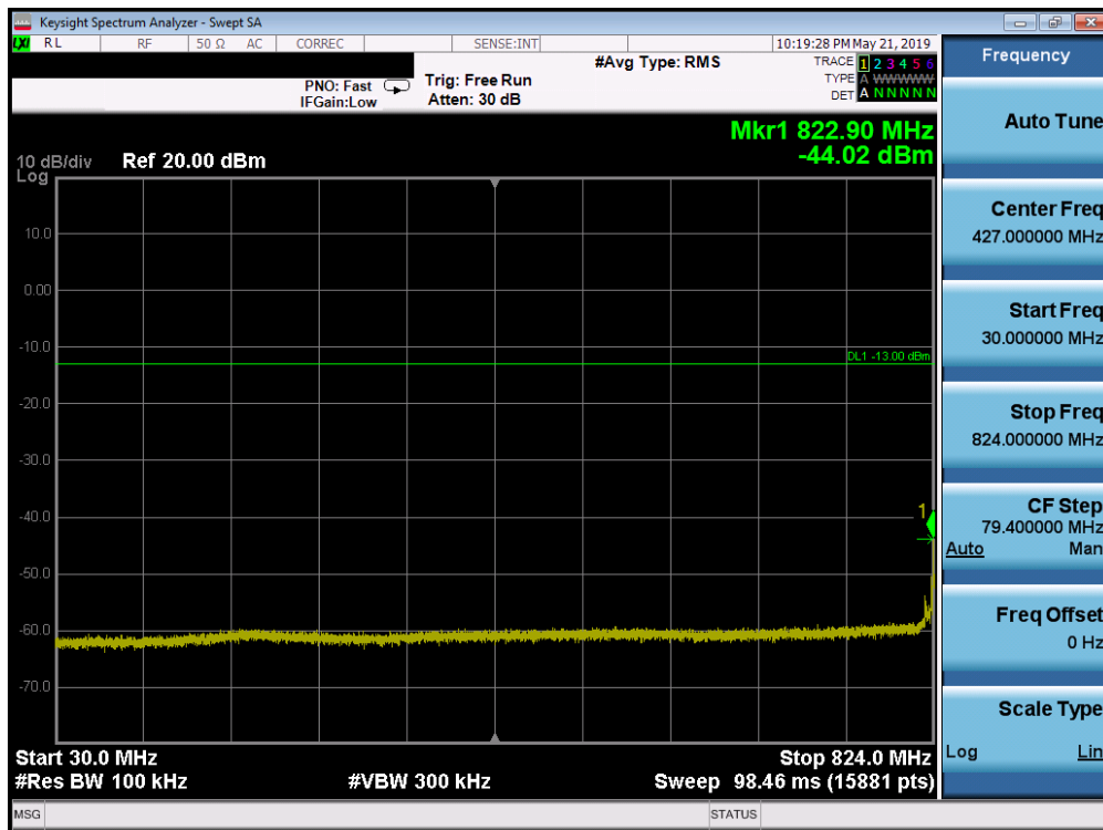
Plot 7-195. Conducted Spurious Plot (Band 26/5 - 10.0MHz QPSK - RB Size 1, RB Offset 0 - Mid Channel)
