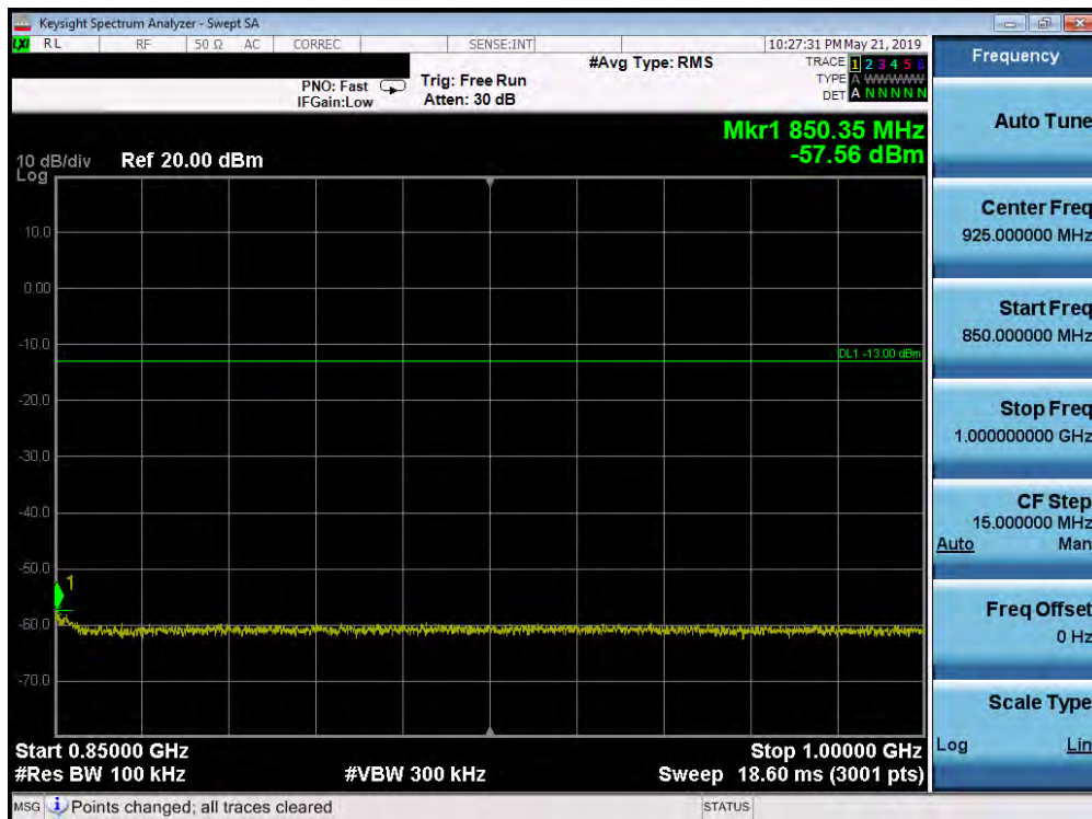
Plot 7-199. Conducted Spurious Plot (Band 26/5 - 10.0MHz QPSK - RB Size 1, RB Offset 0 - High Channel)
