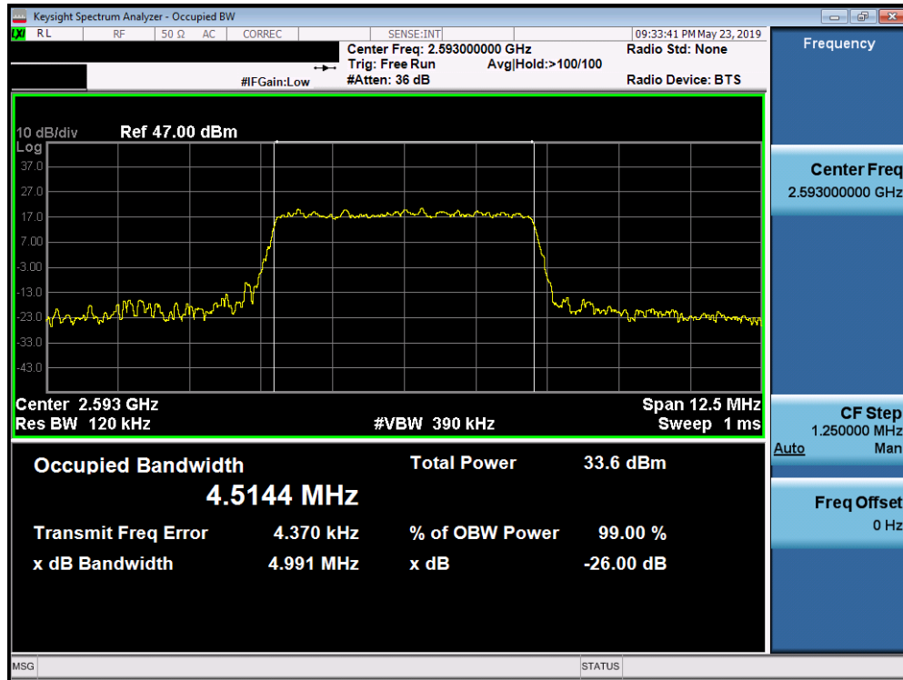
Plot 7-149. Occupied Bandwidth Plot (Band 41 (PC2) - 5.0MHz QPSK - Full RB Configuration)
