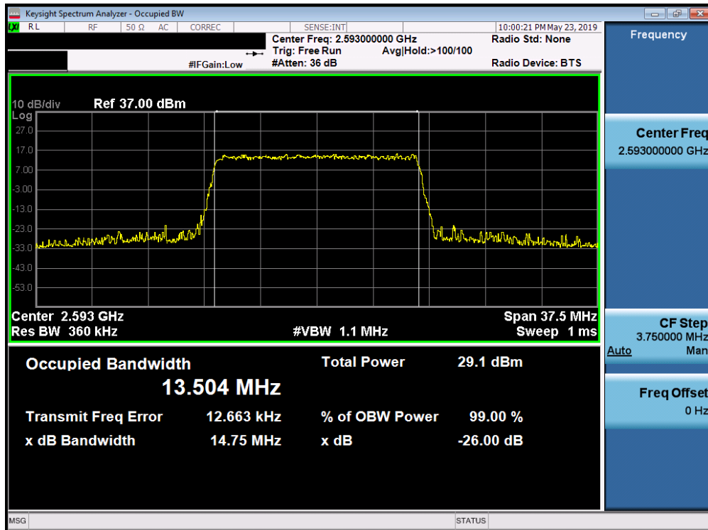
Plot 7-143. Occupied Bandwidth Plot (Band 41/38 (PC3) - 15.0MHz 64-QAM - Full RB Configuration)
