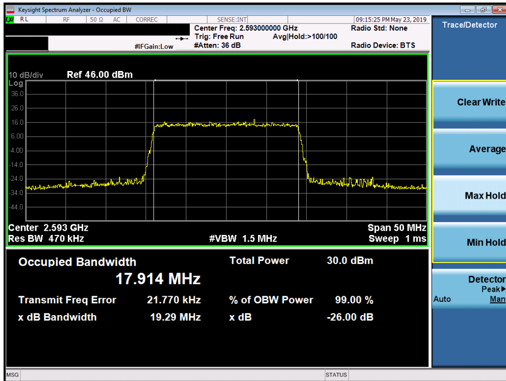
Plot 7-164. Occupied Bandwidth Plot (Band 41 (PC2) - 20.0MHz 256-QAM - Full RB Configuration)
