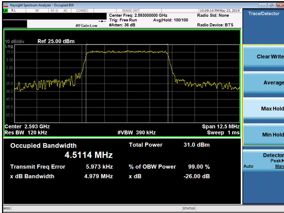
Plot 7-133. Occupied Bandwidth Plot (Band 41/38 (PC3) - 5.0MHz QPSK - Full RB Configuration)
