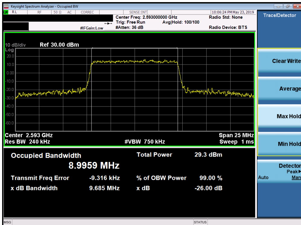
Plot 7-138. Occupied Bandwidth Plot (Band 41/38 (PC3) - 10.0MHz 16-QAM - Full RB Configuration)
