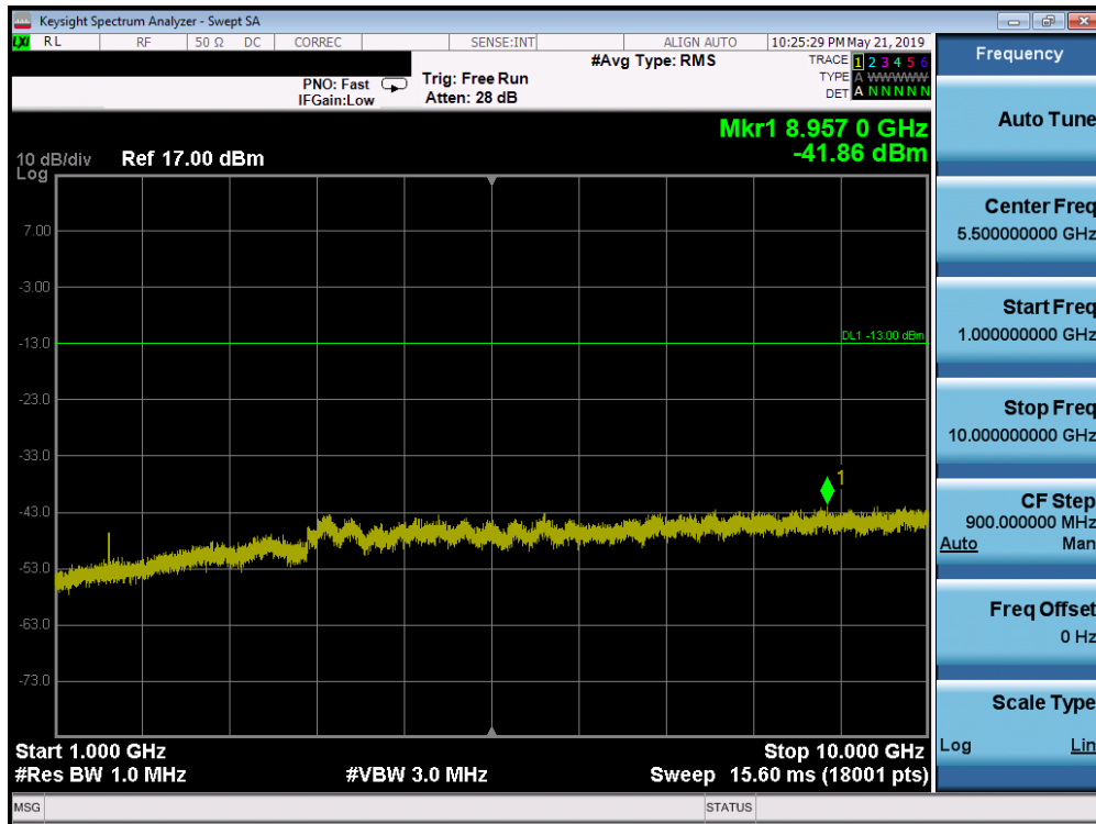
Plot 7-185. Conducted Spurious Plot (Band 13 - 5.0MHz QPSK - RB Size 1, RB Offset 0 - Low Channel)
