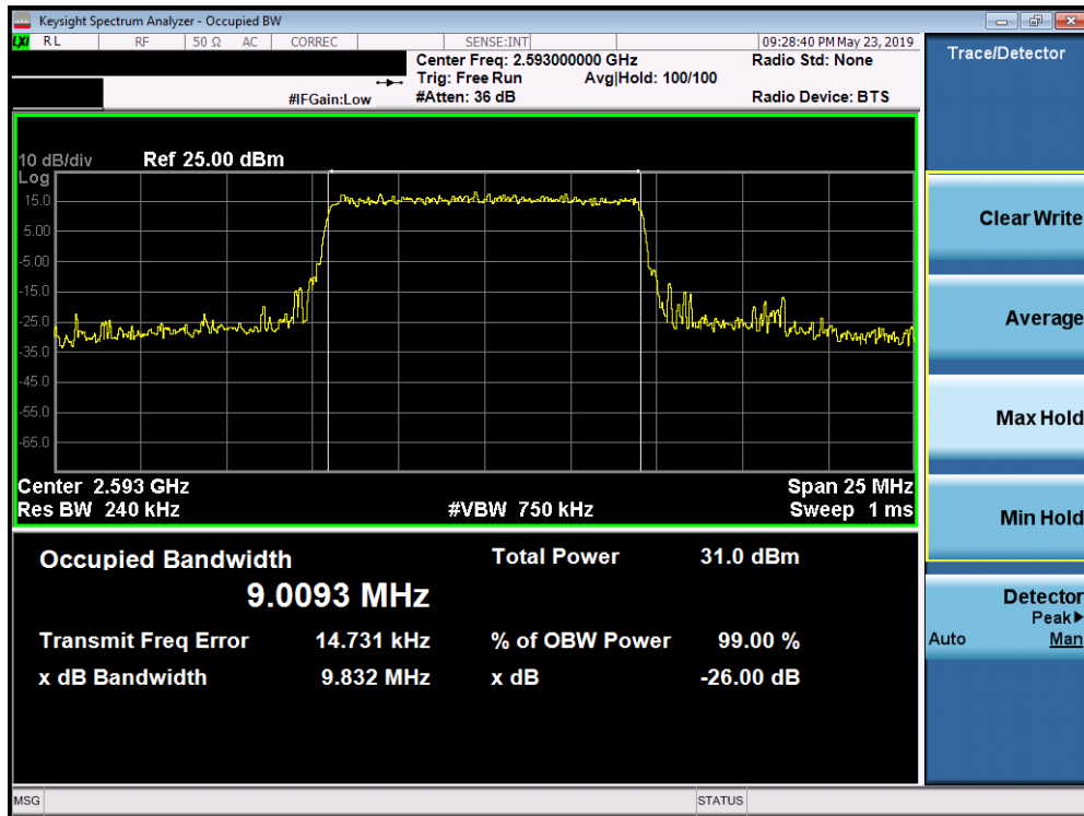
Plot 7-155. Occupied Bandwidth Plot (Band 41 (PC2) - 10.0MHz 64-QAM - Full RB Configuration)
