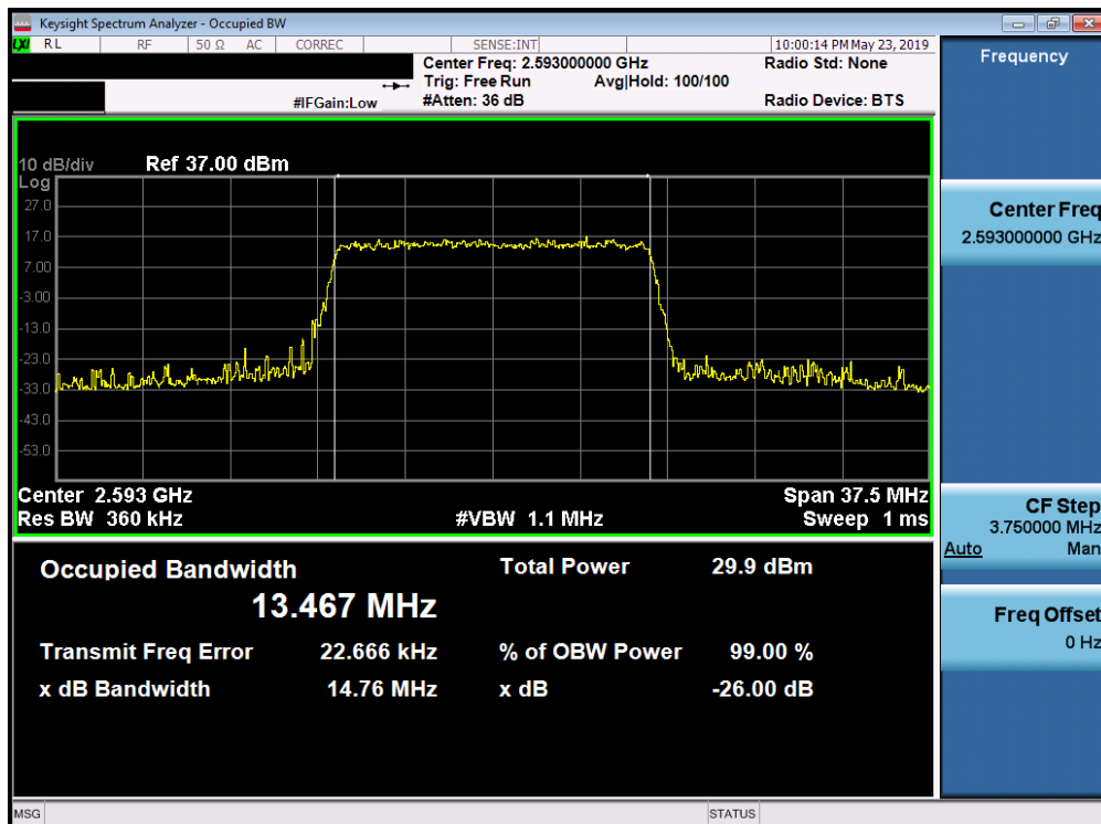
Plot 7-142. Occupied Bandwidth Plot (Band 41/38 (PC3) - 15.0MHz 16-QAM - Full RB Configuration)
