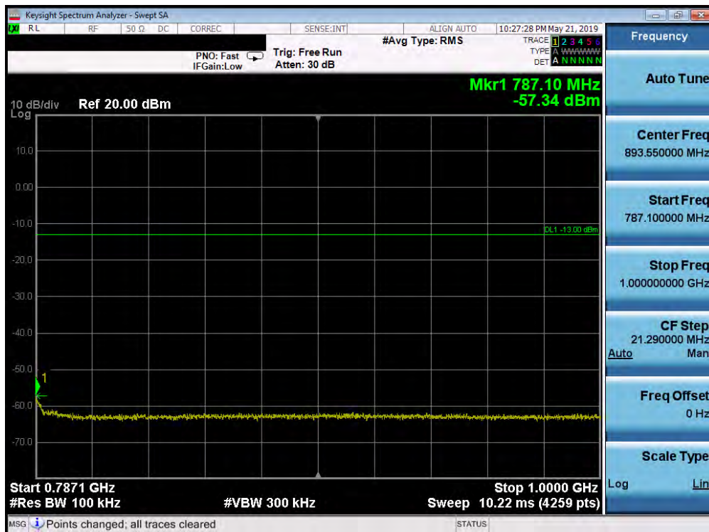
Plot 7-190. Conducted Spurious Plot (Band 13 - 5.0MHz QPSK - RB Size 1, RB Offset 0 - High Channel)
