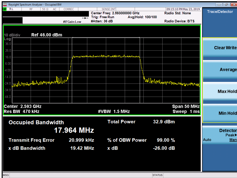
Plot 7-162. Occupied Bandwidth Plot (Band 41 (PC2) - 20.0MHz 16-QAM - Full RB Configuration)
