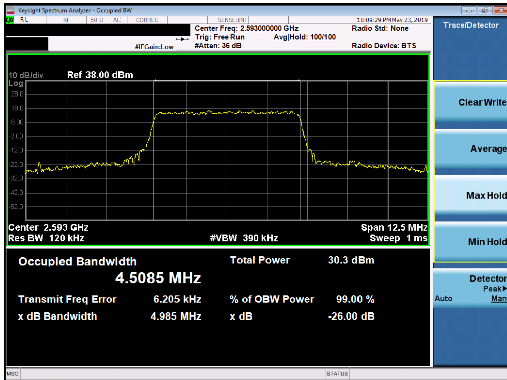
Plot 7-134. Occupied Bandwidth Plot (Band 41/38 (PC3) - 5.0MHz 16-QAM - Full RB Configuration)
