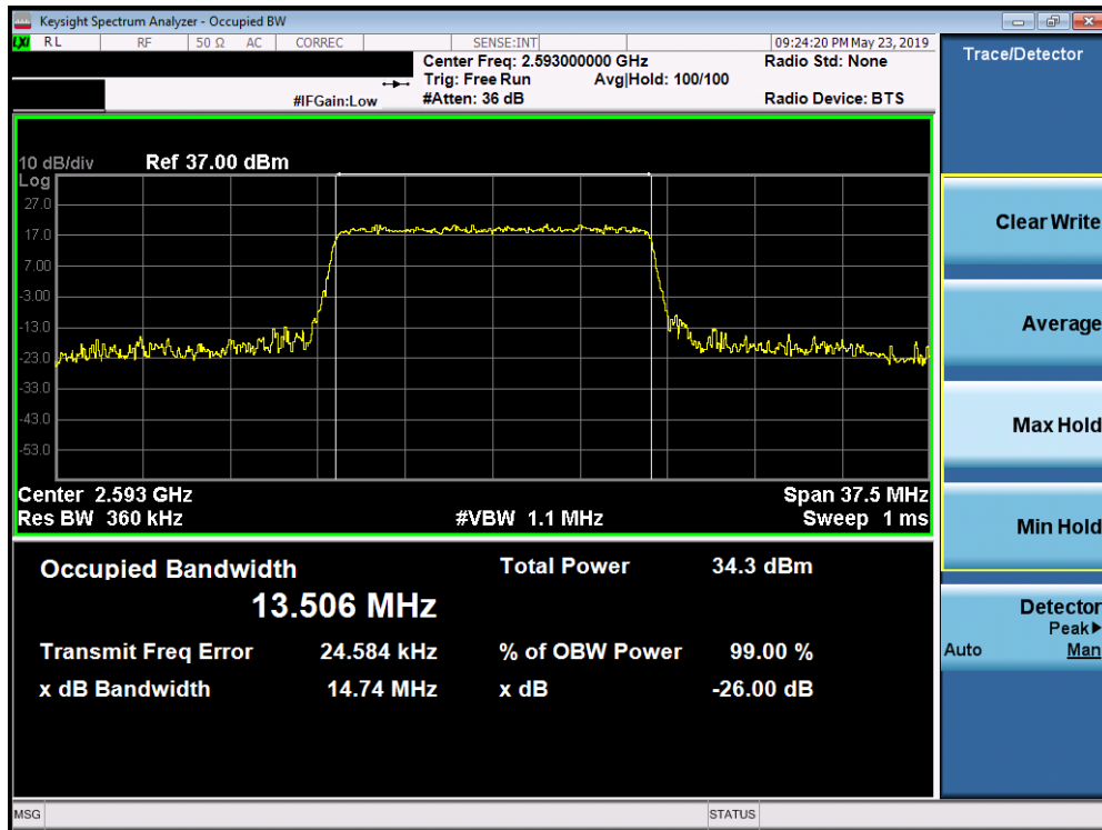
Plot 7-157. Occupied Bandwidth Plot (Band 41 (PC2) - 15.0MHz QPSK - Full RB Configuration)
