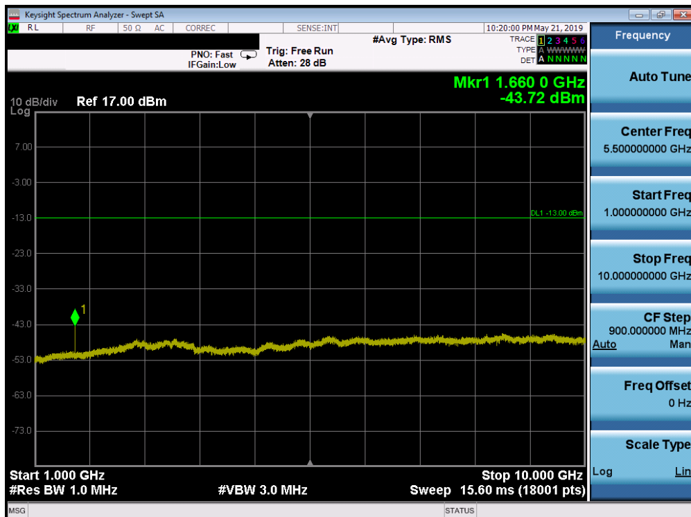
Plot 7-197. Conducted Spurious Plot (Band 26/5 - 10.0MHz QPSK - RB Size 1, RB Offset 0 - Mid Channel)
