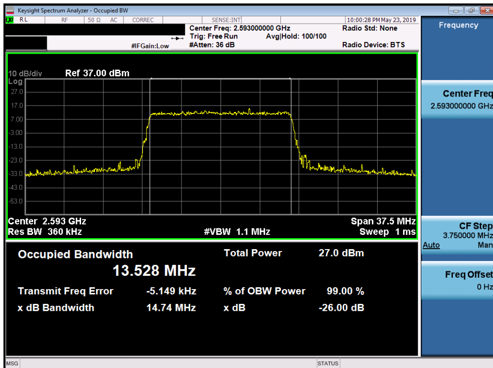
Plot 7-144. Occupied Bandwidth Plot (Band 41/38 (PC3) - 15.0MHz 256-QAM - Full RB Configuration)
