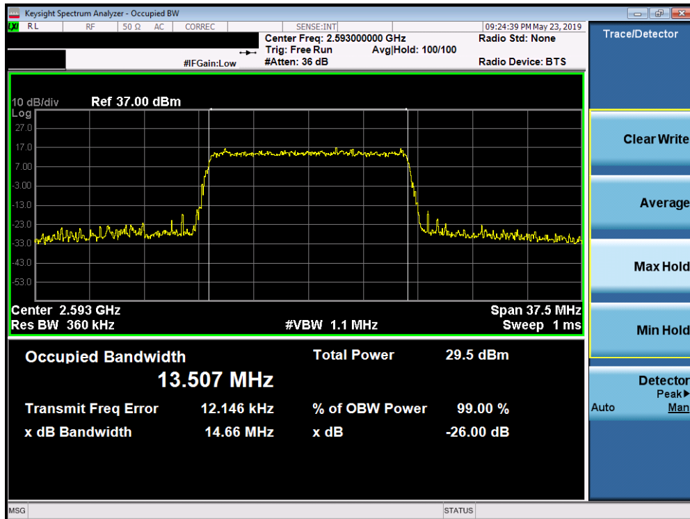
Plot 7-160. Occupied Bandwidth Plot (Band 41 (PC2) - 15.0MHz 256-QAM - Full RB Configuration)
