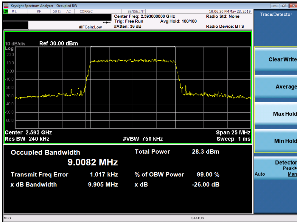
Plot 7-139. Occupied Bandwidth Plot (Band 41/38 (PC3) - 10.0MHz 64-QAM - Full RB Configuration)
