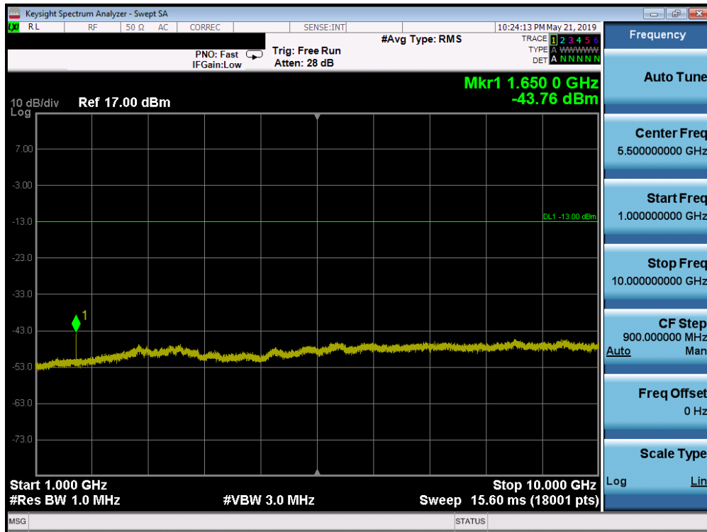
Plot 7-194. Conducted Spurious Plot (Band 26/5 - 10.0MHz QPSK - RB Size 1, RB Offset 0 - Low Channel)
