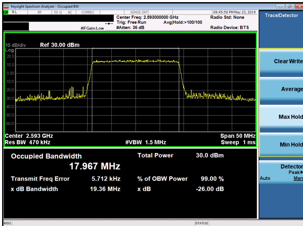
Plot 7-146. Occupied Bandwidth Plot (Band 41/38 (PC3) - 20.0MHz 16-QAM - Full RB Configuration)
