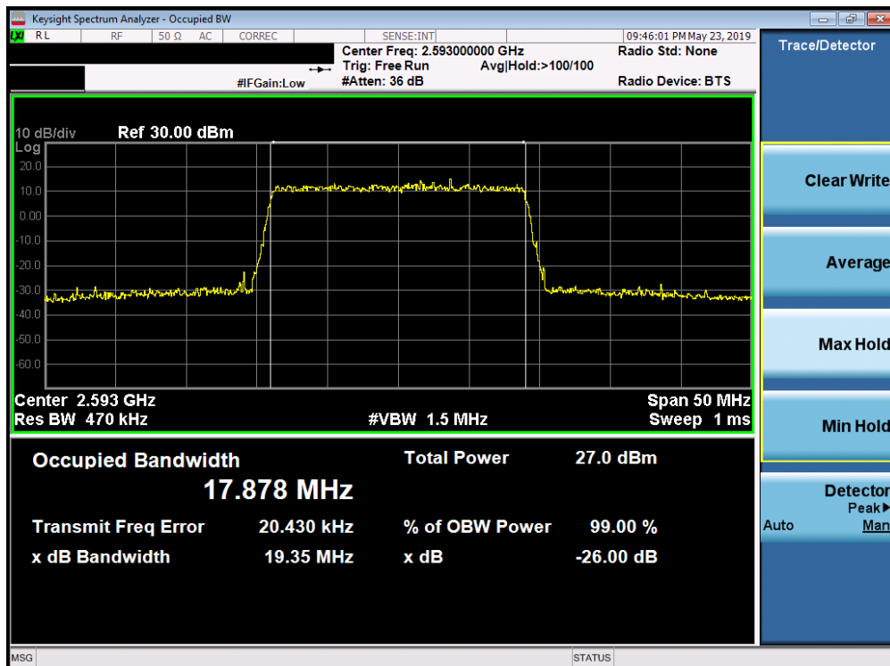
Plot 7-148. Occupied Bandwidth Plot (Band 41/38 (PC3) - 20.0MHz 256-QAM - Full RB Configuration)
