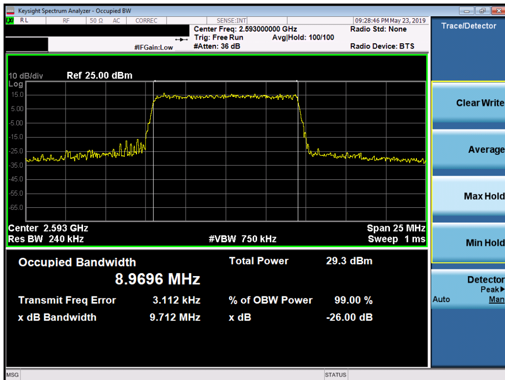
Plot 7-156. Occupied Bandwidth Plot (Band 41 (PC2) - 10.0MHz 256-QAM - Full RB Configuration)
