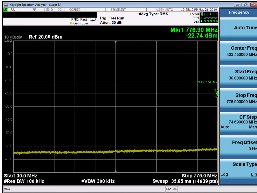
Plot 7-183. Conducted Spurious Plot (Band 13 - 5.0MHz QPSK - RB Size 1, RB Offset 0 - Low Channel)
