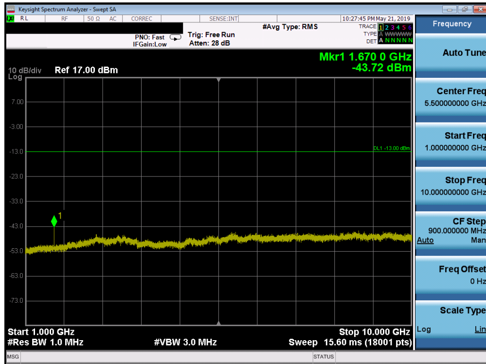
Plot 7-200. Conducted Spurious Plot (Band 26/5 - 10.0MHz QPSK - RB Size 1, RB Offset 0 - High Channel)
