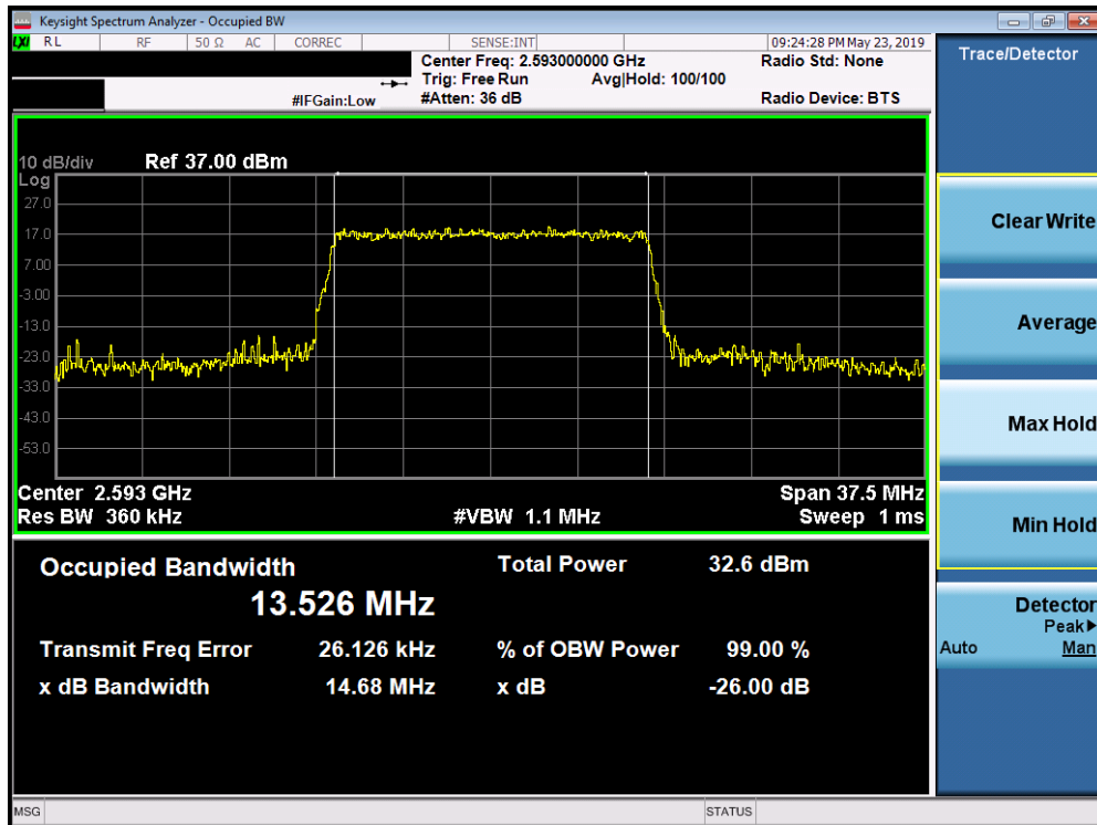
Plot 7-158. Occupied Bandwidth Plot (Band 41 (PC2) - 15.0MHz 16-QAM - Full RB Configuration)
