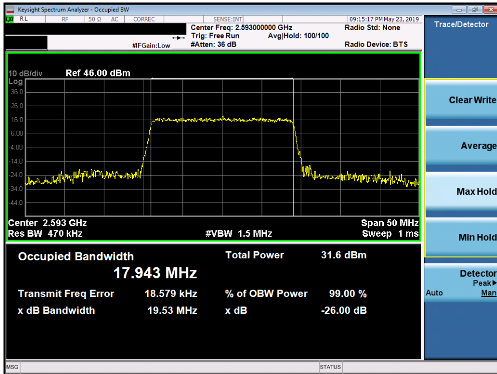
Plot 7-163. Occupied Bandwidth Plot (Band 41 (PC2) - 20.0MHz 64-QAM - Full RB Configuration)
