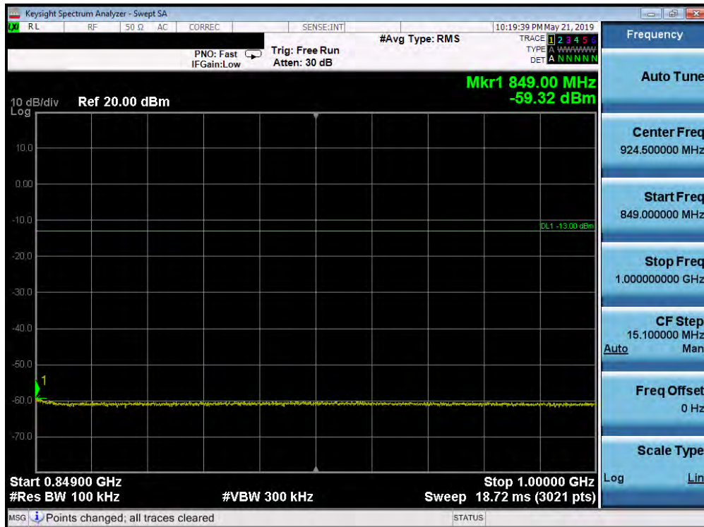
Plot 7-196. Conducted Spurious Plot (Band 26/5 - 10.0MHz QPSK - RB Size 1, RB Offset 0 - Mid Channel)
