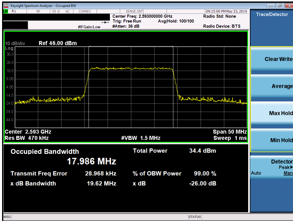
Plot 7-161. Occupied Bandwidth Plot (Band 41 (PC2) - 20.0MHz QPSK - Full RB Configuration)
