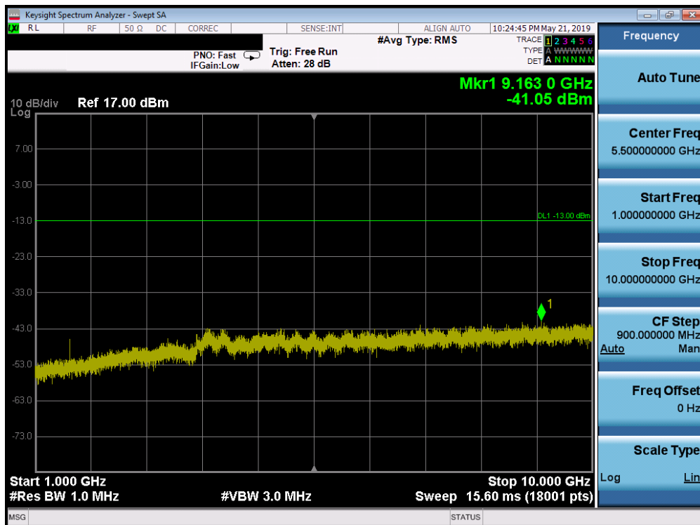
Plot 7-188. Conducted Spurious Plot (Band 13 - 5.0MHz QPSK - RB Size 1, RB Offset 0 - Mid Channel)
