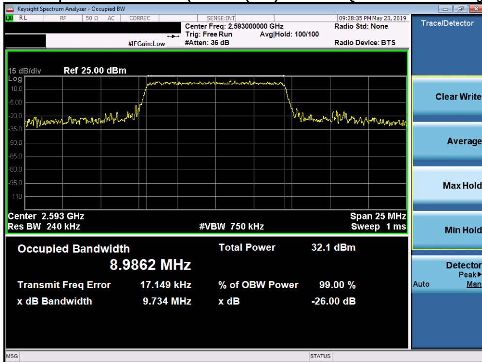
Plot 7-154. Occupied Bandwidth Plot (Band 41 (PC2) - 10.0MHz 16-QAM - Full RB Configuration)
