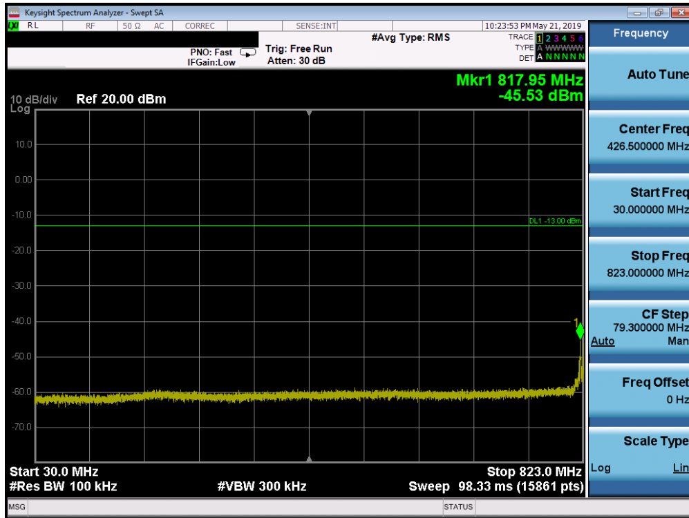
Plot 7-192. Conducted Spurious Plot (Band 26/5 - 10.0MHz QPSK - RB Size 1, RB Offset 0 - Low Channel)
