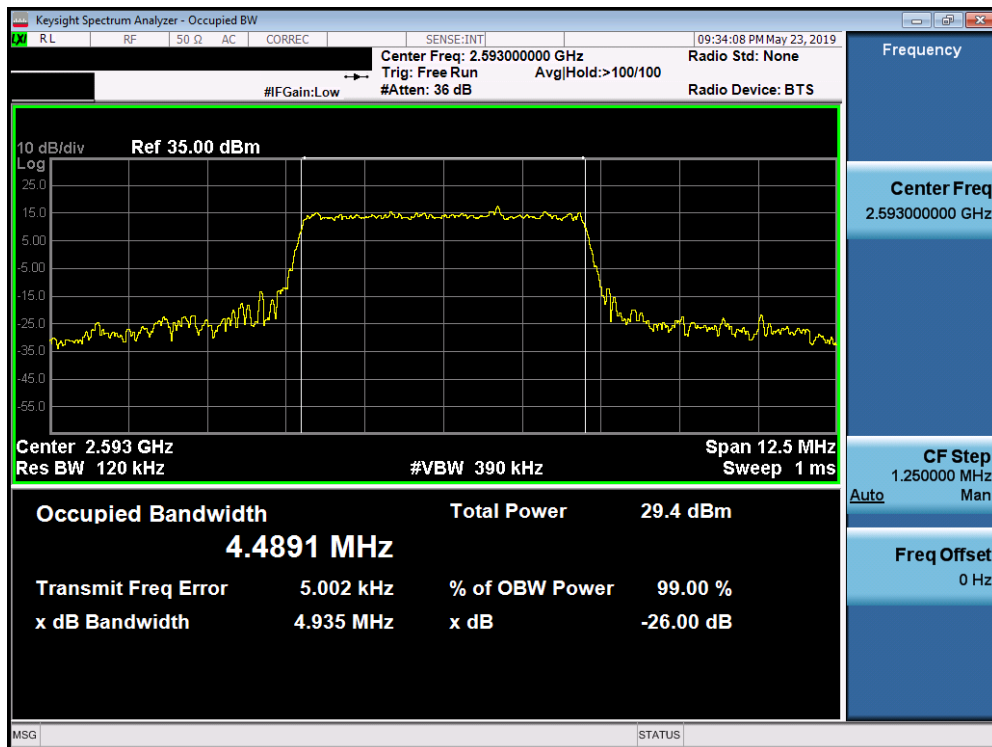
Plot 7-152. Occupied Bandwidth Plot (Band 41 (PC2) - 5.0MHz 256-QAM - Full RB Configuration)
