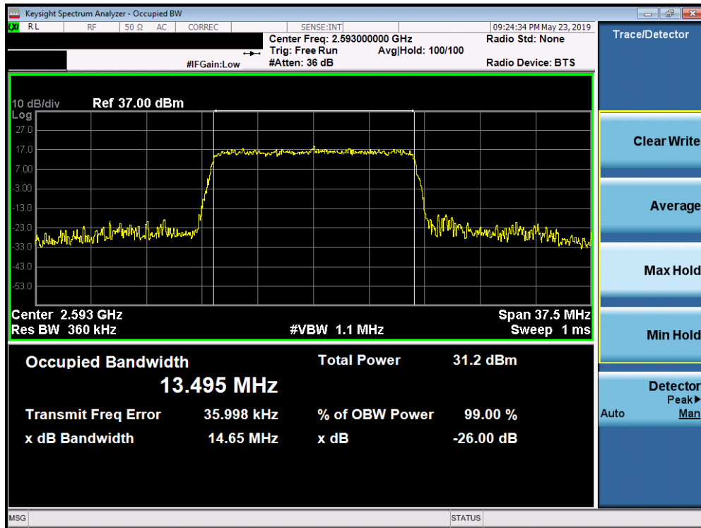
Plot 7-159. Occupied Bandwidth Plot (Band 41 (PC2) - 15.0MHz 64-QAM - Full RB Configuration)
