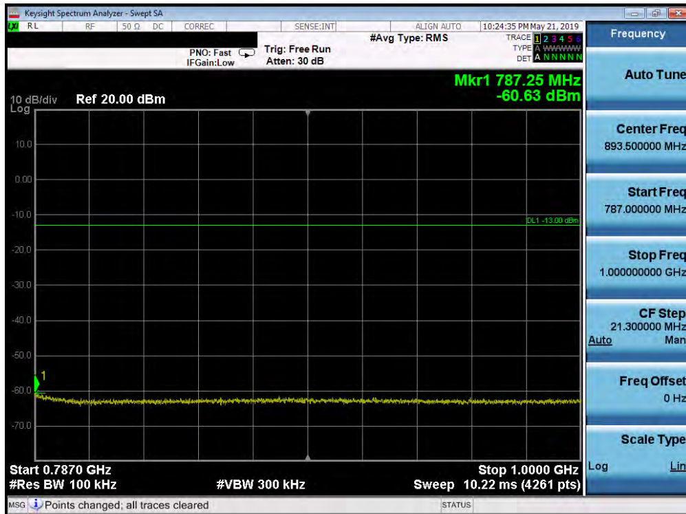
Plot 7-187. Conducted Spurious Plot (Band 13 - 5.0MHz QPSK - RB Size 1, RB Offset 0 - Mid Channel)
