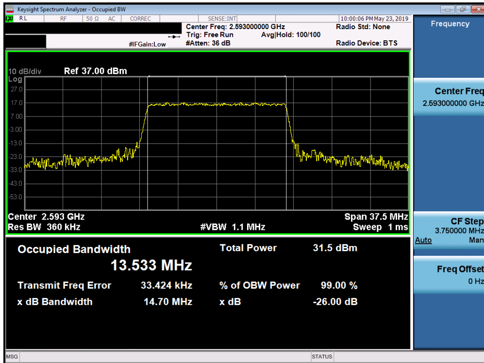
Plot 7-141. Occupied Bandwidth Plot (Band 41/38 (PC3) - 15.0MHz QPSK - Full RB Configuration)
