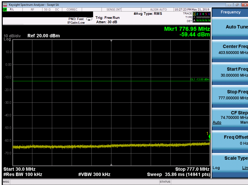
Plot 7-189. Conducted Spurious Plot (Band 13 - 5.0MHz QPSK - RB Size 1, RB Offset 0 - High Channel)
