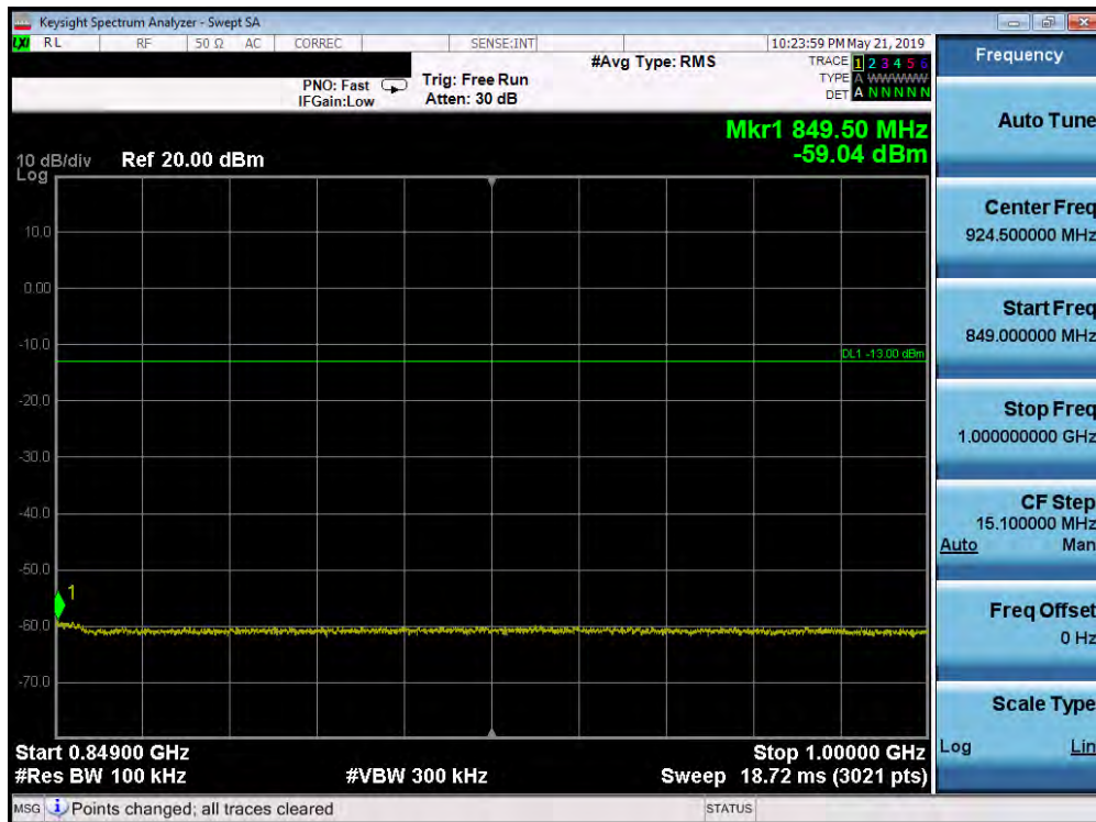
Plot 7-193. Conducted Spurious Plot (Band 26/5 - 10.0MHz QPSK - RB Size 1, RB Offset 0 - Low Channel)
