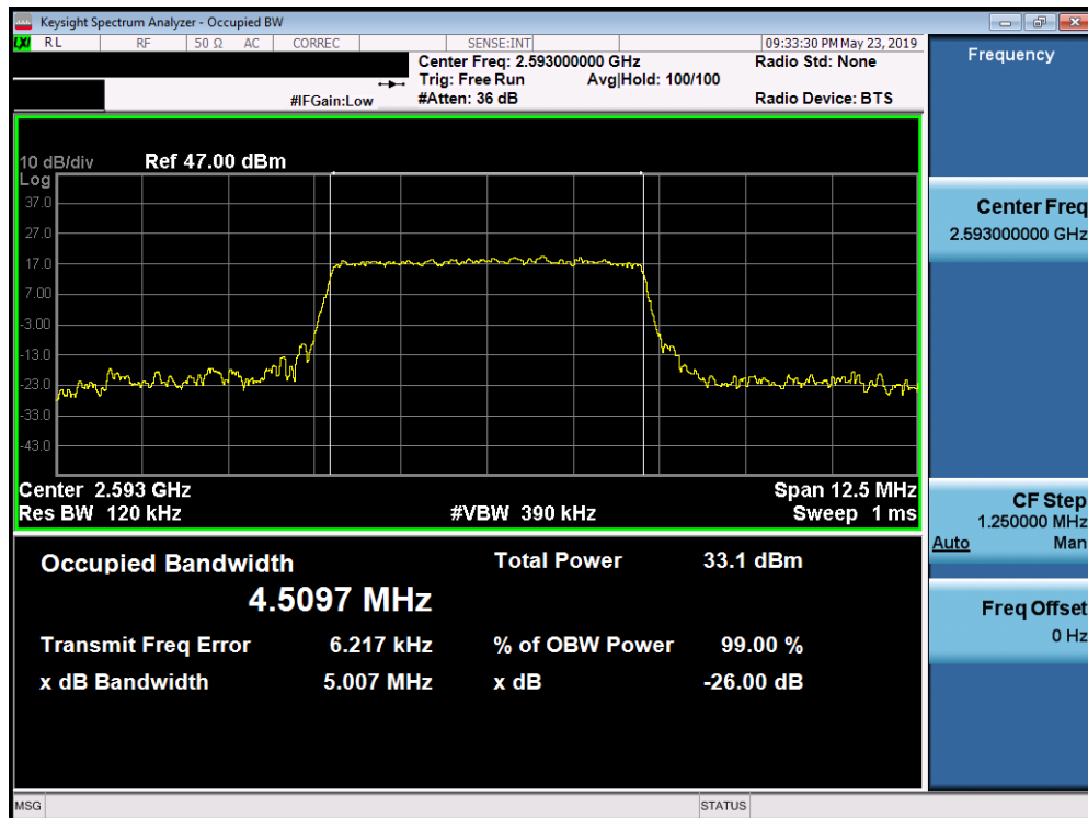
Plot 7-150. Occupied Bandwidth Plot (Band 41 (PC2) - 5.0MHz 16-QAM - Full RB Configuration)
