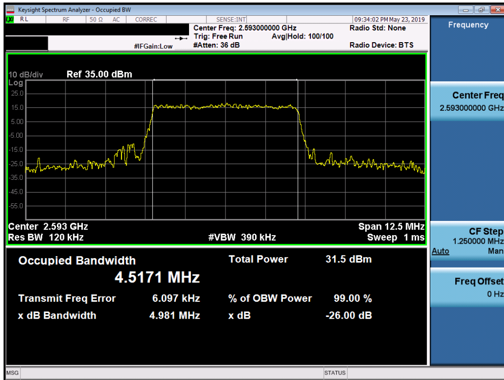
Plot 7-151. Occupied Bandwidth Plot (Band 41 (PC2) - 5.0MHz 64-QAM - Full RB Configuration)
