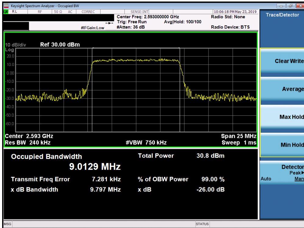
Plot 7-137. Occupied Bandwidth Plot (Band 41/38 (PC3) - 10.0MHz QPSK - Full RB Configuration)
