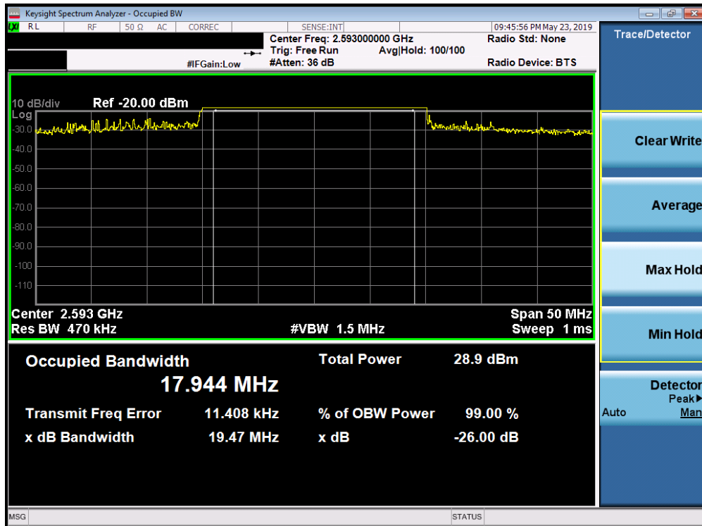
Plot 7-147. Occupied Bandwidth Plot (Band 41/38 (PC3) - 20.0MHz 64-QAM - Full RB Configuration)
