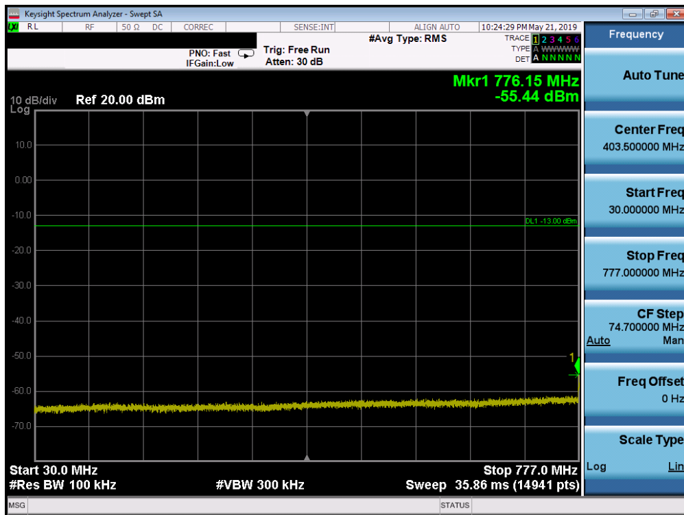
Plot 7-186. Conducted Spurious Plot (Band 13 - 5.0MHz QPSK - RB Size 1, RB Offset 0 - Mid Channel)
