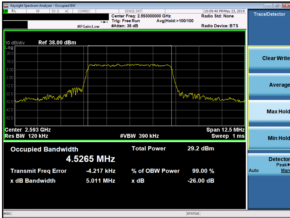
Plot 7-135. Occupied Bandwidth Plot (Band 41/38 (PC3) - 5.0MHz 64-QAM - Full RB Configuration)
