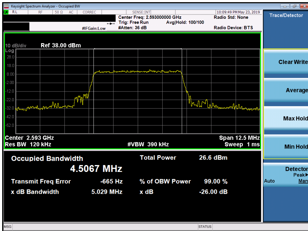
Plot 7-136. Occupied Bandwidth Plot (Band 41/38 (PC3) - 5.0MHz 256-QAM - Full RB Configuration)
