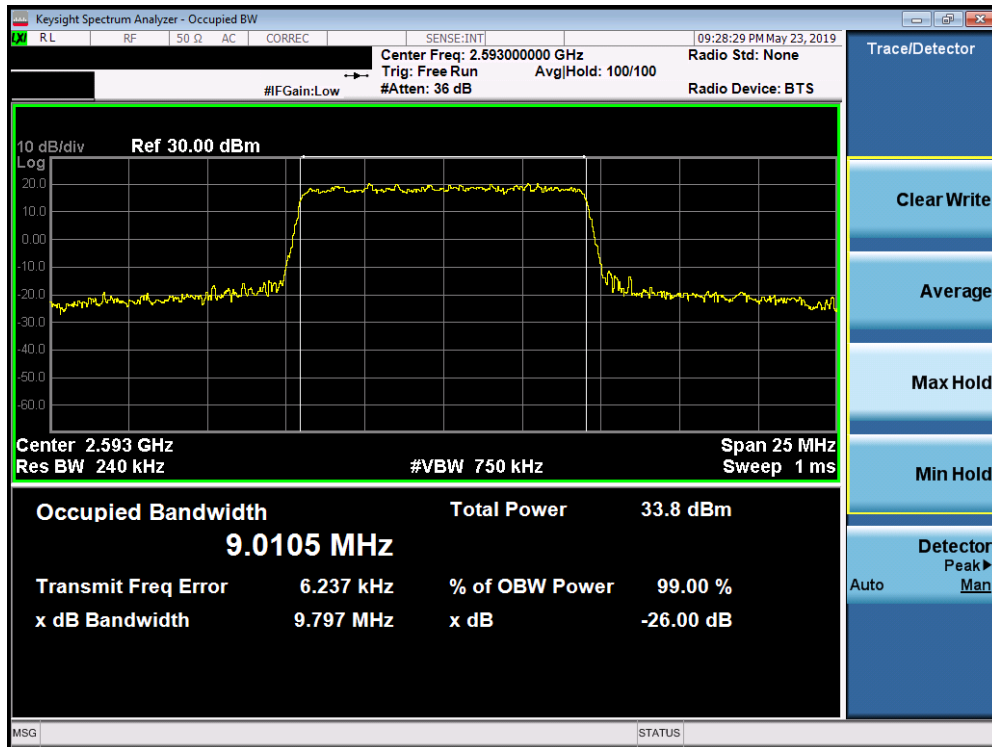
Plot 7-153. Occupied Bandwidth Plot (Band 41 (PC2) - 10.0MHz QPSK - Full RB Configuration)
