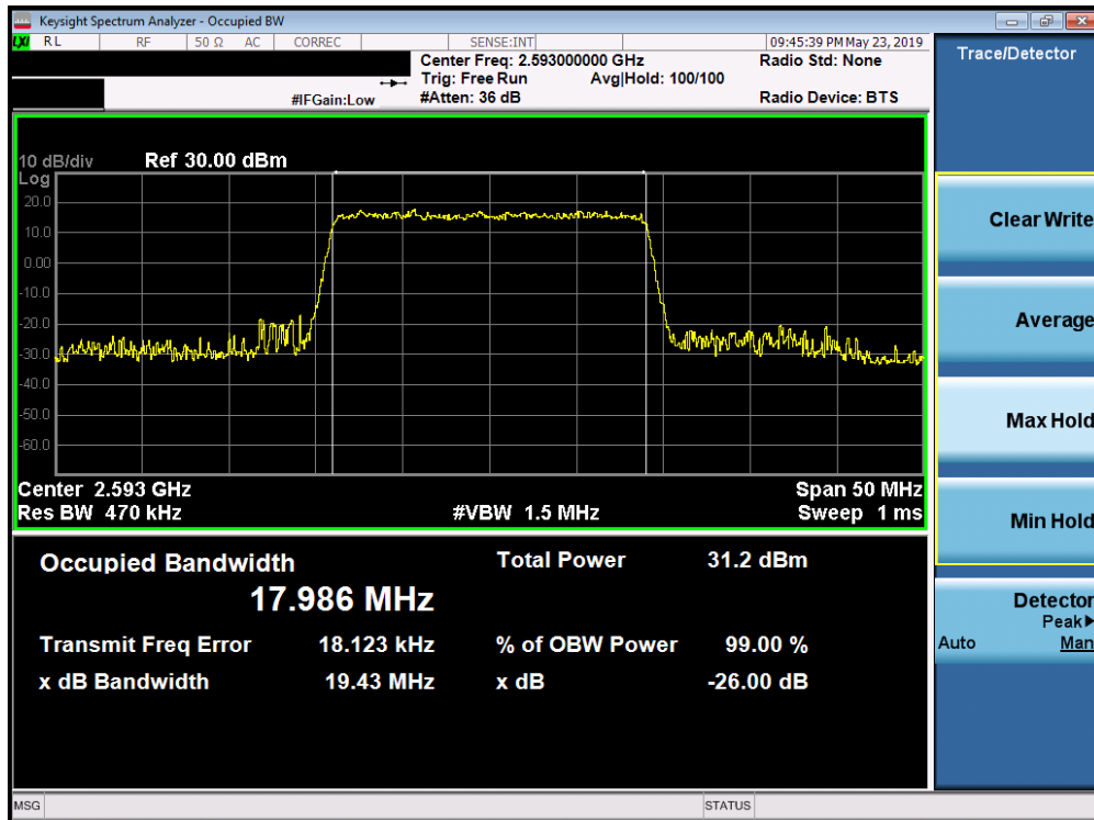
Plot 7-145. Occupied Bandwidth Plot (Band 41/38 (PC3) - 20.0MHz QPSK - Full RB Configuration)
