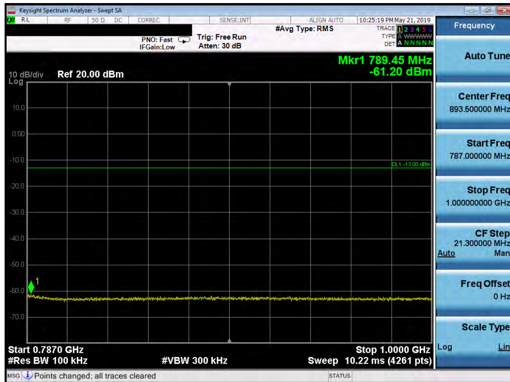
Plot 7-184. Conducted Spurious Plot (Band 13 - 5.0MHz QPSK - RB Size 1, RB Offset 0 - Low Channel)
