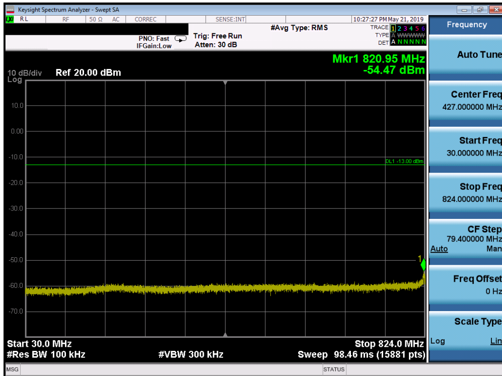
Plot 7-198. Conducted Spurious Plot (Band 26/5 - 10.0MHz QPSK - RB Size 1, RB Offset 0 - High Channel)
