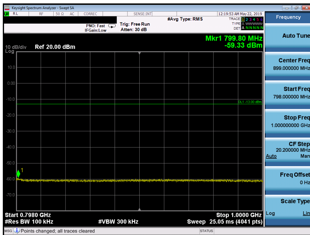
Plot 7-44. Conducted Spurious Plot (LTE Band 14, 5.0 MHz QPSK – RB Size 1, RB Offset 0 – Low Channel)
