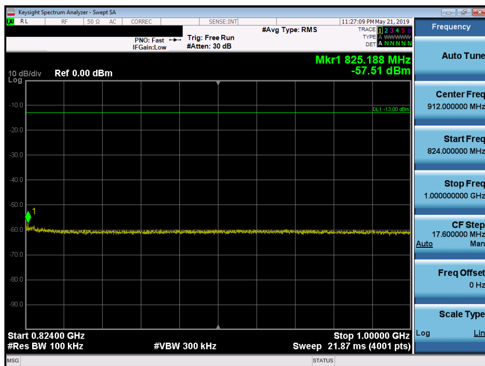
Plot 7-38. Conducted Spurious Plot (LTE Band 26, 5.0 MHz QPSK – RB Size 1, RB Offset 0 – Low Channel)
