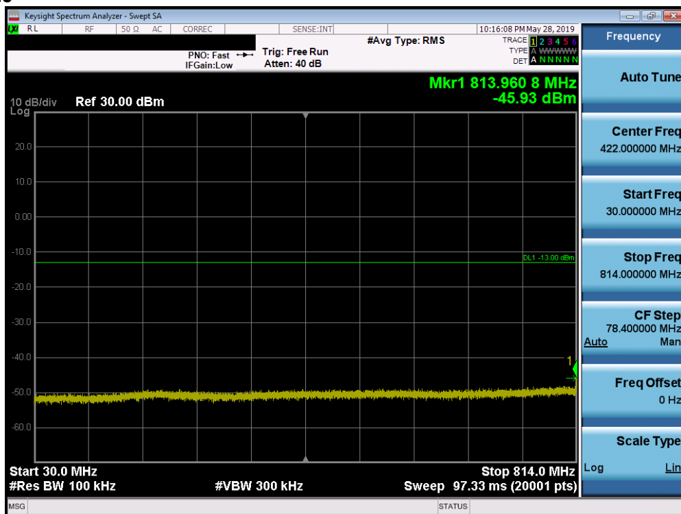
Plot 7-31. Conducted Spurious Plot (CDMA BC10 - Ch. 476)
