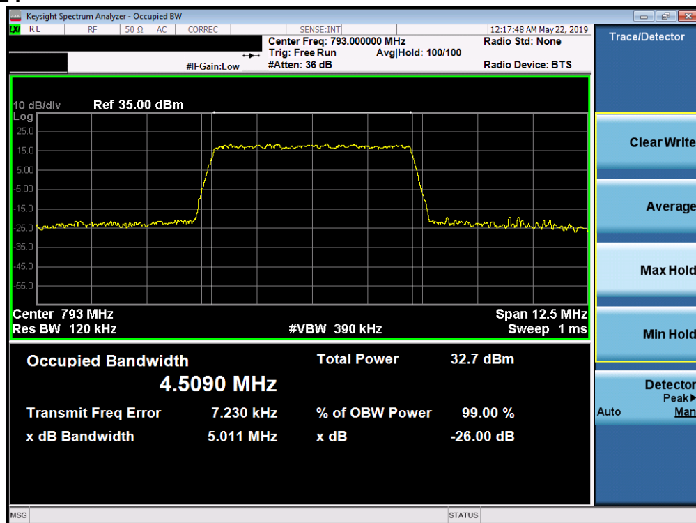
Plot 7-23. Occupied Bandwidth Plot (LTE Band 14, 5MHz QPSK – RB Size 25)
