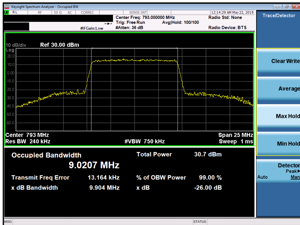
Plot 7-29. Occupied Bandwidth Plot (LTE Band 14, 10MHz 64-QAM – RB Size 50)
