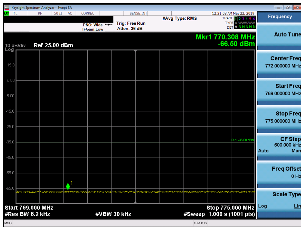
Plot 7-63. Lower Emission Mask Plot (LTE Band 14, 5MHz QPSK – RB Size 25)
