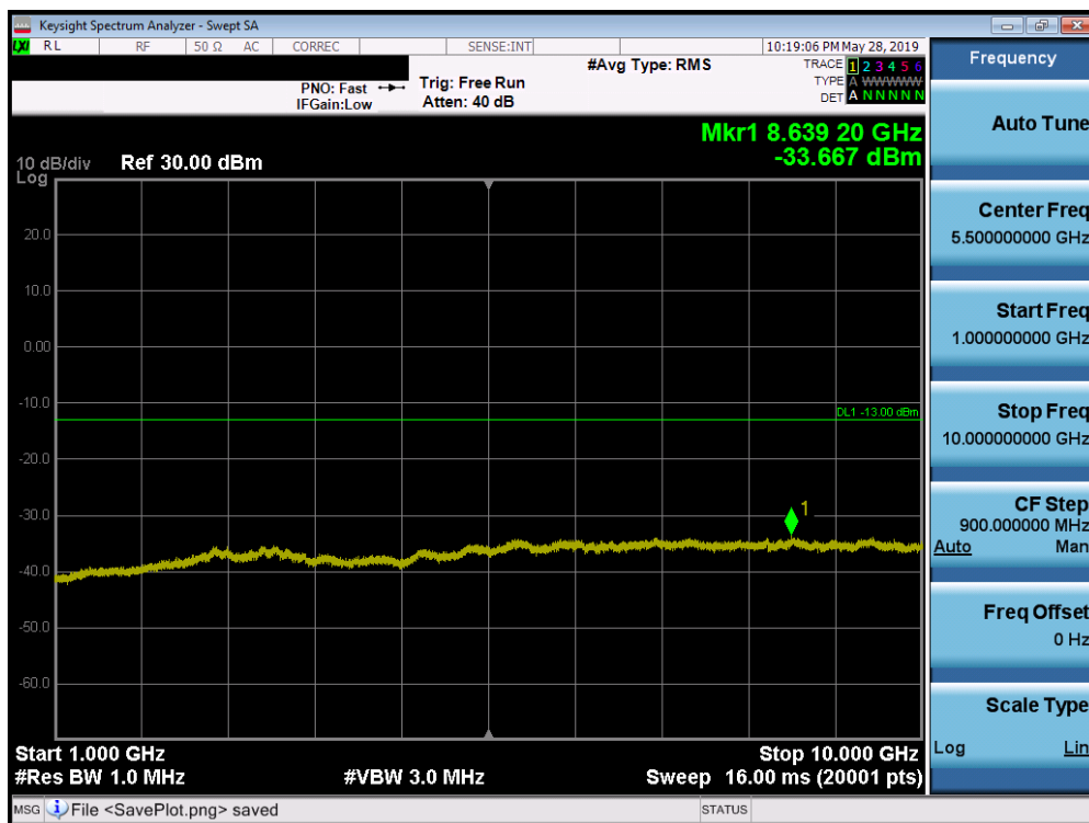
Plot 7-33. Conducted Spurious Plot (CDMA BC10 - Ch. 476)
