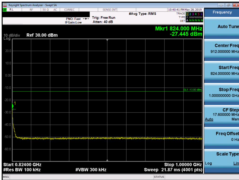
Plot 7-35. Conducted Spurious Plot (CDMA BC10 - Ch. 684)
