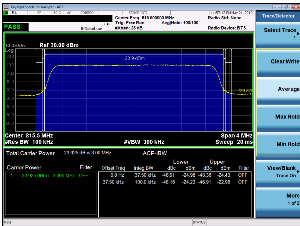
Plot 7-56. Channel Edge Plot (LTE Band 26, 3MHz QPSK – RB Size 15– Low Channel)
