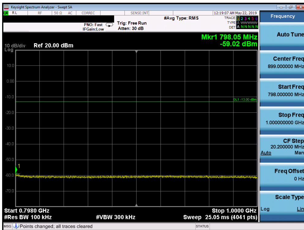
Plot 7-47. Conducted Spurious Plot (LTE Band 14, 5.0 MHz QPSK – RB Size 1, RB Offset 0 – Mid Channel)
