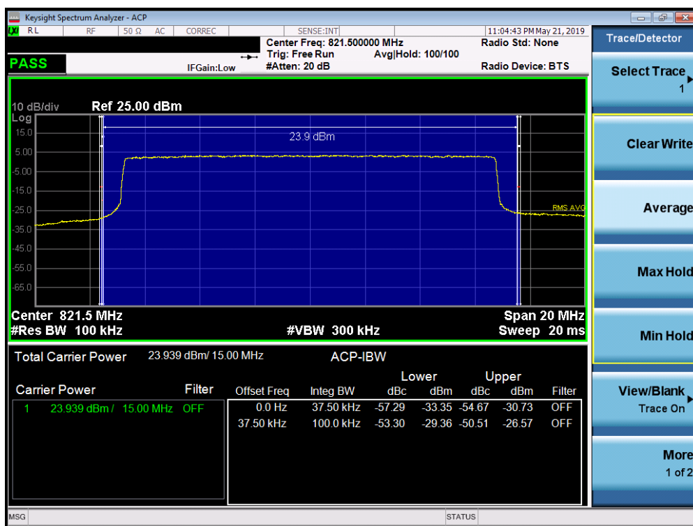
Plot 7-61. Channel Edge Plot (LTE Band 26, 15MHz QPSK – RB Size 75)
