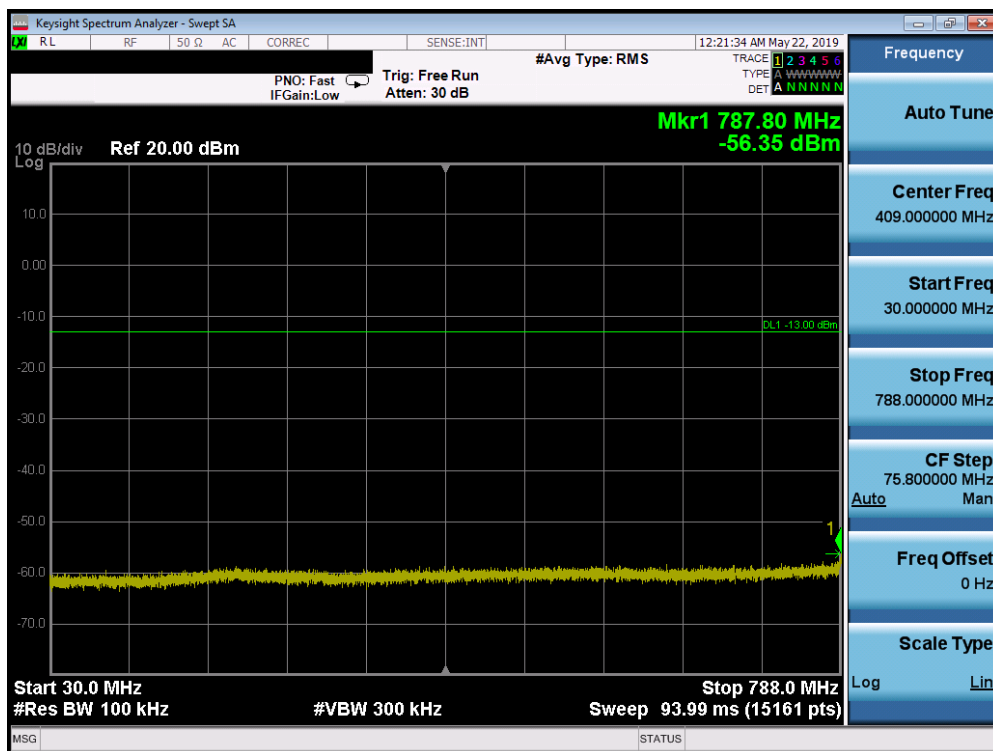
Plot 7-49. Conducted Spurious Plot (LTE Band 14, 5.0 MHz QPSK – RB Size 1, RB Offset 0 – High Channel)
