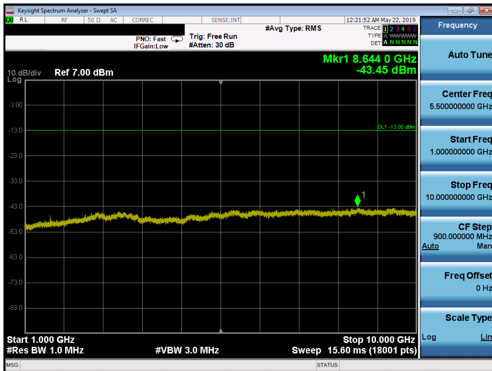
Plot 7-51. Conducted Spurious Plot (LTE Band 14, 5.0 MHz QPSK – RB Size 1, RB Offset 0 – High Channel)
