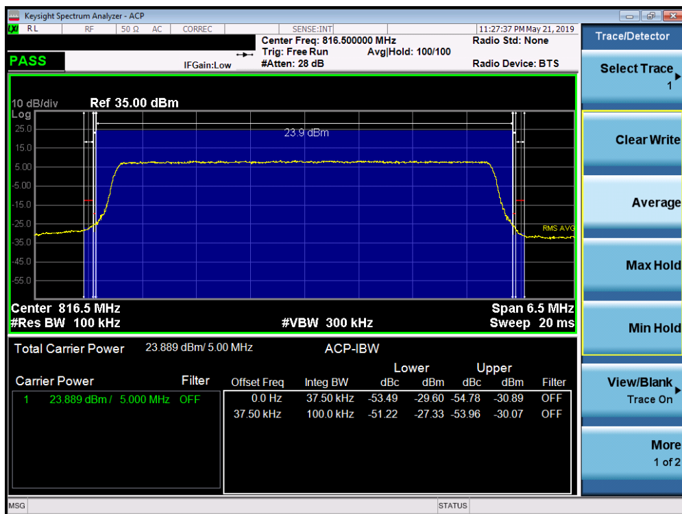
Plot 7-58. Channel Edge Plot (LTE Band 26, 5MHz QPSK – RB Size 25– Low Channel)
