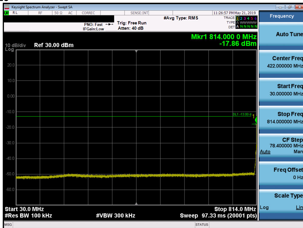
Plot 7-37. Conducted Spurious Plot (LTE Band 26, 5.0 MHz QPSK – RB Size 1, RB Offset 0 – Low Channel)
