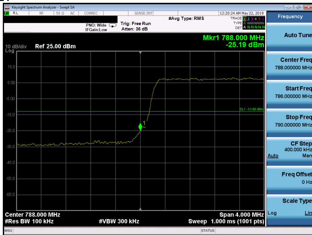
Plot 7-62. Lower Band Edge Plot (LTE Band 14, 5MHz QPSK – RB Size 25)
