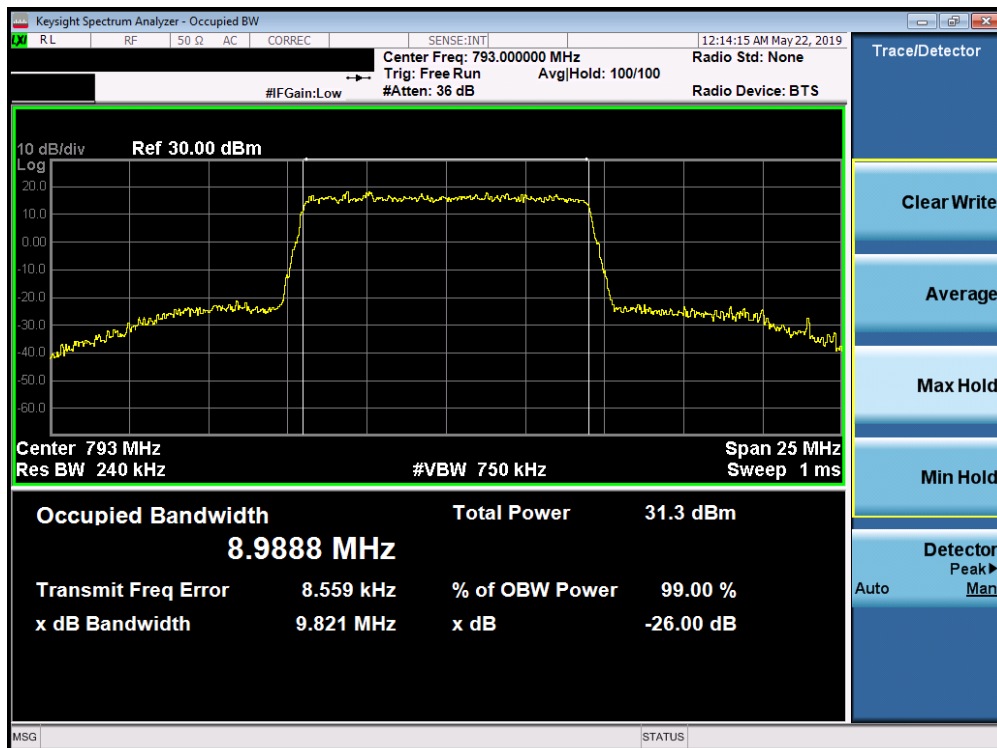
Plot 7-28. Occupied Bandwidth Plot (LTE Band 14, 10MHz 16-QAM – RB Size 50)
