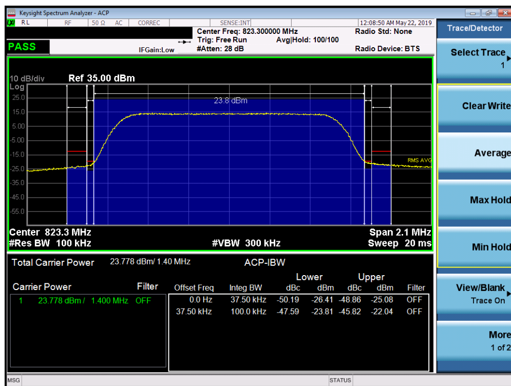
Plot 7-55. Channel Edge Plot (LTE Band 26, 1.4MHz QPSK – RB Size 6 – High Channel)
