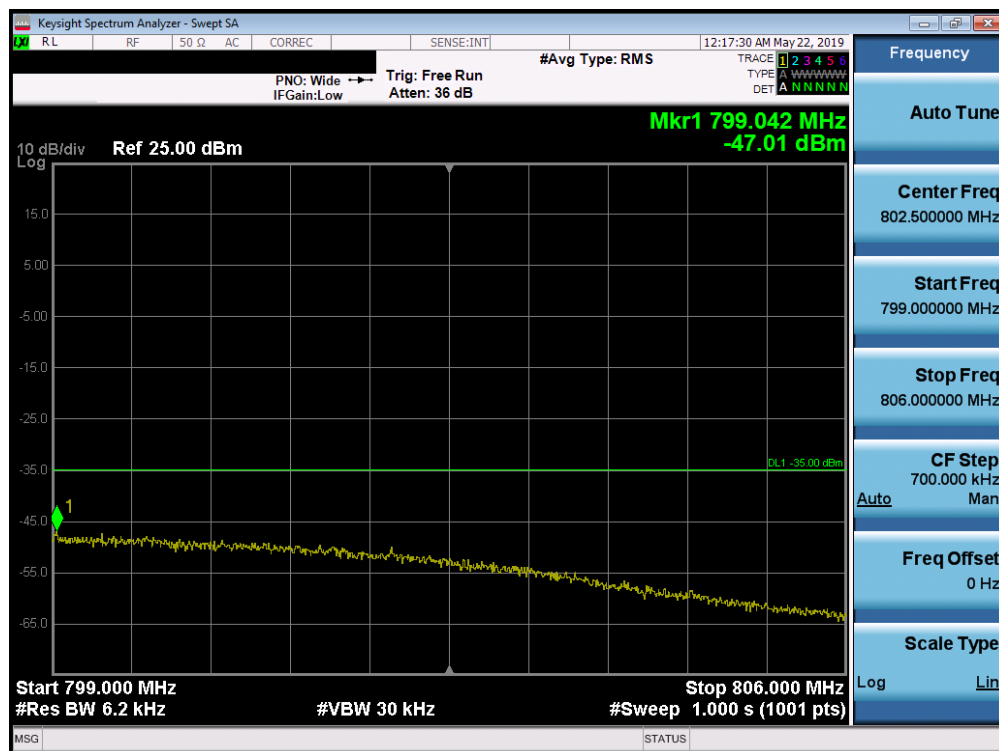
Plot 7-69. Upper Emission Mask Plot (LTE Band 14, 10MHz QPSK – RB Size 50)
