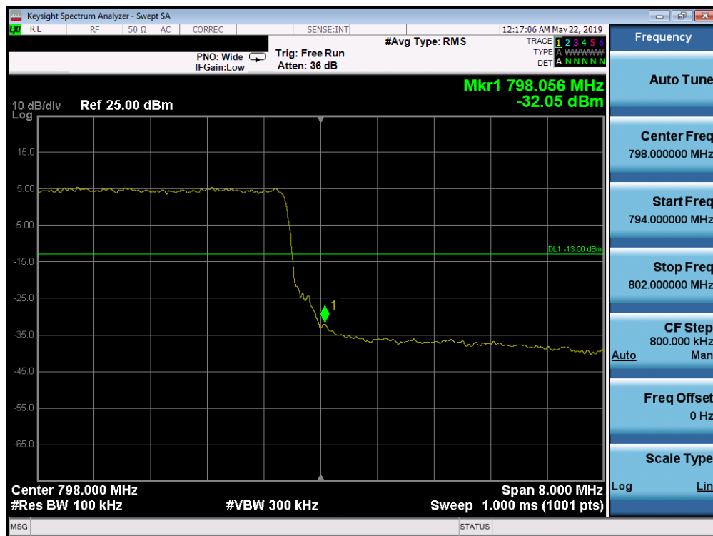
Plot 7-68. Upper Band Edge Plot (LTE Band 14, 10MHz QPSK – RB Size 50)
