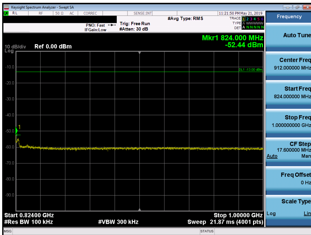
Plot 7-41. Conducted Spurious Plot (LTE Band 26, 5.0 MHz QPSK – RB Size 1, RB Offset 0 – High Channel)
