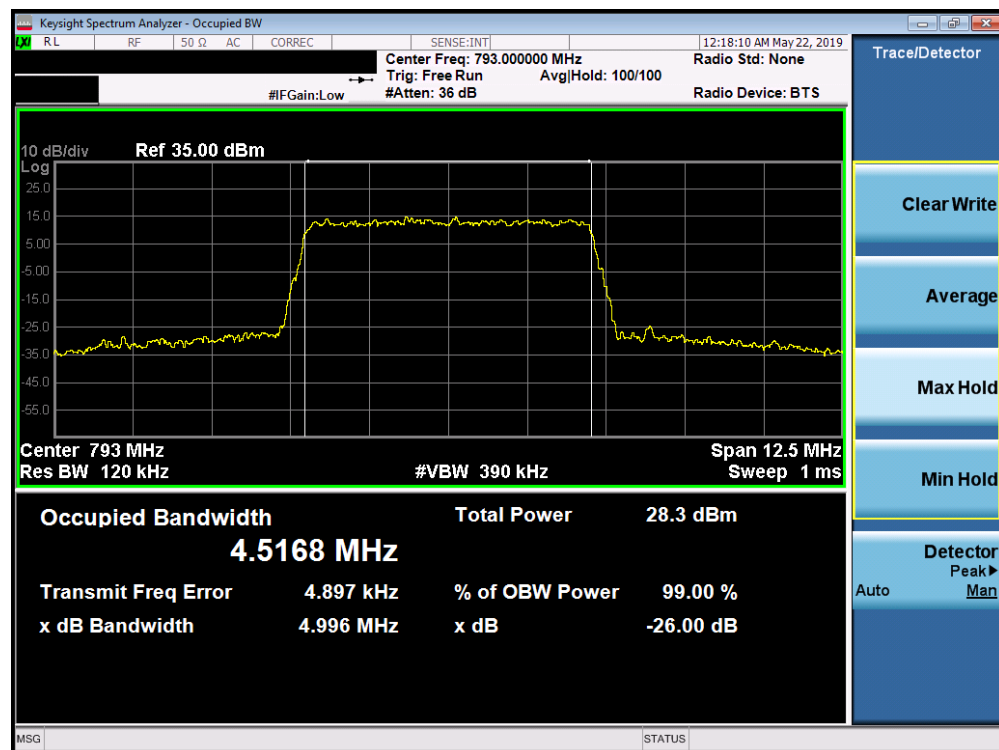
Plot 7-26. Occupied Bandwidth Plot (LTE Band 14, 5MHz 256-QAM – RB Size 25)
