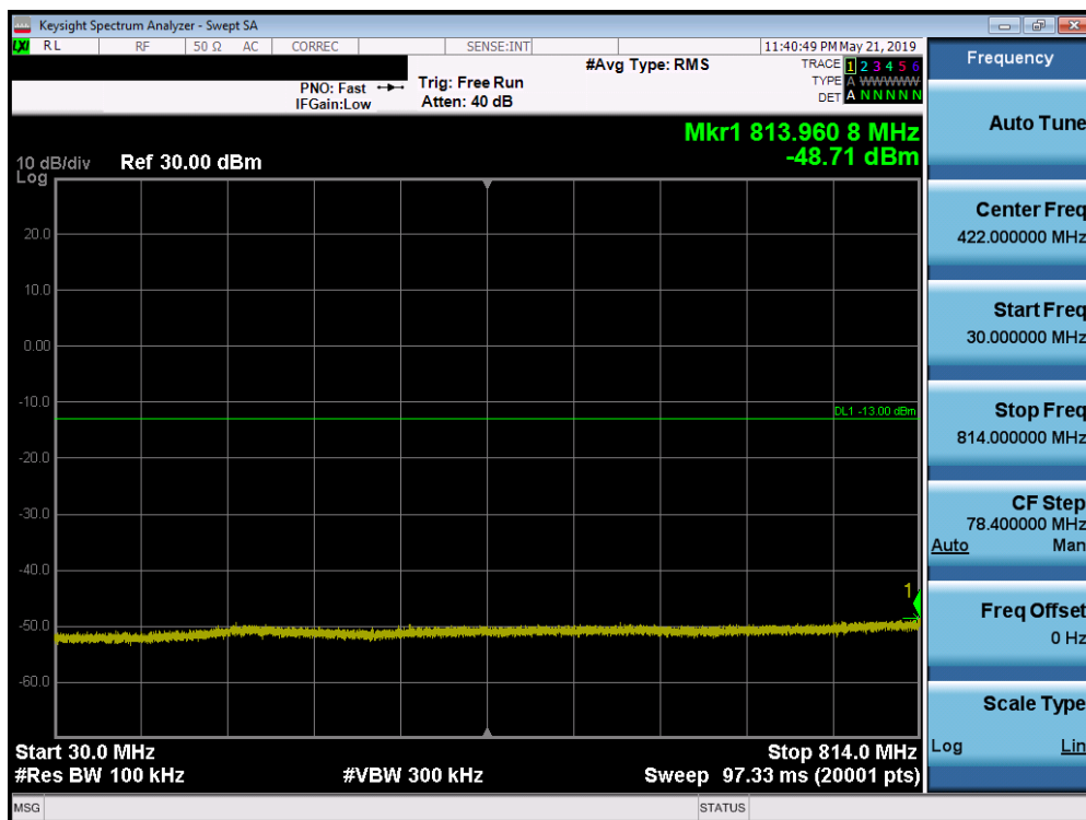
Plot 7-40. Conducted Spurious Plot (LTE Band 26, 5.0 MHz QPSK – RB Size 1, RB Offset 0 – High Channel)
