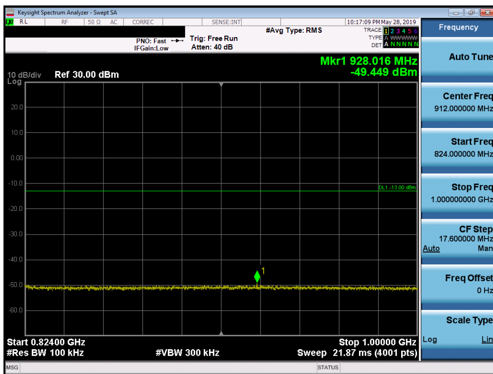
Plot 7-32. Conducted Spurious Plot (CDMA BC10 - Ch. 476)
