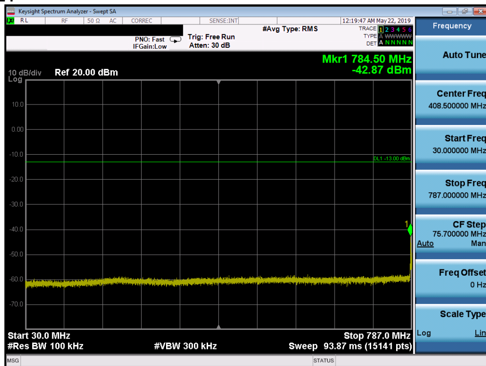
Plot 7-43. Conducted Spurious Plot (LTE Band 14, 5.0 MHz QPSK – RB Size 1, RB Offset 0 – Low Channel)
