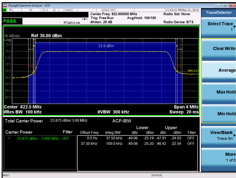
Plot 7-57. Channel Edge Plot (LTE Band 26, 3MHz QPSK – RB Size 15 – High Channel)
