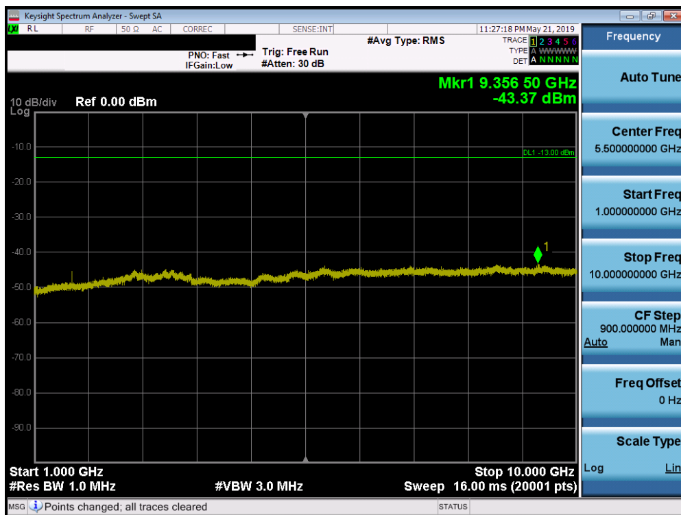
Plot 7-39. Conducted Spurious Plot (LTE Band 26, 5.0 MHz QPSK – RB Size 1, RB Offset 0 – Low Channel)
