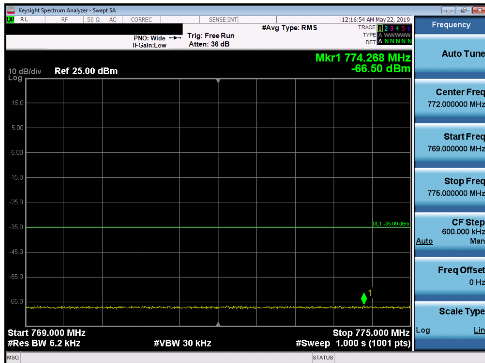
Plot 7-67. Lower Emission Mask Plot (LTE Band 14, 10MHz QPSK - RB Size 50)
