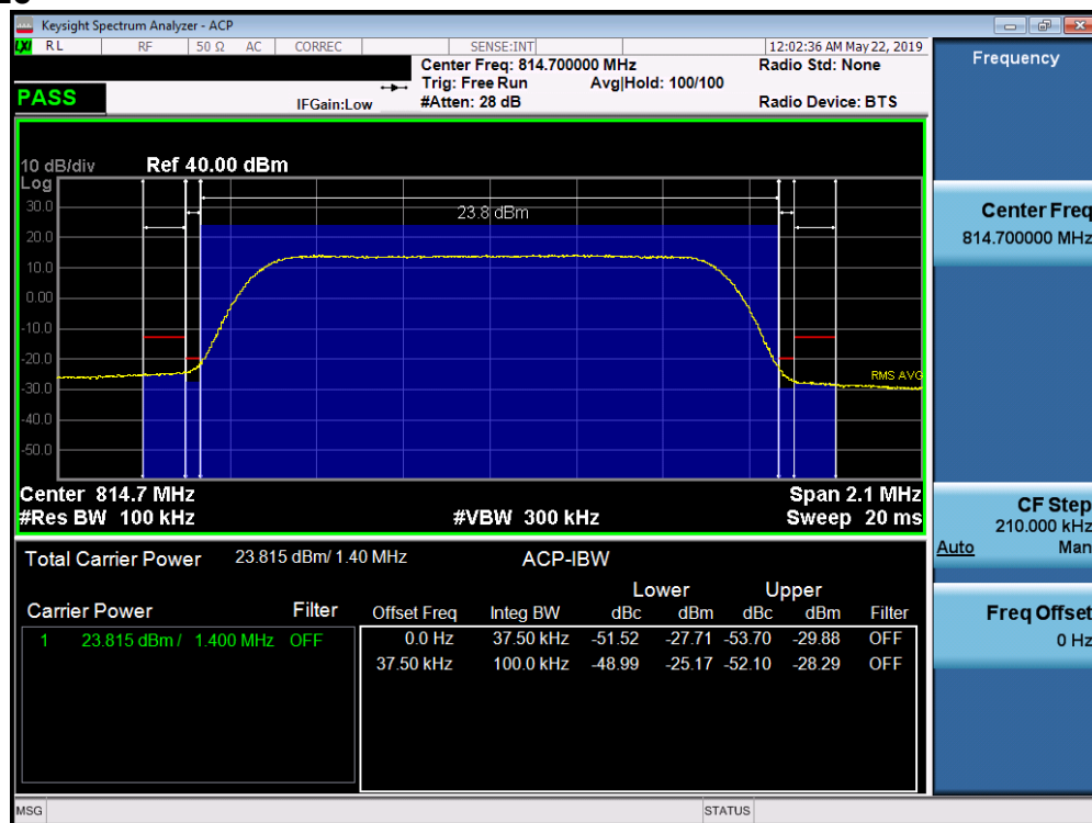
Plot 7-54. Channel Edge Plot (LTE Band 26, 1.4MHz QPSK – RB Size 6– Low Channel)
