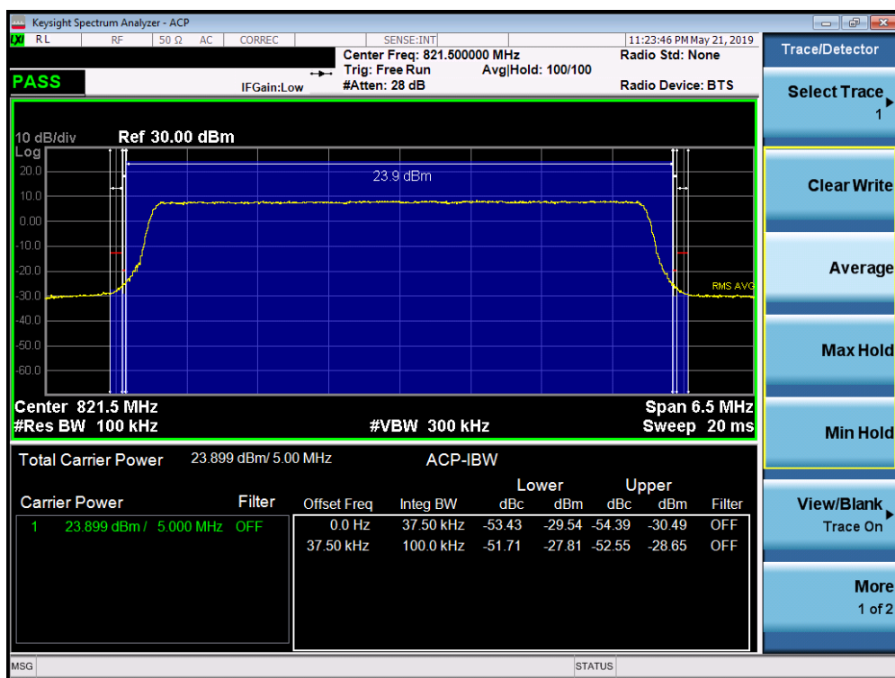
Plot 7-59. Channel Edge Plot (LTE Band 26, 5MHz QPSK – RB Size 25 – High Channel)
