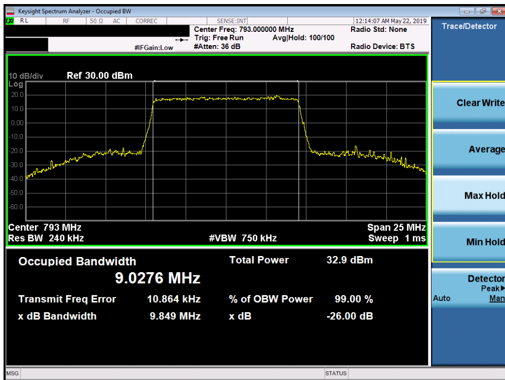
Plot 7-27. Occupied Bandwidth Plot (LTE Band 14, 10MHz QPSK – RB Size 50)
