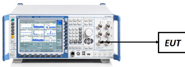
Figure 7-4. ERP/EIRP Measurement Setup
