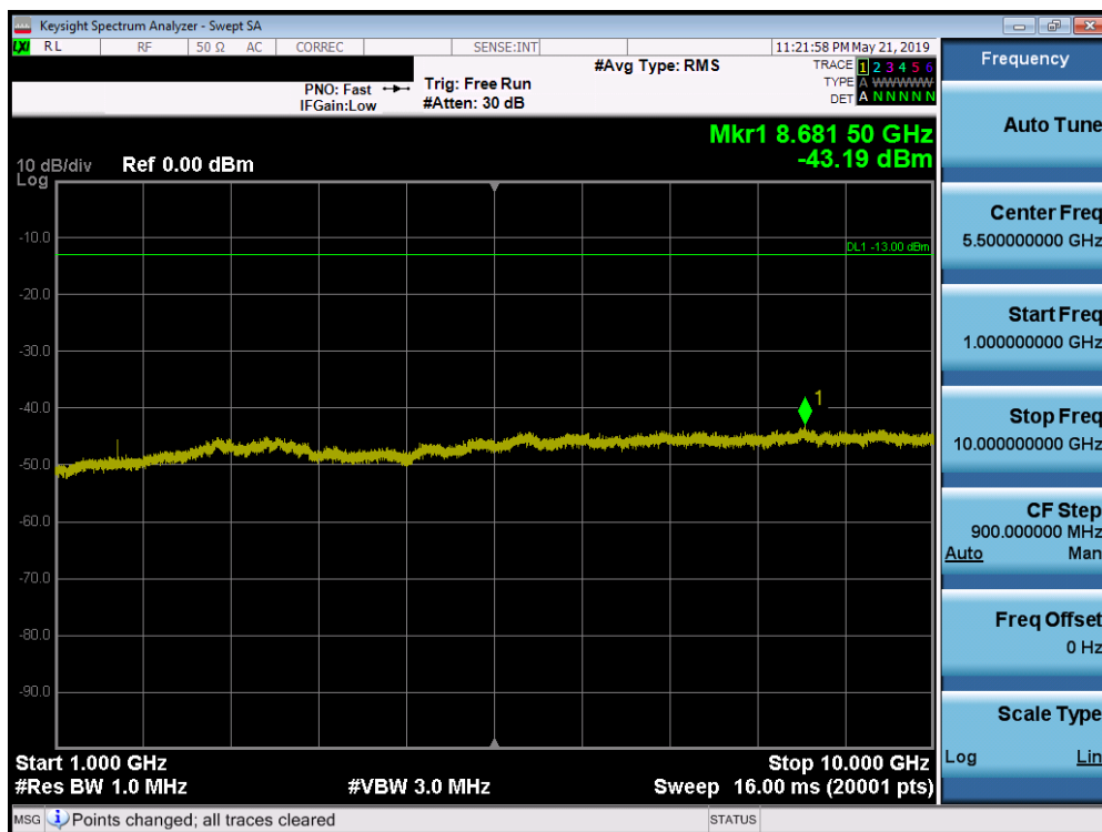
Plot 7-42. Conducted Spurious Plot (LTE Band 26, 5.0 MHz QPSK – RB Size 1, RB Offset 0 – High Channel)
