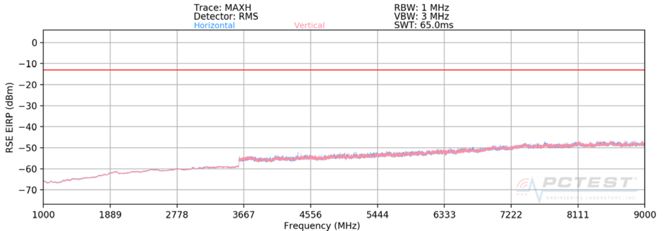
Plot 7-72. Radiated Spurious Plot above 1GHz (CDMA BC10)
