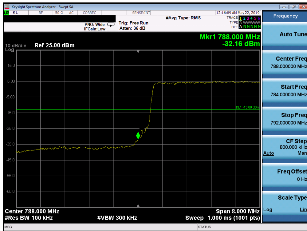
Plot 7-66. Lower Band Edge Plot (LTE Band 14, 10MHz QPSK - RB Size 50)
