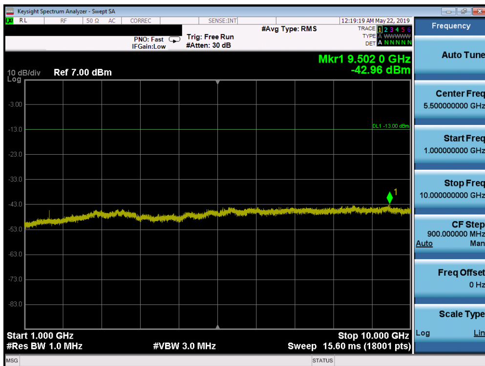
Plot 7-48. Conducted Spurious Plot (LTE Band 14, 5.0 MHz QPSK – RB Size 1, RB Offset 0 – Mid Channel)
