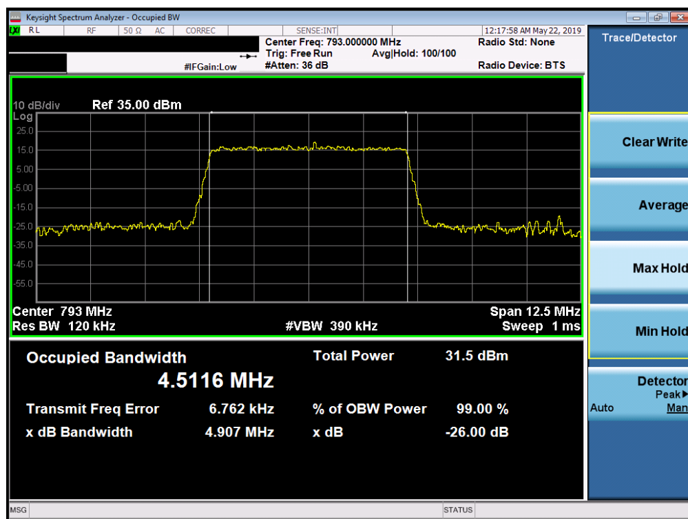
Plot 7-24. Occupied Bandwidth Plot (LTE Band 14, 5MHz 16-QAM – RB Size 25)
