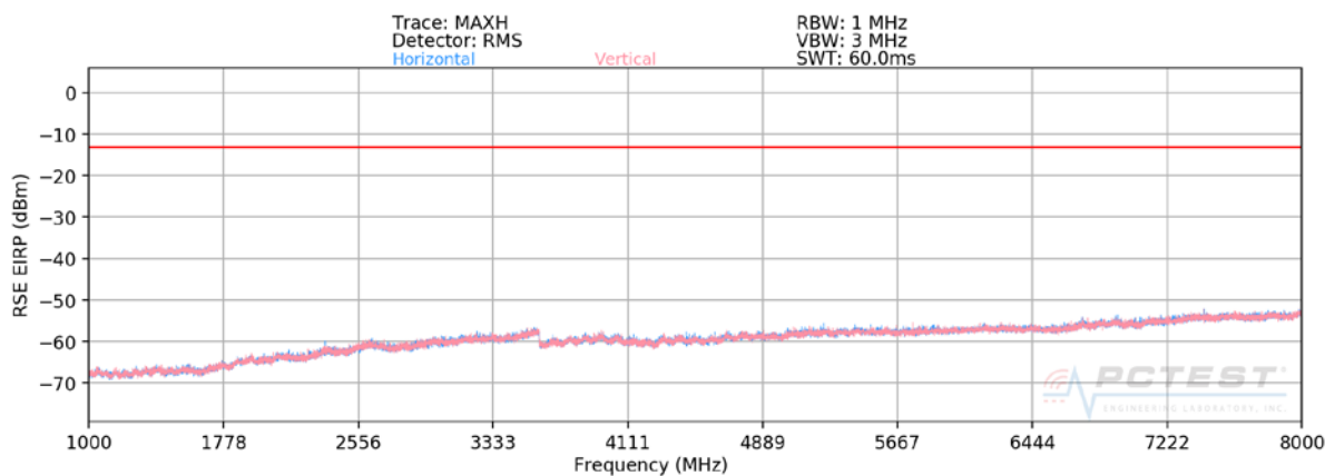
Plot 7-74. Radiated Spurious Plot above 1GHz (LTE Band 14)
