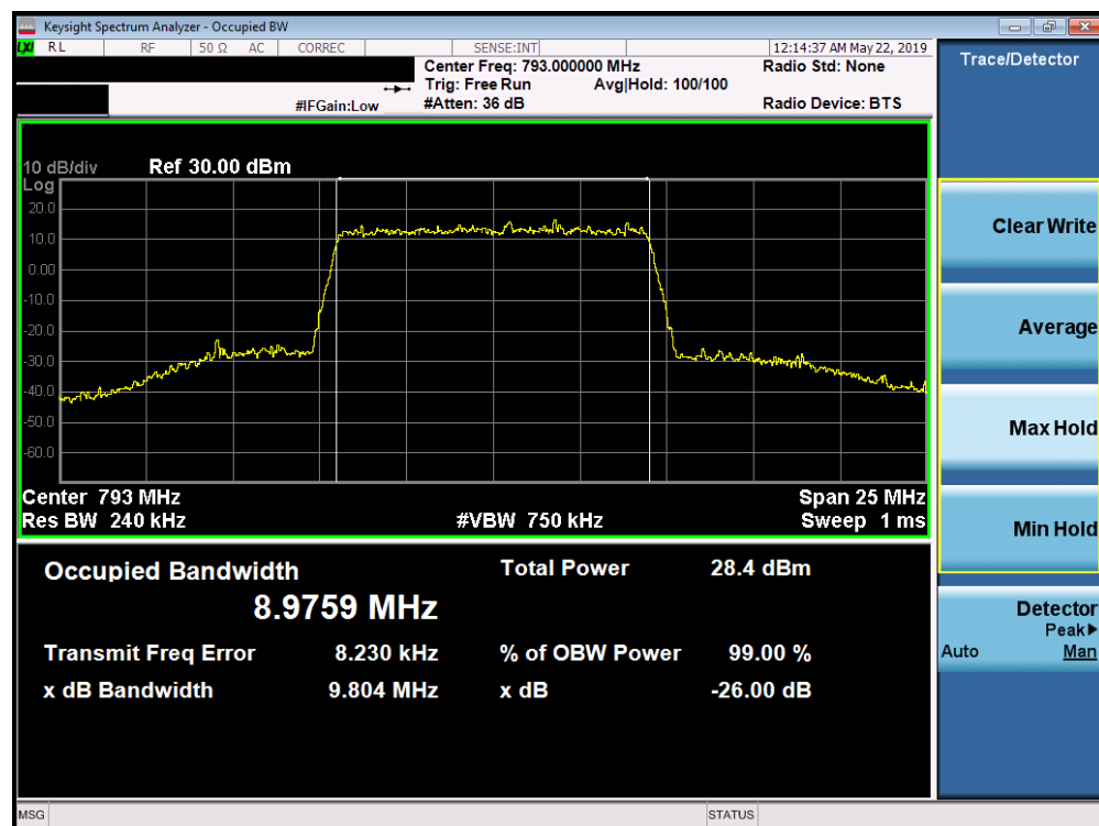
Plot 7-30. Occupied Bandwidth Plot (LTE Band 14, 10MHz 256-QAM – RB Size 50)
