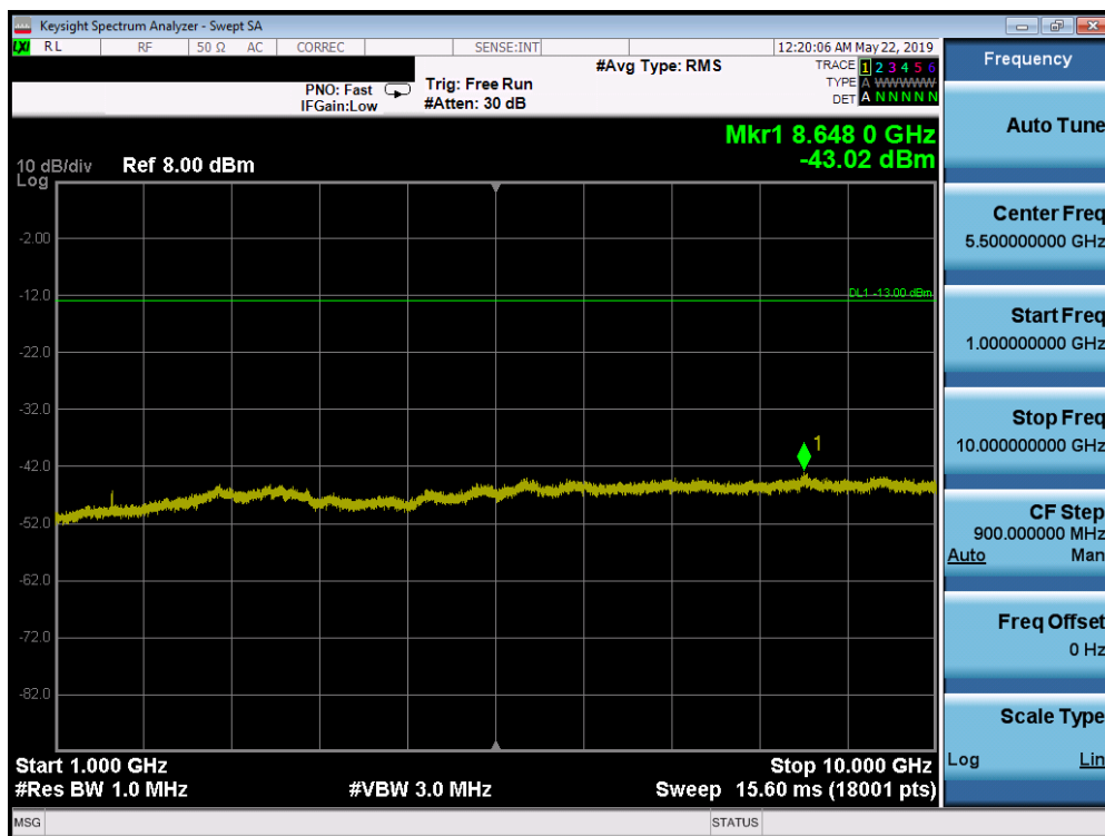
Plot 7-45. Conducted Spurious Plot (LTE Band 14, 5.0 MHz QPSK – RB Size 1, RB Offset 0 – Low Channel)
