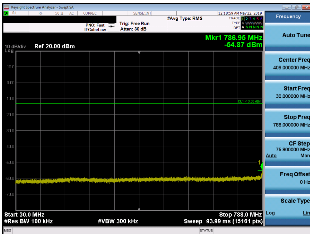
Plot 7-46. Conducted Spurious Plot (LTE Band 14, 5.0 MHz QPSK – RB Size 1, RB Offset 0 – Mid Channel)
