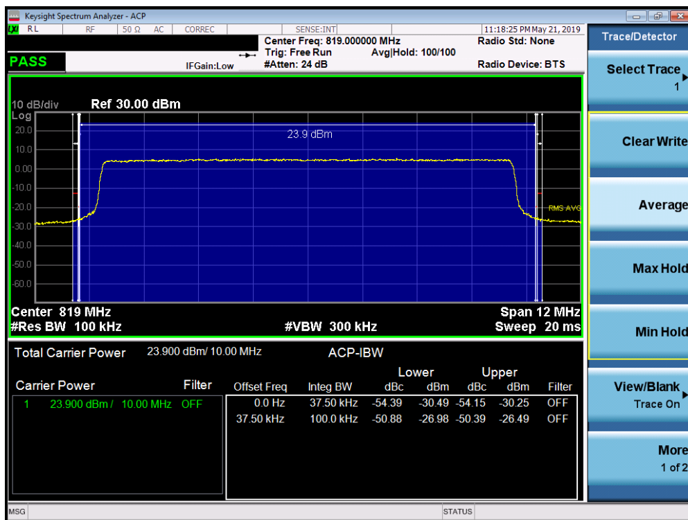
Plot 7-60. Channel Edge Plot (LTE Band 26, 10MHz QPSK – RB Size 50)
