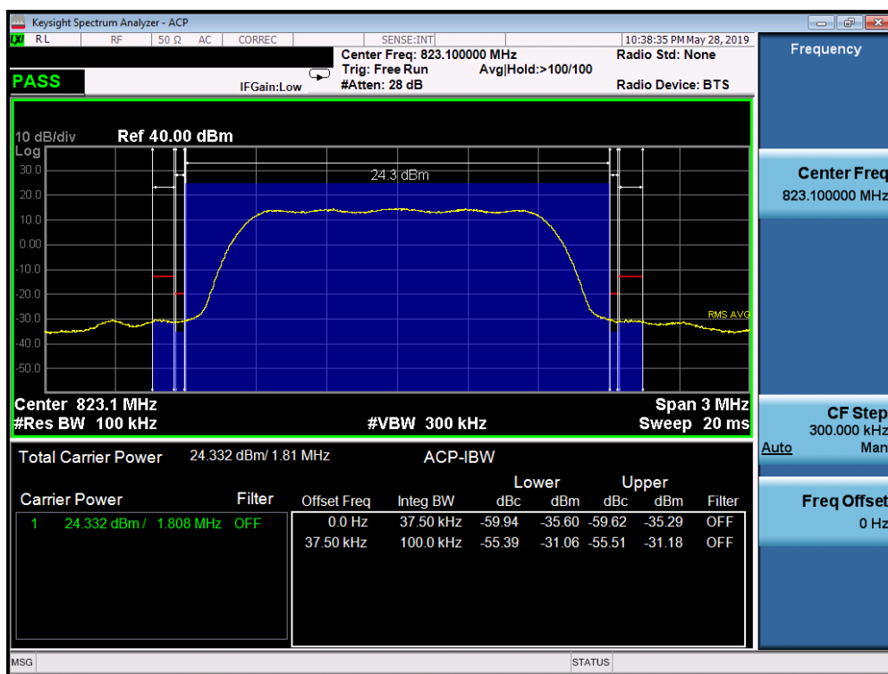
Plot 7-53. Channel Edge Plot (CDMA BC10 - Ch. 684)
