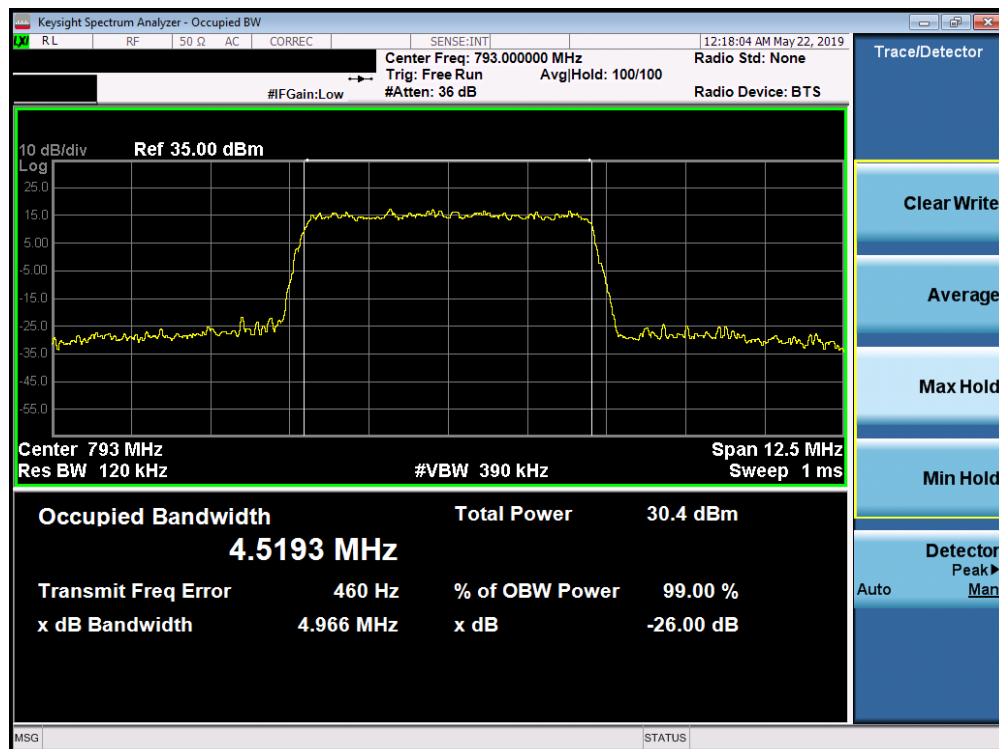
Plot 7-25. Occupied Bandwidth Plot (LTE Band 14, 5MHz 64-QAM – RB Size 25)
