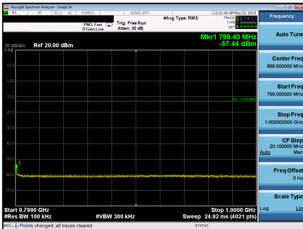
Plot 7-50. Conducted Spurious Plot (LTE Band 14, 5.0 MHz QPSK – RB Size 1, RB Offset 0 – High Channel)
