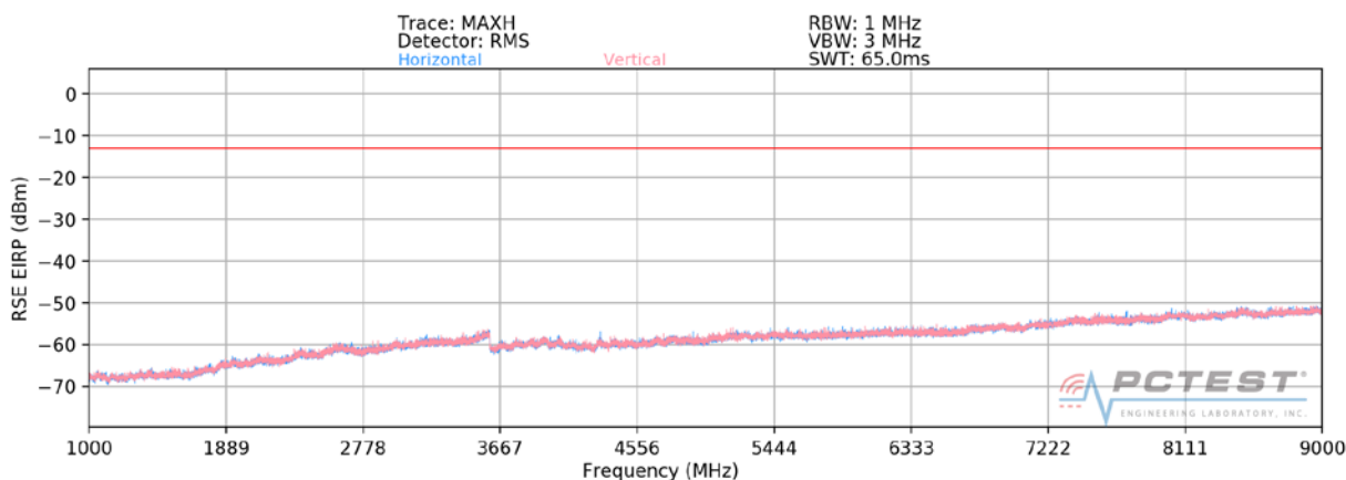
Plot 7-73. Radiated Spurious Plot above 1GHz (LTE Band 26)
