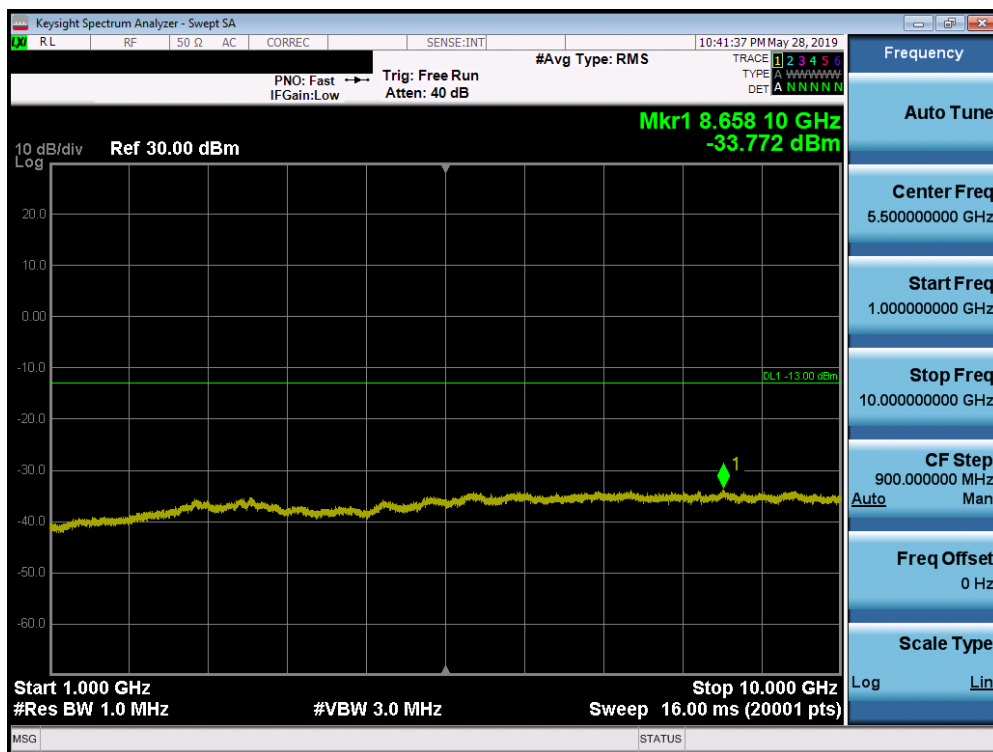
Plot 7-36. Conducted Spurious Plot (CDMA BC10 - Ch. 684)
