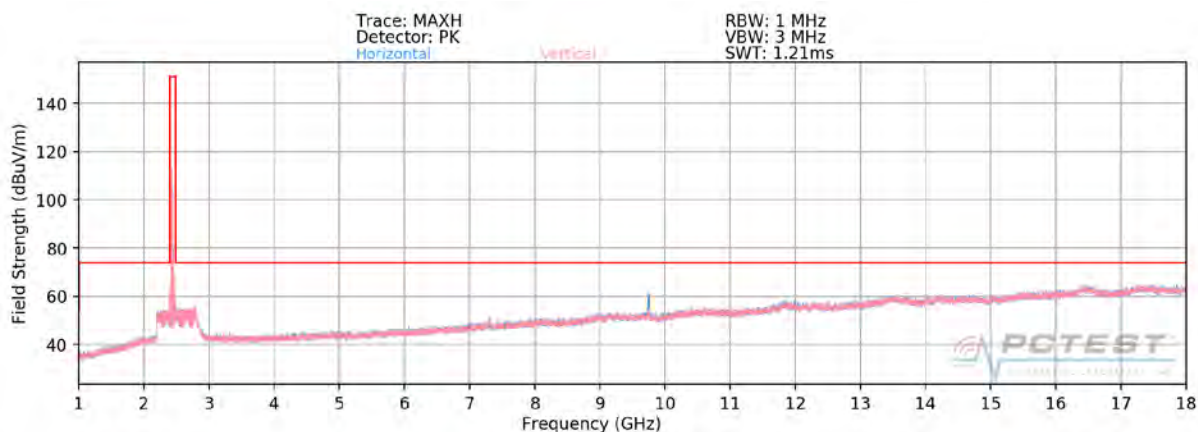
Plot 7-102. Radiated Spurious Plot above 1GHz MIMO/CDD (802.11g – Ch. 6)
