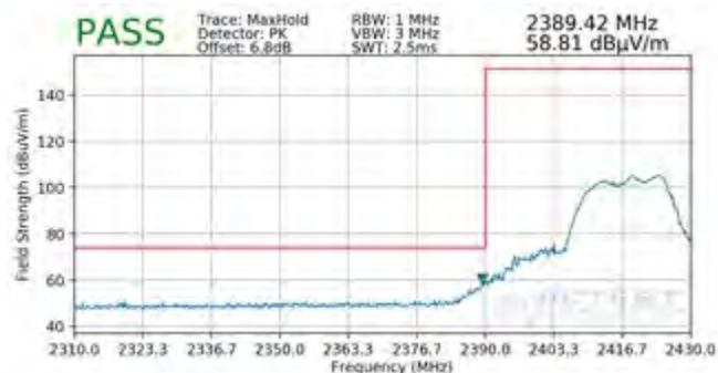
Plot 7-140. Radiated Restricted Band Edge Measurement CDD with WCP (Peak)
