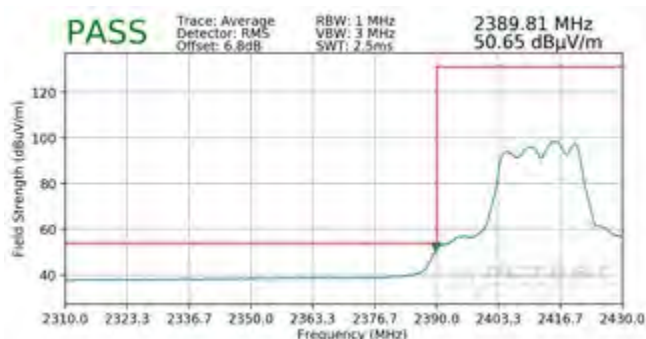
Plot 7-131. Radiated Restricted Lower Band Edge Measurement CDD (Average)
