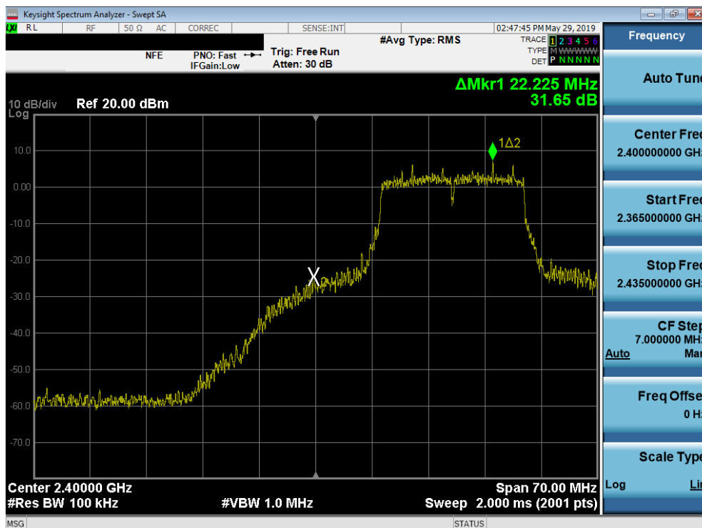
Plot 7-74. Band Edge Plot SISO ANT2 (802.11n(2.4GHz) – Ch. 2)
