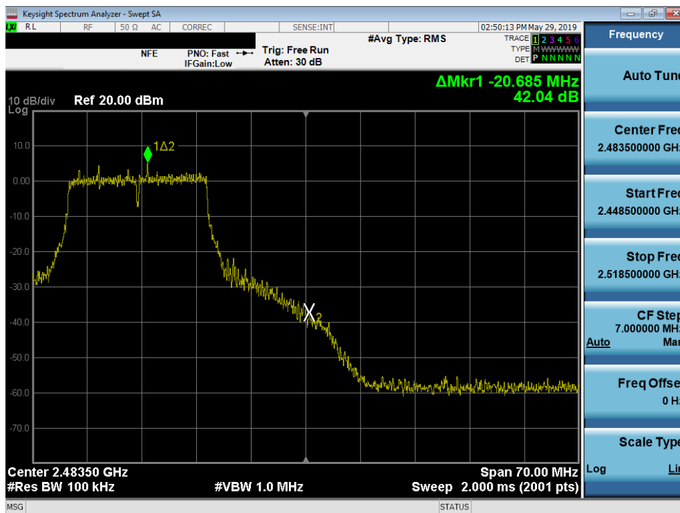
Plot 7-76. Band Edge Plot SISO ANT2 (802.11n(2.4GHz) – Ch. 11)
