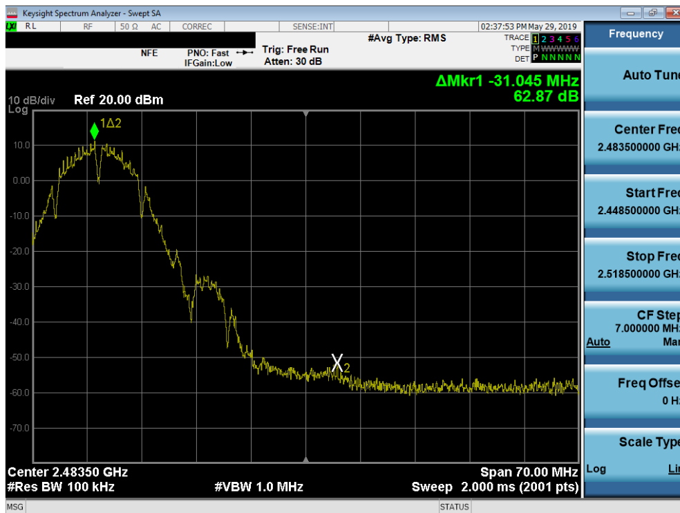
Plot 7-67. Band Edge Plot SISO ANT2 (802.11b – Ch. 10)
