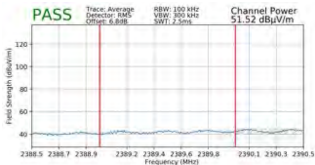
Plot 7-133. Radiated Restricted Lower Band Edge Measurement CDD (Average)
