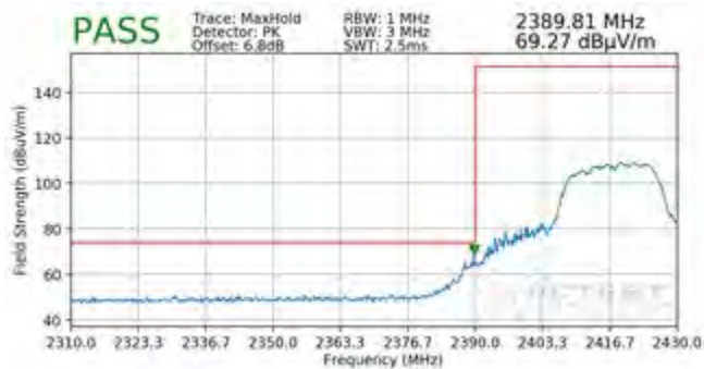
Plot 7-124. Radiated Restricted Lower Band Edge Measurement MIMO (Peak)
