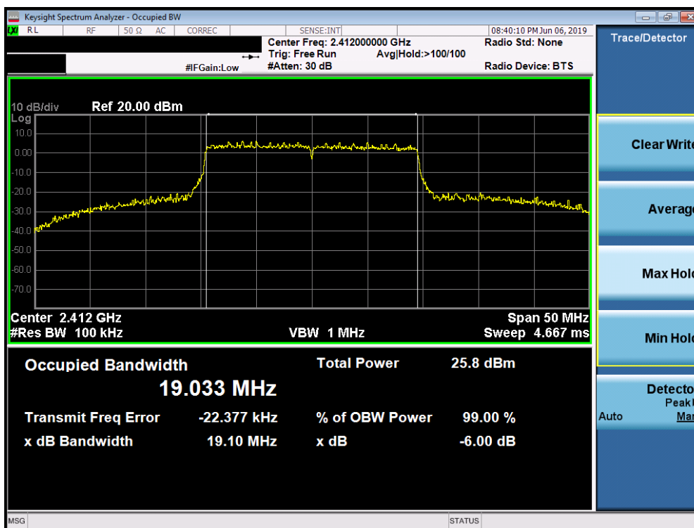
Plot 7-10. 6dB Bandwidth Plot SISO ANT1 (802.11ax (2.4GHz) – Ch. 1)
