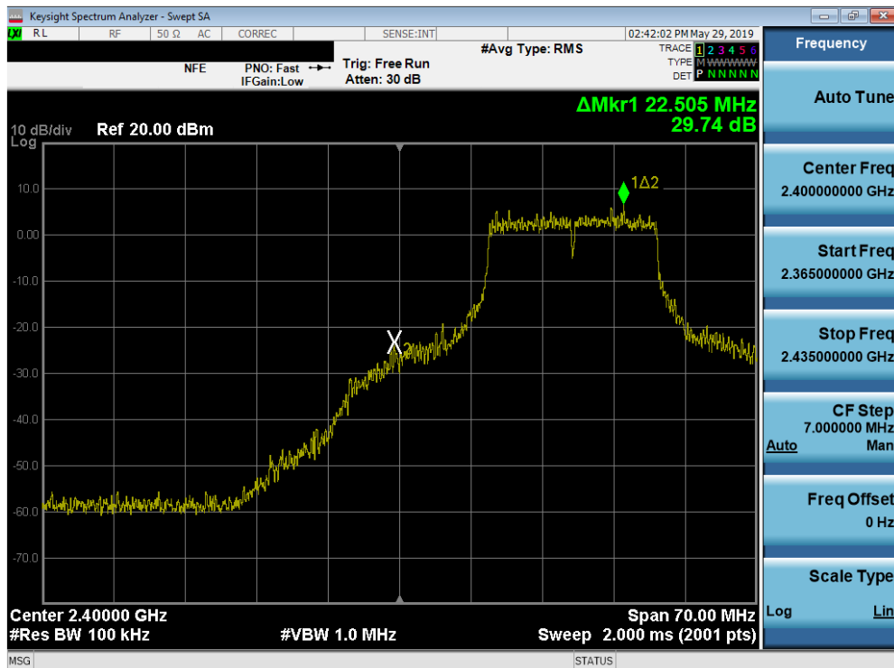
Plot 7-70. Band Edge Plot SISO ANT2 (802.11g - Ch. 2)
