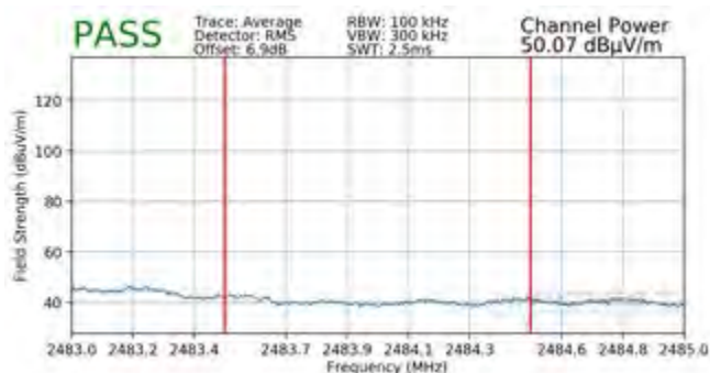
Plot 7-127. Radiated Restricted Upper Band Edge Measurement MIMO (Average)
