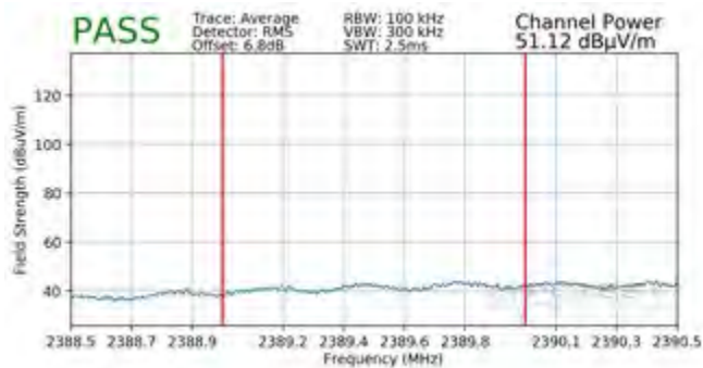
Plot 7-121. Radiated Restricted Lower Band Edge Measurement MIMO (Average)
