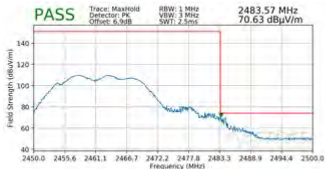
Plot 7-138. Radiated Restricted Upper Band Edge Measurement CDD (Peak)
