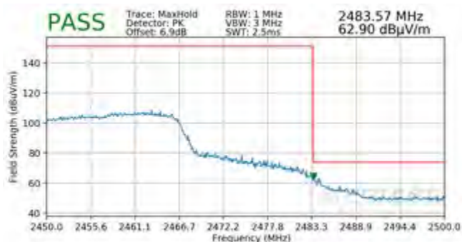
Plot 7-130. Radiated Restricted Band Edge Measurement MIMO with WCP (Peak)
