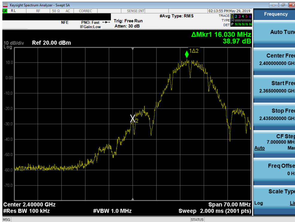
Plot 7-50. Band Edge Plot SISO ANT1 (802.11b – Ch. 2)
