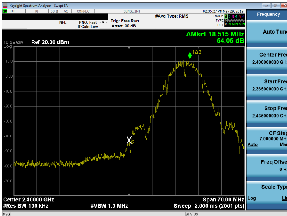
Plot 7-66. Band Edge Plot SISO ANT2 (802.11b - Ch. 2)
