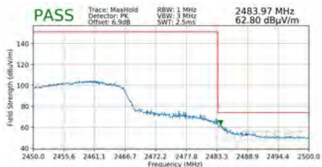
Plot 7-118. Radiated Restricted Upper Band Edge Measurement SISO ANT2 (Peak)
