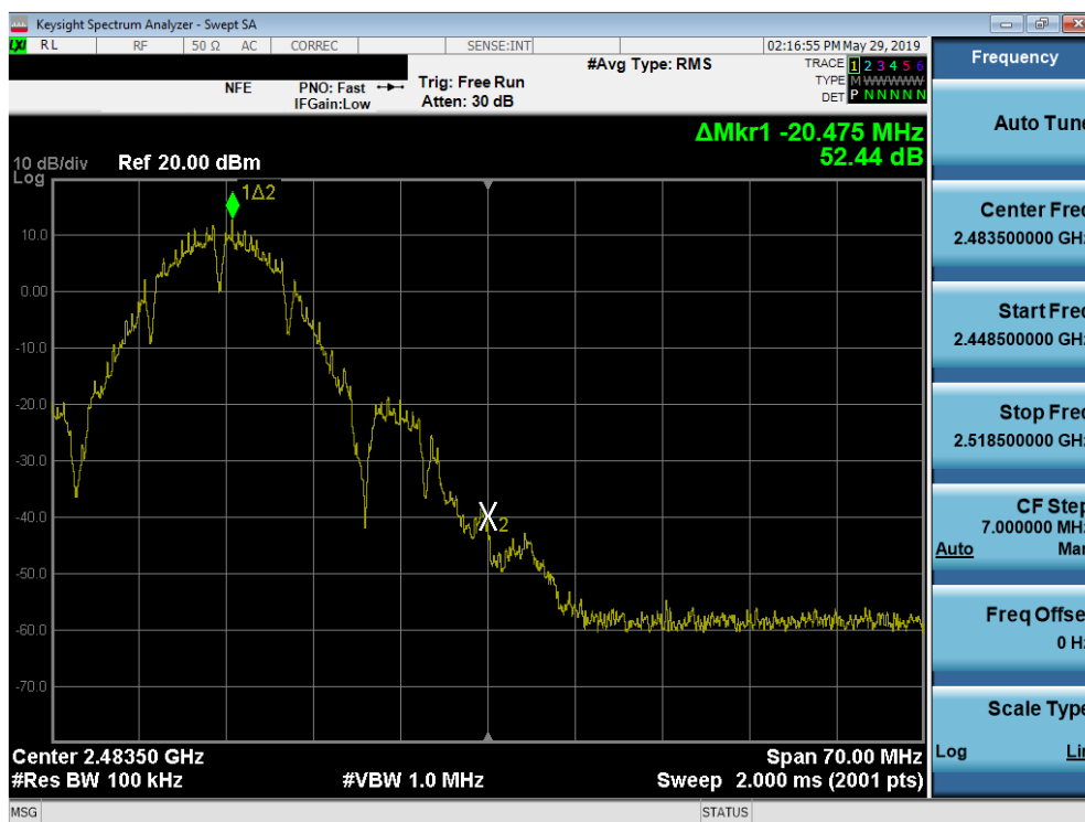
Plot 7-52. Band Edge Plot SISO ANT1 (802.11b – Ch. 11)
