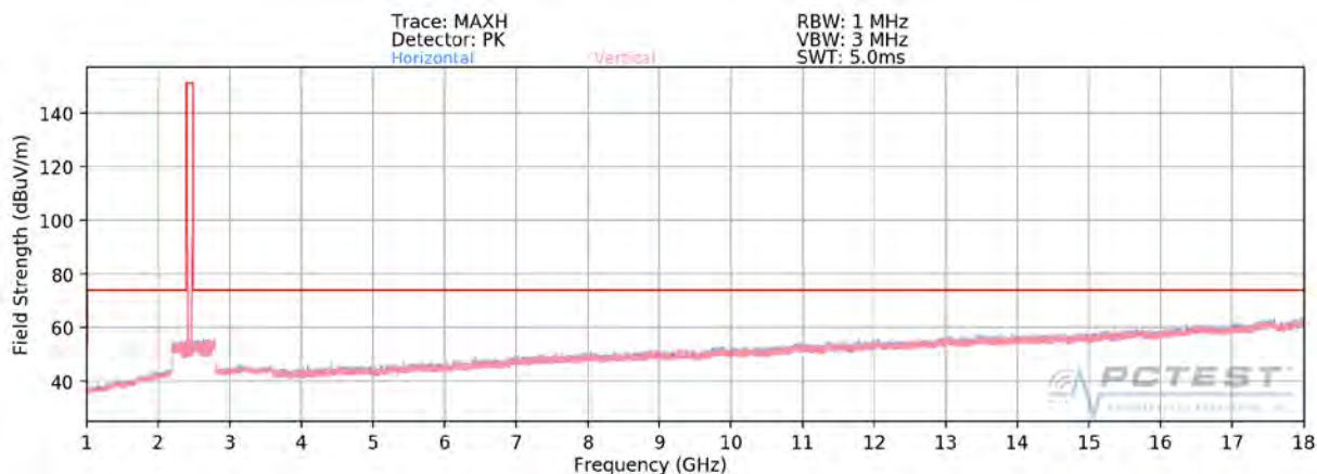
Plot 7-95. Radiated Spurious Plot above 1GHz SISO ANT1 (802.11b – Ch. 11)
