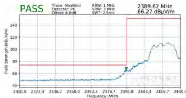
Plot 7-134. Radiated Restricted Lower Band Edge Measurement CDD (Peak)
