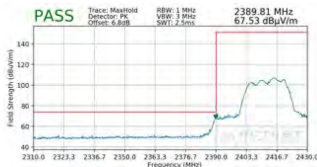
Plot 7-132. Radiated Restricted Lower Band Edge Measurement CDD (Peak)
