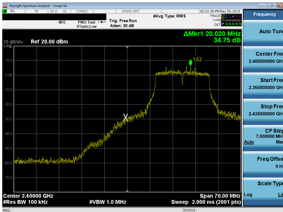
Plot 7-54. Band Edge Plot SISO ANT1 (802.11g - Ch. 2)
