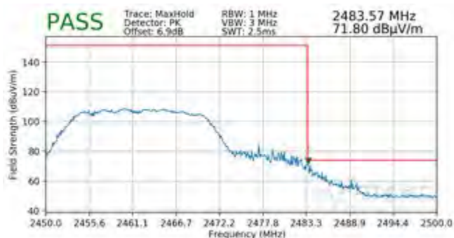
Plot 7-128. Radiated Restricted Upper Band Edge Measurement MIMO (Peak)
