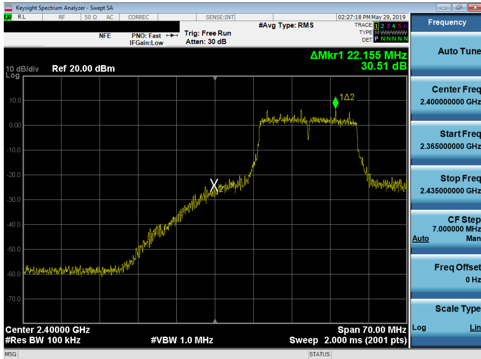
Plot 7-58. Band Edge Plot SISO ANT1 (802.11n(2.4GHz) – Ch. 2)
