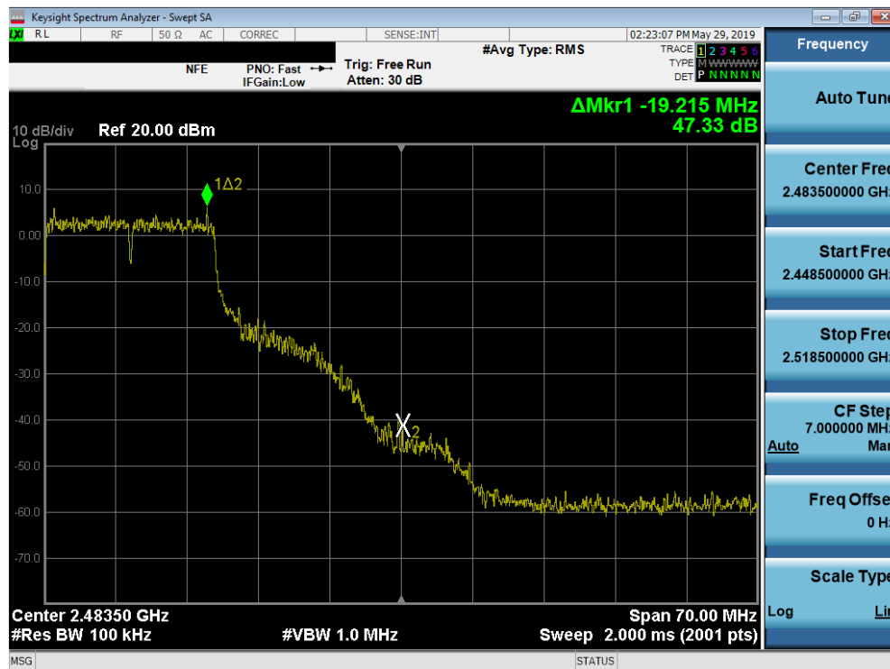
Plot 7-55. Band Edge Plot SISO ANT1 (802.11g – Ch. 10)
