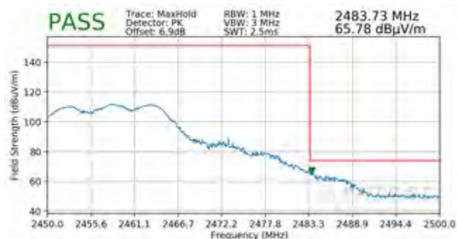
Plot 7-136. Radiated Restricted Upper Band Edge Measurement CDD (Peak)
