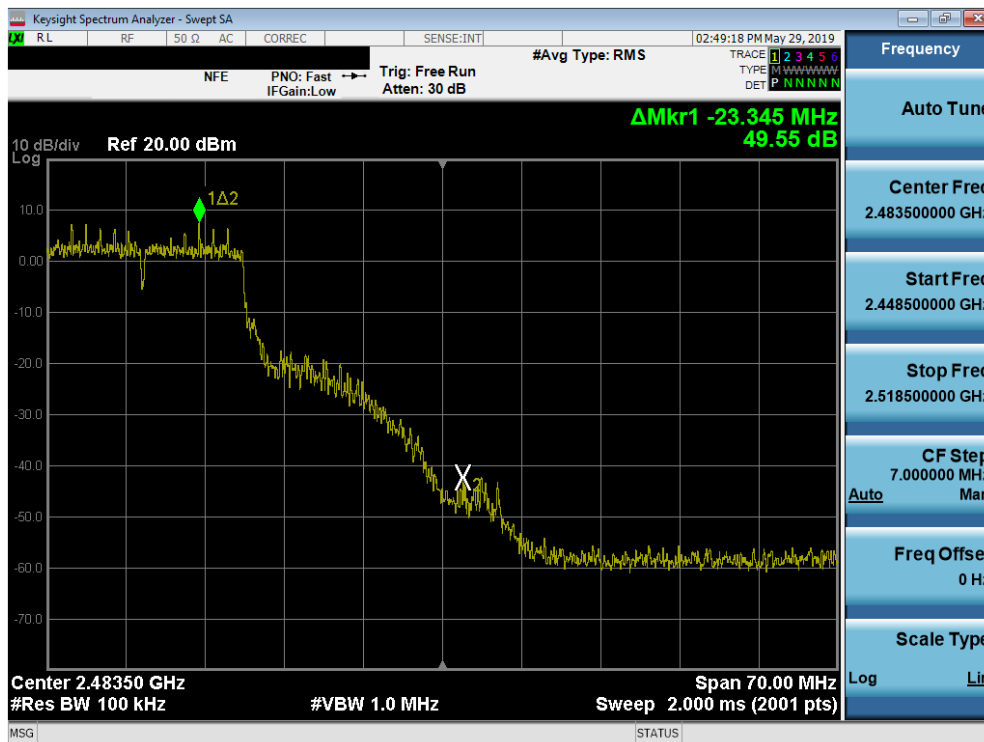
Plot 7-75. Band Edge Plot SISO ANT2 (802.11n(2.4GHz) – Ch. 10)
