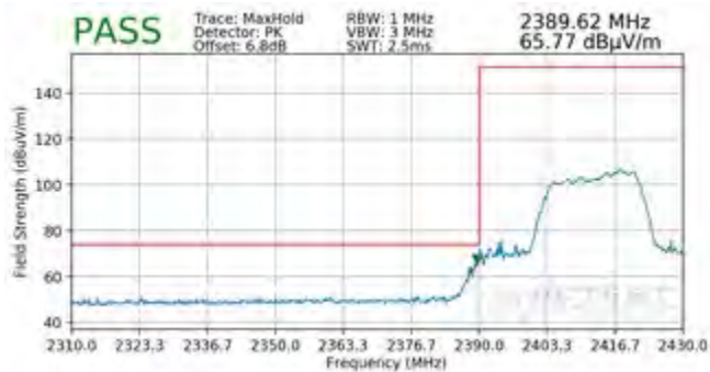
Plot 7-122. Radiated Restricted Lower Band Edge Measurement MIMO (Peak)
