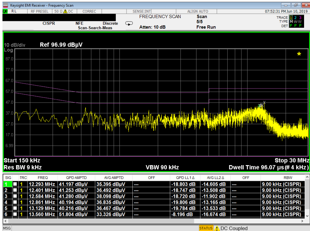
Plot 7-144. Line Conducted Plot with 802.11b (L1) with Wireless Charging Pad
