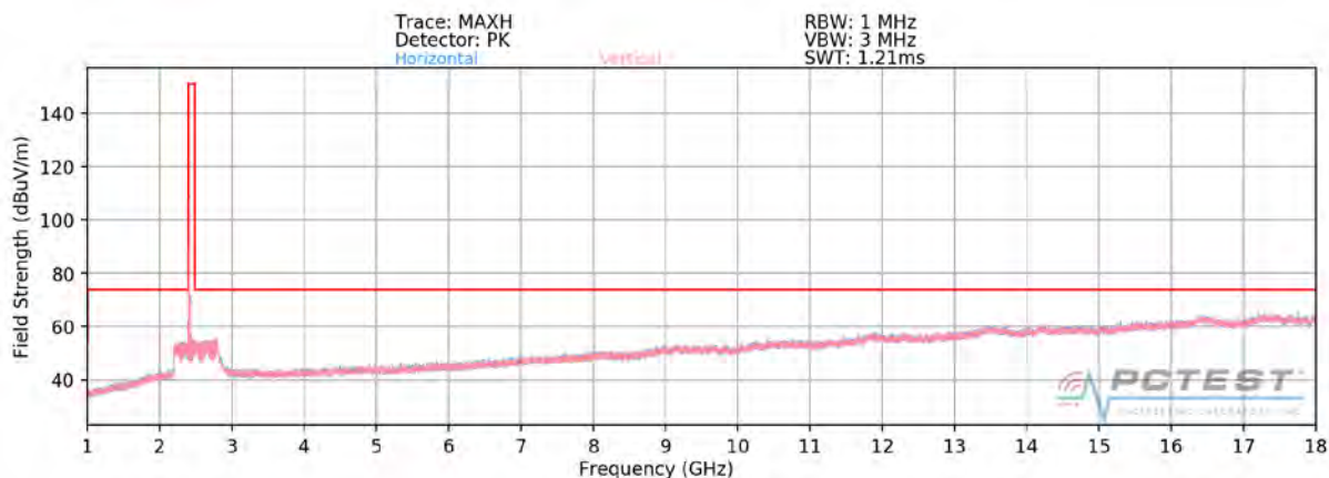
Plot 7-101. Radiated Spurious Plot above 1GHz MIMO/CDD (802.11g – Ch. 1)
