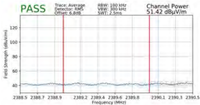
Plot 7-123. Radiated Restricted Lower Band Edge Measurement MIMO (Average)
