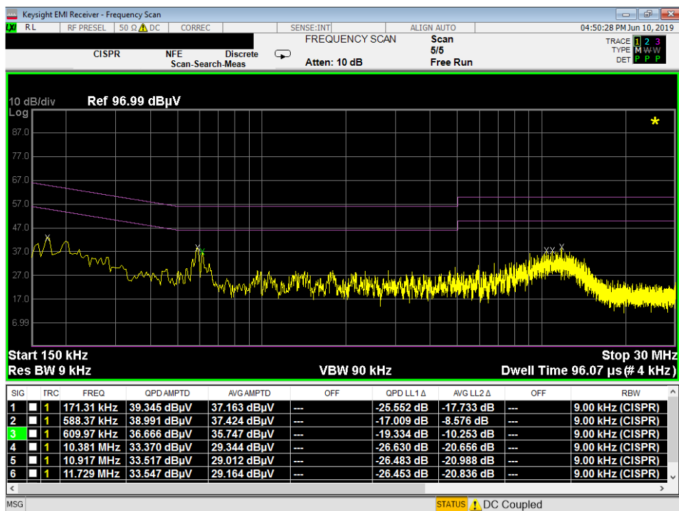
Plot 7-143. Line Conducted Plot with 802.11b (N) with Travel Adapter
