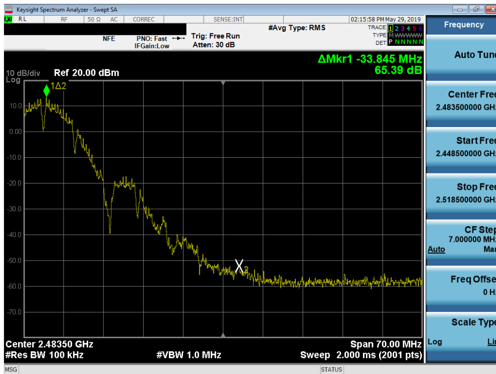
Plot 7-51. Band Edge Plot SISO ANT1 (802.11b – Ch. 10)
