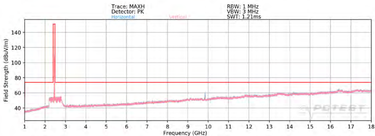
Plot 7-103. Radiated Spurious Plot above 1GHz MIMO/CDD (802.11g – Ch. 11)
