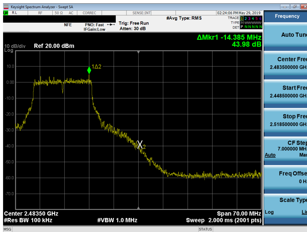
Plot 7-56. Band Edge Plot SISO ANT1 (802.11g – Ch. 11)
