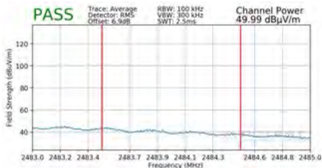
Plot 7-137. Radiated Restricted Upper Band Edge Measurement CDD (Average)
