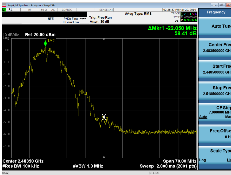
Plot 7-68. Band Edge Plot SISO ANT2 (802.11b – Ch. 11)
