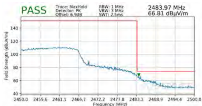
Plot 7-126. Radiated Restricted Upper Band Edge Measurement MIMO (Peak)
