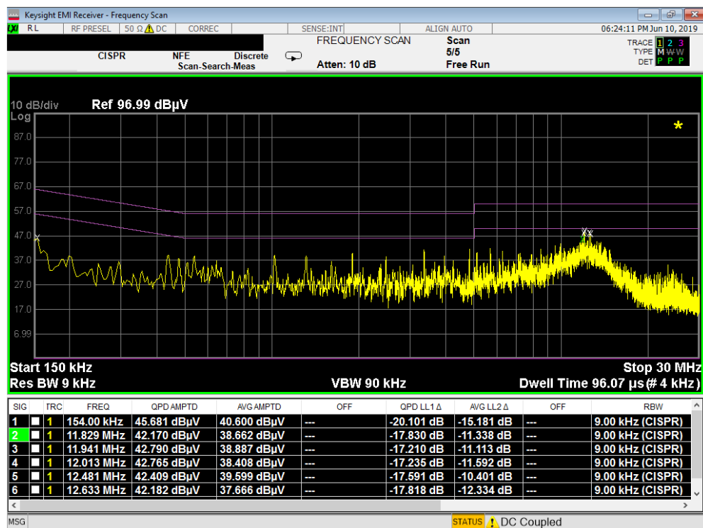
Plot 7-14. Line-Conducted Test Plot (N) – Device to Device
