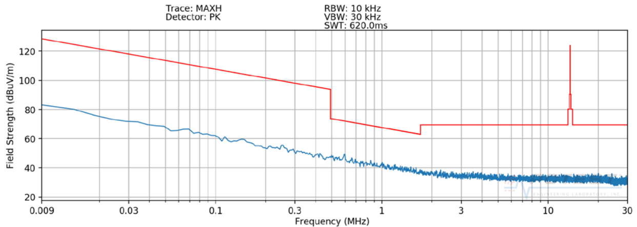
Plot 7-2Radiated Spurious Plot 9kHz – 30MHz (Pol. Y – WPT - Device to Device)
