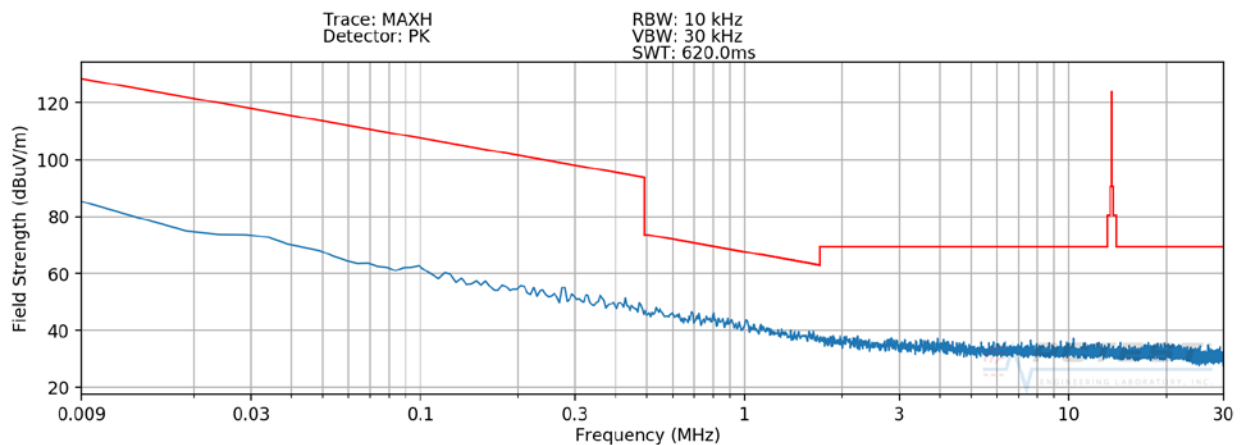
Plot 7-3. Radiated Spurious Plot 9kHz – 30MHz (Pol. Z – WPT - Device to Device)
