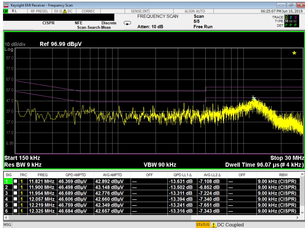
Plot 7-13. Line-Conducted Test Plot (L1) – Device to Device
