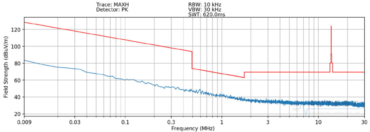
Plot 7-1. Radiated Spurious Plot 9kHz – 30MHz (Pol. X - WPT- Device to Device)
