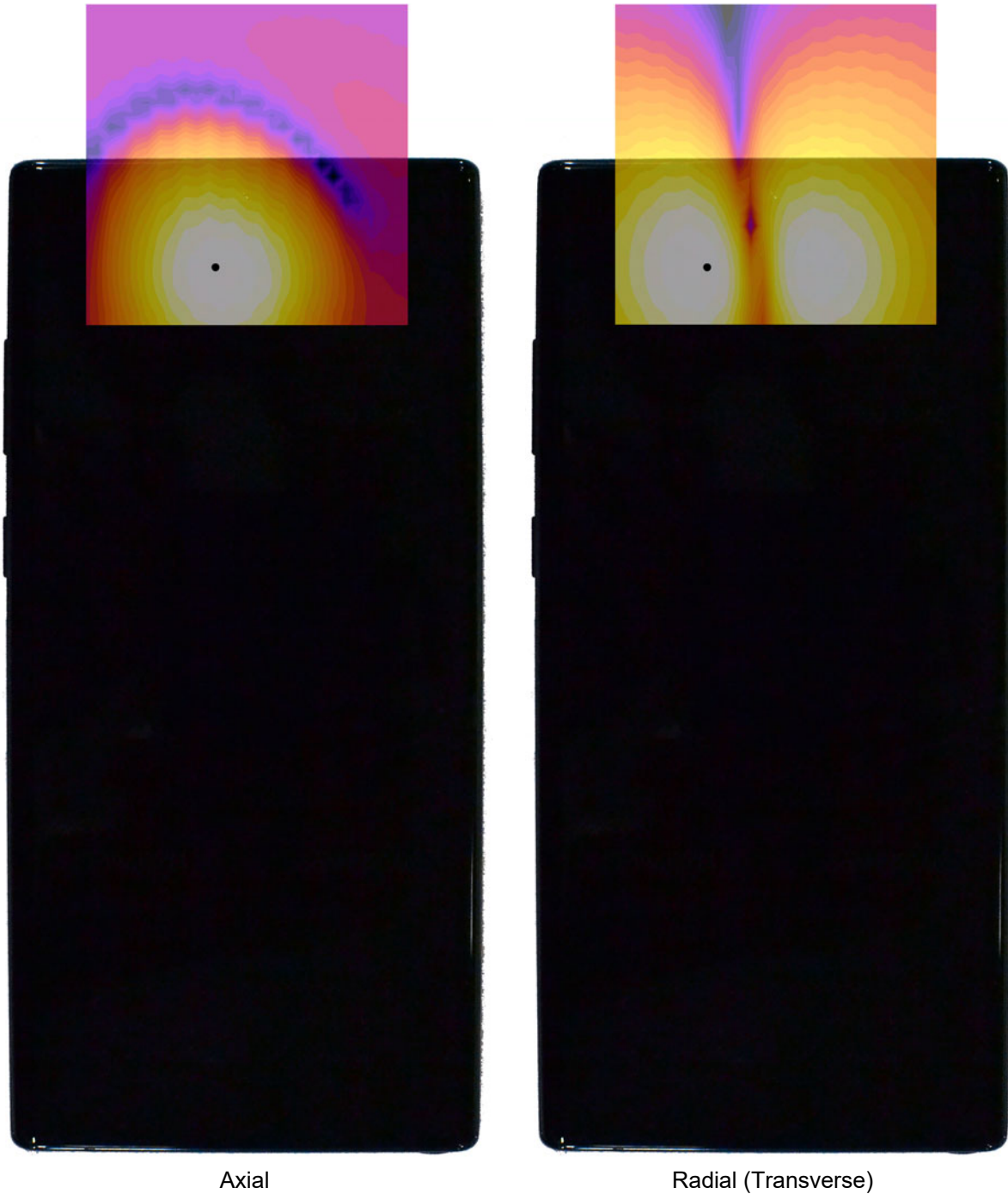
Axial Radial (Transverse) Figure 16-3 T-Coil Scan Overlay Magnetic Field Distributions
