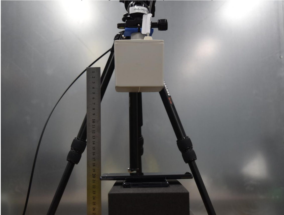
Top – charger below client (20cm distance)
