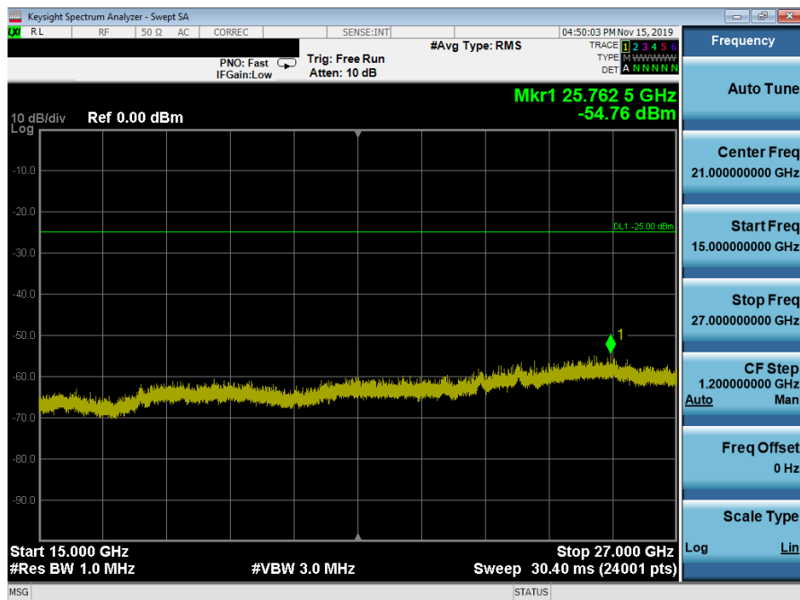
Plot 7-34. Conducted Spurious Plot (n41 - 100MHz DFT-QPSK - RB Size 1, RB Offset 0 - Mid Channel)
