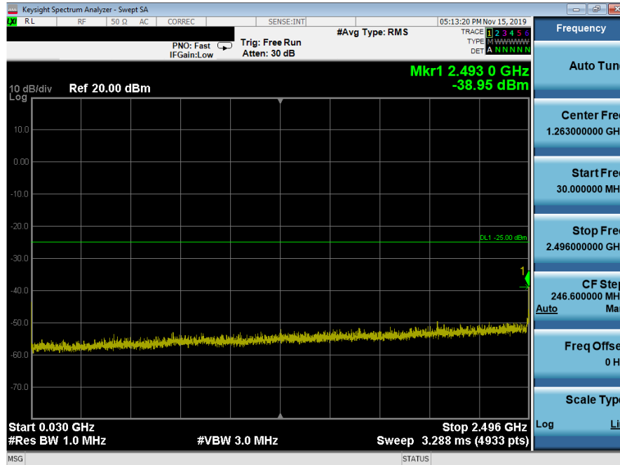
Plot 7-35. Conducted Spurious Plot (n41 - 100MHz DFT-QPSK - RB Size 1, RB Offset 0 - High Channel)
