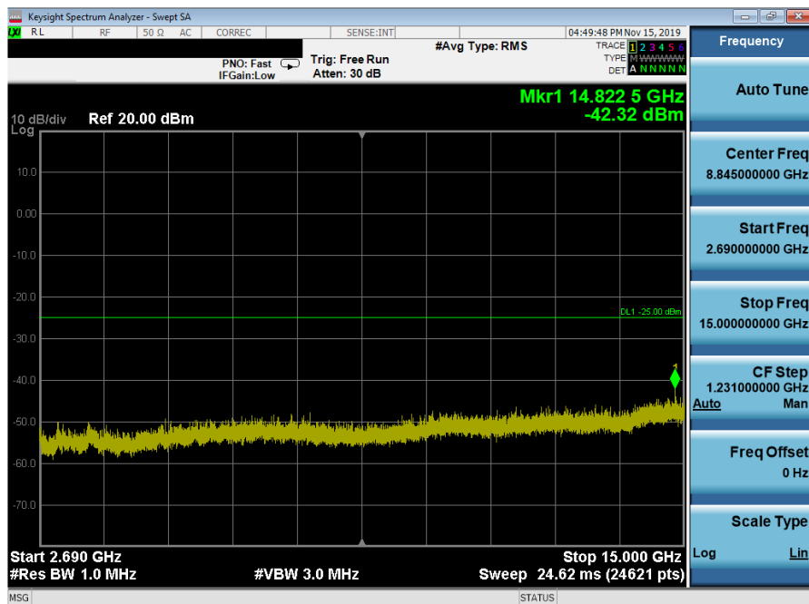
Plot 7-33. Conducted Spurious Plot (n41 - 100MHz DFT-QPSK - RB Size 1, RB Offset 0 - Mid Channel)
