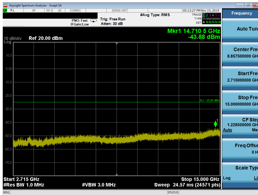
Plot 7-36. Conducted Spurious Plot (n41 - 100MHz DFT-QPSK - RB Size 1, RB Offset 0 - High Channel)
