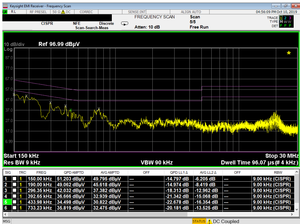
Plot 7-9. Line-Conducted Test Plot (N) with Antenna Terminated in 50 Ω
