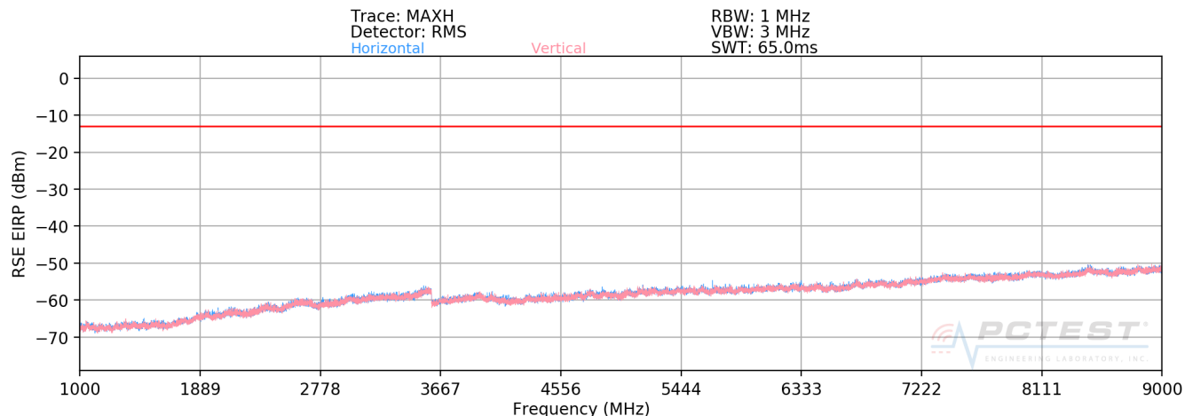
Plot 7-53. Radiated Spurious Plot above 1GHz (Band 26)
