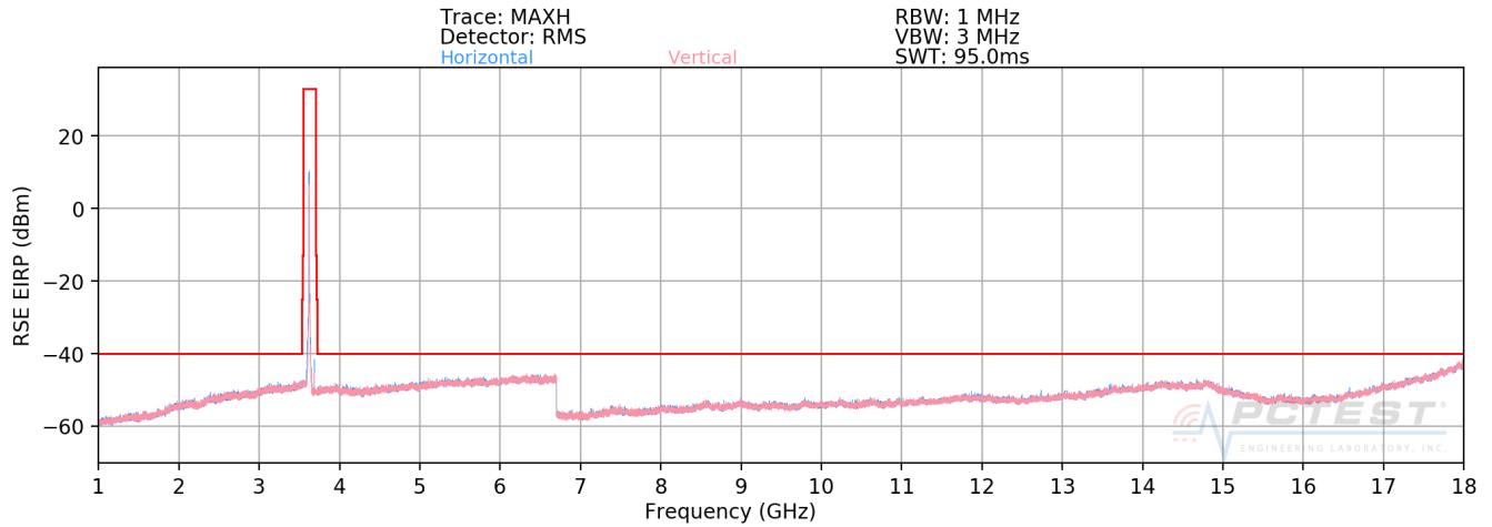
Plot 7-41. Radiated Spurious Plot 1 - 18GHz (Band 48)
