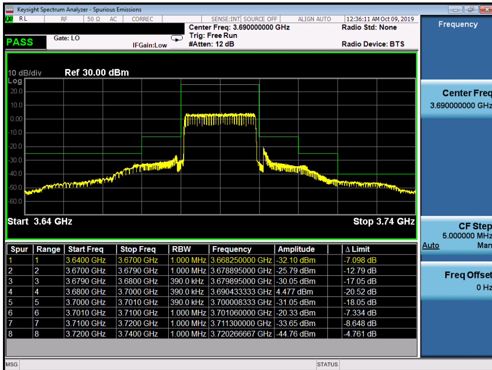
Plot 7-40. Upper ACP Plot (LTE Band 48 - 20.0MHz QPSK - Full RB Configuration)
