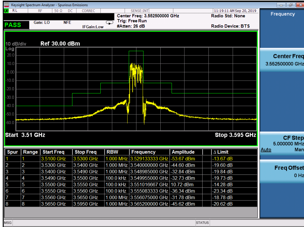
Plot 7-29. Lower ACP Plot (LTE Band 48 - 5.0MHz QPSK - Full RB Configuration)
