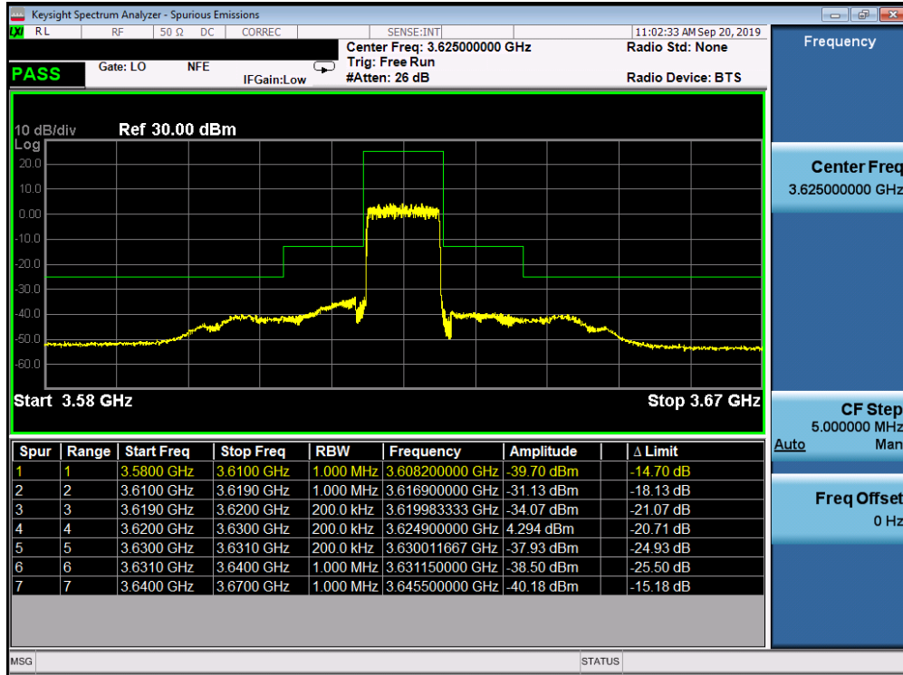
Plot 7-33. Mid ACP Plot (LTE Band 48 - 10.0MHz QPSK - Full RB Configuration)
