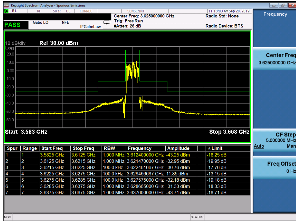
Plot 7-30. Mid ACP Plot (LTE Band 48 - 5.0MHz QPSK - Full RB Configuration)
