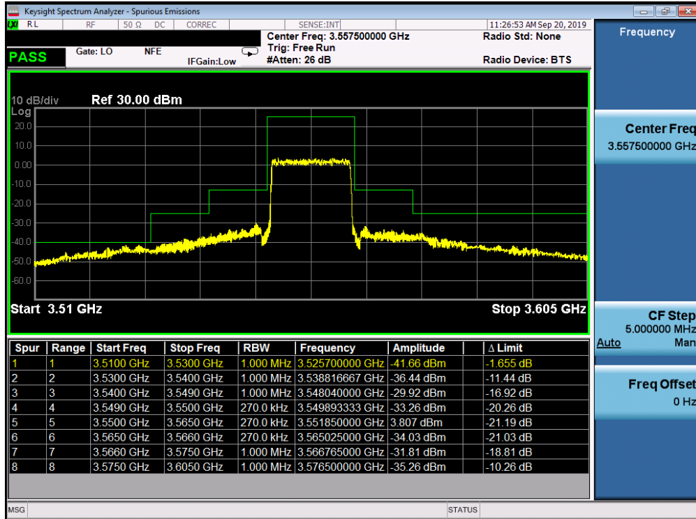
Plot 7-35. Lower ACP Plot (LTE Band 48 - 15.0MHz QPSK - Full RB Configuration)
