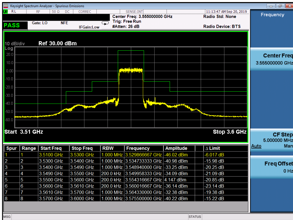
Plot 7-32. Lower ACP Plot (LTE Band 48 - 10.0MHz QPSK - Full RB Configuration)
