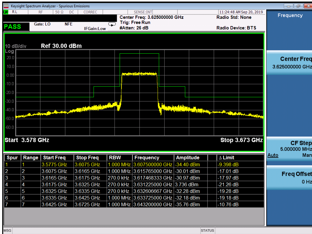
Plot 7-36. Mid ACP Plot (LTE Band 48 - 15.0MHz QPSK - Full RB Configuration)
