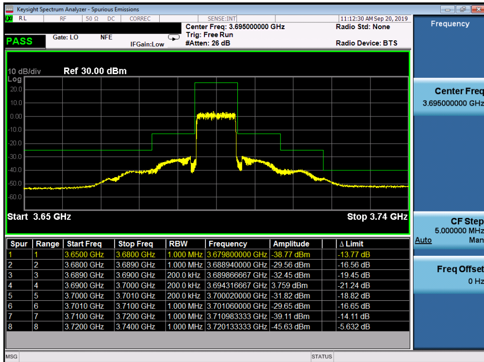
Plot 7-34. Upper ACP Plot (LTE Band 48 - 10.0MHz QPSK - Full RB Configuration)
