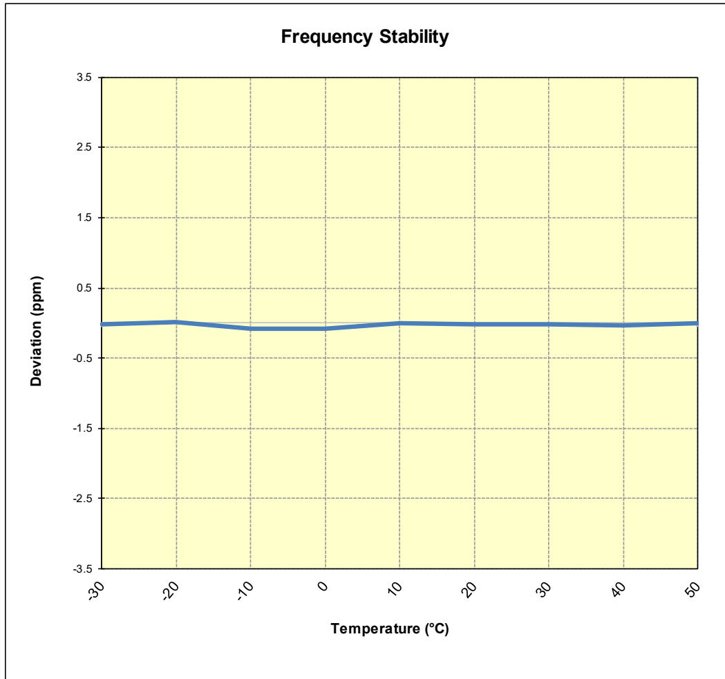
Figure 7-6. Frequency Stability Graph (LTE Band 48)
