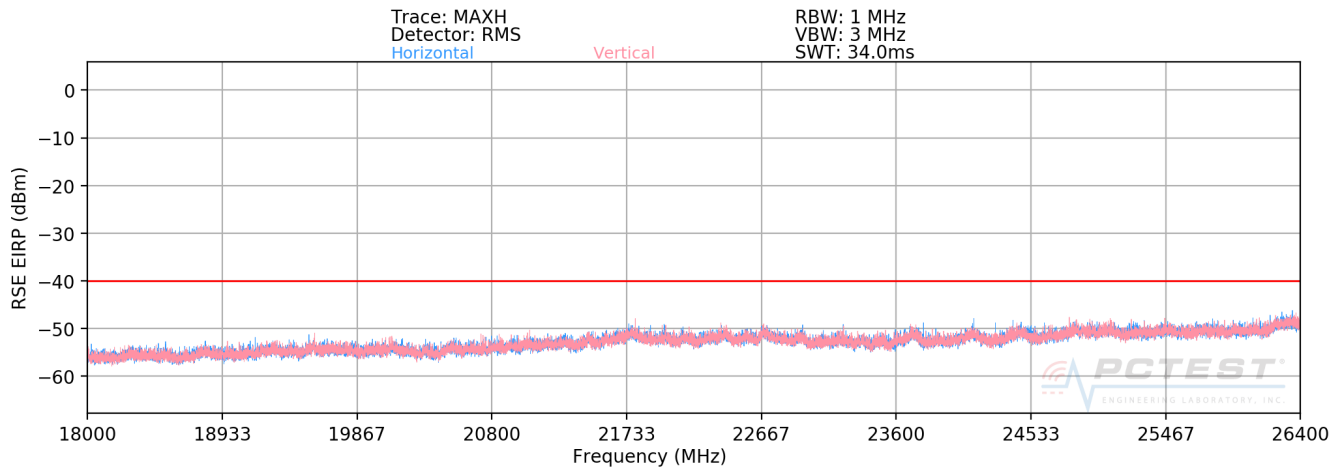
Plot 7-42. Radiated Spurious Plot 18 - 26.5GHz (Band 48)
