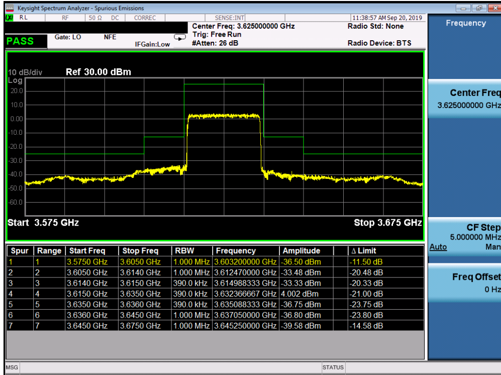
Plot 7-39. Mid ACP Plot (LTE Band 48 - 20.0MHz QPSK - Full RB Configuration)
