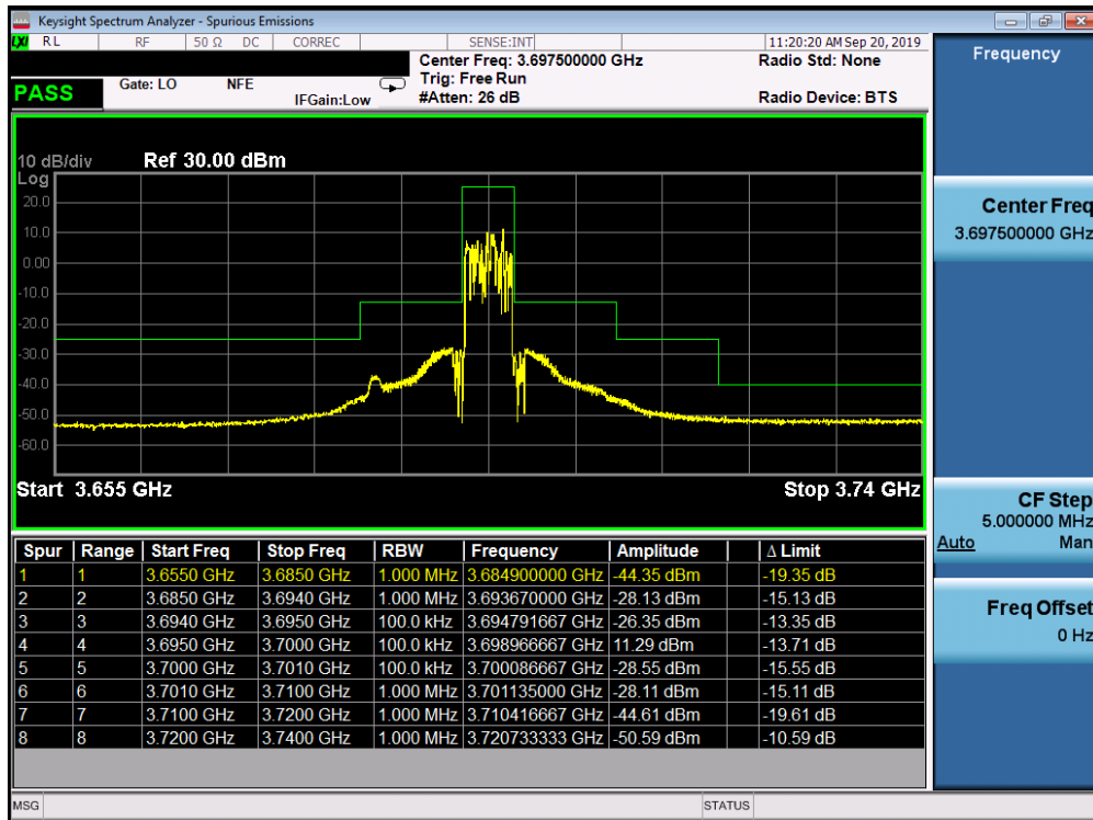
Plot 7-31. Upper ACP Plot (LTE Band 48 - 5.0MHz QPSK - Full RB Configuration)
