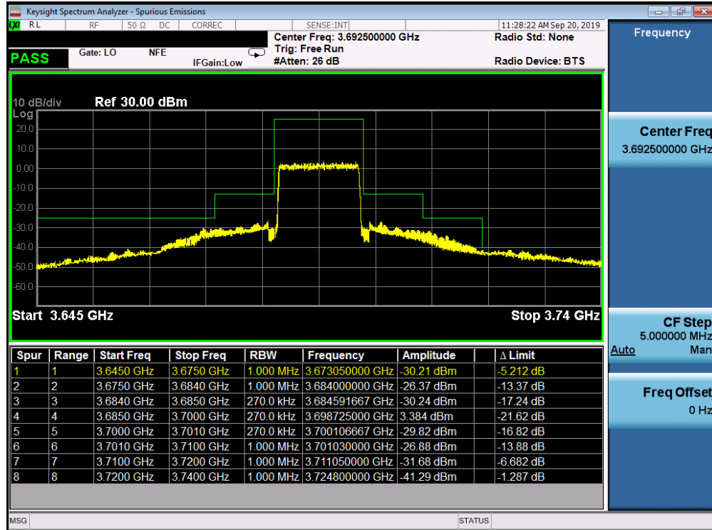
Plot 7-37. Upper ACP Plot (LTE Band 48 - 15.0MHz QPSK - Full RB Configuration)
