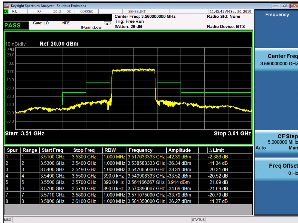
Plot 7-38. Lower ACP Plot (LTE Band 48 - 20.0MHz QPSK - Full RB Configuration)
