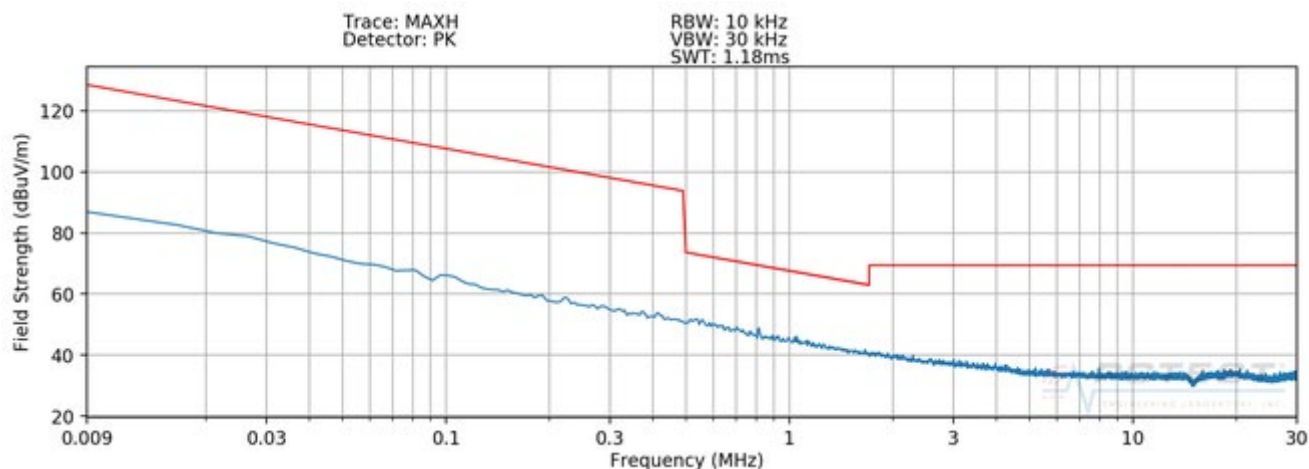
Plot 7-6. Radiated Spurious Plot 9kHz – 30MHz (Pol. Z – Device to S-Pen WPT)
