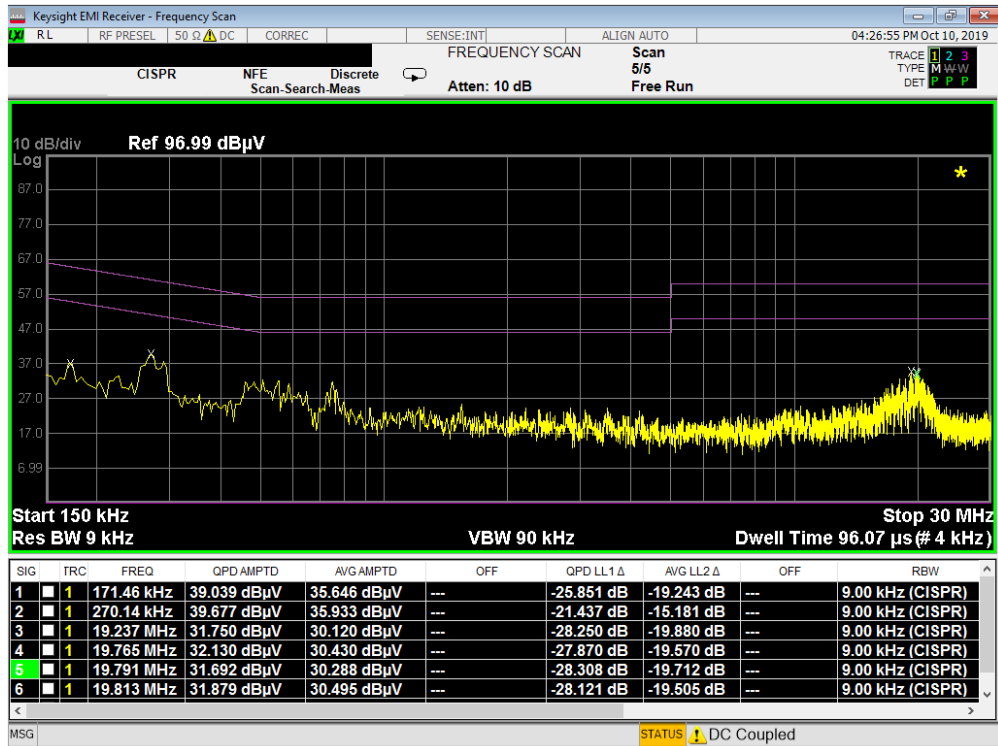
Plot 7-15. Line-Conducted Test Plot (L1) - Device to S-Pen WPT
