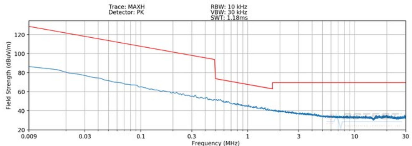
Plot 7-12. Radiated Spurious Plot 9kHz – 30MHz (Pol. Z – Digitizer Mode 2)
