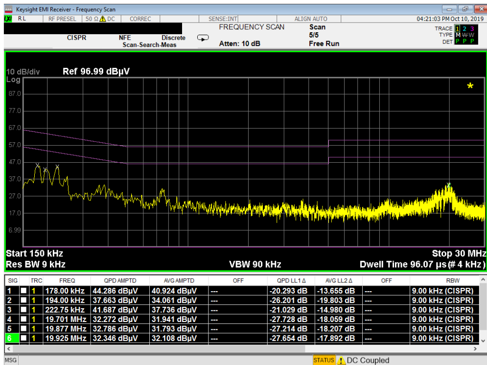
Plot 7-19. Line-Conducted Test Plot (L1) - Digitizer Mode 2
