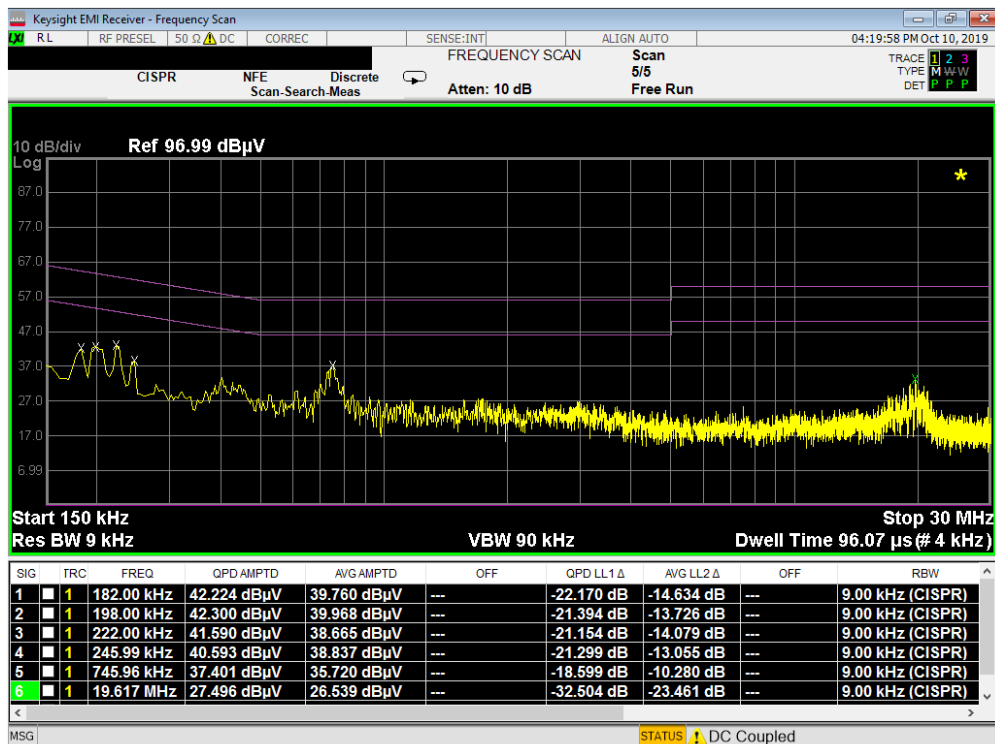
Plot 7-20. Line-Conducted Test Plot (N) - Digitizer Mode 2
