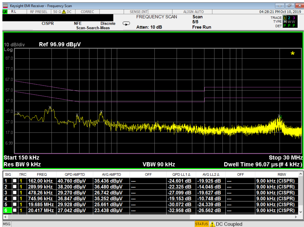
Plot 7-16. Line-Conducted Test Plot (N) - Device to S-pen WPT
