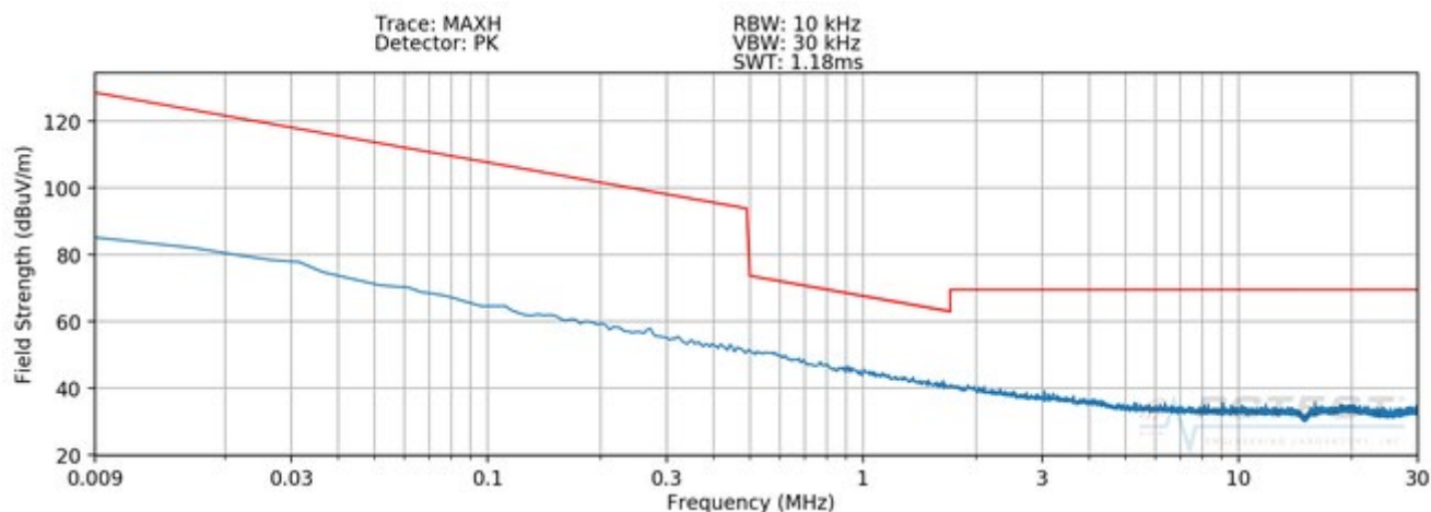
Plot 7-9. Radiated Spurious Plot 9kHz – 30MHz (Pol. Z – Digitizer Mode 1)
