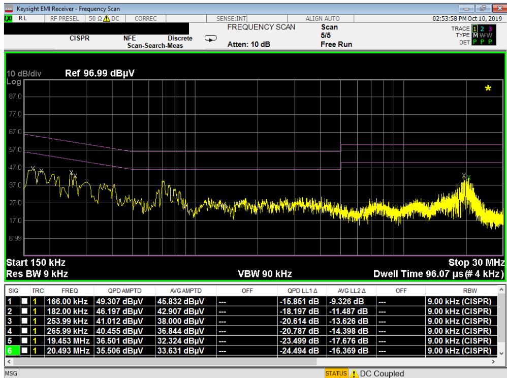
Plot 7-18. Line-Conducted Test Plot (N) - Digitizer Mode 1
