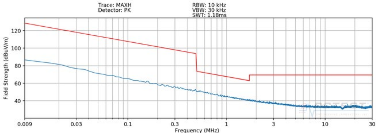
lot 7-7. Radiated Spurious Plot 9kHz – 30MHz (Pol. X – Digitizer Mode 1)
