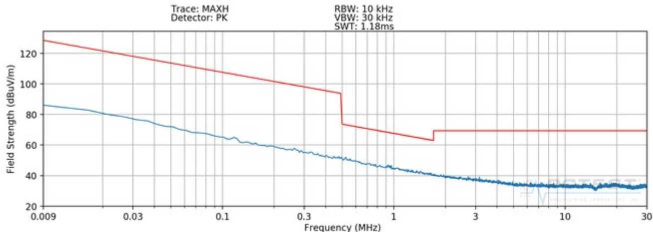
Plot 7-4. Radiated Spurious Plot 9kHz – 30MHz (Pol. X – Device to S-Pen WPT)
