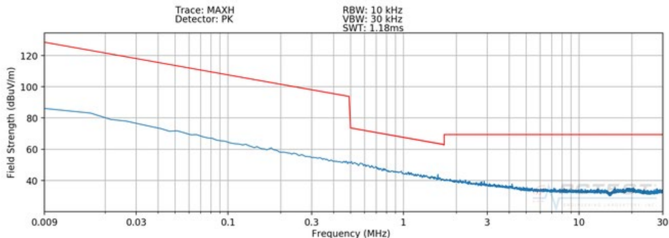
Plot 7-8 Radiated Spurious Plot 9kHz – 30MHz (Pol. Y – Digitizer Mode 1)
