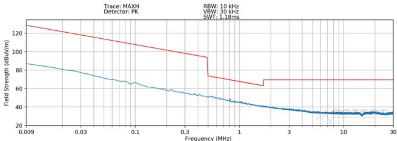
Plot 7-5 Radiated Spurious Plot 9kHz – 30MHz (Pol. Y – Device to S-Pen WPT)
