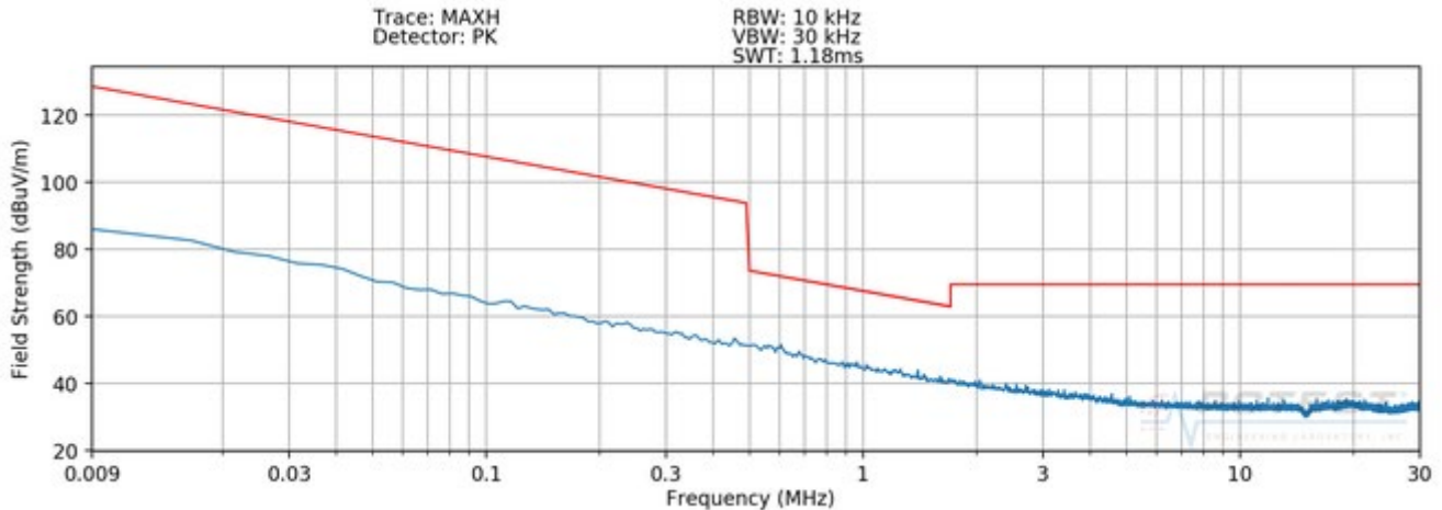
lot 7-10. Radiated Spurious Plot 9kHz – 30MHz (Pol. X – Digitizer Mode 2)
