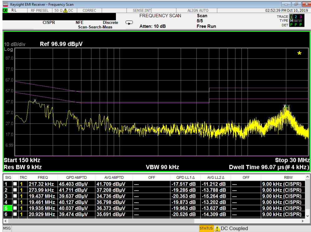
Plot 7-17. Line-Conducted Test Plot (L1) - Digitizer Mode 1
