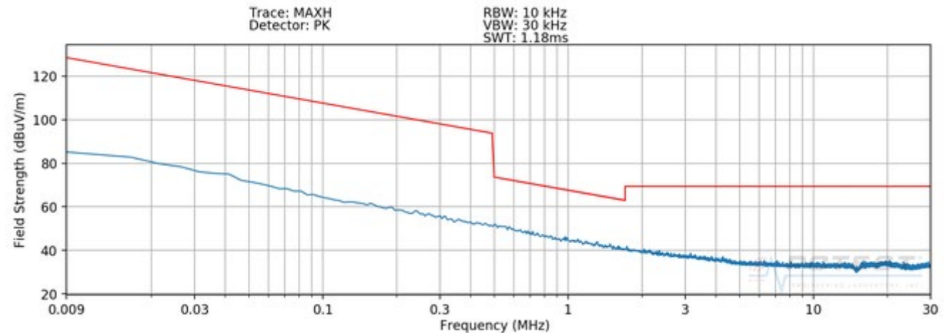
Plot 7-11Radiated Spurious Plot 9kHz – 30MHz (Pol. Y – Digitizer Mode 2)
