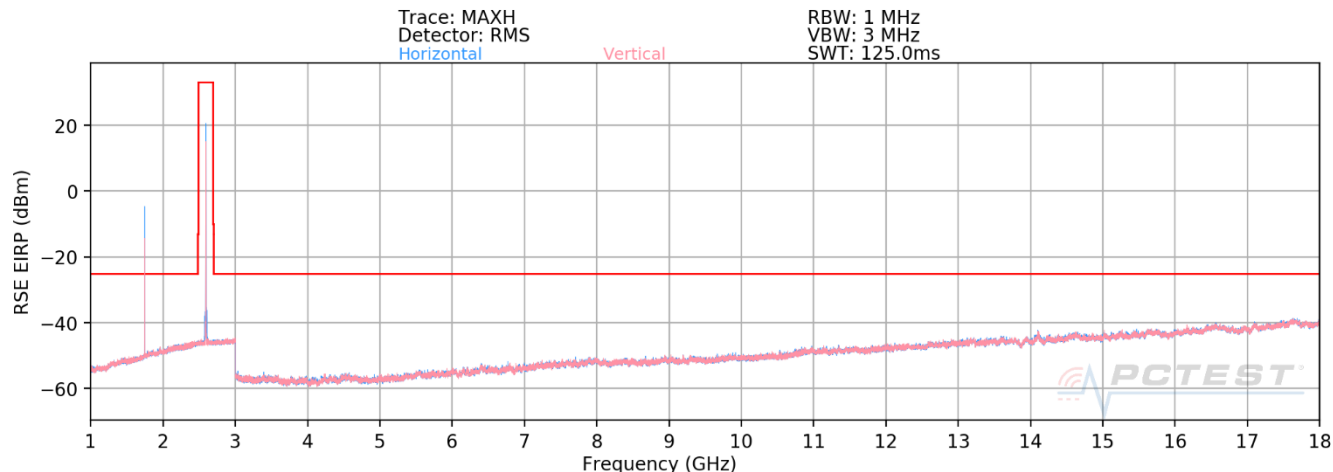
Plot 7-54. Radiated Spurious Plot 1GHz - 18GHz (EN-DC n41+ LTE B66)
