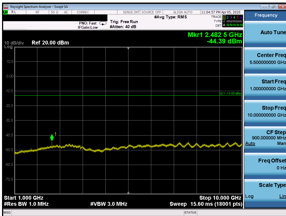
Plot 7-30. Conducted Spurious Plot (n5 - 20MHz DFT-s-OFDM-BPSK - RB Size 1, RB Offset 1 - Mid Channel)
