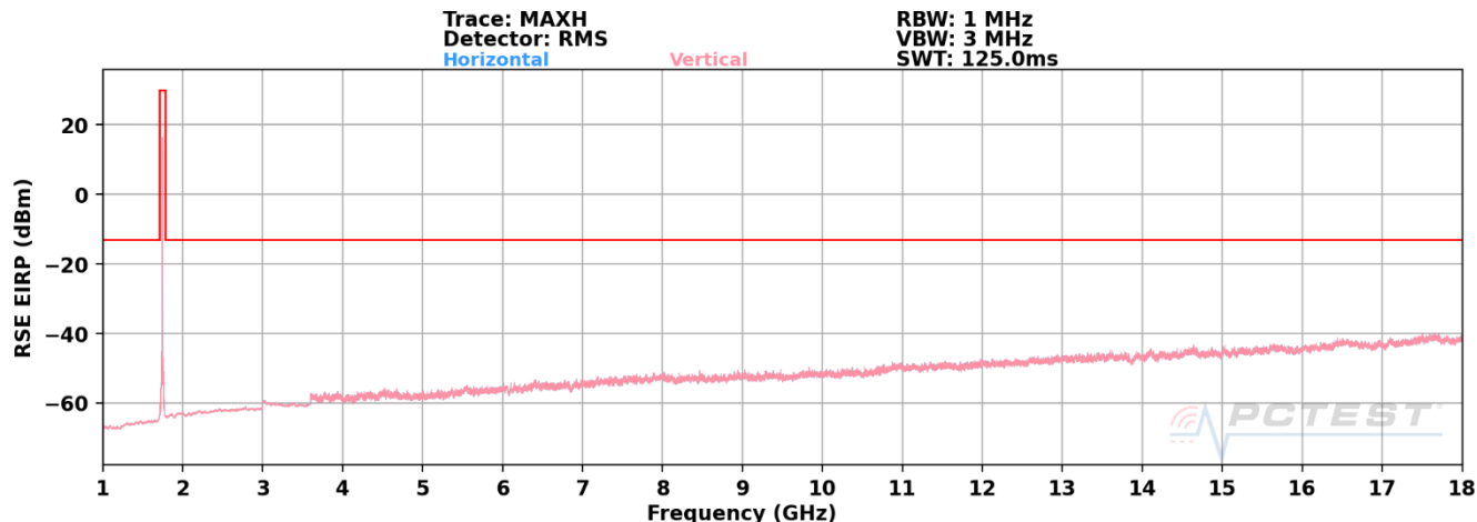
Plot 7-52. Radiated Spurious Plot above 1GHz (EN-DC n71 + LTE B66)
