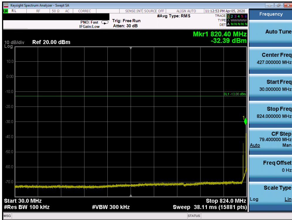
Plot 7-31. Conducted Spurious Plot (n5 - 20MHz DFT-s-OFDM-BPSK - RB Size 1, RB Offset 1 - High Channel)
