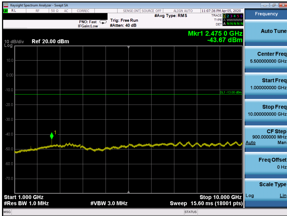
Plot 7-27. Conducted Spurious Plot (n5 - 20MHz DFT-s-OFDM-BPSK - RB Size 1, RB Offset 1 - Low Channel)
