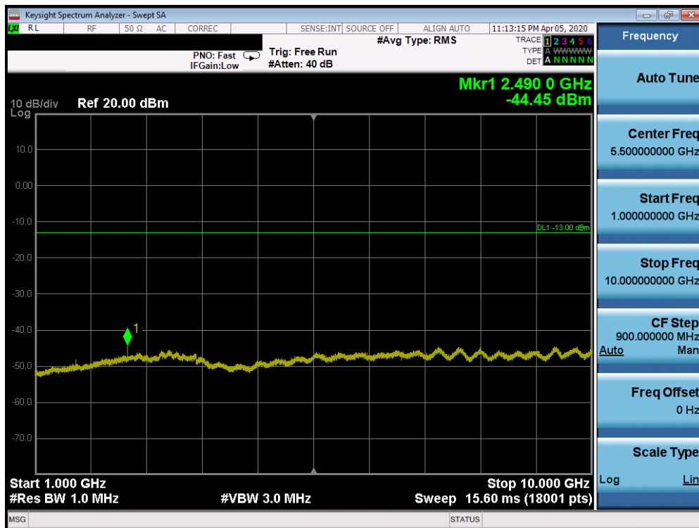
Plot 7-33. Conducted Spurious Plot (n5 - 20MHz DFT-s-OFDM-BPSK - RB Size 1, RB Offset 1 - High Channel)
