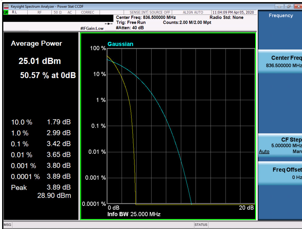
Plot 7-50. PAR Plot (Band n5 - 20.0MHz DFT-s-OFDM-BPSK - Full RB Configuration)
