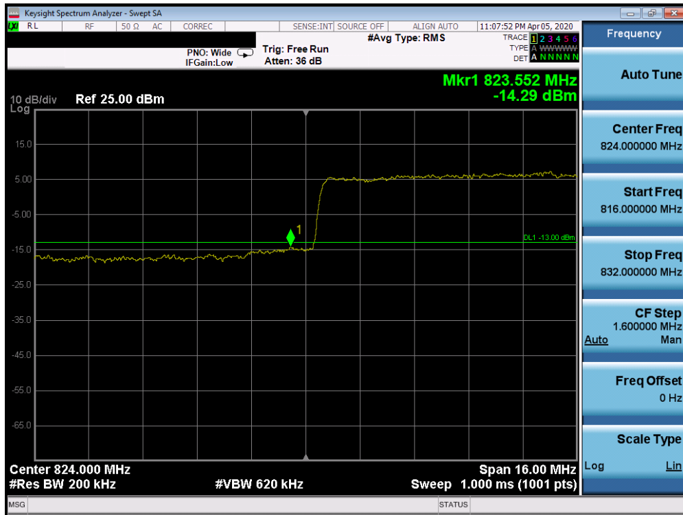
Plot 7-45. Lower Band Edge Plot (n5 - 20MHz DFT-s-OFDM-BPSK - Full RB Configuration)
