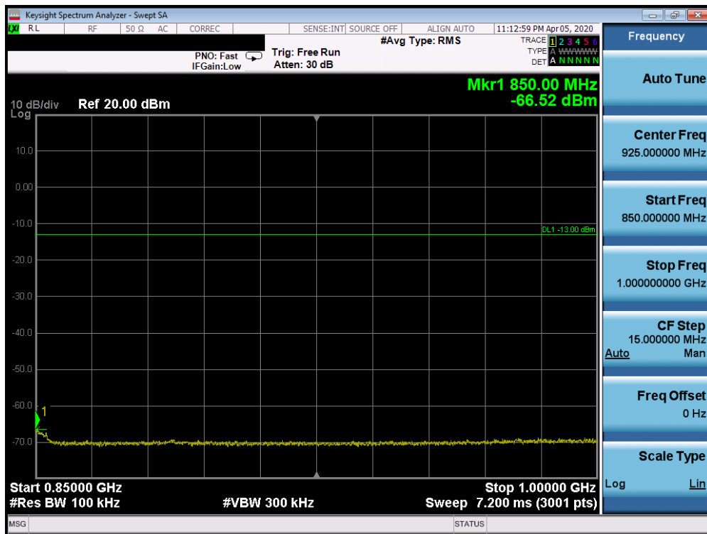
Plot 7-32. Conducted Spurious Plot (n5 - 20MHz DFT-s-OFDM-BPSK - RB Size 1, RB Offset 1 - High Channel)
