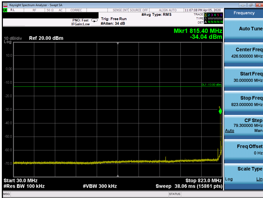
Plot 7-25. Conducted Spurious Plot (n5 - 20MHz DFT-s-OFDM-BPSK - RB Size 1, RB Offset 1 - Low Channel)
