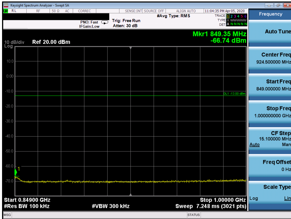
Plot 7-29. Conducted Spurious Plot (n5 - 20MHz DFT-s-OFDM-BPSK - RB Size 1, RB Offset 1 - Mid Channel)
