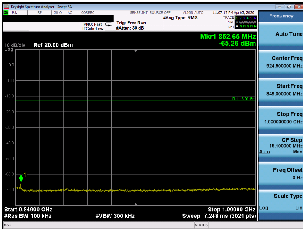
Plot 7-26. Conducted Spurious Plot (n5 - 20MHz DFT-s-OFDM-BPSK - RB Size 1, RB Offset 1 - Low Channel)
