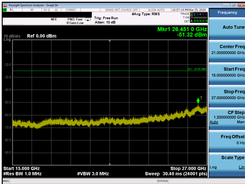
Plot 7-39. Conducted Spurious Plot (n41 - 100MHz DFT-s-OFDM-BPSK - RB Size 1, RB Offset 1 - Mid Channel)
