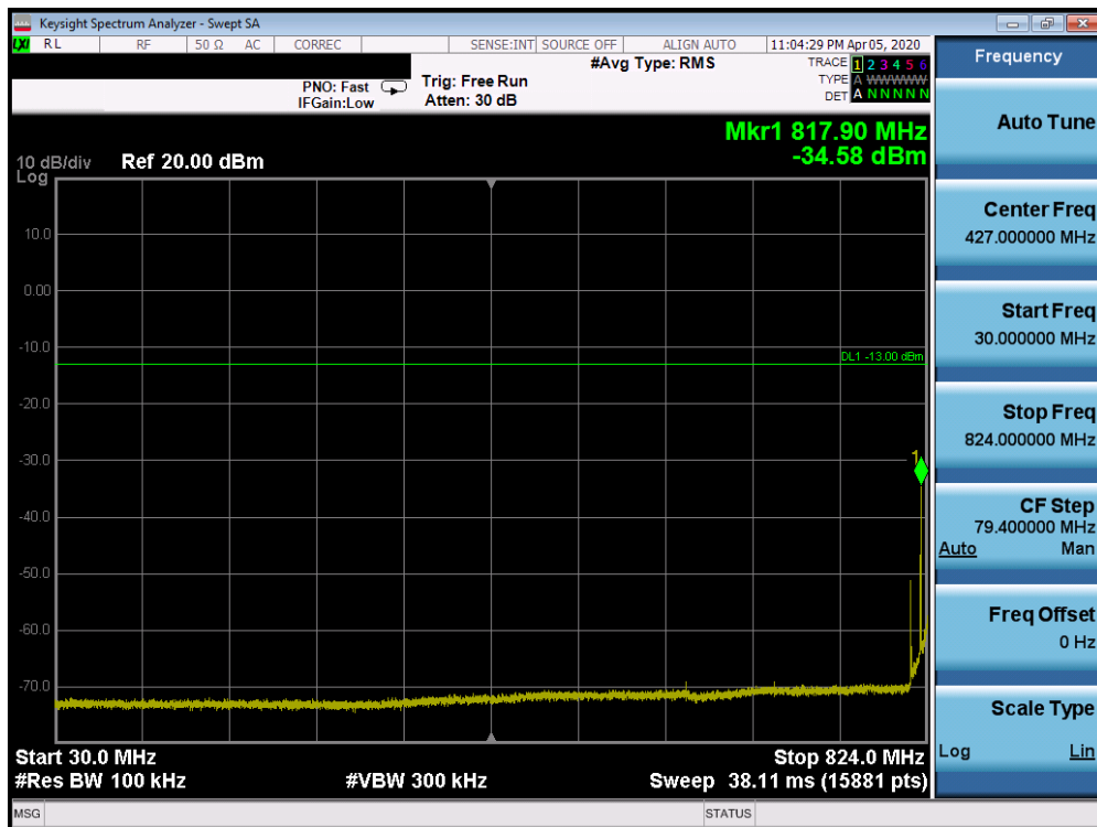
Plot 7-28. Conducted Spurious Plot (n5 - 20MHz DFT-s-OFDM-BPSK - RB Size 1, RB Offset 1 - Mid Channel)
