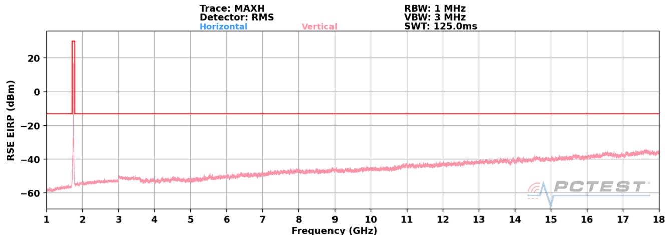
Plot 7-53. Radiated Spurious Plot above 1GHz (EN-DC n5+LTE B66)
