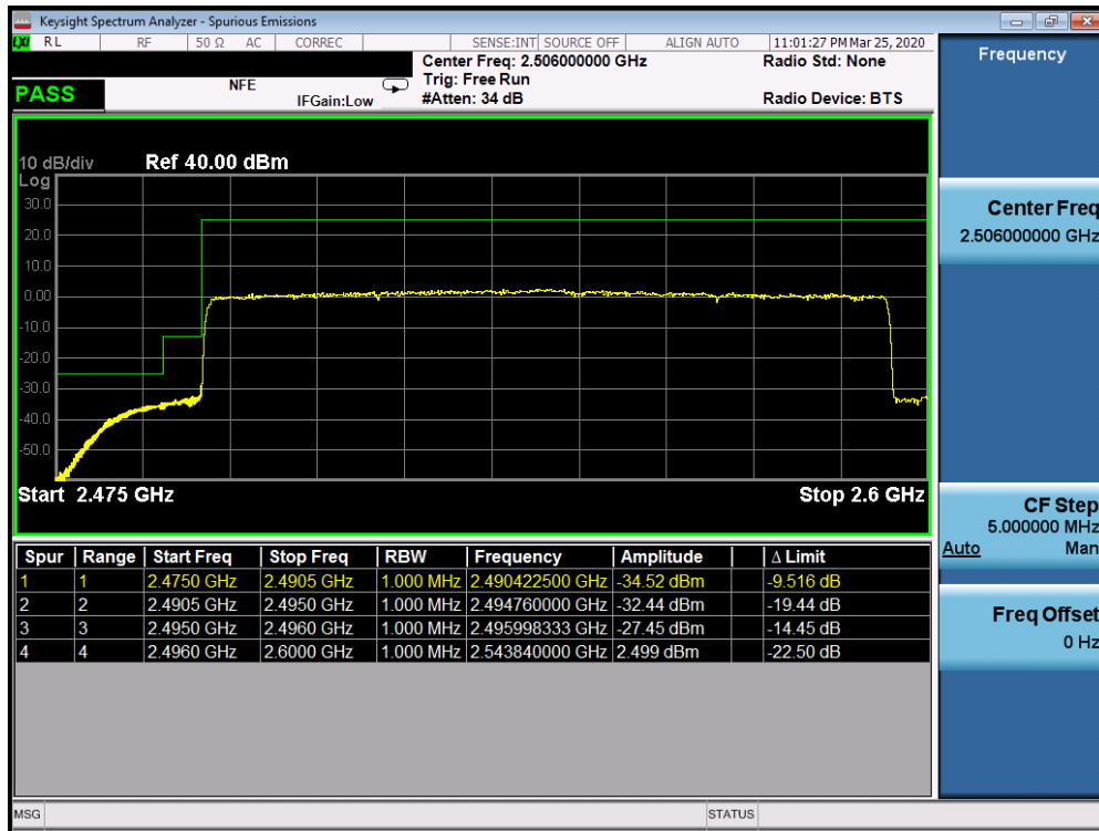
Plot 7-47. Lower Band Edge Plot (n41 - 100MHz DFT-s-OFDM-BPSK - Full RB Configuration)
