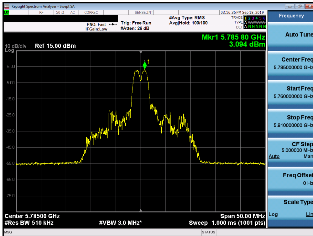
Plot 7-185. Power Spectral Density Plot MIMO ANT1 (20MHz BW 802.11ax – Full Tones (UNII Band 3) – Ch. 157)
