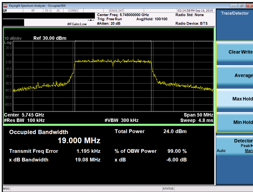
Plot 7-109. 6dB Bandwidth Plot SISO ANT1 (20MHz BW 802.11ax (UNII Band 3) – Ch. 149)
