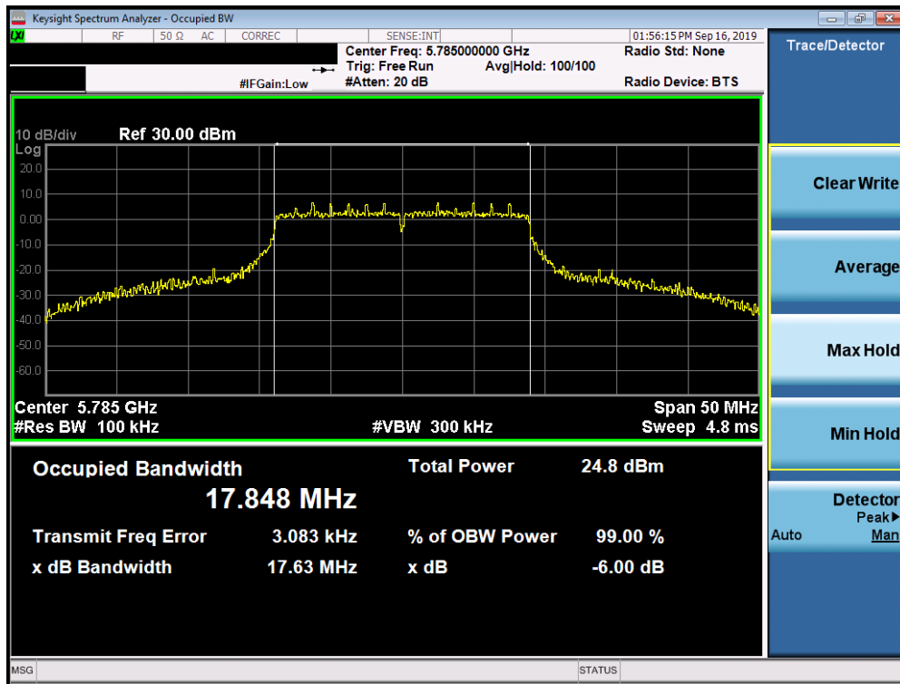
Plot 7-107. 6dB Bandwidth Plot SISO ANT1 (20MHz BW 802.11n (UNII Band 3) – Ch. 157)
