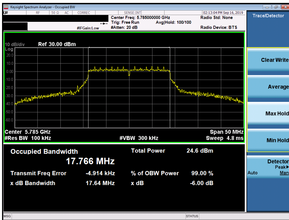
Plot 7-122. 6dB Bandwidth Plot SISO ANT2 (20MHz BW 802.11n (UNII Band 3) – Ch. 157)
