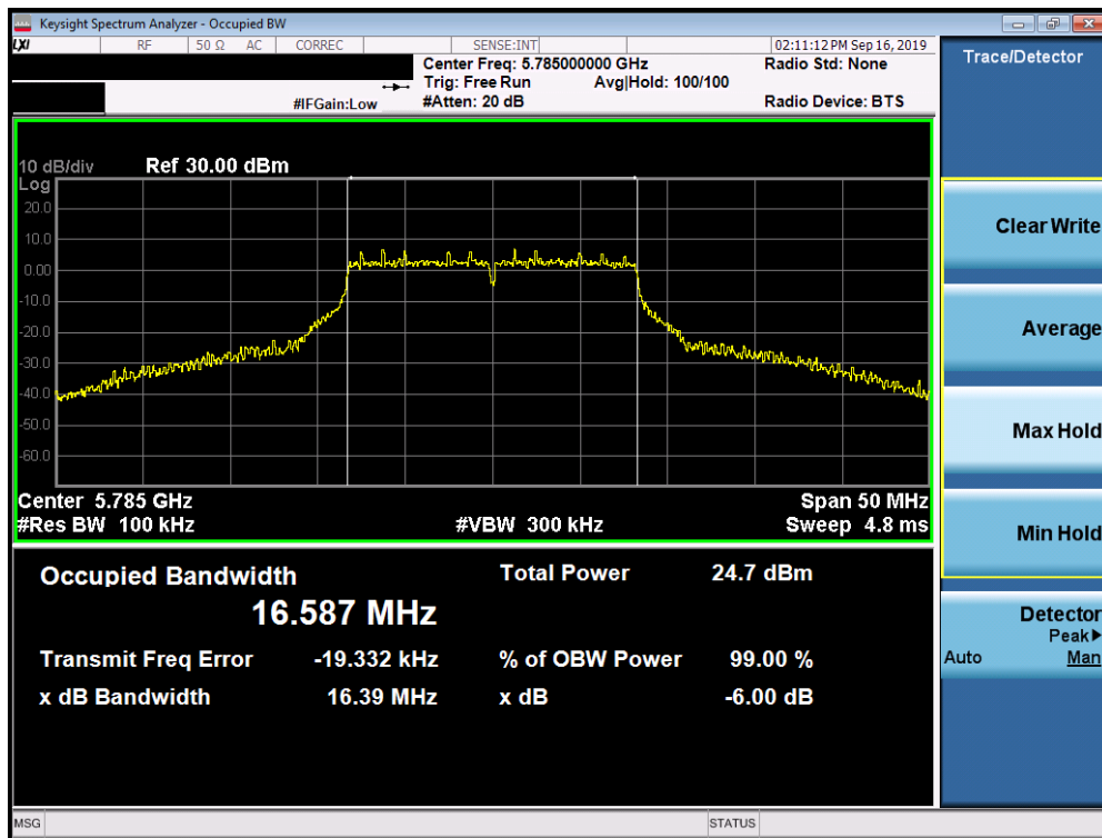
Plot 7-119. 6dB Bandwidth Plot SISO ANT2 (802.11a (UNII Band 3) – Ch. 157)
