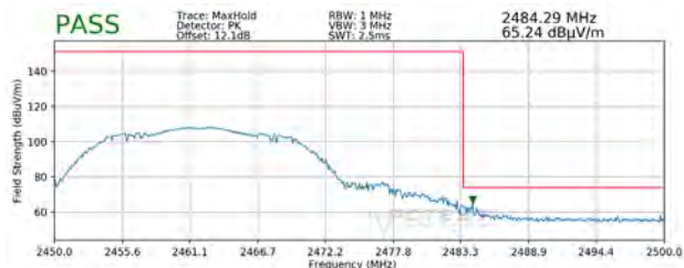
Plot 7-94. Radiated Restricted Band Edge Measurement SISO ANT1 with WCP (Peak)
