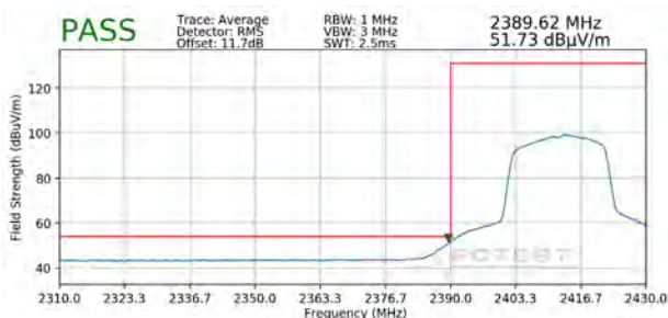
Plot 7-101. Radiated Restricted Lower Band Edge Measurement MIMO (Average)
