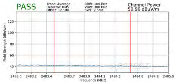
Plot 7-105. Radiated Restricted Band Edge Measurement MIMO with WCP (Average)
