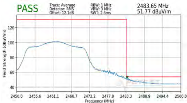
Plot 7-103. Radiated Restricted Upper Band Edge Measurement MIMO (Average)
