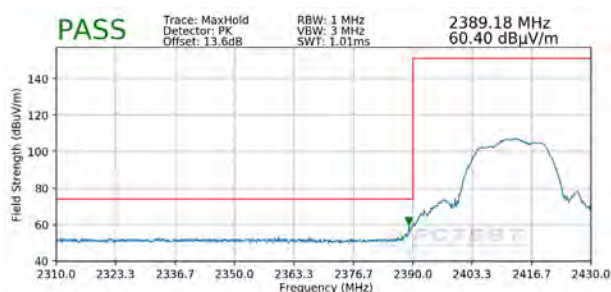
Plot 7-90. Radiated Restricted Lower Band Edge Measurement SISO ANT1 (Peak)
