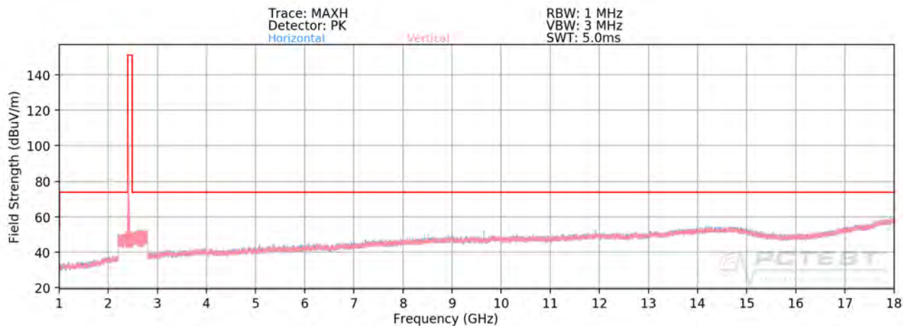
Plot 7-77. Radiated Spurious Plot above 1GHz SISO ANT1 (802.11b – Ch. 1)
