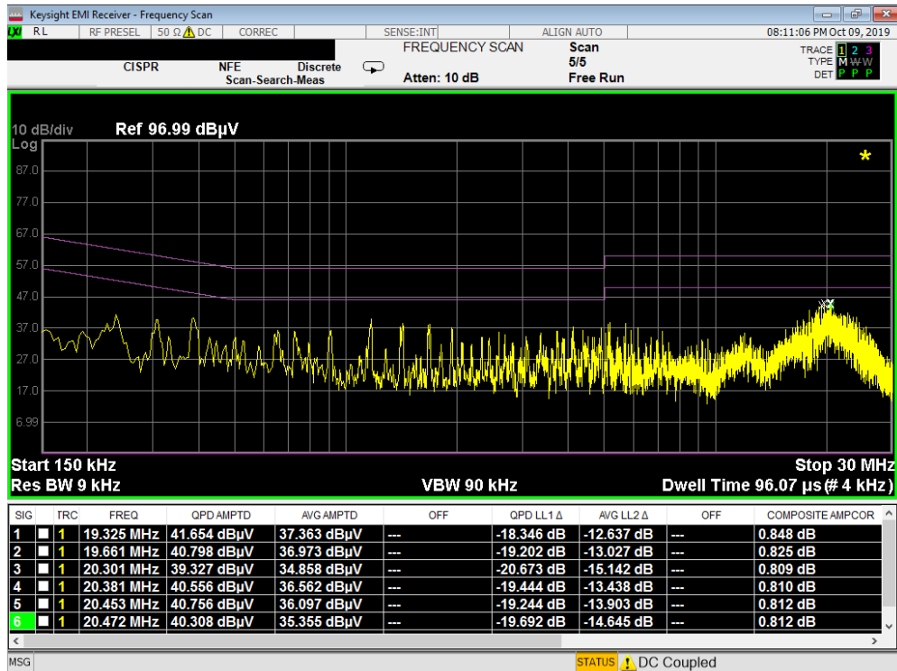
Plot 7-111. Line Conducted Plot with 802.11b (L1) with WCP
