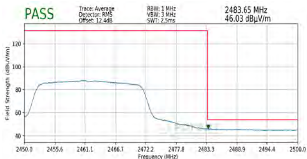
Plot 7-99. Radiated Restricted Band Edge Measurement SISO ANT2 with WCP (Average)
