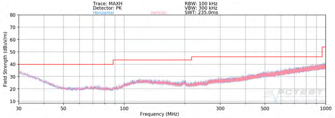
Plot 7-107. Radiated Spurious Plot below 1GHz SISO ANT1
