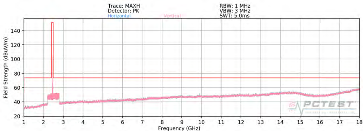
Plot 7-79. Radiated Spurious Plot above 1GHz SISO ANT1 (802.11b – Ch. 11)
