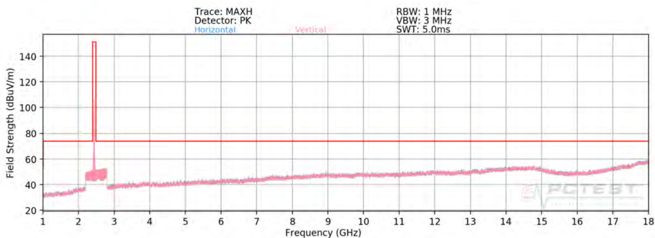
Plot 7-78. Radiated Spurious Plot above 1GHz SISO ANT1 (802.11b – Ch. 6)
