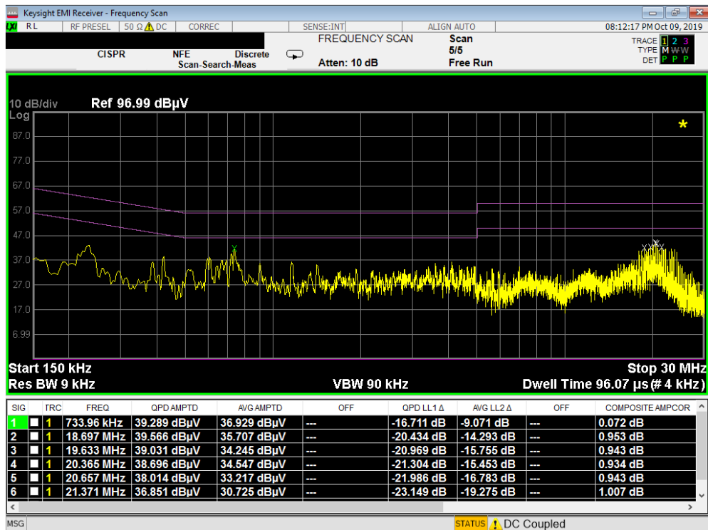
Plot 7-112. Line Conducted Plot with 802.11b (N) with WCP
