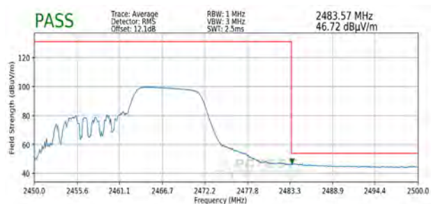
Plot 7-91. Radiated Restricted Upper Band Edge Measurement SISO ANT1 (Average)
