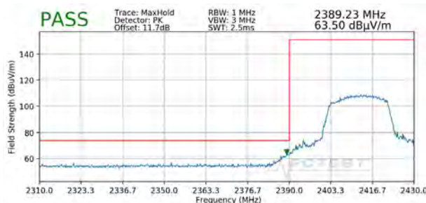
Plot 7-102. Radiated Restricted Lower Band Edge Measurement MIMO (Peak)
